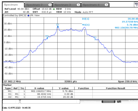
Figure 7.3.2-7: 20dB BW Low Channel – 50kbps
