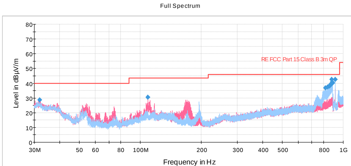
Figure A-3: Radiated Emissions – 30MHz-1GHz
