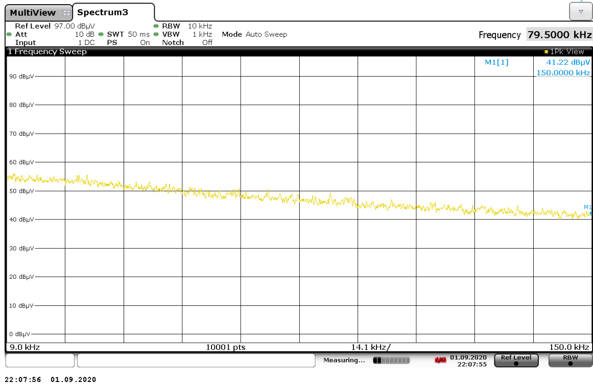
Figure A-1: Radiated Emissions – 9kHz-150kHz
