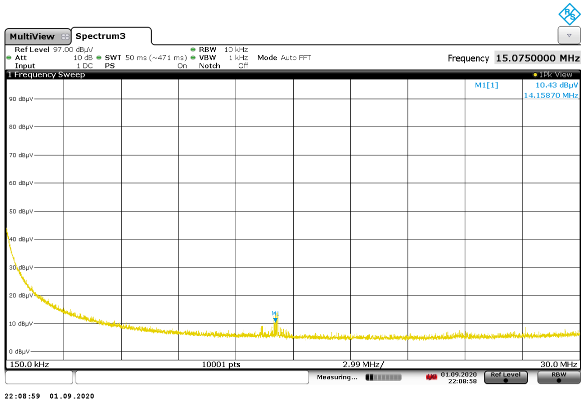
Figure A-2: Radiated Emissions – 150kHz-30MHz
