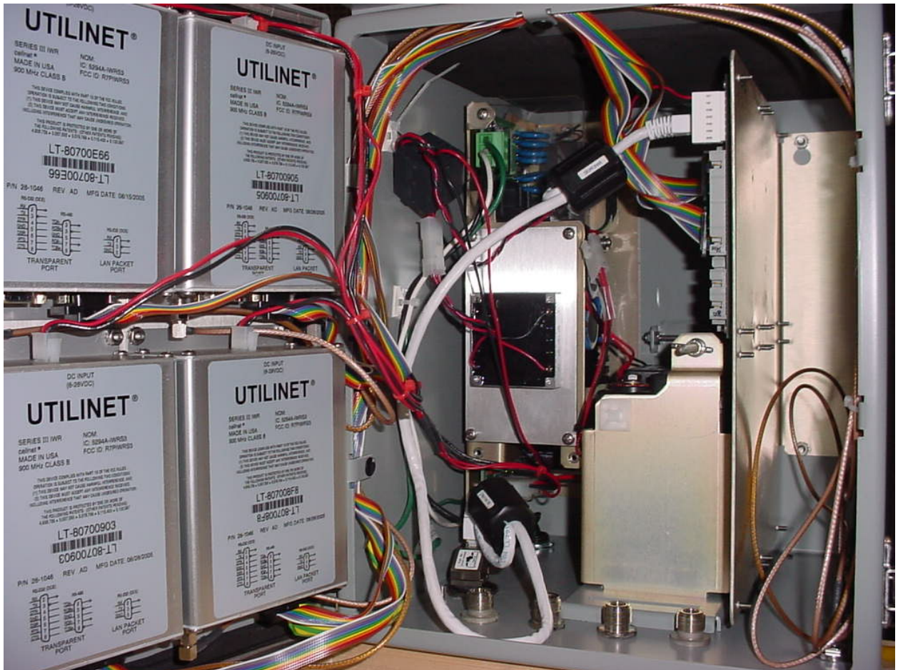
Figure 1: Shielded internal Ethernet cable with two Fair-Rite brand ferrites, 0444164181, with two turns each. Each of the ferrites were situated close to the cable ends.
