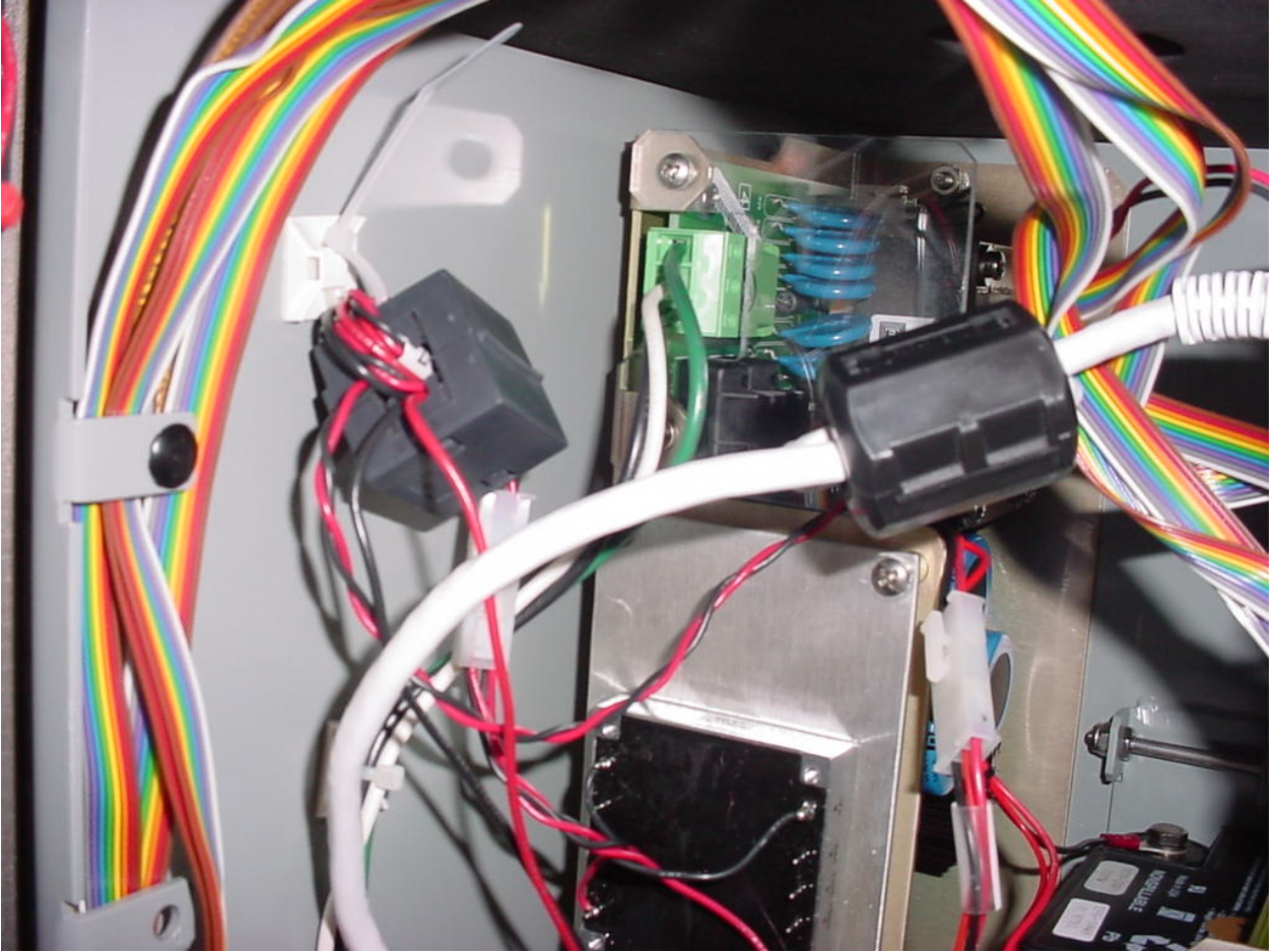
Figure 3: Internal power leads, Red and Black, with one Fair-Rite brand ferrite, 0443164151, with three turns. Ferrite situated halfway between the supply board and the processor board against the inside wall.
