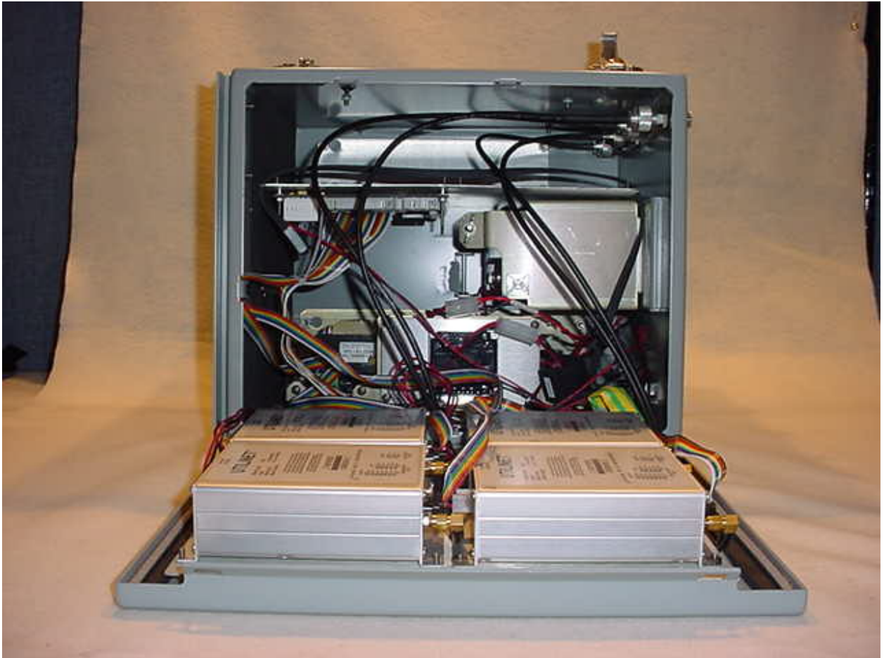
Figure 1: Internal – Enclosure
