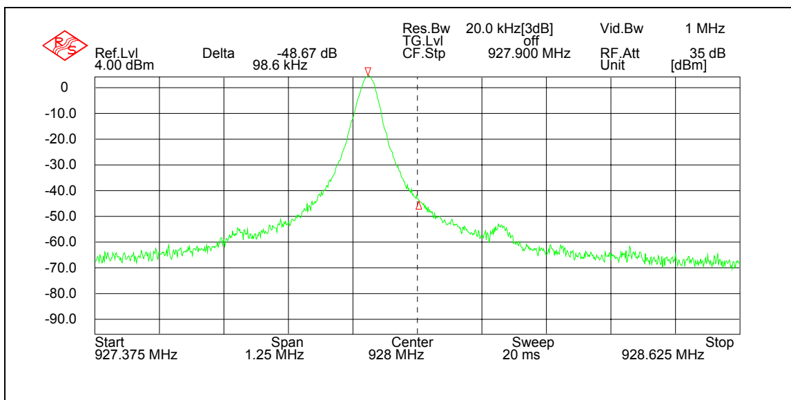
Figure 7.6.1.2-1: Lower Band-edge
