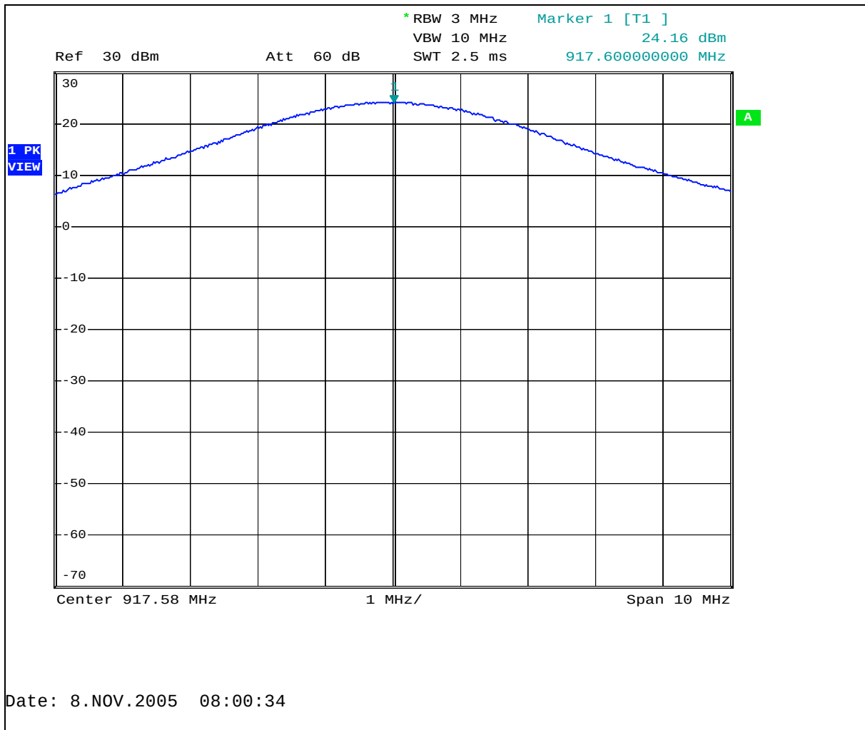
Figure 7.5.2-1: Output power
