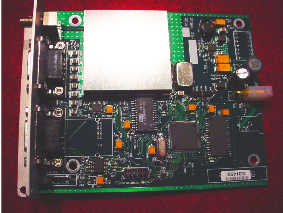
Figure 1: PCB Front
