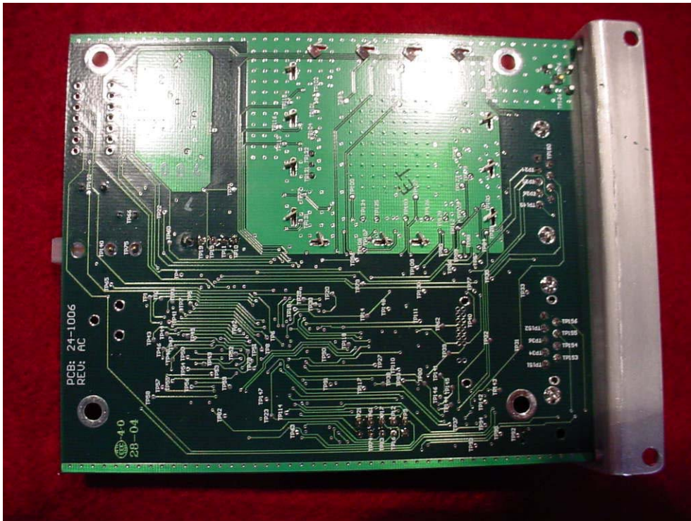
Figure 2: PCB Rear
