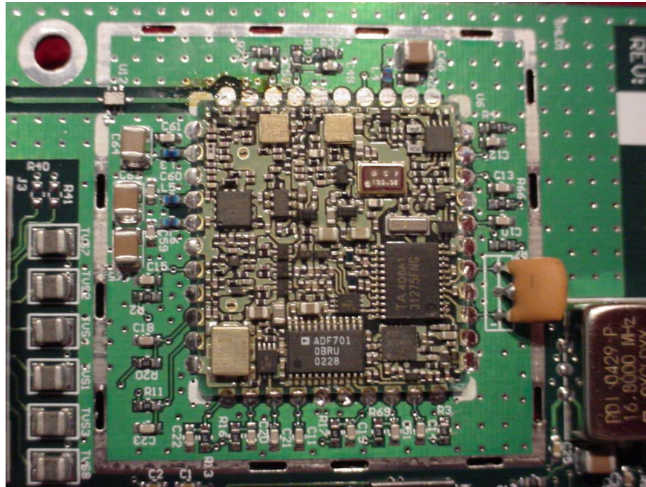
Figure 3: RF Circuitry - Front
