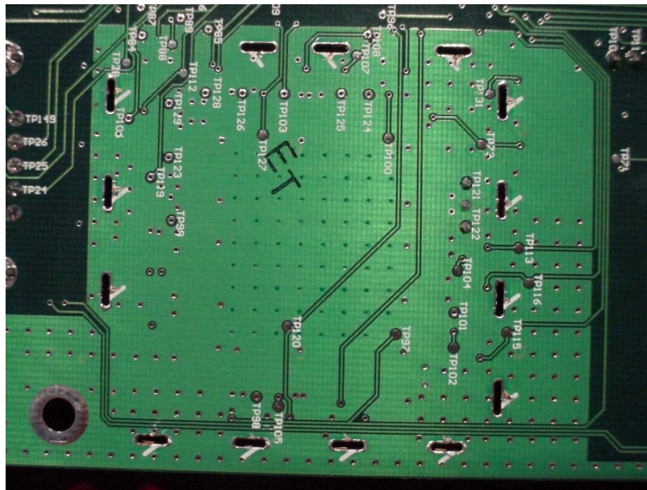
Figure 4: RF Circuitry - Rear
