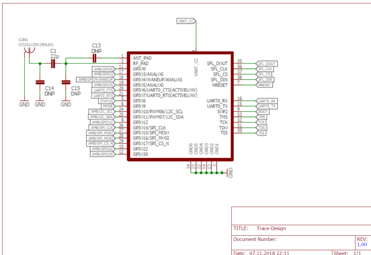
Figure 30: Close-up Schematic
