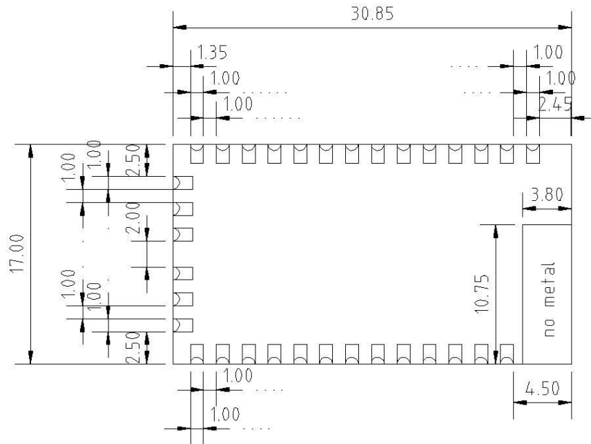
Figure 3: Dimensions [mm]
