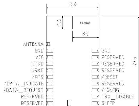
Figure 1 Pinout
