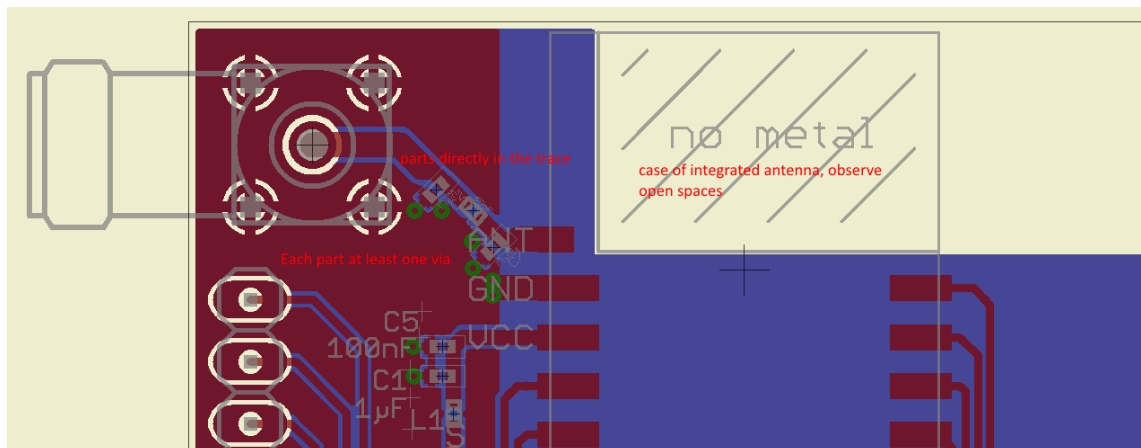
Figure 8: Layout
