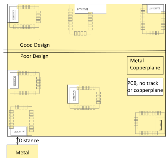
Figure 9: Placement of the module with integrated antenna
