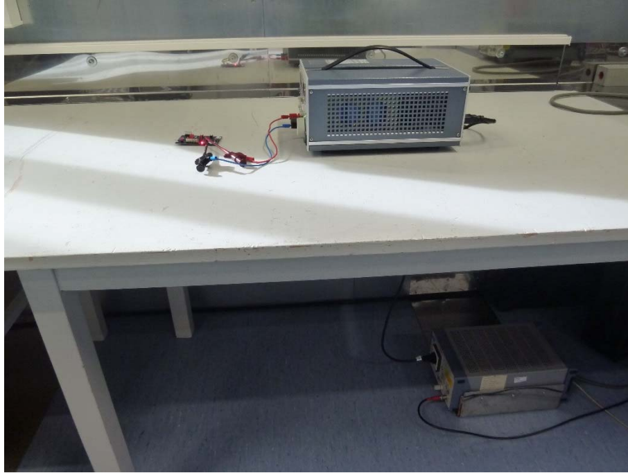
Photo 9: AC conducted test setup
