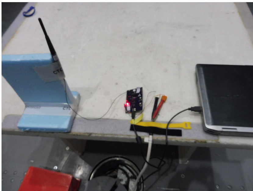
Photo 18: EUT at the semi-anechoic chamber, module with external antenna
