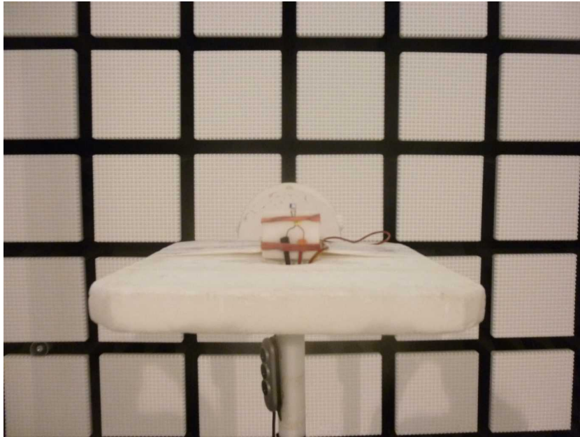
Photo 5: EUT at the anechoic chamber, stand-alone module with integrated antenna
