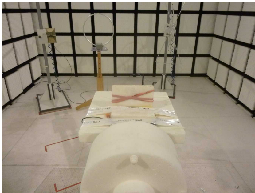
Photo 10: EUT at the anechoic chamber, module with external antenna
