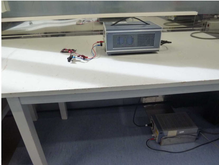
Photo 19: AC conducted test setup
