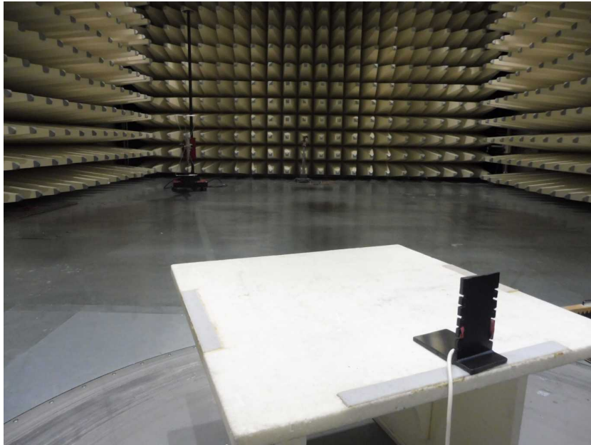
Photo 15: EUT at the semi-anechoic chamber, stand-alone module with integrated antenna
