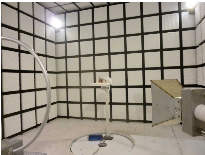
Photo 14: EUT at the anechoic chamber, module with external antenna
