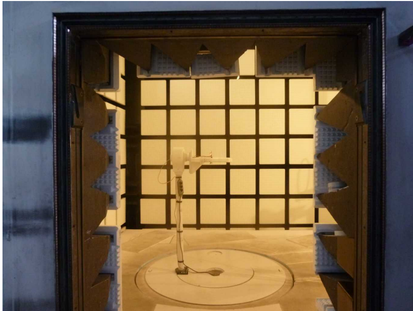
Photo 1: EUT at the anechoic chamber, stand-alone module with integrated antenna
