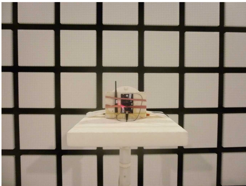
Photo 12: EUT at the anechoic chamber, module with external antenna
