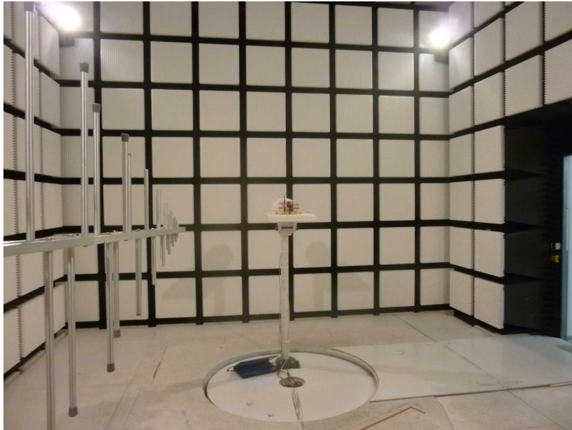
Photo 13: EUT at the anechoic chamber, module with external antenna
