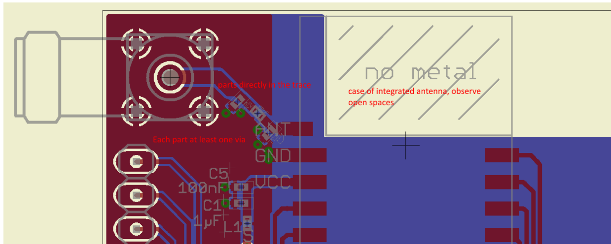
Figure 4 Layout
