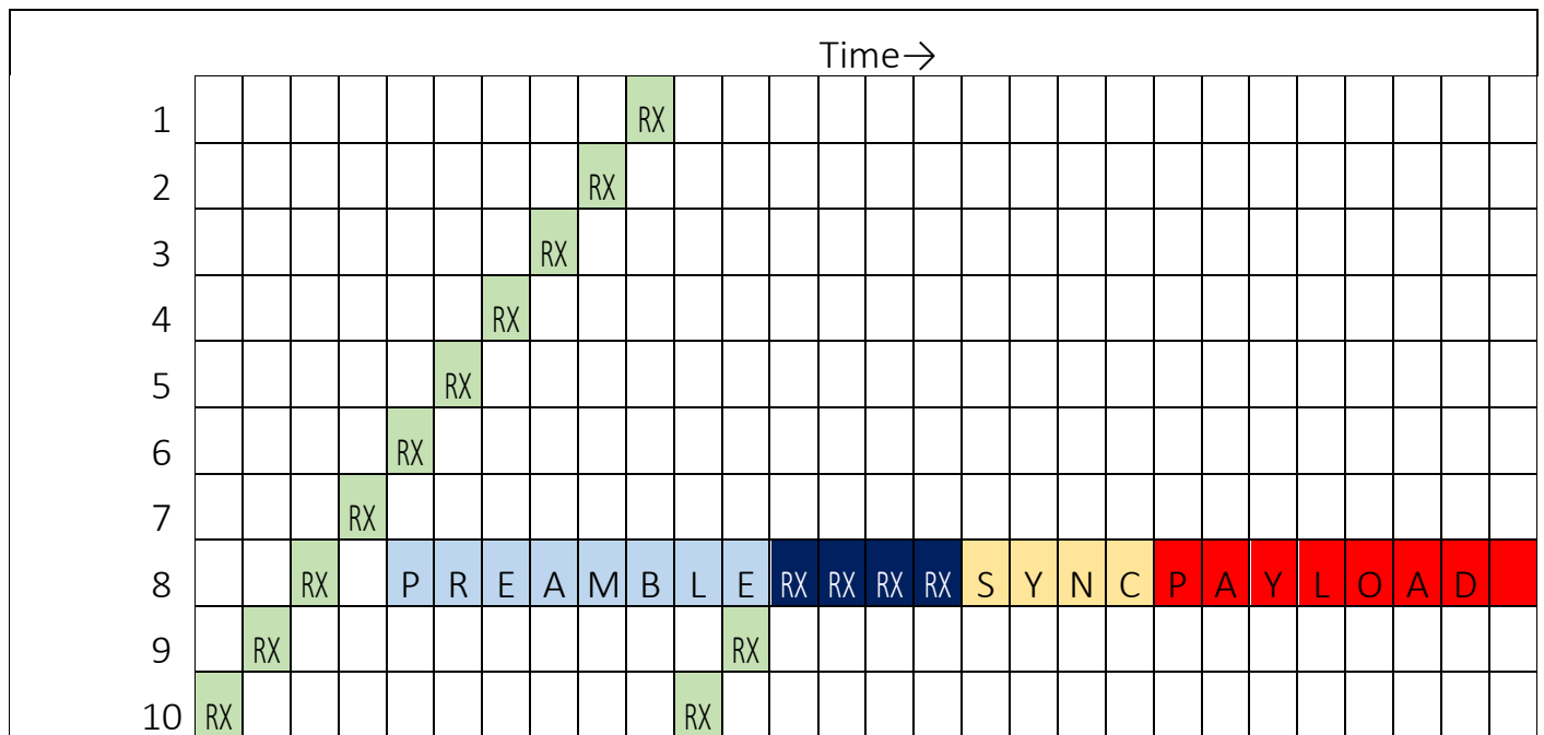
Figure 2 Channel hopping for a 10 channel system
