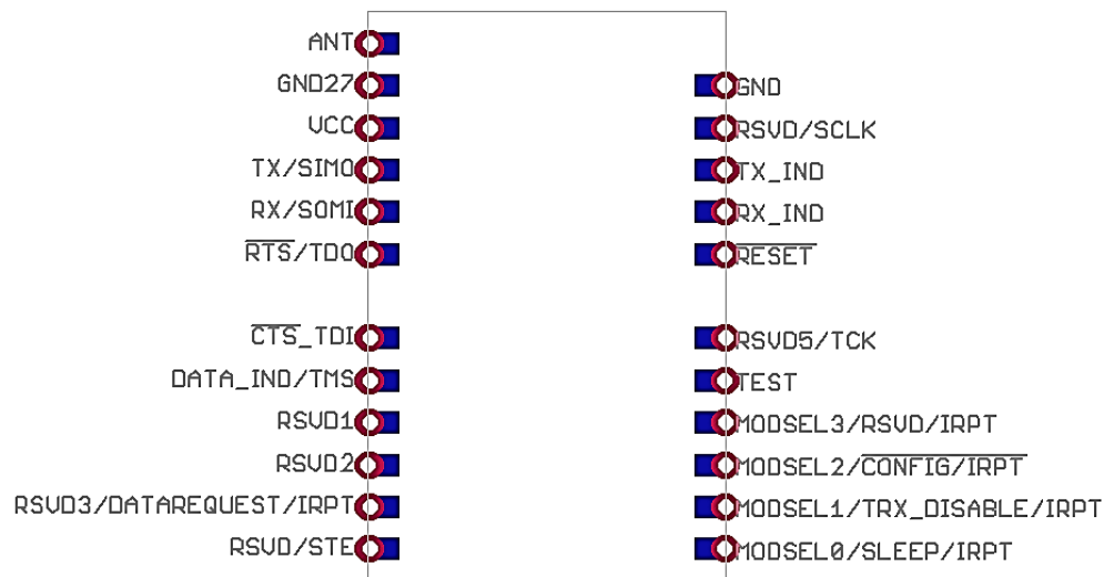
Figure 1 Pinout
