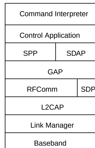
Figure 2. Bluetooth Protocol Stack
