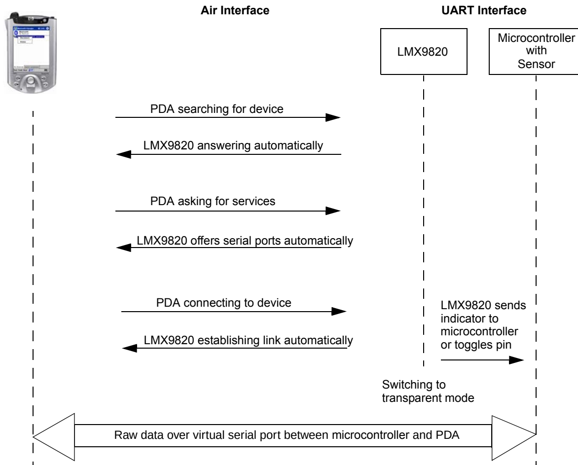
Figure 3. Point-to-Point Connection
