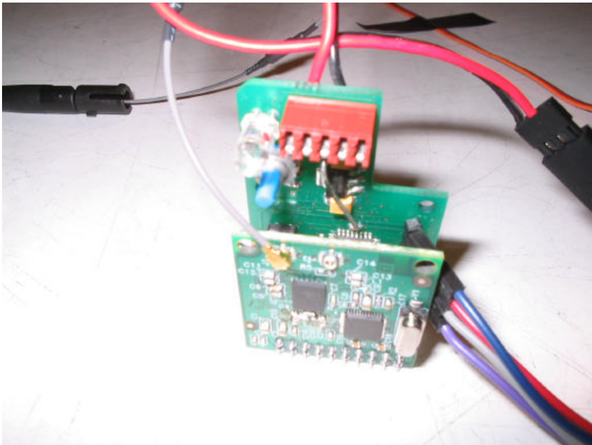
close-up of EUT with antenna horizontal
