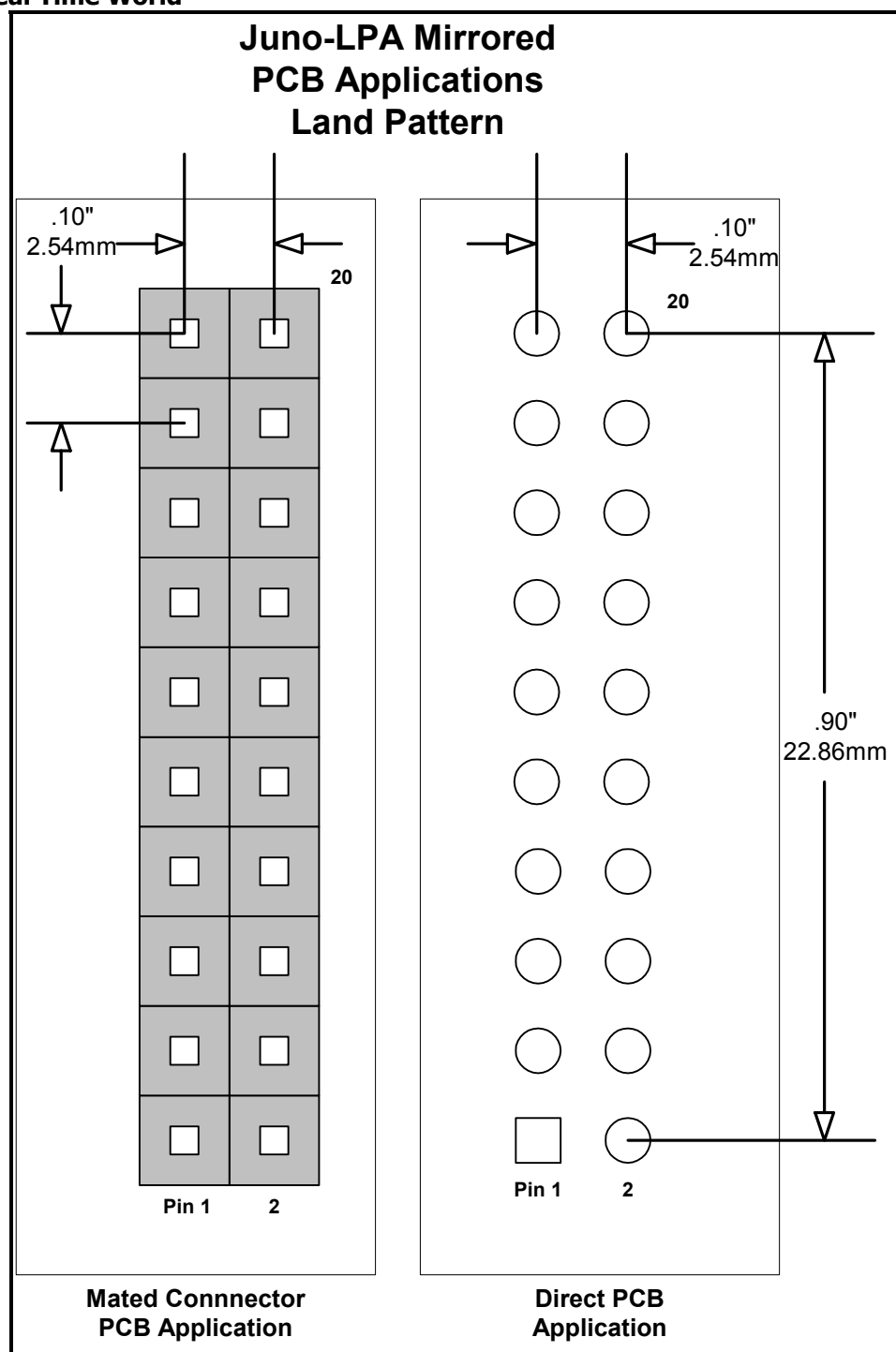
Figure 2 – Juno-LPA Mirrored Land Pattern
