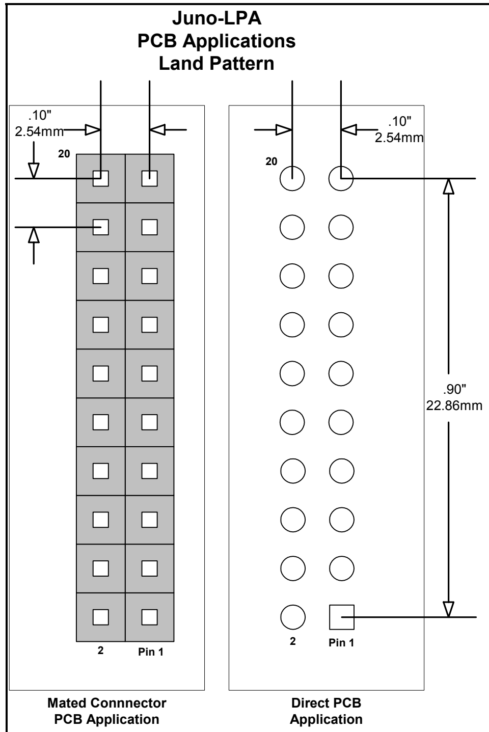
Figure 1 – Juno-LPA Land Pattern
