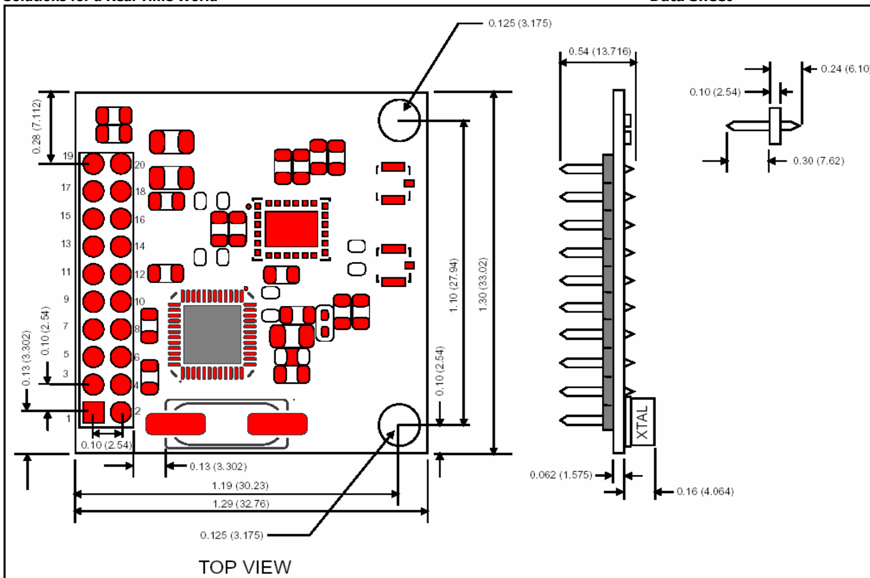
Figure 4 – Juno-LPA Mirrored Dimensions
