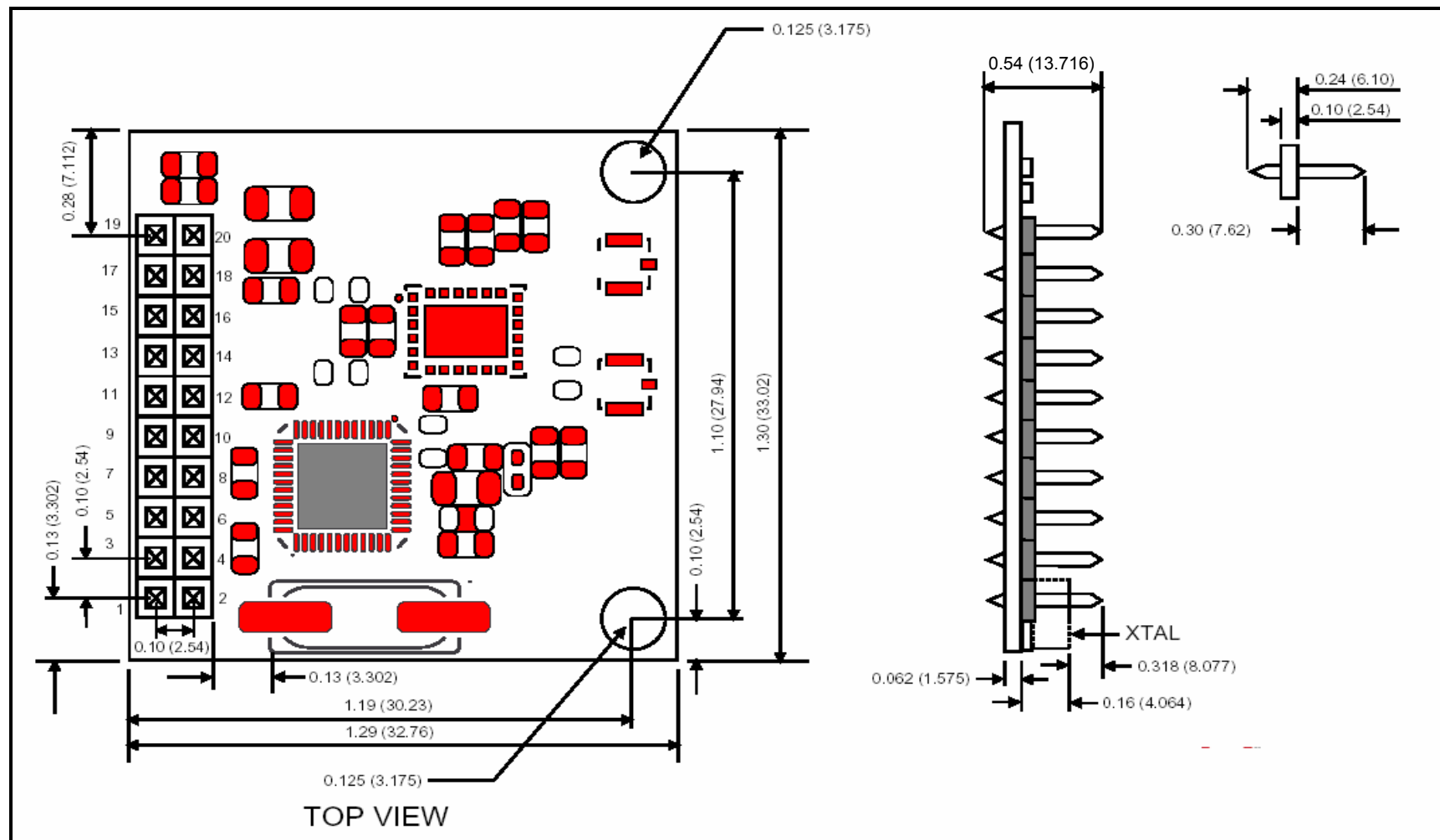
Figure 3 – Juno-LPA Dimensions
