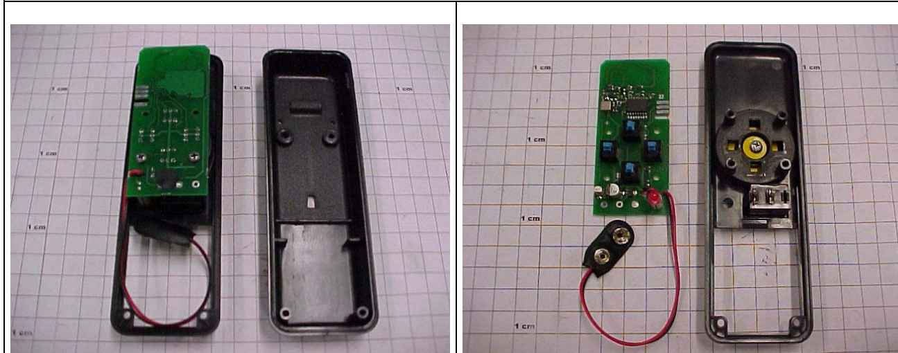
PHOTO N° 2 – INTERNAL VIEW
