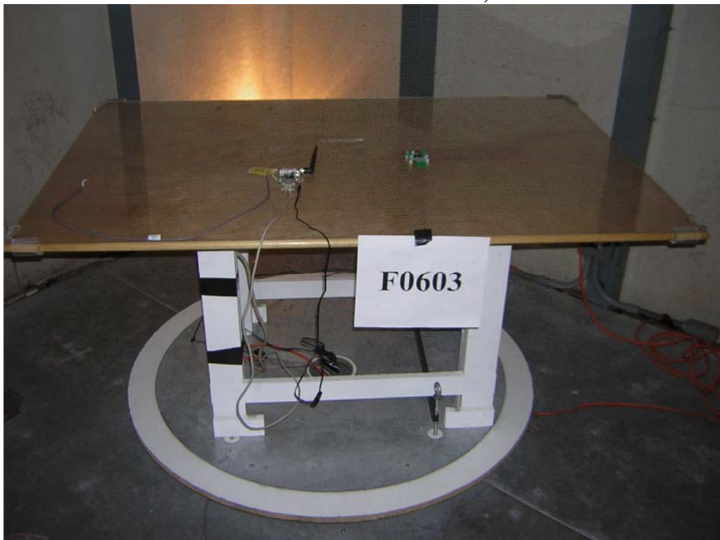
Spurious Emissions
