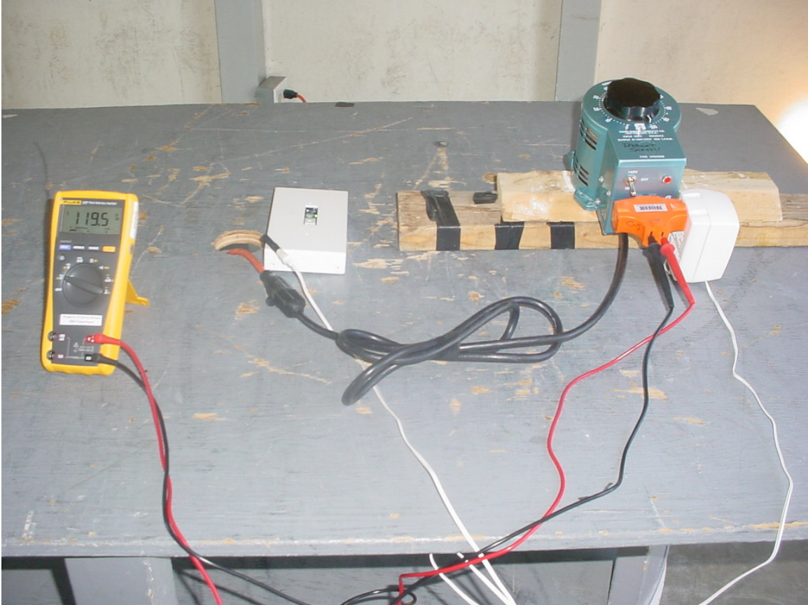
Voltage Variation
