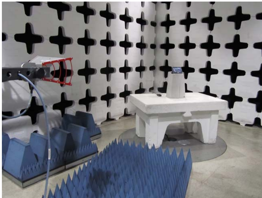
Photo 5. Radiated emissions up to 15GHz test setup.
