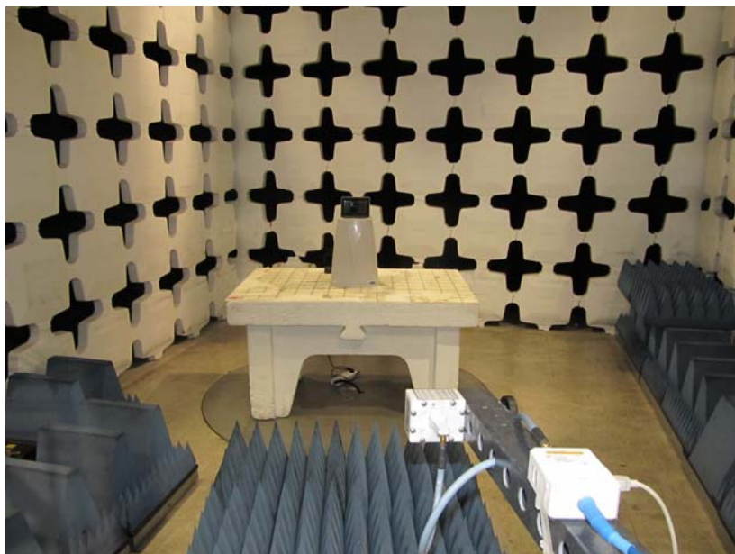
Photo 6. Radiated emissions test 15-26GHz test setup.
