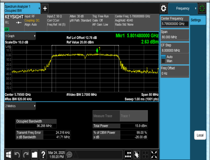
11AC40SISO-Ant2-5795
