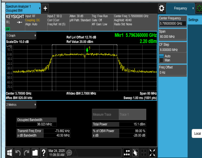
11AC40SISO-Ant1-5795
