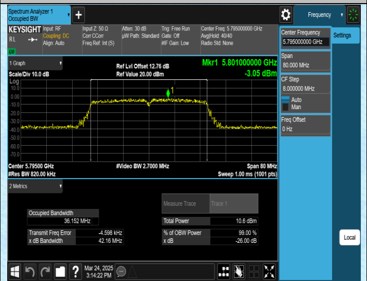
11AC40MIMO-Ant2-5795
