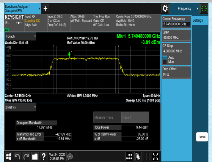
11AC20MIMO-Ant2-5745
