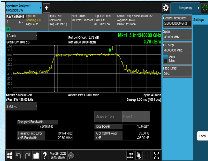
11AC20SISO-Ant1-5805
