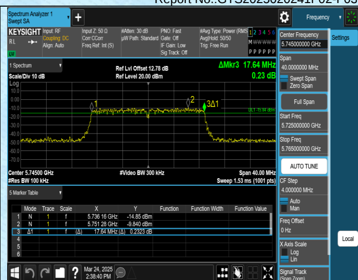
11AC20MIMO-Ant2-5745-PASS
