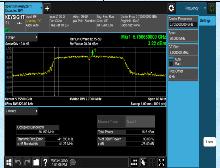
11AC40SISO-Ant2-5755
