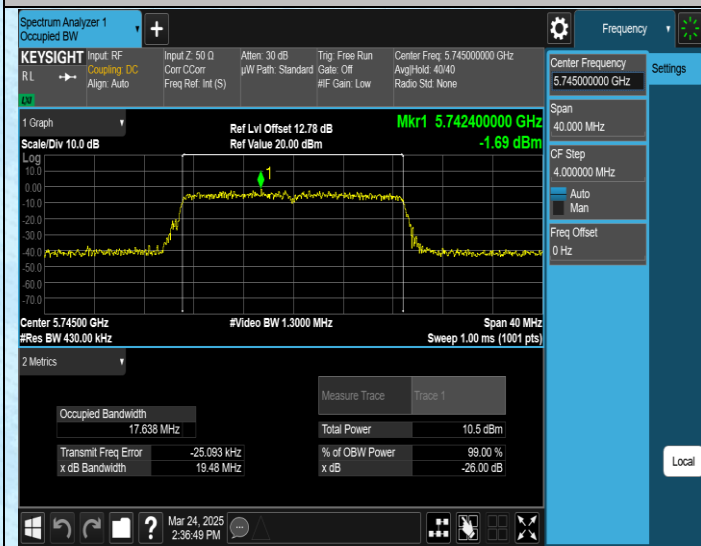
11AC20MIMO-Ant1-5745
