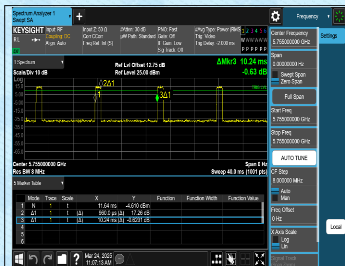
NTNV-11AC40SISO-Ant1-5755
