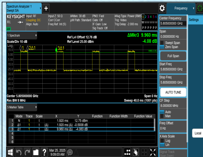
NTNV-11AC20MIMO-Ant1-5805
