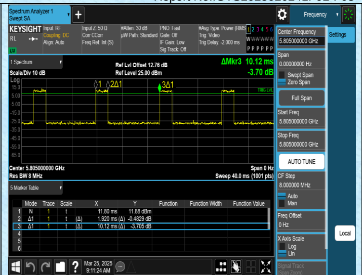
NTNV-11AC20MIMO-Ant2-5805
