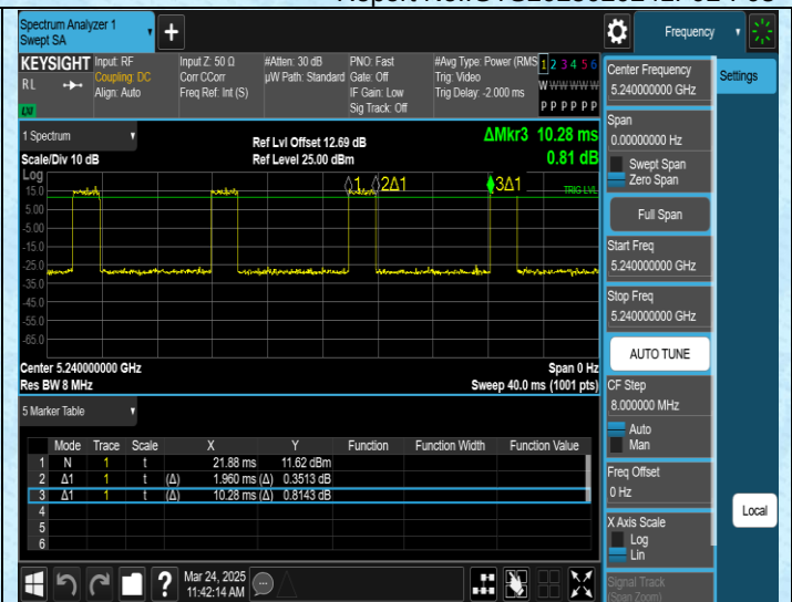
NTNV-11AC20SISO-Ant2-5240
