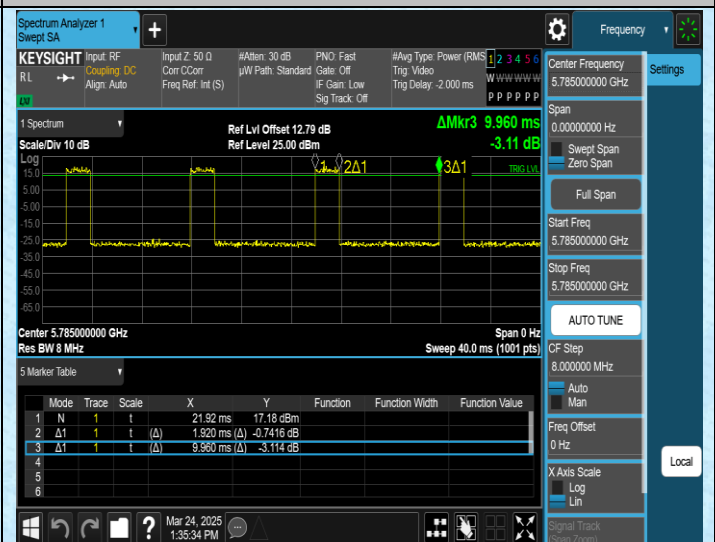
NTNV-11AC20SISO-Ant2-5785
