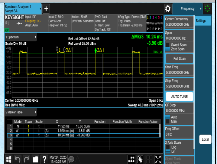
NTNV-11AC20SISO-Ant2-5200
