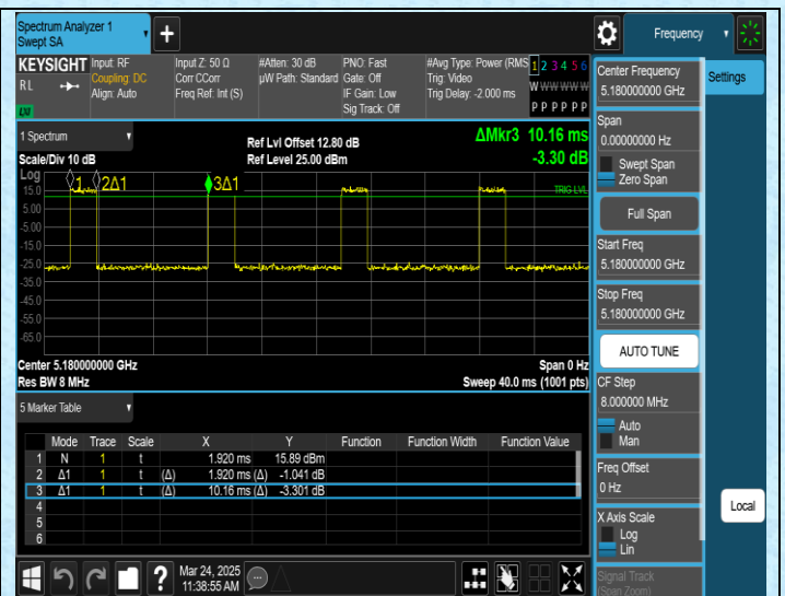
NTNV-11AC20SISO-Ant2-5180
