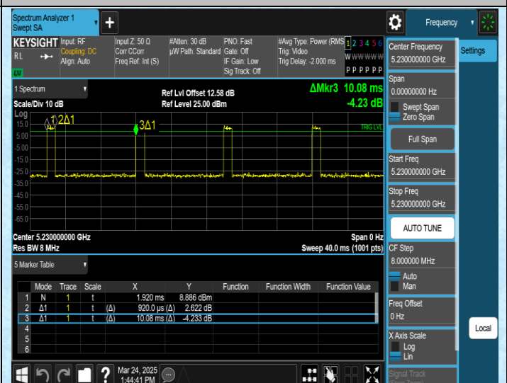
NTNV-11AC40SISO-Ant2-5230
