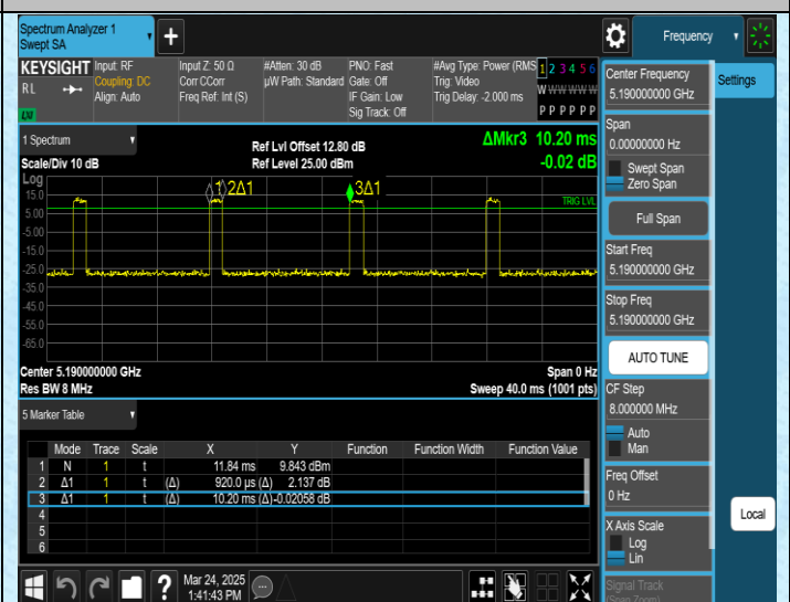
NTNV-11AC40SISO-Ant2-5190
