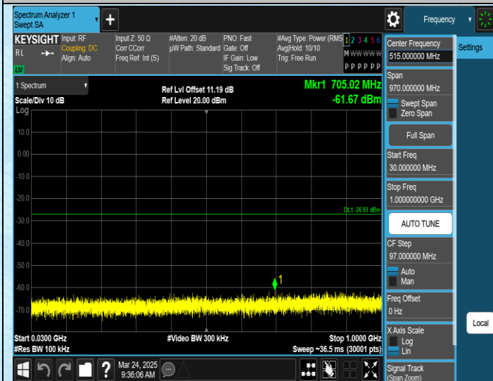
11N20SISO-Ant2-2462-30~1000-PASS
