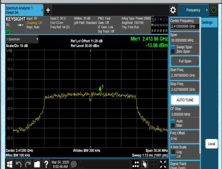
11N20MIMO-Ant2-2412-0~Reference-PASS
