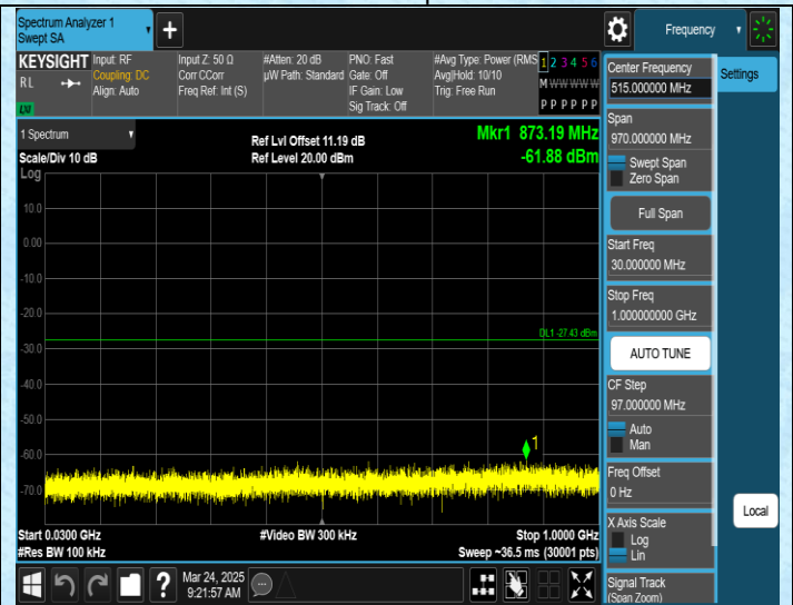
11N20SISO-Ant1-2462-30~1000-PASS
