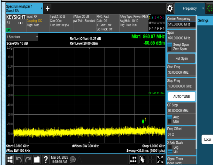
11N20MIMO-Ant2-2437-30~1000-PASS
