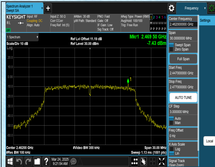
11N20SISO-Ant1-2462-0~Reference-PASS
