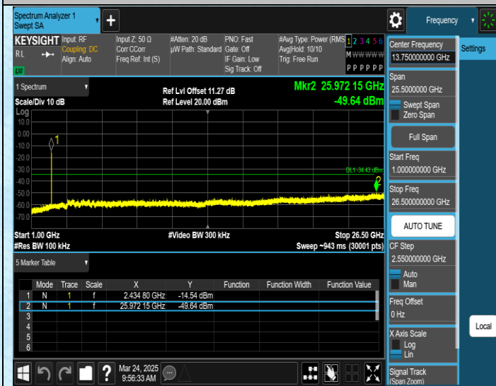
11N20MIMO-Ant1-2437-1000~26500-PASS
