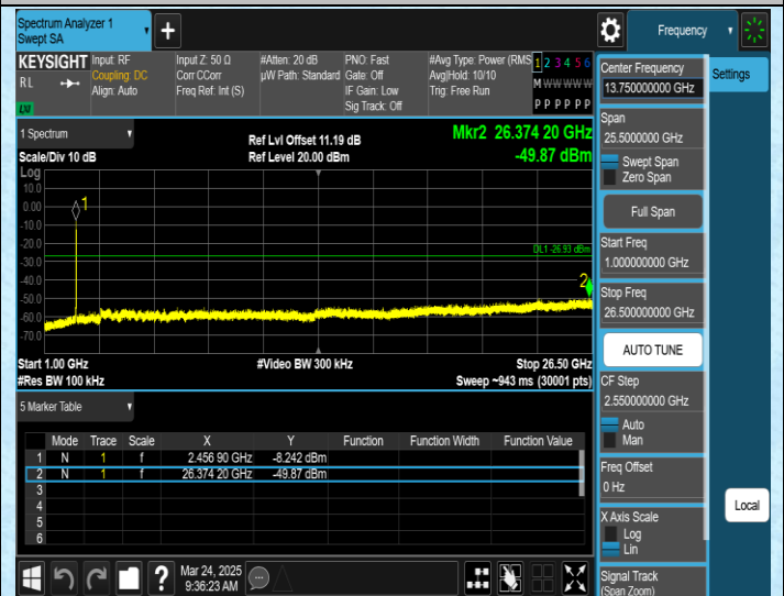
11N20SISO-Ant2-2462-1000~26500-PASS
