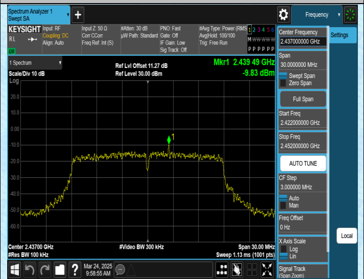
11N20MIMO-Ant2-2437-0~Reference-PASS
