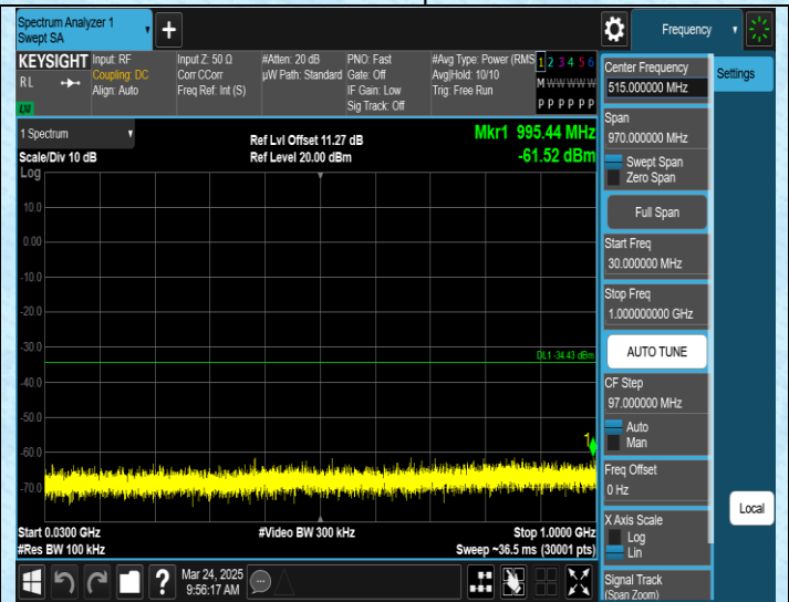
11N20MIMO-Ant1-2437-30~1000-PASS
