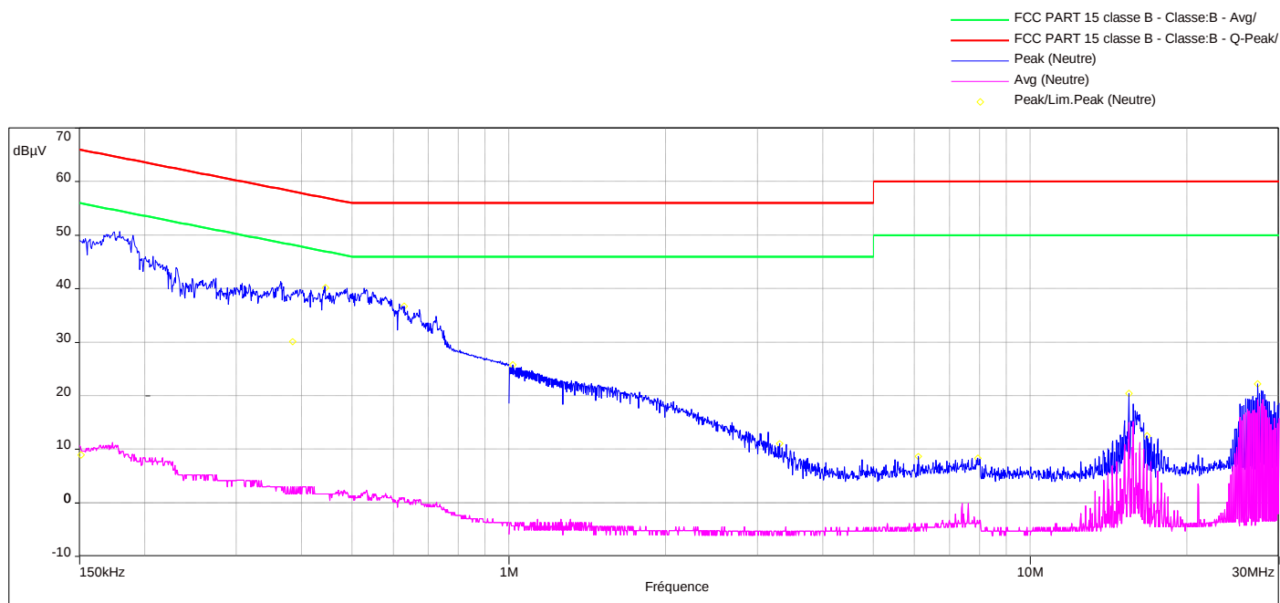
Diagram N°2 Neutral 240V/50Hz
