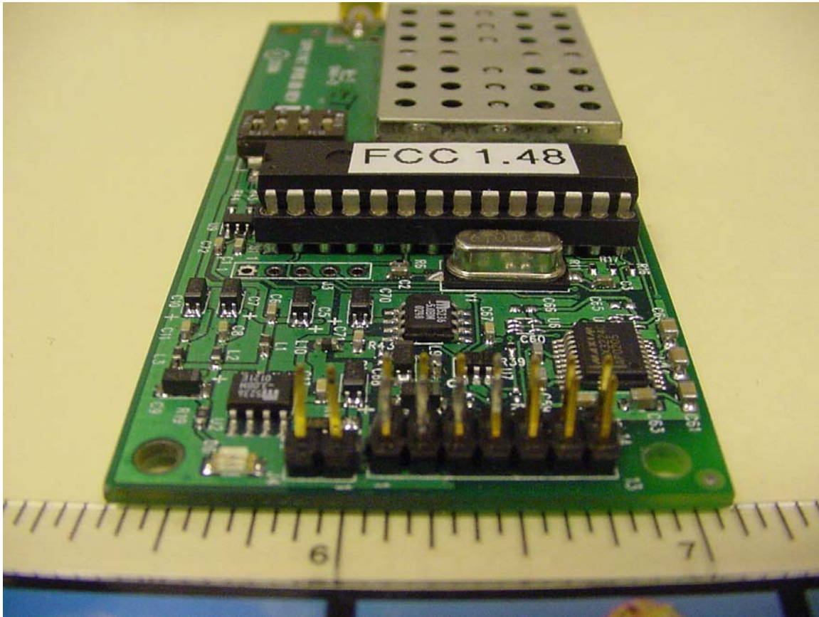
Side view showing data/power interface connector
