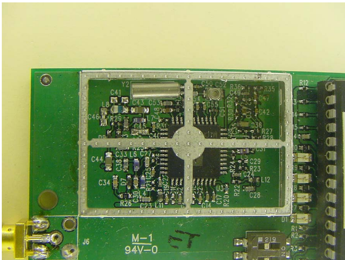
RF section with top shield removed.
