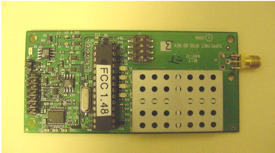
Component Side
