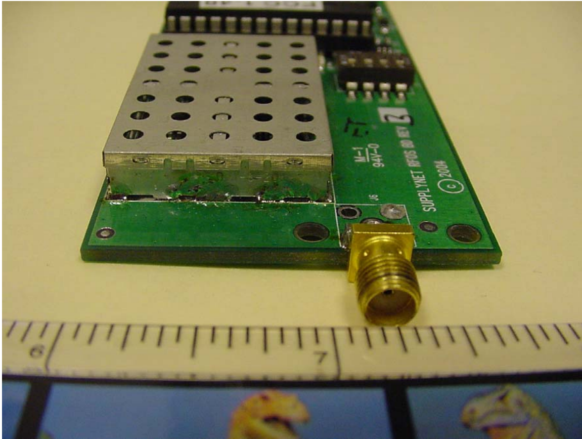
Side view of EUT showing SMA RF antenna connector
