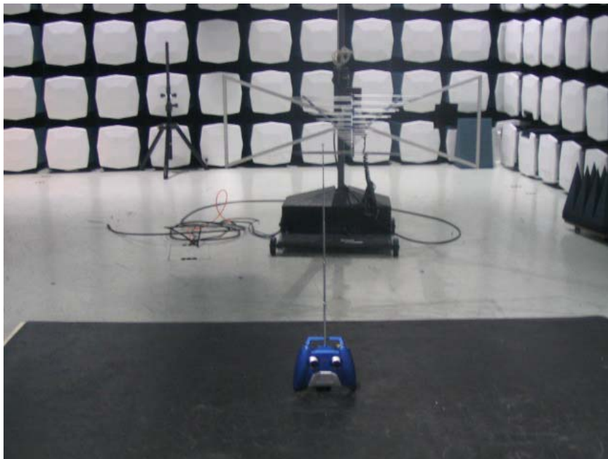
Photo of Emissions within Band Edges Test
