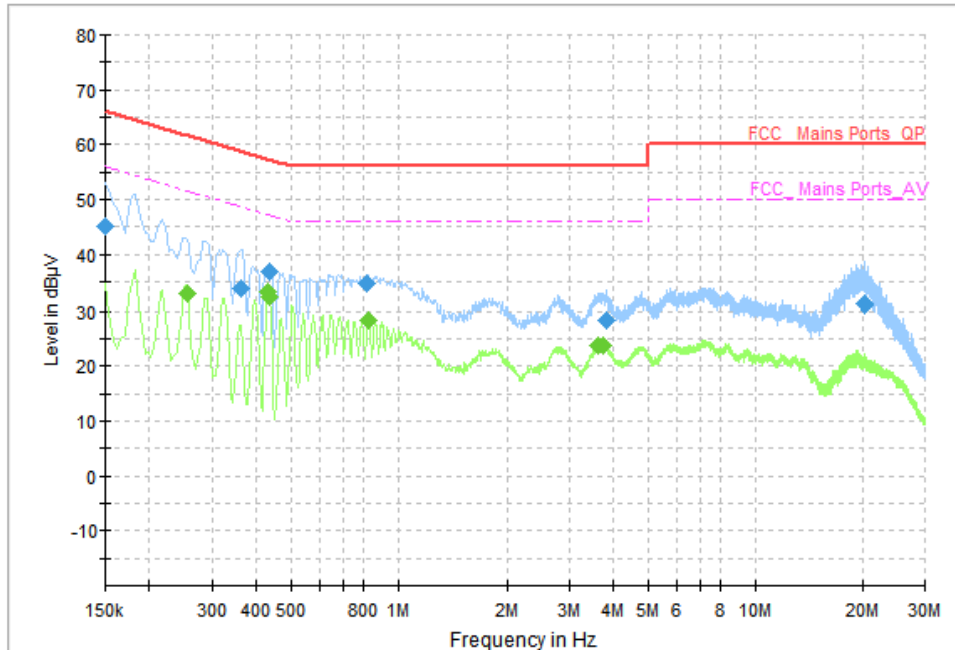
Fig. 80 AC Power line Conducted Emission (Idle)
