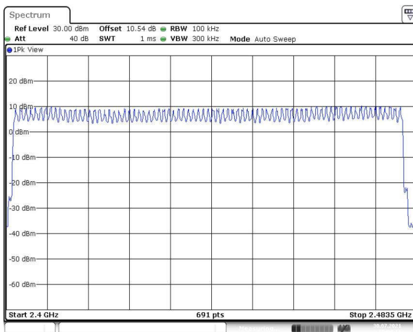
Fig. 74 Number of Hopping Channels ( \pi/4 DQPSK, CH39)
