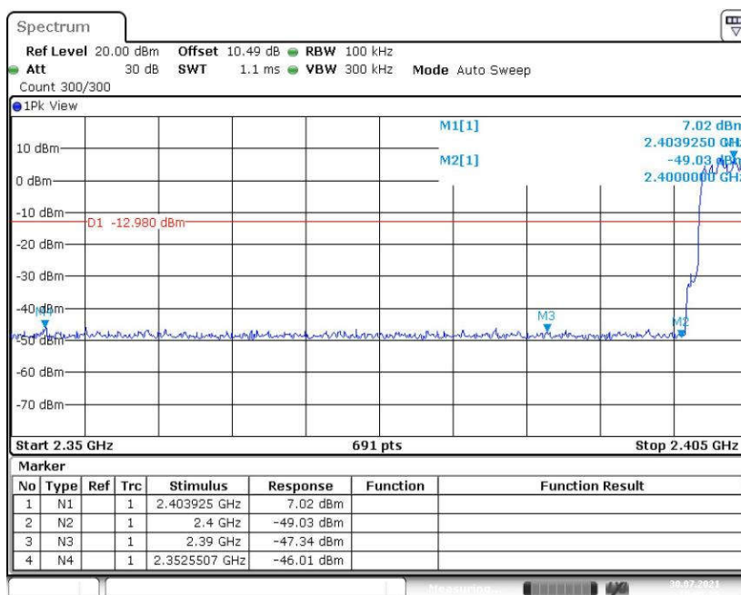
Fig. 5 Band Edges (8DPSK, CH0, Hopping ON)
