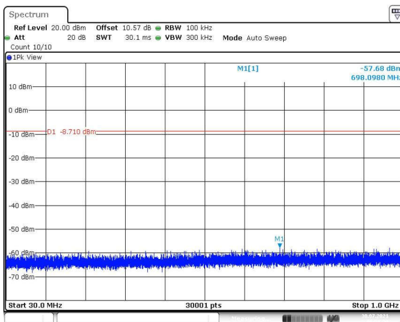
Fig. 17 Conducted Spurious Emission (GFSK, CH39, 30MHz -1GHz)
