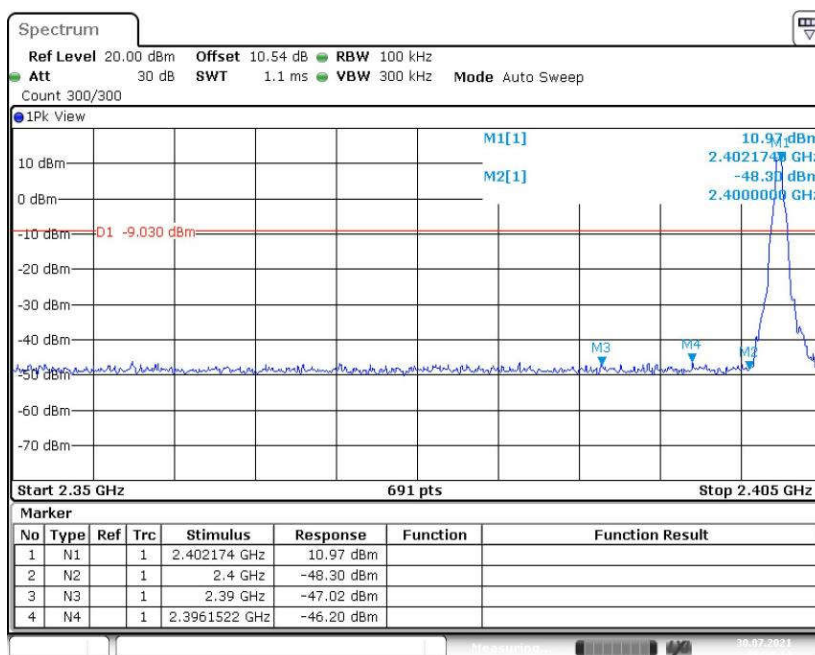
Fig. 7 Band Edges (GFSK, CH0, Hopping OFF)
