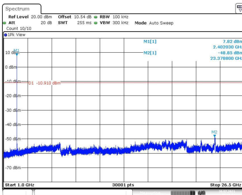
Fig. 33 Conducted Spurious Emission (8DPSK, CH0, 1GHz-26.5GHz)
