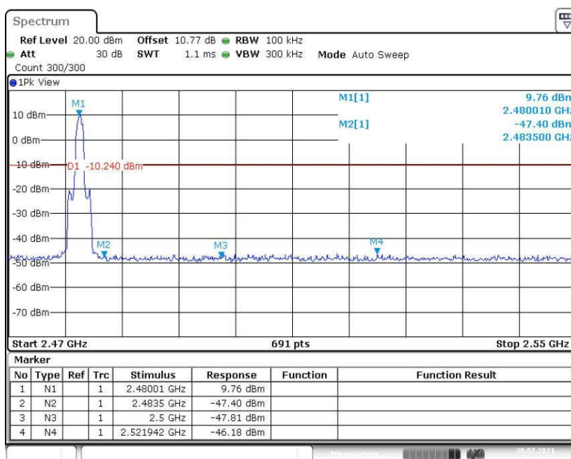
Fig. 12 Band Edges (8DPSK, CH78, Hopping OFF)
