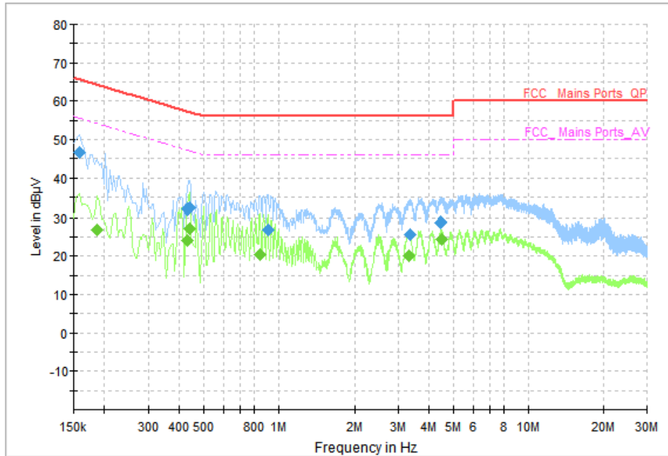
Fig. 79 AC Power line Conducted Emission (Traffic)
