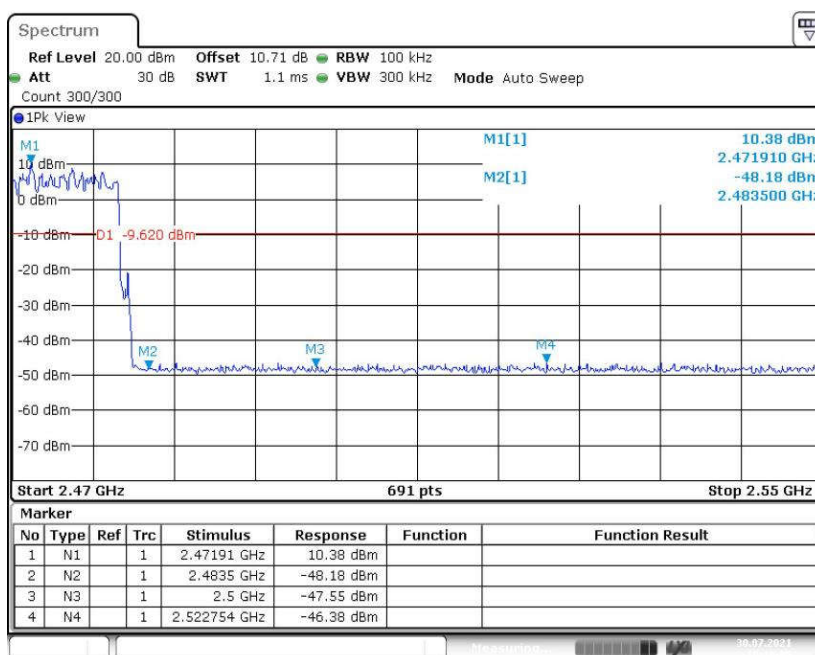
Fig. 6 Band Edges (8DPSK, CH78, Hopping ON)
