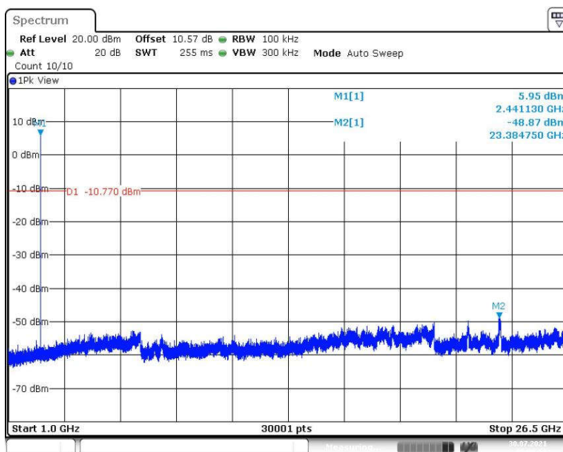
Fig. 27 Conducted Spurious Emission ( \pi/4 DQPSK, CH39, 1GHz-26.5GHz)
