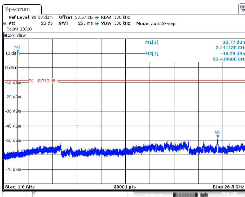
Fig. 18 Conducted Spurious Emission (GFSK, CH39, 1GHz-26.5GHz)
