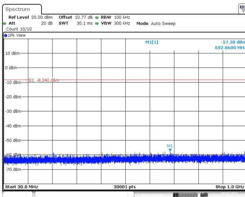
Fig. 20 Conducted Spurious Emission (GFSK, CH78, 30MHz -1GHz)
