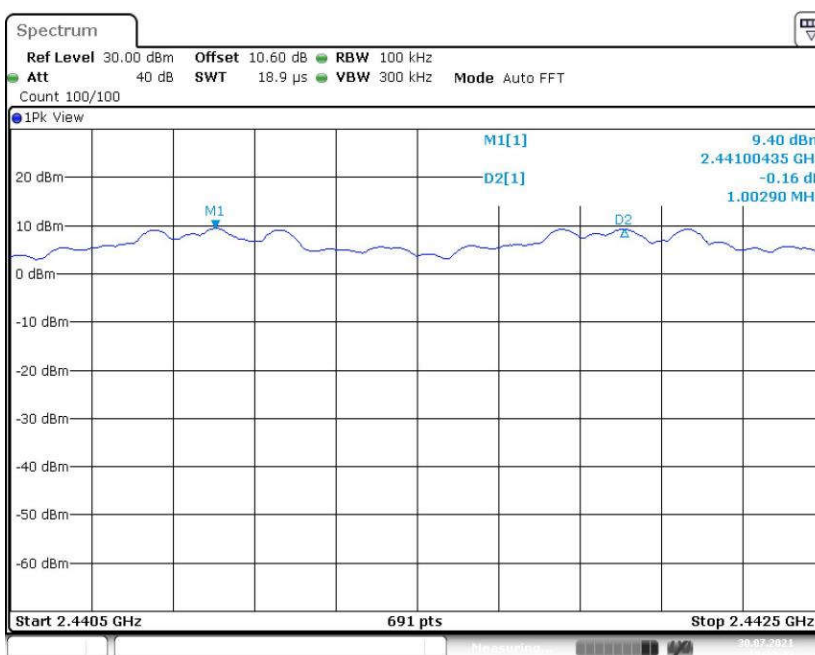
Fig. 78 Carrier Frequency Separation (8DPSK, CH39)
