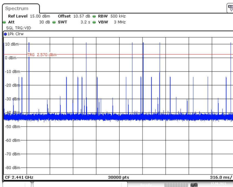
Fig. 68 Number of Burst in Observation Period (Dwell Time) (GFSK, CH39)
