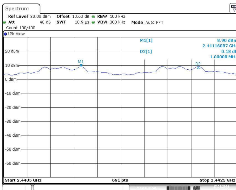
Fig. 77 Carrier Frequency Separation ( \pi/4 DQPSK, CH39)
