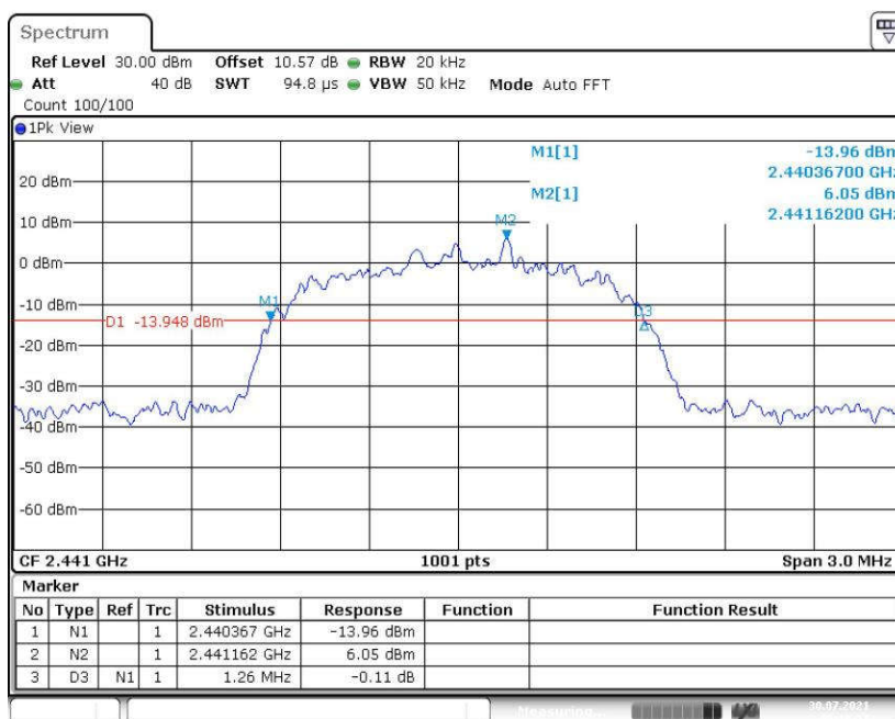
Fig. 65 20dB Bandwidth (8DPSK, CH39)
