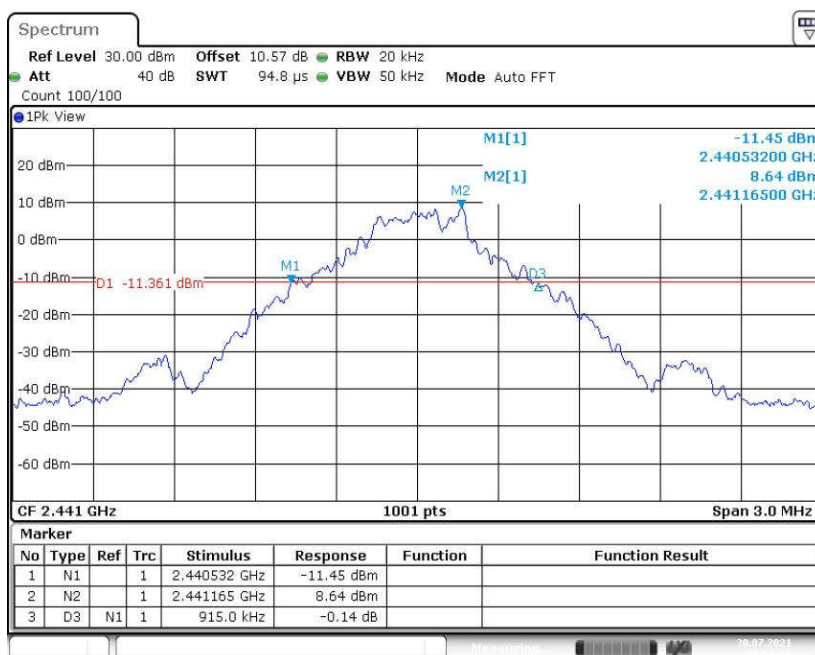
Fig. 59 20dB Bandwidth (GFSK, CH39)
