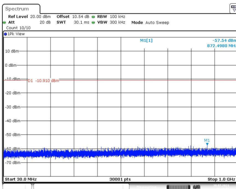
Fig. 32 Conducted Spurious Emission (8DPSK, CH0, 30MHz -1GHz)
