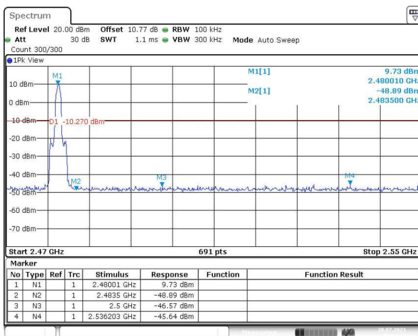
Fig. 10 Band Edges ( \pi/4 DQPSK, CH78, Hopping OFF)
