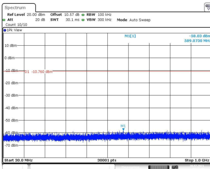
Fig. 35 Conducted Spurious Emission (8DPSK, CH39, 30MHz -1GHz)
