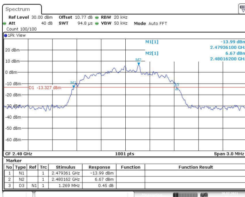
Fig. 66 20dB Bandwidth (8DPSK, CH78)
