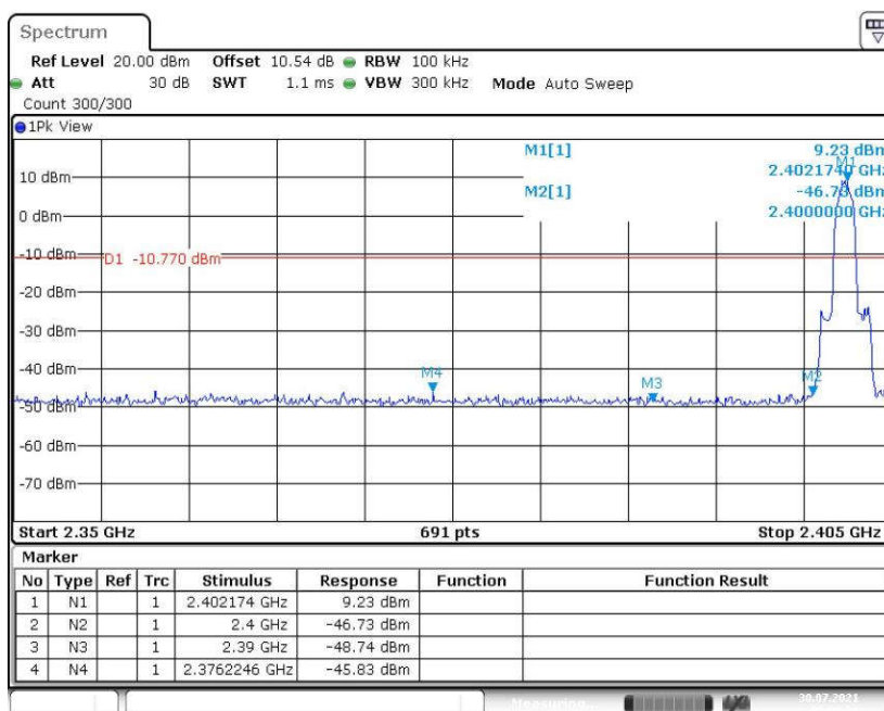
Fig. 9 Band Edges ( \pi/4 DQPSK, CH0, Hopping OFF)
