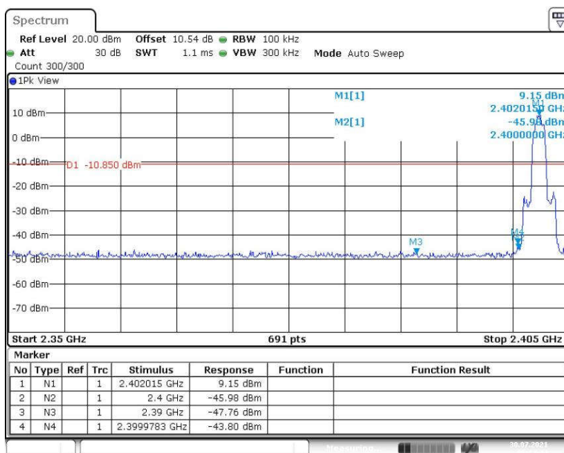
Fig. 11 Band Edges (8DPSK, CH0, Hopping OFF)
