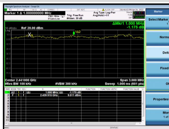
8-DPSK
