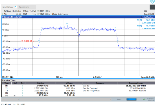
41-41-15MHz-15MHz-QPSK-QPSK-39725-39875-75RB#0-75RB#0
