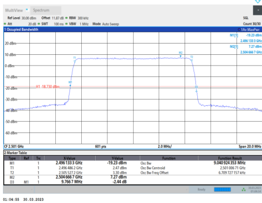
Band41-10MHz-64QAM-39700-50RB#0
