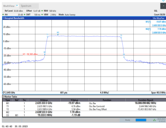
Band41-20MHz-QPSK-41140-100RB#0
