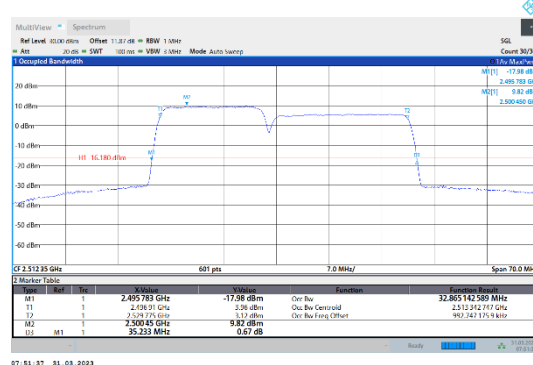
41-41-15MHz-20MHz-16QAM-16QAM-39728-39899-75RB#0-100RB#0
