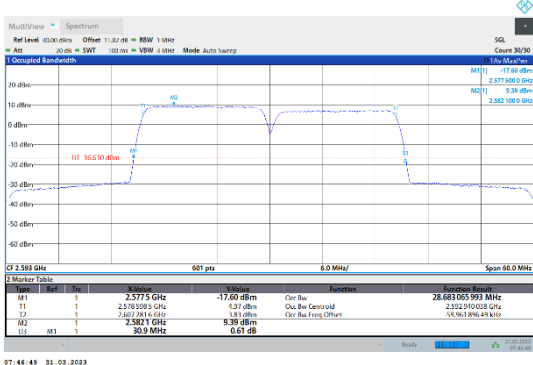
41-41-15MHz-15MHz-64QAM-64QAM-40545-40695-75RB#0-75RB#0
