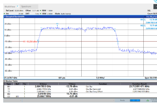
41-41-15MHz-10MHz-QPSK-QPSK-41417-41537-75RB#0-50RB#0
