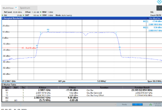
41-41-15MHz-10MHz-64QAM-64QAM-40571-40691-75RB#0-50RB#0
