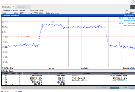
41-41-10MHz-20MHz-QPSK-QPSK-41346-41490-50RB#0-100RB#0
