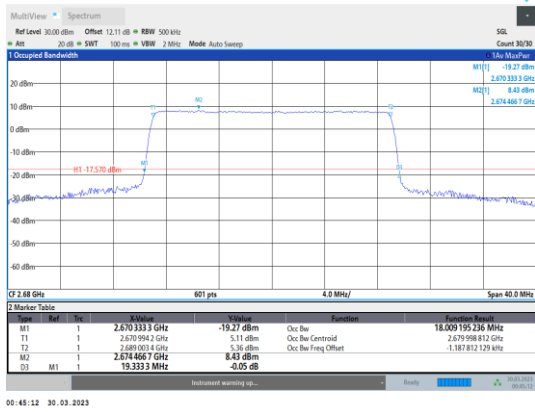
Band41-20MHz-QPSK-41490-100RB#0
