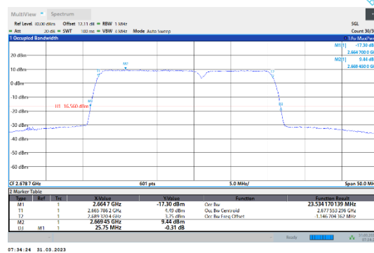
41-41-15MHz-10MHz-16QAM-16QAM-41417-41537-75RB#0-50RB#0
