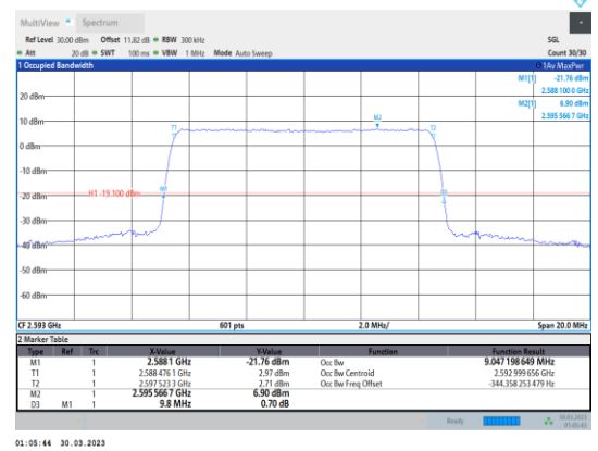
Band41-10MHz-64QAM-40620-50RB#0
