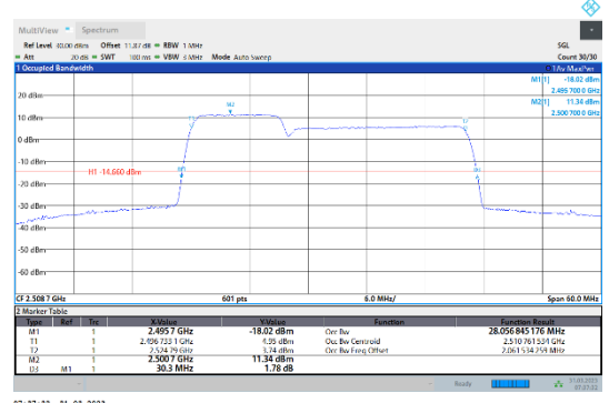
41-41-10MHz-20MHz-64QAM-64QAM-39705-39849-50RB#0-100RB#0
