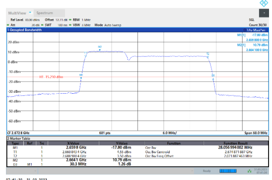
41-41-10MHz-20MHz-16QAM-16QAM-41346-41490-50RB#0-100RB#0
