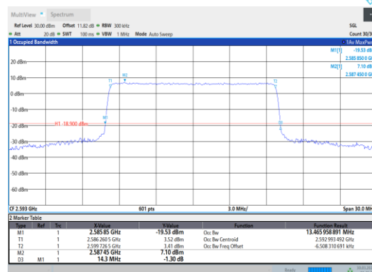
Band41-15MHz-QPSK-40620-75RB#0
