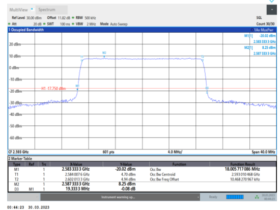
Band41-20MHz-QPSK-40620-100RB#0
