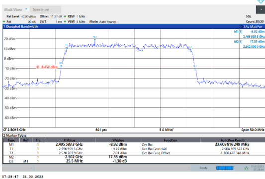
41-41-15MHz-10MHz-QPSK-QPSK-39725-39845-75RB#0-50RB#0
