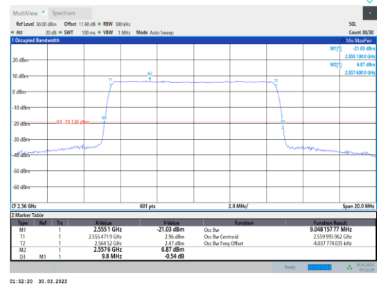
Band41-10MHz-64QAM-40290-50RB#0
