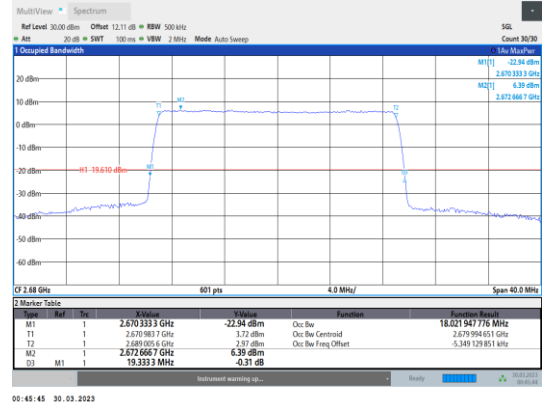
Band41-20MHz-64QAM-41490-100RB#0
