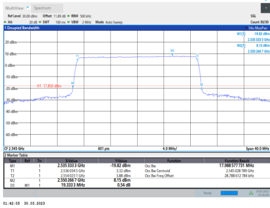
Band41-20MHz-QPSK-40140-100RB#0
