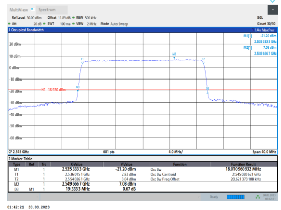
Band41-20MHz-16QAM-40140-100RB#0
