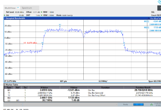
41-41-15MHz-15MHz-QPSK-QPSK-41365-41515-75RB#0-75RB#0
