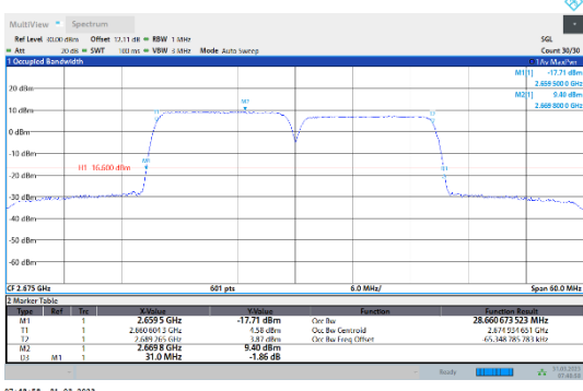
41-41-15MHz-15MHz-16QAM-16QAM-41365-41515-75RB#0-75RB#0
