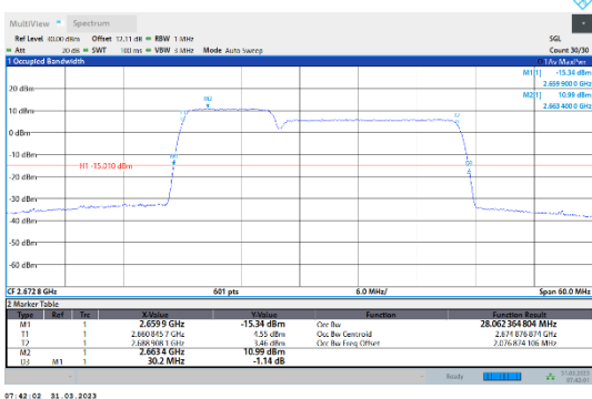
41-41-10MHz-20MHz-64QAM-64QAM-41346-41490-50RB#0-100RB#0
