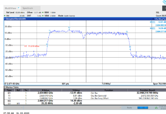
41-41-15MHz-20MHz-QPSK-QPSK-41319-41490-75RB#0-100RB#0
