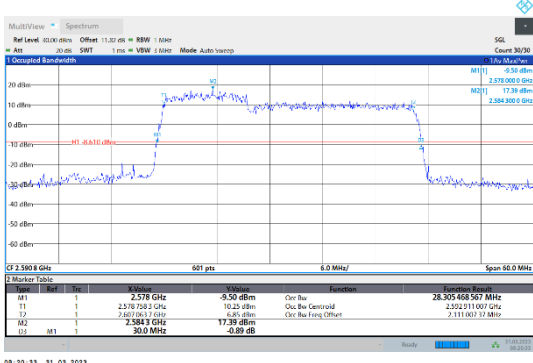
41-41-10MHz-20MHz-QPSK-QPSK-40526-40670-50RB#0-100RB#0
