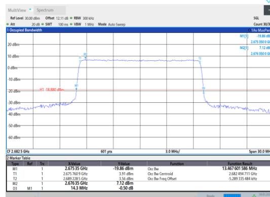
Band41-15MHz-QPSK-41515-75RB#0
