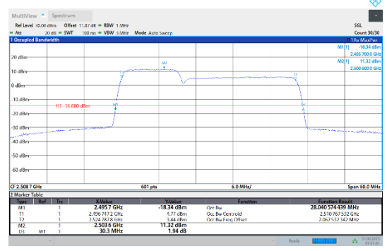
41-41-10MHz-20MHz-16QAM-16QAM-39705-39849-50RB#0-100RB#0
