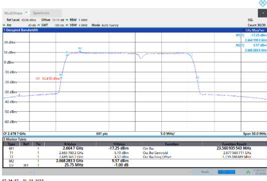
41-41-15MHz-10MHz-64QAM-64QAM-41417-41537-75RB#0-50RB#0
