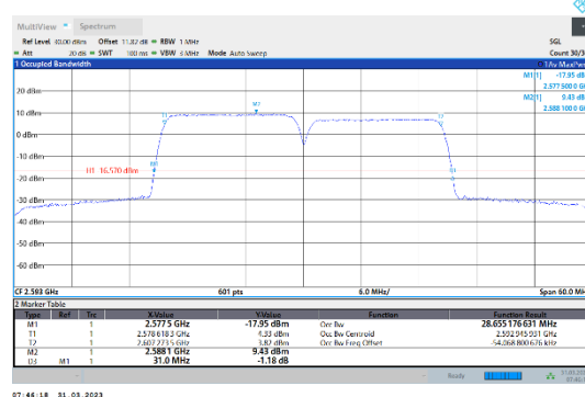
41-41-15MHz-15MHz-16QAM-16QAM-40545-40695-75RB#0-75RB#0
