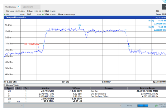
41-41-15MHz-15MHz-QPSK-QPSK-40545-40695-75RB#0-75RB#0
