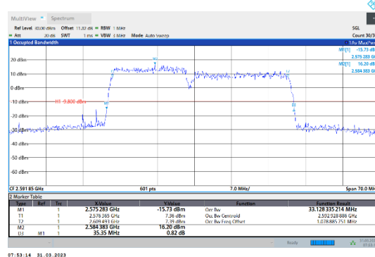
41-41-15MHz-20MHz-QPSK-QPSK-40523-40694-75RB#0-100RB#0
