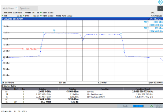
41-41-15MHz-15MHz-64QAM-64QAM-41365-41515-75RB#0-75RB#0
