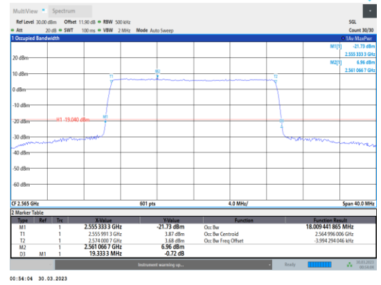
Band41-20MHz-16QAM-40340-100RB#0
