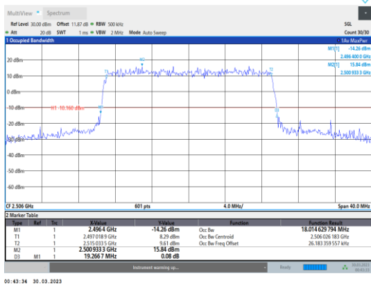
Band41-20MHz-QPSK-39750-100RB#0
