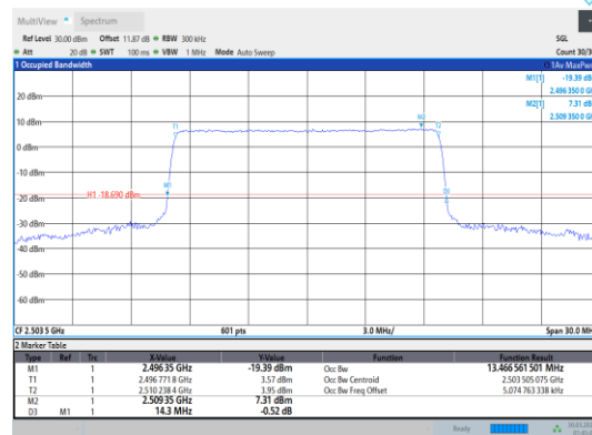
Band41-15MHz-QPSK-39725-75RB#0
