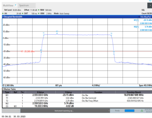
Band41-20MHz-64QAM-40340-100RB#0
