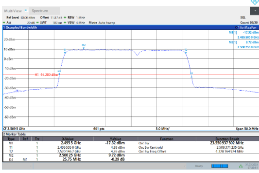
41-41-15MHz-10MHz-64QAM-64QAM-39725-39845-75RB#0-50RB#0
