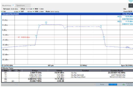
41-41-10MHz-15MHz-64QAM-64QAM-41395-41515-50RB#0-75RB#0
