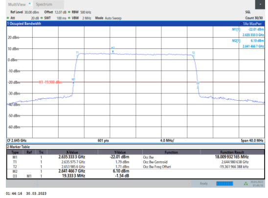
Band41-20MHz-64QAM-41140-100RB#0
