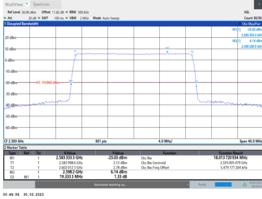
Band41-20MHz-64QAM-40620-100RB#0
