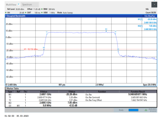
Band41-10MHz-16QAM-40740-50RB#0
