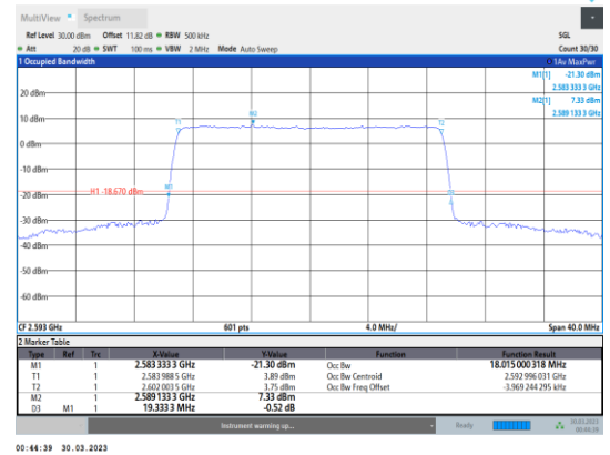
Band41-20MHz-16QAM-40620-100RB#0
