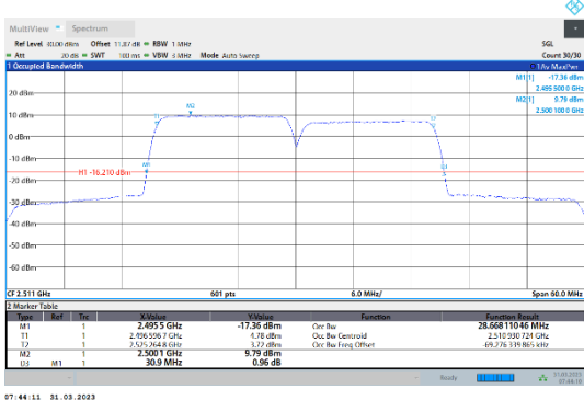
41-41-15MHz-15MHz-64QAM-64QAM-39725-39875-75RB#0-75RB#0
