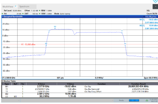
41-41-10MHz-20MHz-64QAM-64QAM-40526-40670-50RB#0-100RB#0
