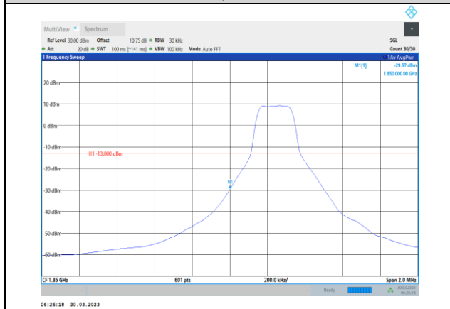
Band2-3MHz-64QAM-18615-1RB#0
