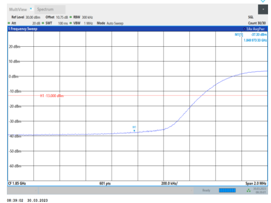
Band2-15MHz-64QAM-18675-75RB#0
