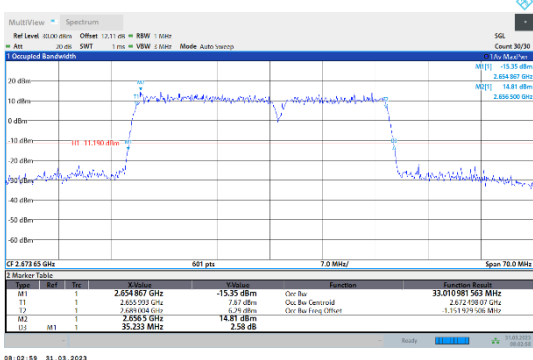
41-41-20MHz-15MHz-QPSK-QPSK-41341-41512-100RB#0-75RB#0
