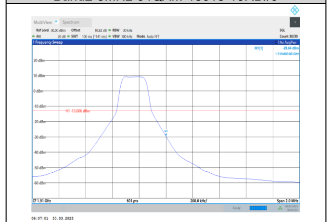
Band2-3MHz-64QAM-19185-1RB#14
