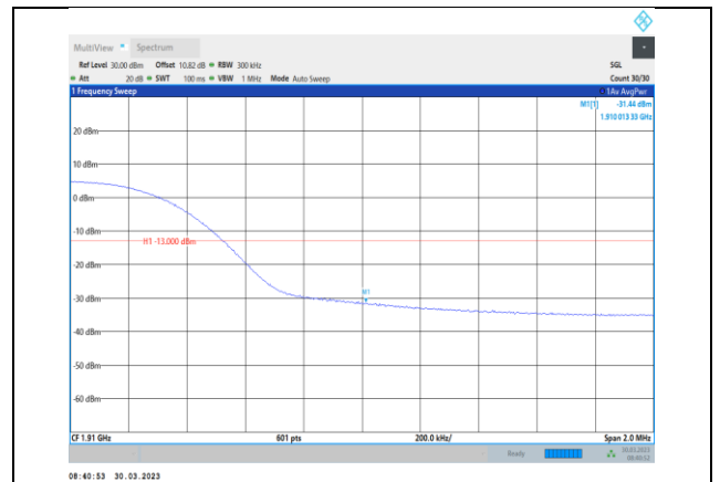
Band2-15MHz-QPSK-19125-75RB#0
