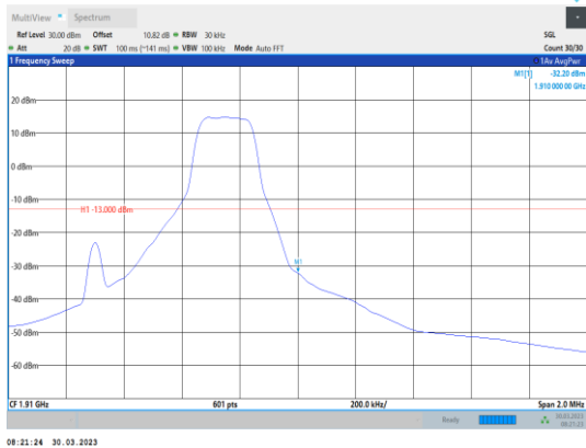
Band2-1.4MHz-16QAM-19193-1RB#5
