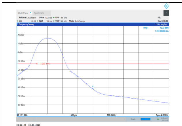
Band2-10MHz-16QAM-19150-1RB#49
