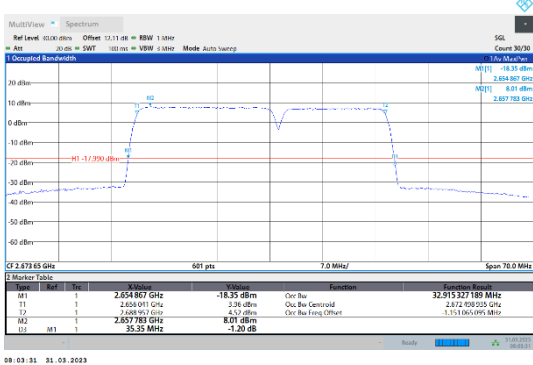
41-41-20MHz-15MHz-16QAM-16QAM-41341-41512-100RB#0-75RB#0
