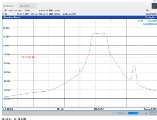
Band2-1.4MHz-64QAM-18607-1RB#0
