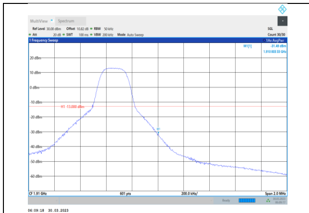
Band2-5MHz-16QAM-19175-1RB#24
