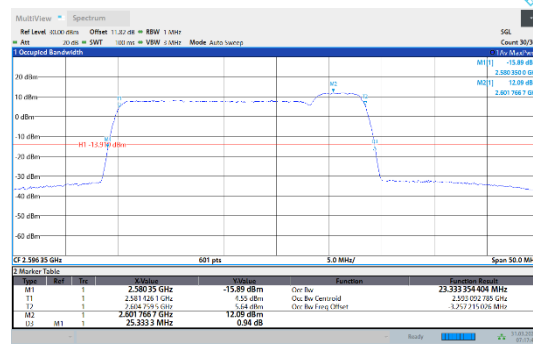
41-41-20MHz-5MHz-64QAM-64QAM-40595-40712-100RB#0-25RB#0
