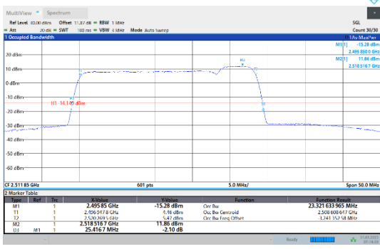
41-41-20MHz-5MHz-16QAM-16QAM-39750-39867-100RB#0-25RB#0
