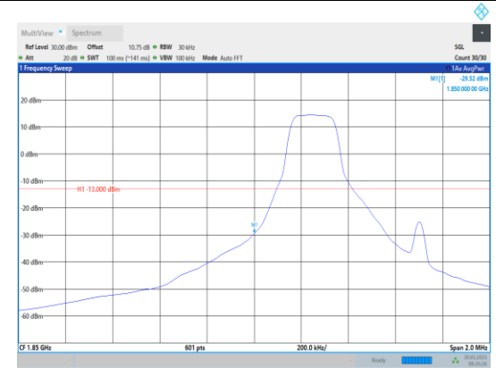
Band2-1.4MHz-16QAM-18607-1RB#0
