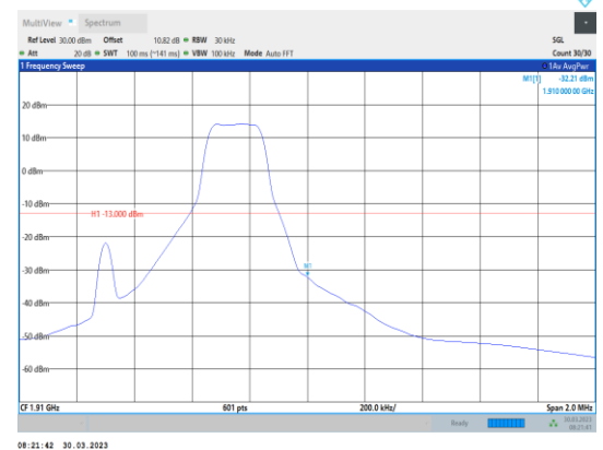
Band2-1.4MHz-64QAM-19193-1RB#5
