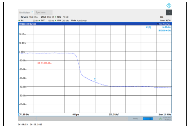
Band2-5MHz-QPSK-19175-25RB#0
