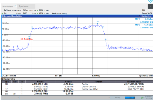
41-41-20MHz-5MHz-QPSK-QPSK-39750-39867-100RB#0-25RB#0
