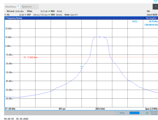
Band2-3MHz-16QAM-18615-1RB#0
