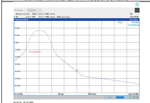
Band2-10MHz-QPSK-19150-1RB#49
