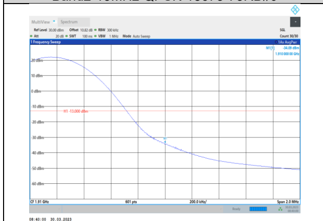
Band2-15MHz-QPSK-19125-1RB#74
