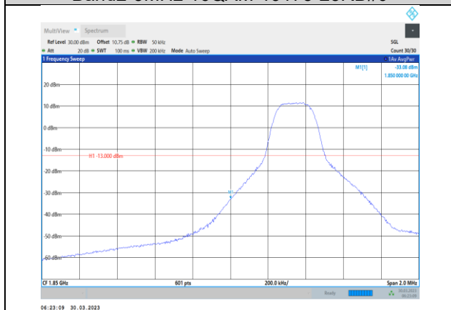
Band2-5MHz-64QAM-18625-1RB#0
