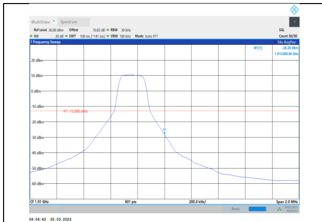
Band2-3MHz-16QAM-19185-1RB#14
