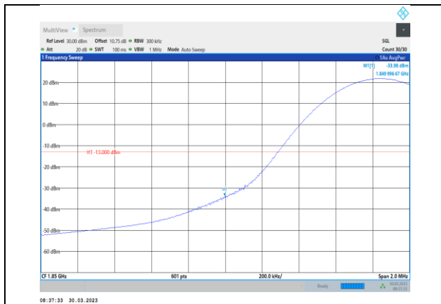
Band2-15MHz-QPSK-18675-1RB#0
