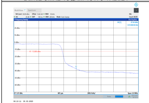
Band2-5MHz-16QAM-19175-25RB#0
