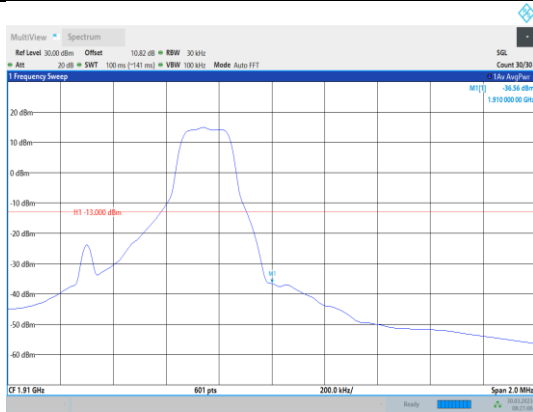
Band2-1.4MHz-QPSK-19193-1RB#5
