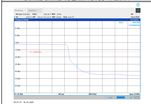
Band2-3MHz-16QAM-19185-15RB#0
