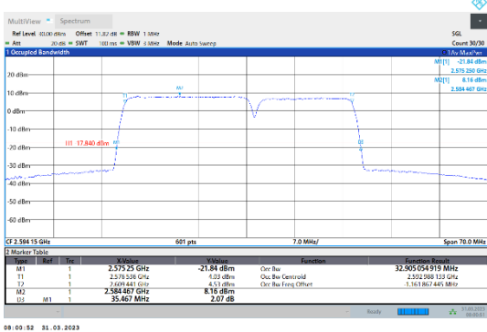
41-41-20MHz-15MHz-16QAM-16QAM-40546-40717-100RB#0-75RB#0
