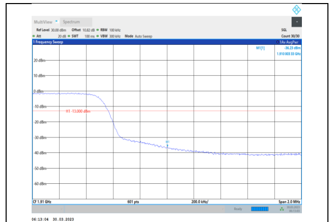
Band2-10MHz-QPSK-19150-50RB#0
