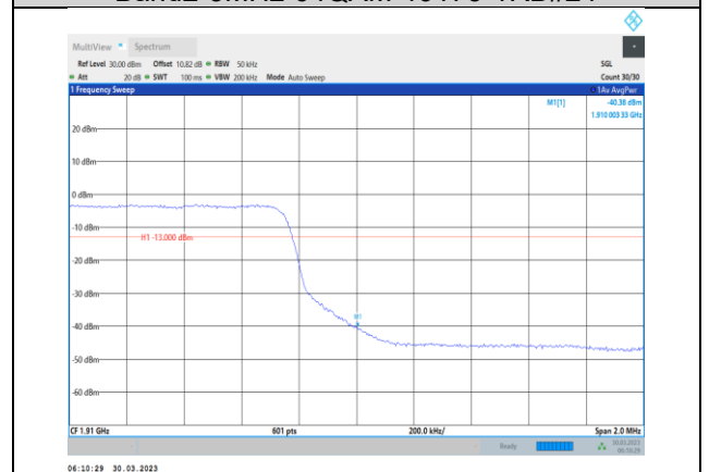
Band2-5MHz-64QAM-19175-25RB#0
