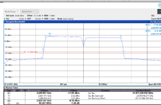
41-41-20MHz-20MHz-64QAM-64QAM-40521-40719-100RB#0-100RB#0
