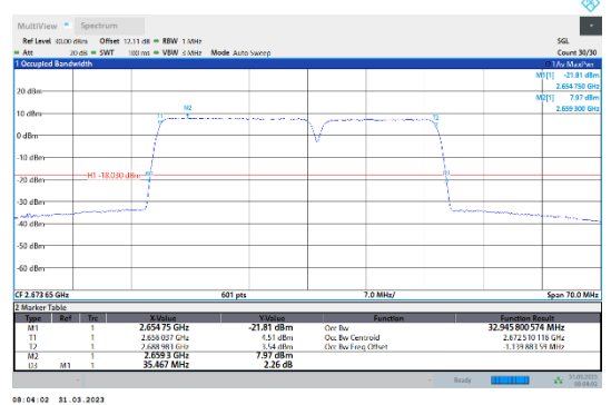
41-41-20MHz-15MHz-64QAM-64QAM-41341-41512-100RB#0-75RB#0
