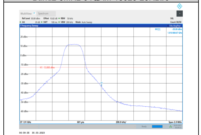
Band2-5MHz-64QAM-19175-1RB#24
