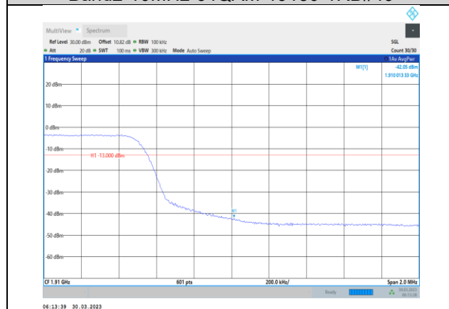
Band2-10MHz-64QAM-19150-50RB#0
