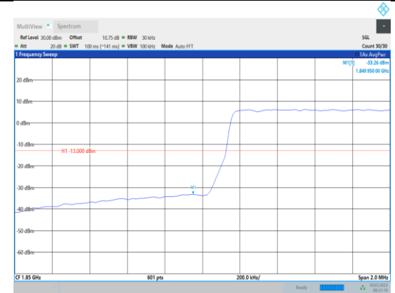
Band2-1.4MHz-16QAM-18607-6RB#0
