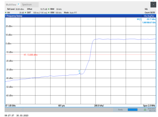
Band2-1.4MHz-64QAM-18607-6RB#0
