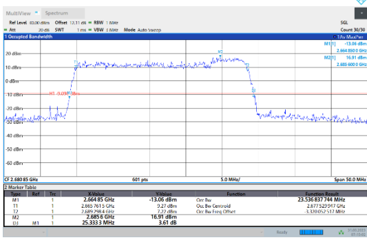
41-41-20MHz-5MHz-QPSK-QPSK-41440-41557-100RB#0-25RB#0
