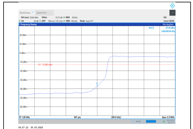
Band2-3MHz-64QAM-18615-15RB#0
