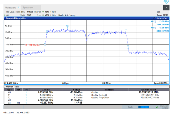
41-41-20MHz-20MHz-QPSK-QPSK-39750-39948-100RB#0-100RB#0
