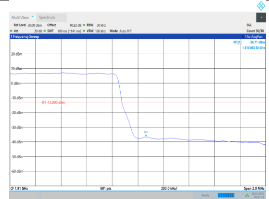
Band2-1.4MHz-QPSK-19193-6RB#0
