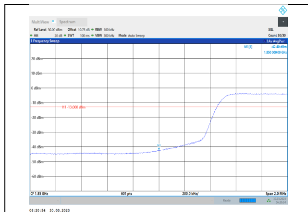
Band2-10MHz-64QAM-18650-50RB#0
