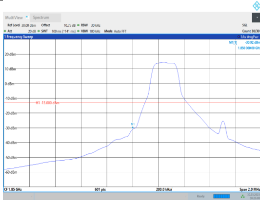
Band2-1.4MHz-QPSK-18607-1RB#0
