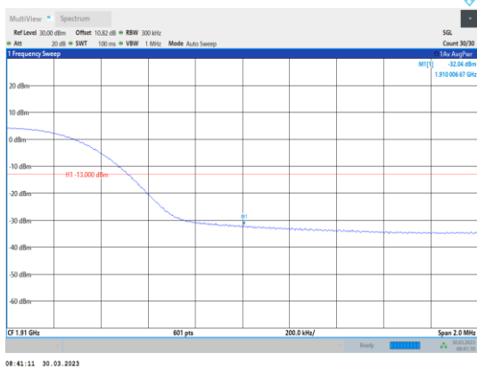
Band2-15MHz-16QAM-19125-75RB#0
