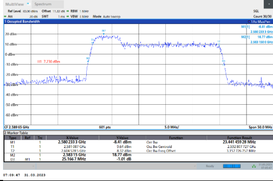
41-41-5MHz-20MHz-QPSK-QPSK-39683-39800-25RB#0-100RB#0
