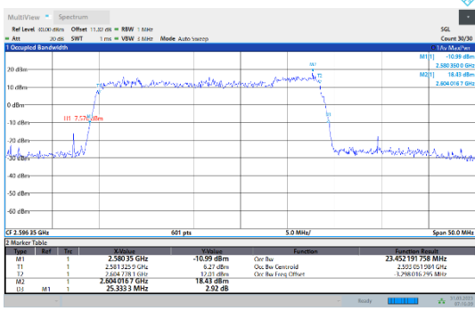
41-41-20MHz-5MHz-QPSK-QPSK-40595-40712-100RB#0-25RB#0
