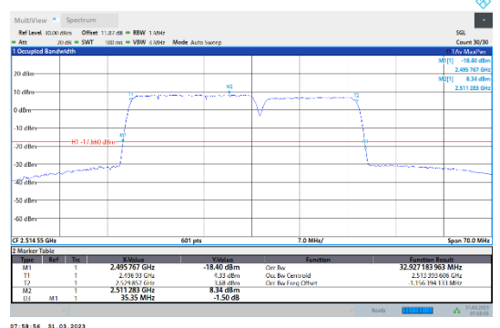
41-41-20MHz-15MHz-64QAM-64QAM-39750-39921-100RB#0-75RB#0
