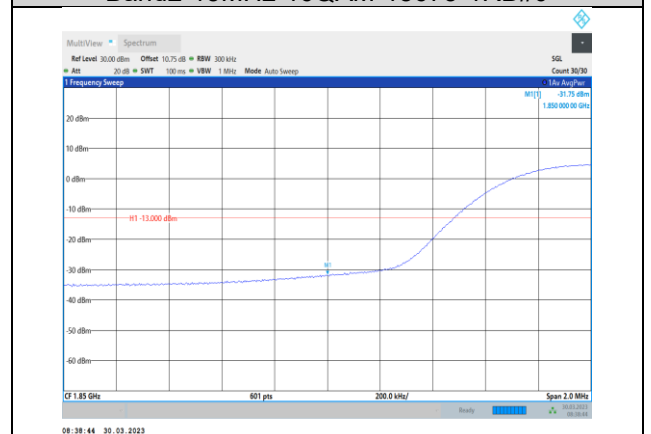
Band2-15MHz-16QAM-18675-75RB#0
