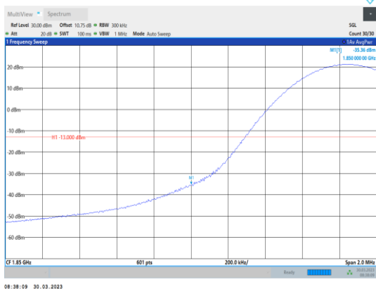
Band2-15MHz-64QAM-18675-1RB#0
