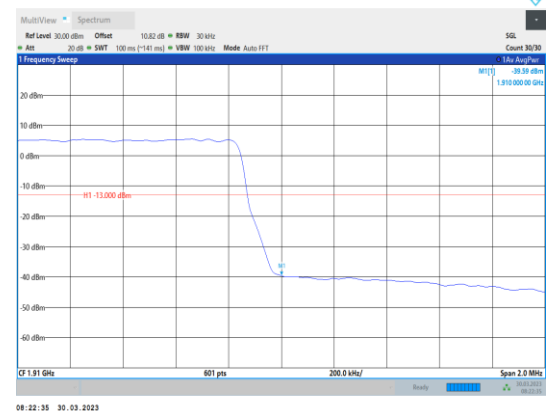
Band2-1.4MHz-64QAM-19193-6RB#0
