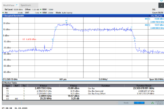
41-41-5MHz-20MHz-16QAM-16QAM-39683-39800-25RB#0-100RB#0
