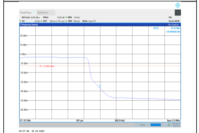
Band2-3MHz-64QAM-19185-15RB#0
