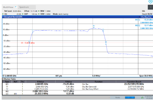
41-41-20MHz-5MHz-64QAM-64QAM-41440-41557-100RB#0-25RB#0
