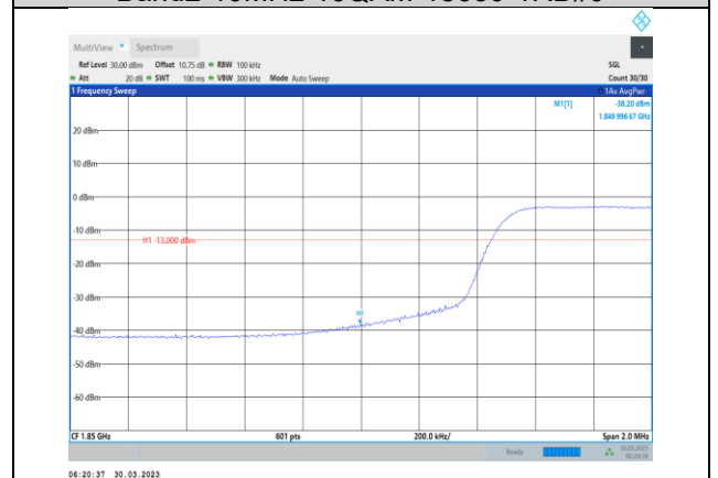
Band2-10MHz-16QAM-18650-50RB#0
