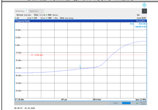
Band2-15MHz-QPSK-18675-75RB#0
