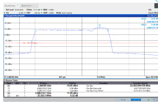
41-41-20MHz-5MHz-16QAM-16QAM-41440-41557-100RB#0-25RB#0
