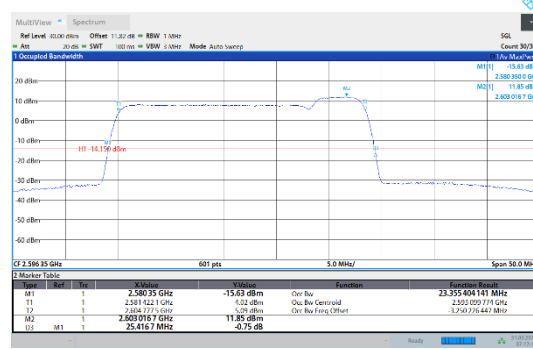
41-41-20MHz-5MHz-16QAM-16QAM-40595-40712-100RB#0-25RB#0
