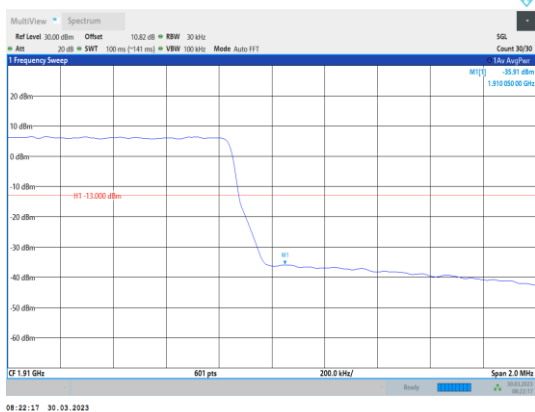
Band2-1.4MHz-16QAM-19193-6RB#0
