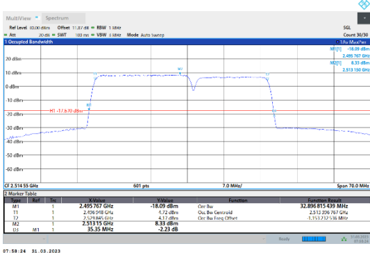
41-41-20MHz-15MHz-16QAM-16QAM-39750-39921-100RB#0-75RB#0
