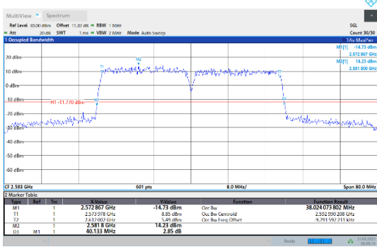
41-41-20MHz-20MHz-QPSK-QPSK-40521-40719-100RB#0-100RB#0
