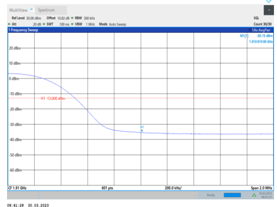
Band2-15MHz-64QAM-19125-75RB#0
