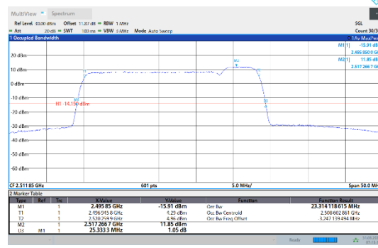
41-41-20MHz-5MHz-64QAM-64QAM-39750-39867-100RB#0-25RB#0
