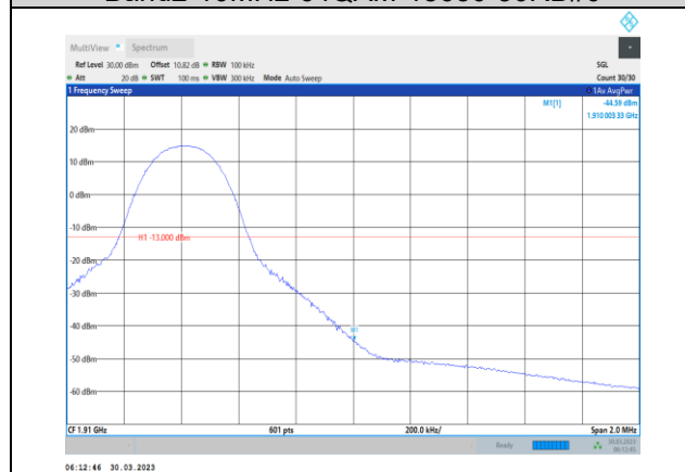
Band2-10MHz-64QAM-19150-1RB#49
