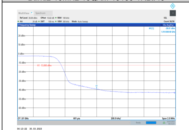
Band2-10MHz-16QAM-19150-50RB#0
