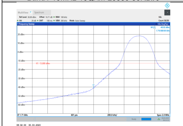
Band4-10MHz-64QAM-20000-1RB#0
