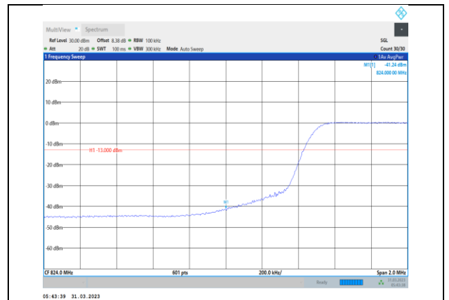
Band5-10MHz-64QAM-20450-50RB#0
