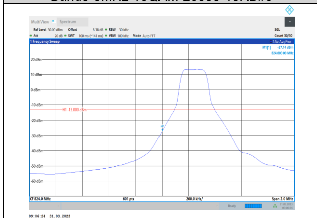
Band5-3MHz-64QAM-20415-1RB#0
