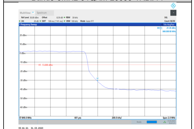
Band5-3MHz-64QAM-20635-15RB#0
