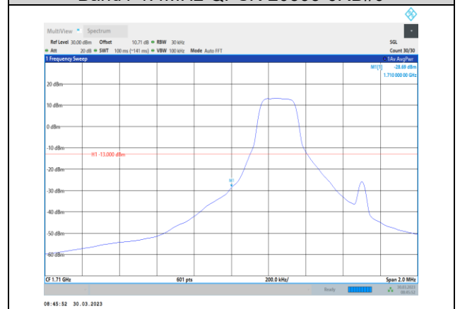
Band4-1.4MHz-16QAM-19957-1RB#0
