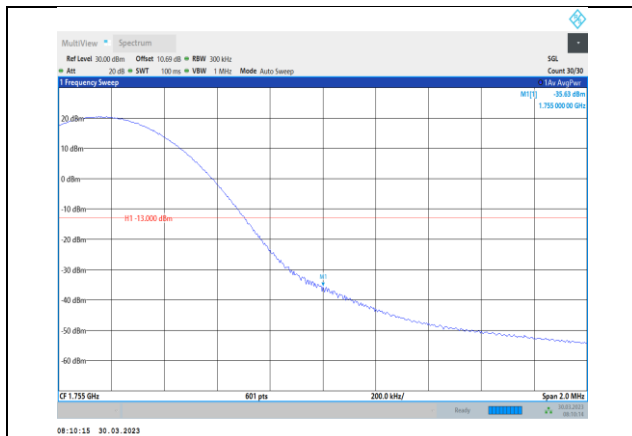
Band4-15MHz-16QAM-20325-1RB#74
