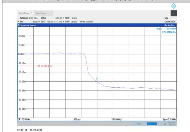
Band4-3MHz-16QAM-20385-15RB#0
