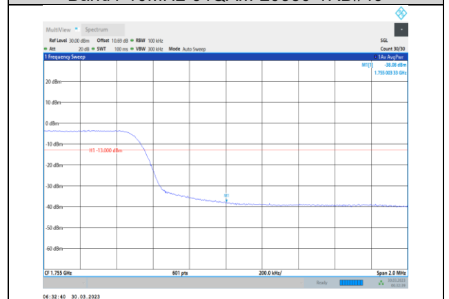
Band4-10MHz-64QAM-20350-50RB#0
