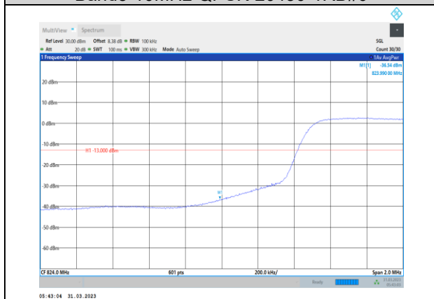
Band5-10MHz-QPSK-20450-50RB#0
