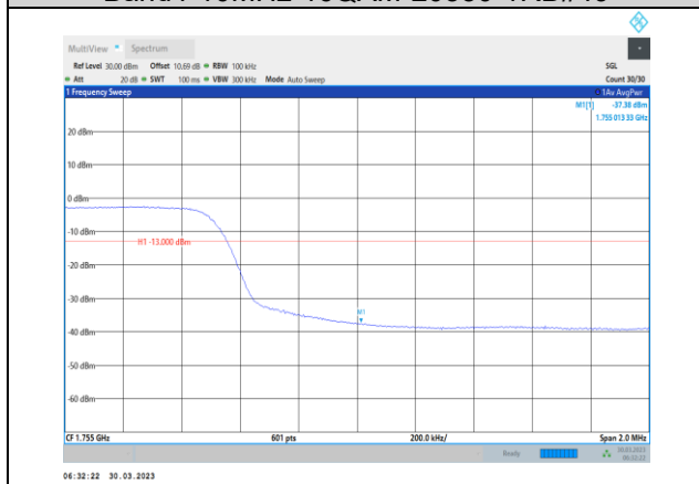
Band4-10MHz-16QAM-20350-50RB#0
