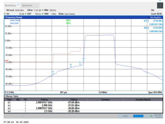
Band7-10MHz-16QAM-20800-50RB#0
