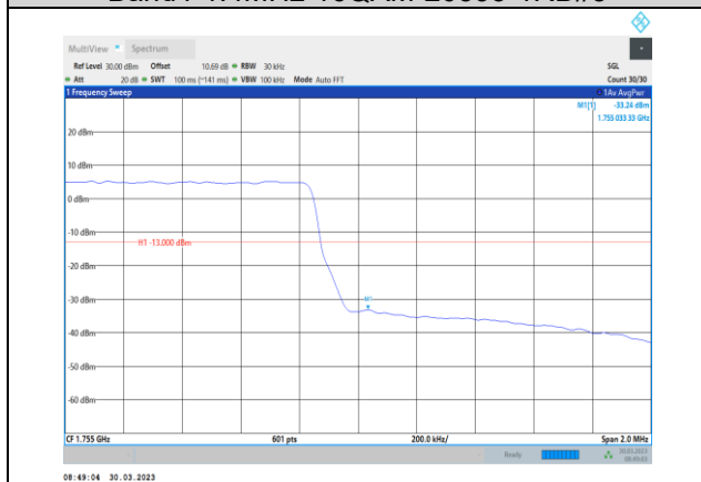
Band4-1.4MHz-16QAM-20393-6RB#0
