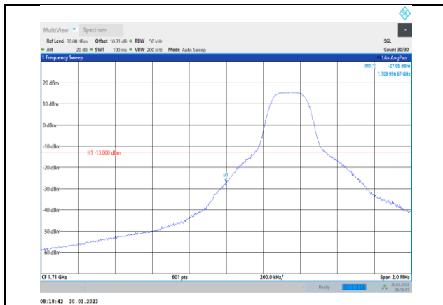
Band4-5MHz-QPSK-19975-1RB#0
