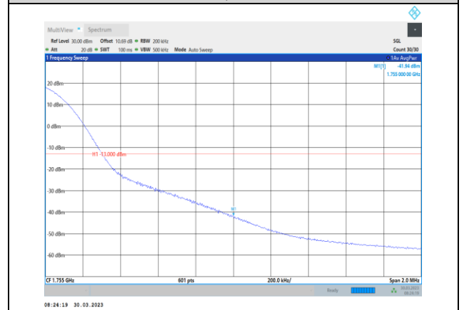
Band4-20MHz-64QAM-20300-1RB#99
