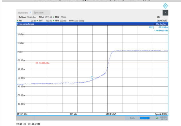
Band4-5MHz-QPSK-19975-25RB#0
