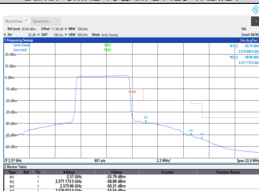
Band7-5MHz-16QAM-21425-1RB#24
