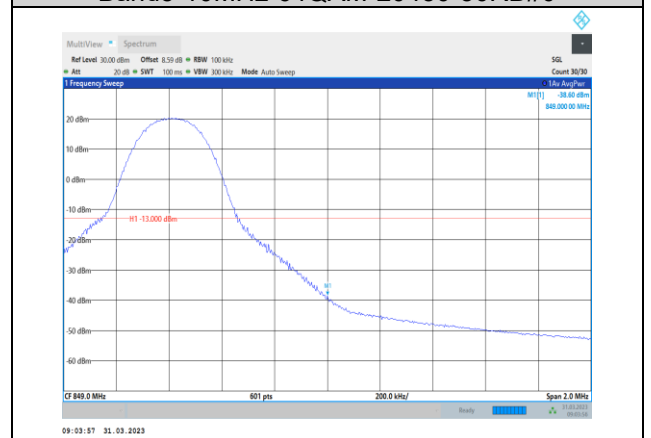
Band5-10MHz-64QAM-20600-1RB#49
