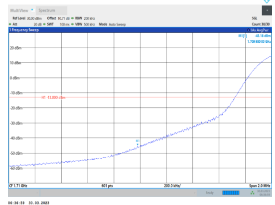
Band4-20MHz-16QAM-20050-1RB#0
