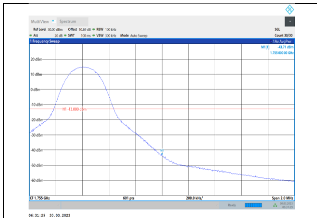
Band4-10MHz-16QAM-20350-1RB#49
