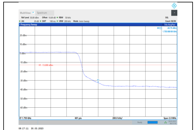
Band4-5MHz-QPSK-20375-25RB#0
