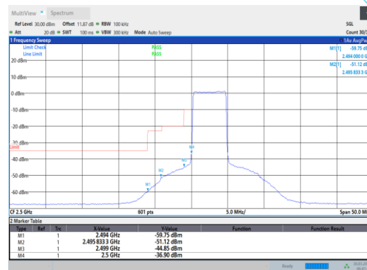
Band7-5MHz-64QAM-20775-25RB#0
