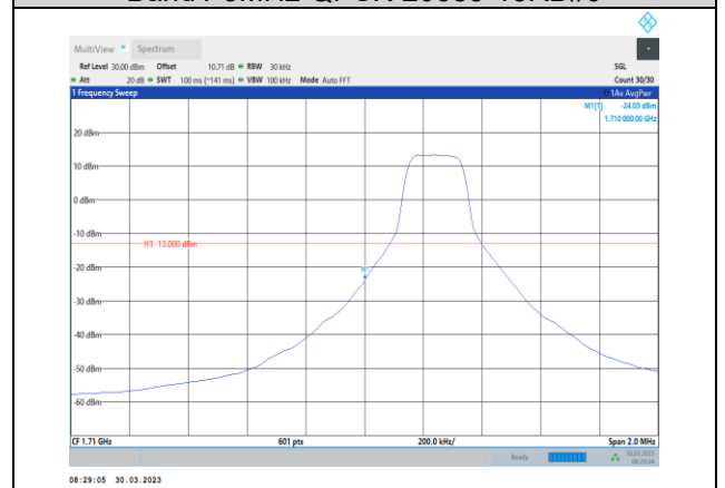
Band4-3MHz-16QAM-19965-1RB#0
