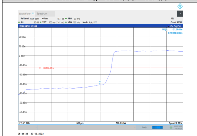
Band4-1.4MHz-QPSK-19957-6RB#0
