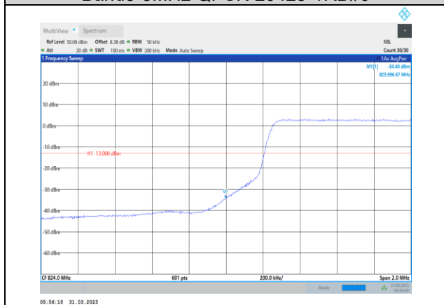
Band5-5MHz-QPSK-20425-25RB#0
