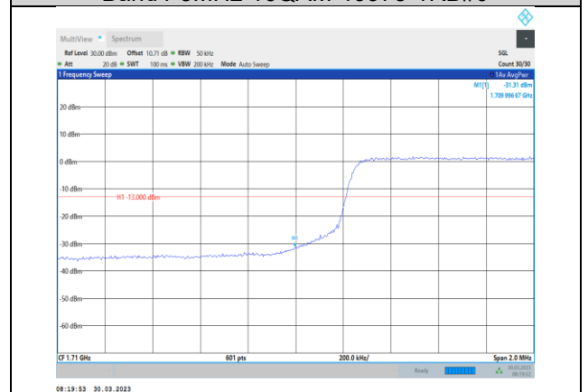
Band4-5MHz-16QAM-19975-25RB#0
