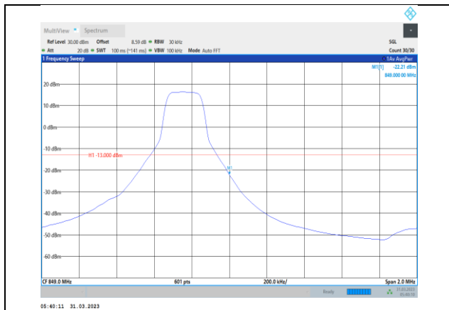
Band5-3MHz-16QAM-20635-1RB#14
