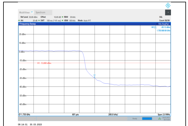
Band4-3MHz-QPSK-20385-15RB#0
