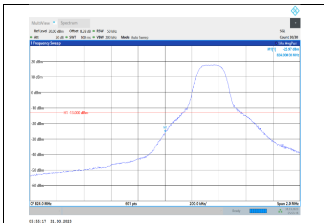
Band5-5MHz-QPSK-20425-1RB#0
