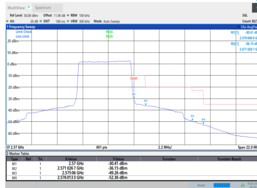
Band7-5MHz-QPSK-21425-25RB#0
