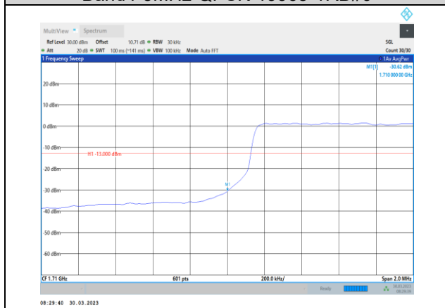
Band4-3MHz-QPSK-19965-15RB#0
