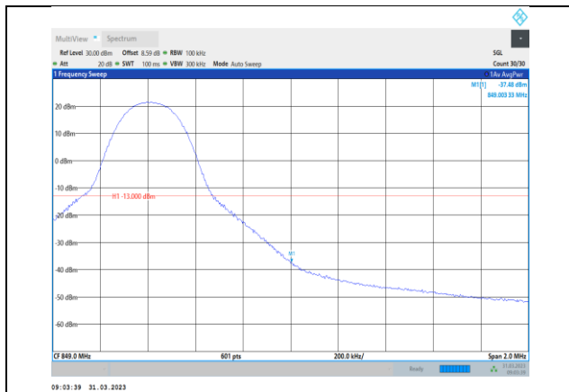
Band5-10MHz-16QAM-20600-1RB#49
