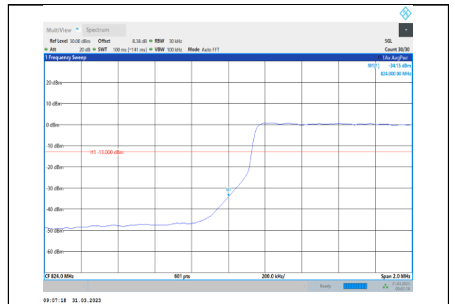
Band5-3MHz-64QAM-20415-15RB#0
