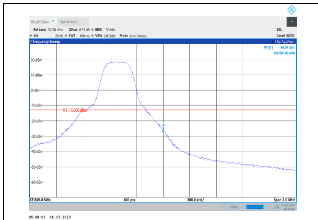
Band5-5MHz-16QAM-20625-1RB#24
