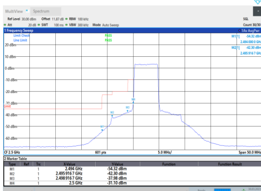
Band7-5MHz-QPSK-20775-25RB#0
