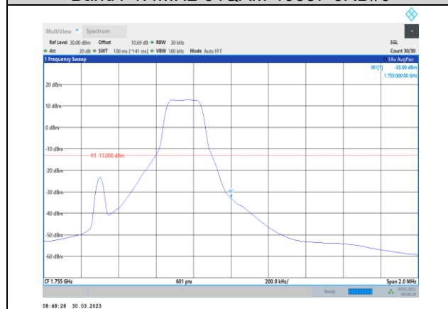
Band4-1.4MHz-64QAM-20393-1RB#5
