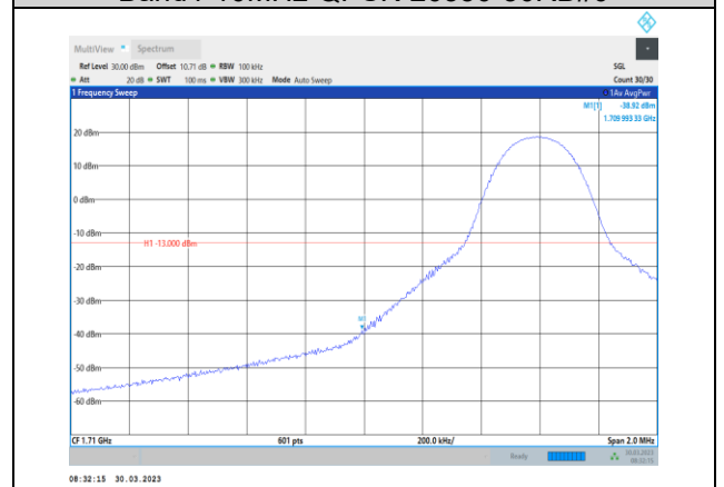
Band4-10MHz-16QAM-20000-1RB#0
