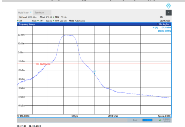
Band5-5MHz-QPSK-20625-1RB#24
