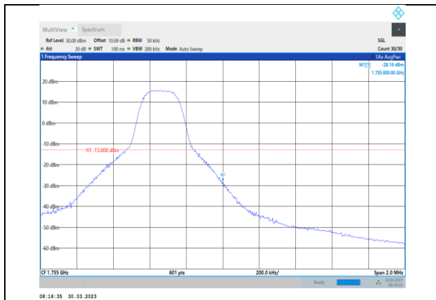
Band4-5MHz-16QAM-20375-1RB#24
