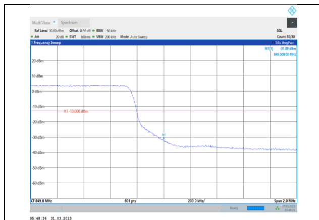
Band5-5MHz-QPSK-20625-25RB#0
