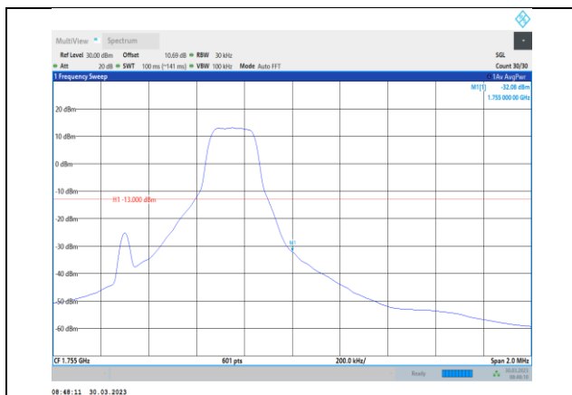
Band4-1.4MHz-16QAM-20393-1RB#5
