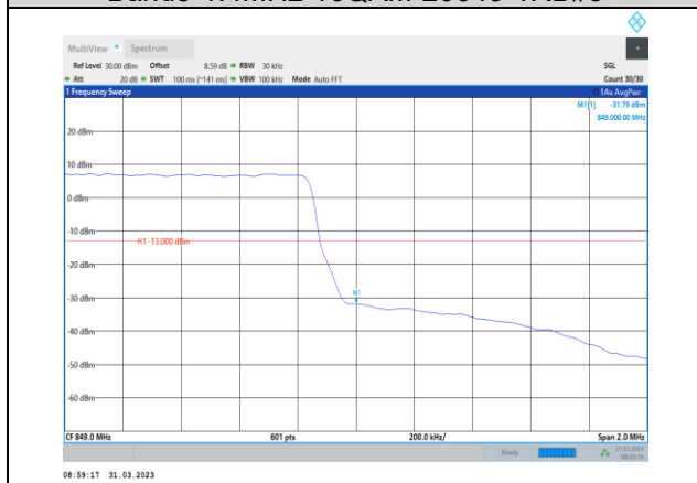
Band5-1.4MHz-16QAM-20643-6RB#0
