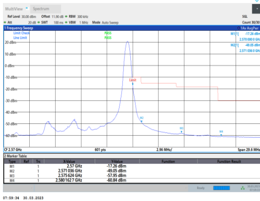
Band7-10MHz-QPSK-21400-1RB#49
