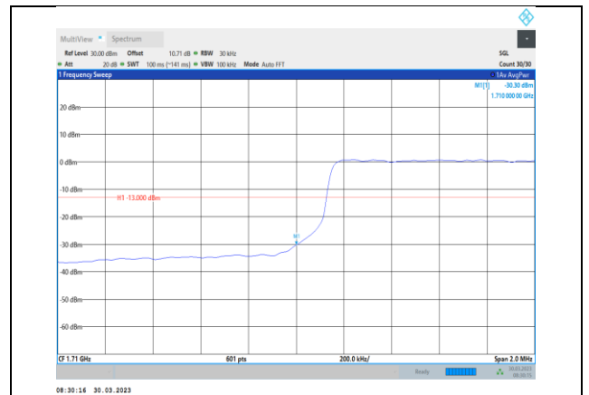
Band4-3MHz-64QAM-19965-15RB#0
