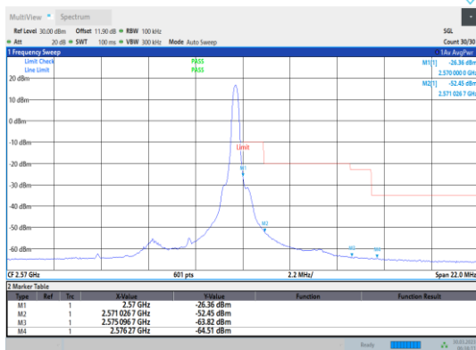
Band7-5MHz-16QAM-21425-1RB#24
