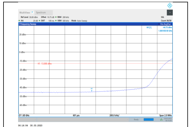
Band2-20MHz-64QAM-18700-100RB#0
