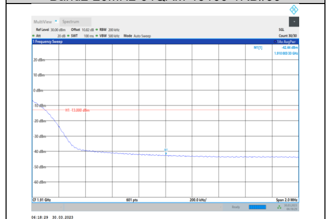
Band2-20MHz-64QAM-19100-100RB#0
