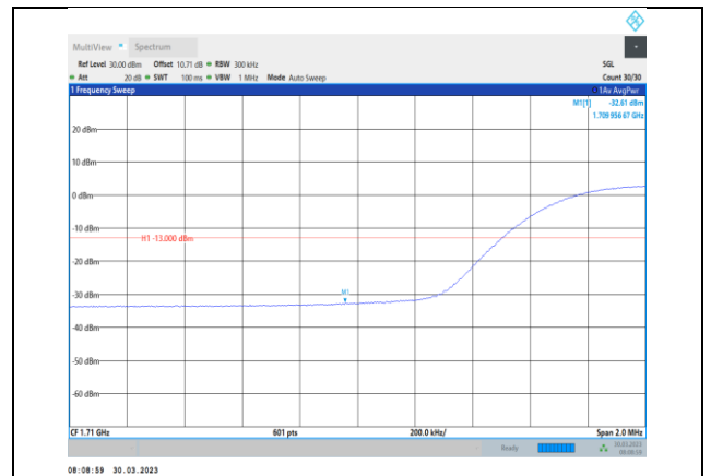
Band4-15MHz-64QAM-20025-75RB#0
