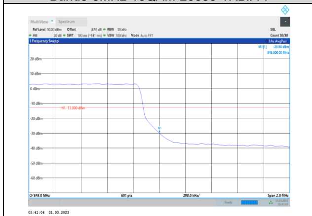
Band5-3MHz-16QAM-20635-15RB#0
