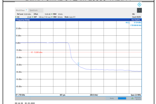
Band4-3MHz-64QAM-20385-15RB#0
