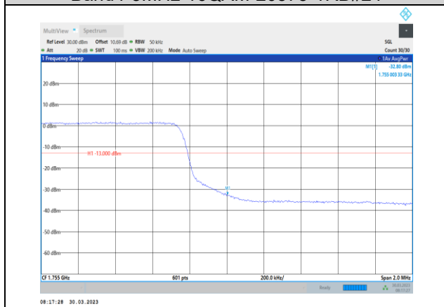
Band4-5MHz-16QAM-20375-25RB#0
