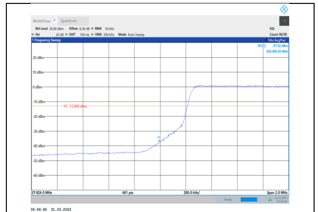
Band5-5MHz-64QAM-20425-25RB#0
