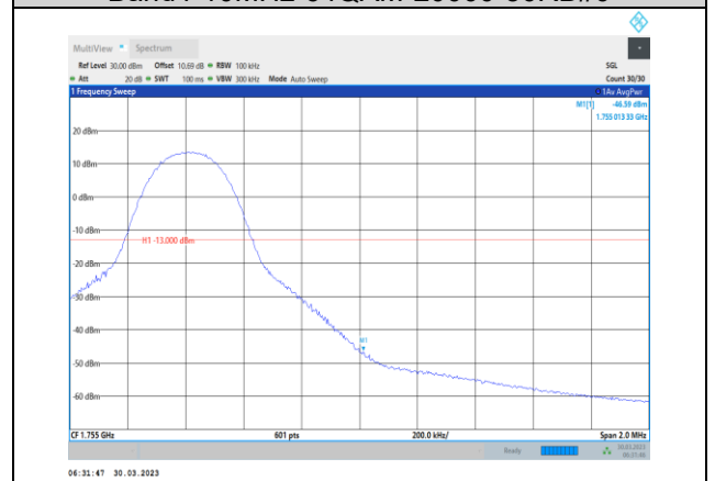
Band4-10MHz-64QAM-20350-1RB#49
