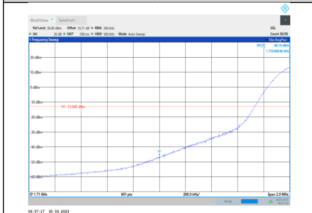
Band4-20MHz-64QAM-20050-1RB#0
