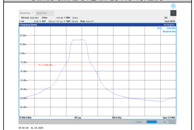
Band5-3MHz-64QAM-20635-1RB#14
