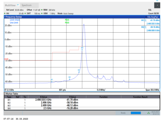
Band7-10MHz-16QAM-20800-1RB#0
