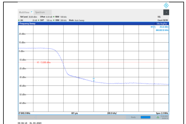
Band5-10MHz-QPSK-20600-50RB#0
