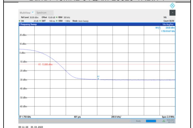
Band4-15MHz-64QAM-20325-75RB#0
