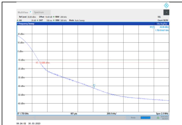
Band4-20MHz-16QAM-20300-1RB#99
