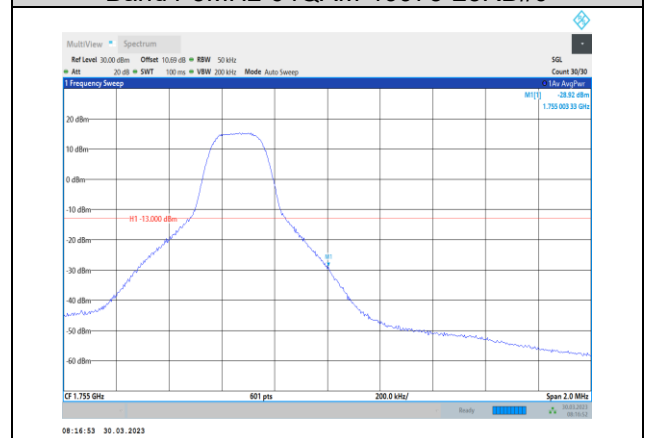
Band4-5MHz-64QAM-20375-1RB#24
