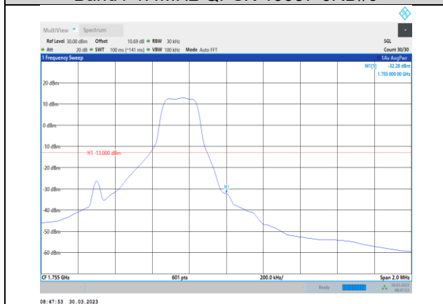
Band4-1.4MHz-QPSK-20393-1RB#5
