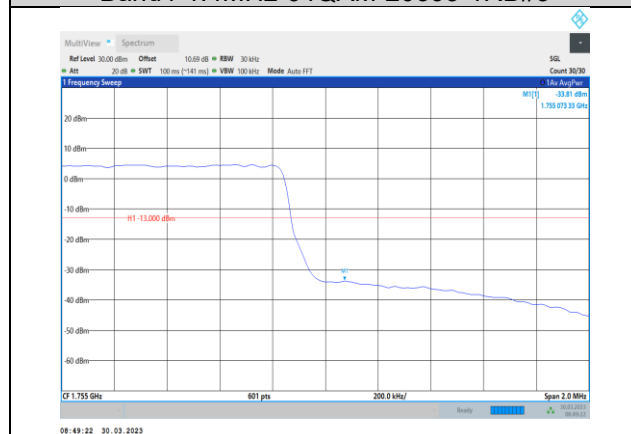
Band4-1.4MHz-64QAM-20393-6RB#0
