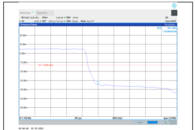
Band4-1.4MHz-QPSK-20393-6RB#0
