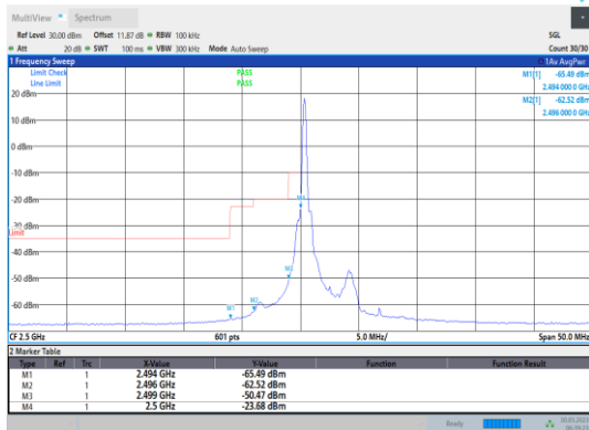
Band7-5MHz-QPSK-20775-1RB#0
