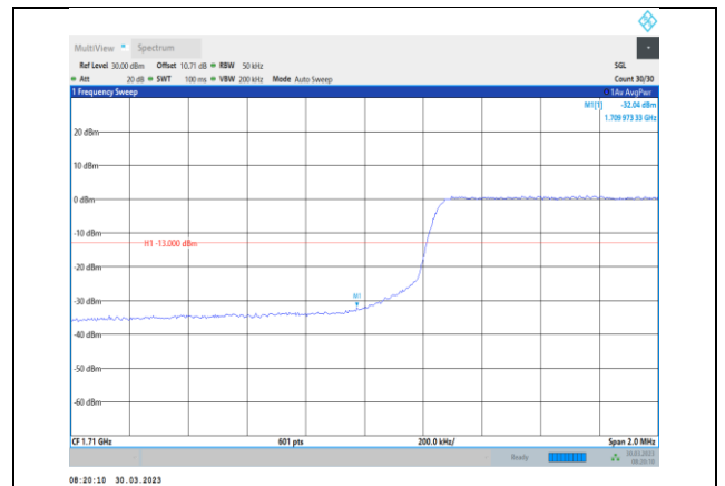
Band4-5MHz-64QAM-19975-25RB#0
