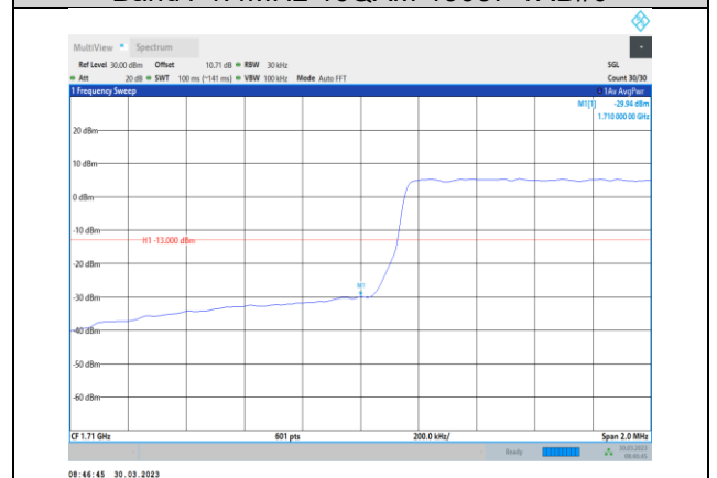
Band4-1.4MHz-16QAM-19957-6RB#0
