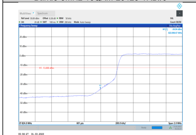
Band5-5MHz-16QAM-20425-25RB#0
