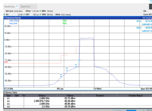
Band7-5MHz-16QAM-20775-25RB#0
