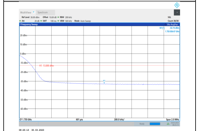
Band4-20MHz-64QAM-20300-100RB#0
