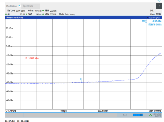
Band4-20MHz-16QAM-20050-100RB#0
