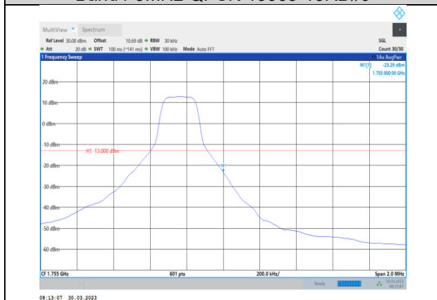
Band4-3MHz-QPSK-20385-1RB#14
