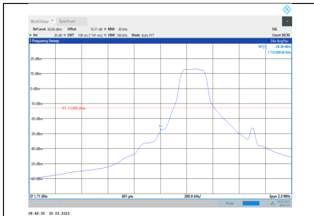
Band4-1.4MHz-QPSK-19957-1RB#0
