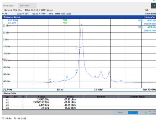
Band7-10MHz-QPSK-20800-1RB#0
