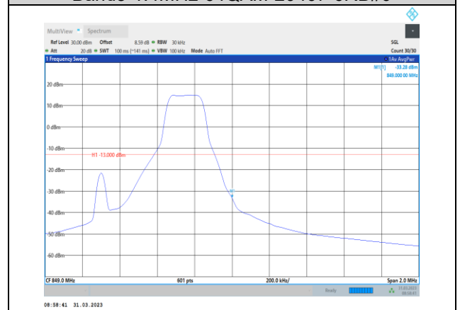
Band5-1.4MHz-64QAM-20643-1RB#5
