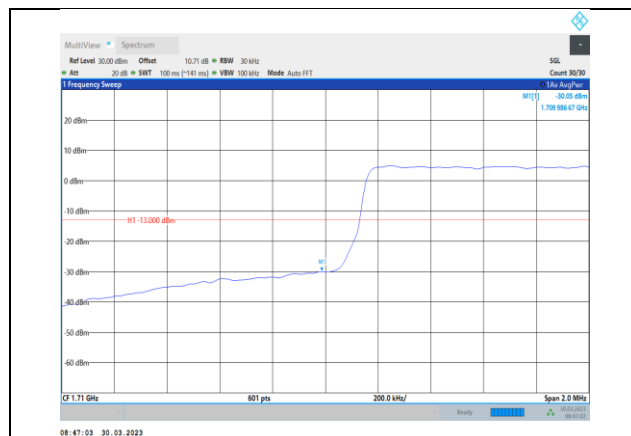
Band4-1.4MHz-64QAM-19957-6RB#0
