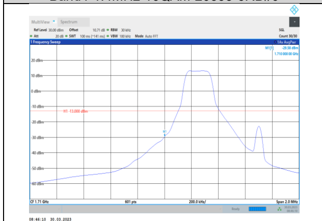
Band4-1.4MHz-64QAM-19957-1RB#0
