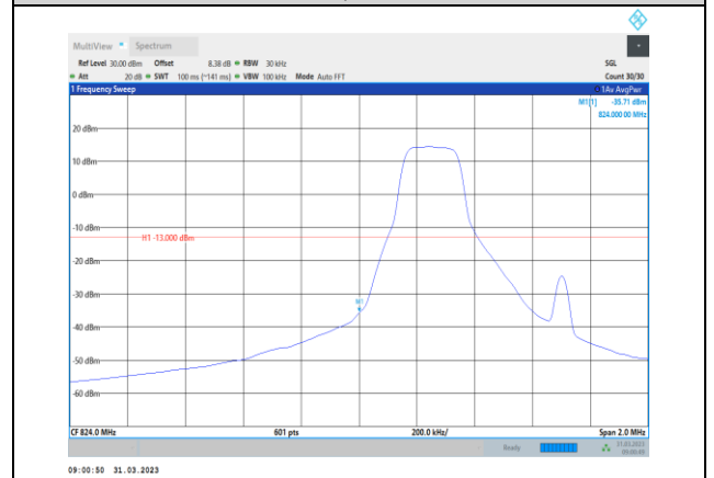
Band5-1.4MHz-16QAM-20407-1RB#0
