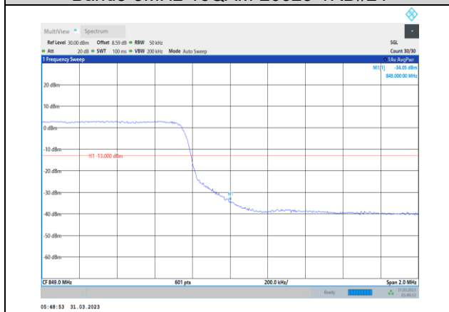
Band5-5MHz-16QAM-20625-25RB#0
