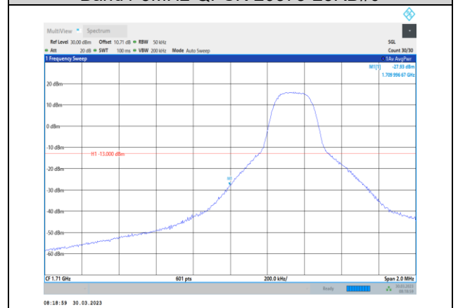
Band4-5MHz-16QAM-19975-1RB#0
