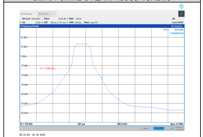
Band4-3MHz-64QAM-20385-1RB#14
