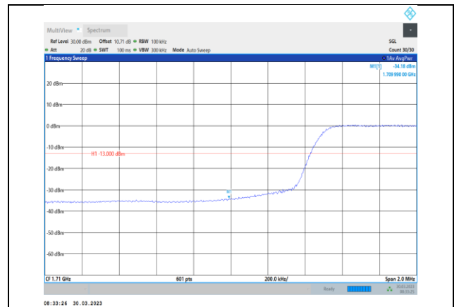
Band4-10MHz-64QAM-20000-50RB#0
