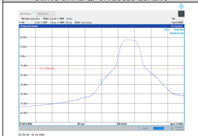
Band5-5MHz-16QAM-20425-1RB#0
