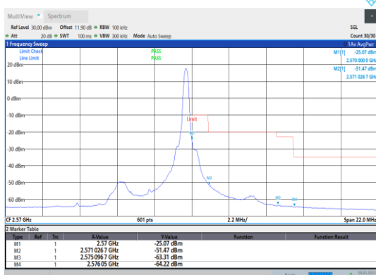
Band7-5MHz-QPSK-21425-1RB#24
