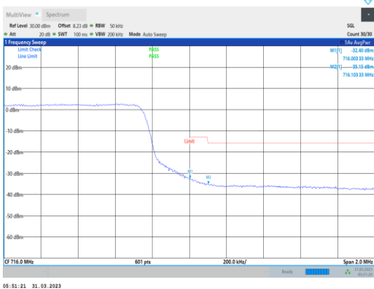
Band17-5MHz-16QAM-23825-25RB#0
