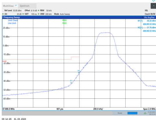
Band12-5MHz-64QAM-23035-1RB#0
