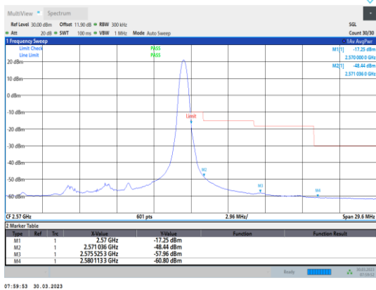
Band7-10MHz-16QAM-21400-1RB#49
