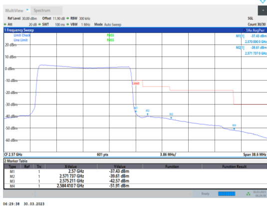
Band7-15MHz-16QAM-21375-75RB#0
