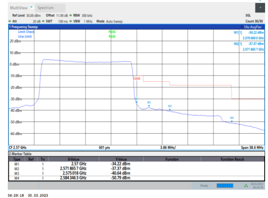
Band7-15MHz-QPSK-21375-75RB#0
