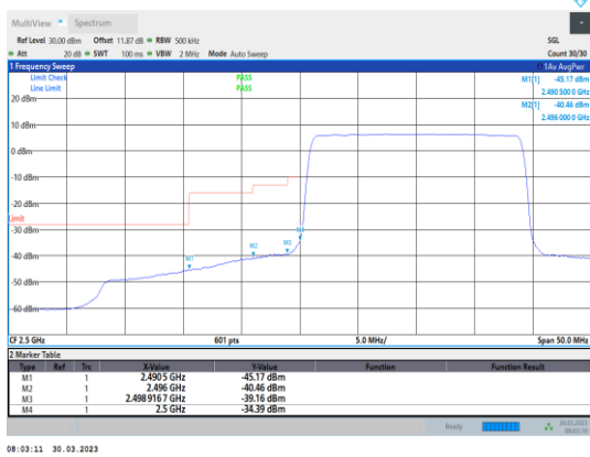
Band7-20MHz-QPSK-20850-100RB#0
