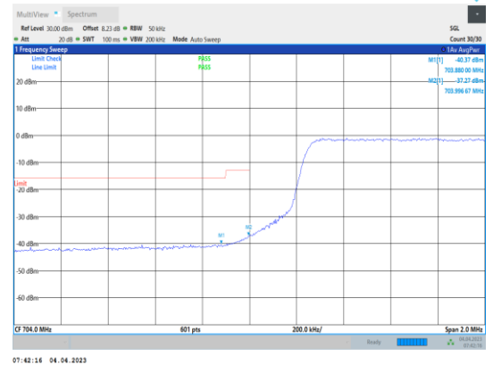
Band17-5MHz-64QAM-23755-25RB#0
