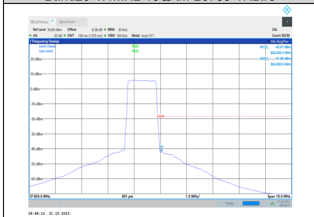
Band26-1.4MHz-16QAM-26783-6RB#0
