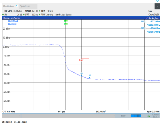
Band12-5MHz-16QAM-23155-25RB#0
