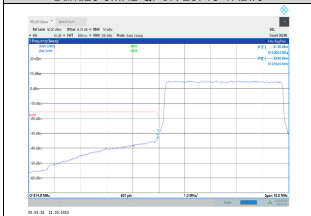
Band26-5MHz-QPSK-26715-25RB#0
