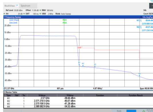
Band7-20MHz-64QAM-21350-100RB#0
