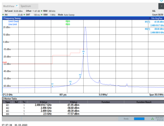
Band7-10MHz-64QAM-20800-1RB#0
