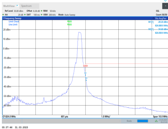
Band26-5MHz-16QAM-26765-1RB#24
