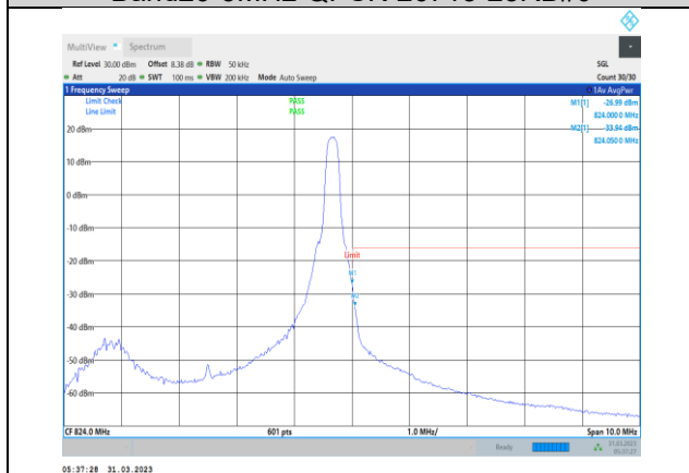
Band26-5MHz-QPSK-26765-1RB#24
