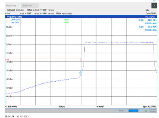
Band26-5MHz-64QAM-26715-25RB#0
