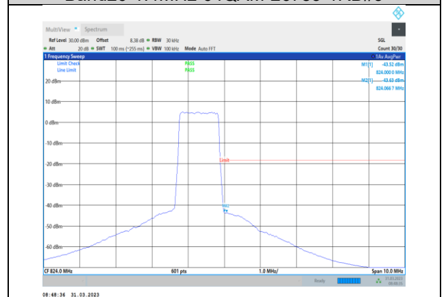
Band26-1.4MHz-64QAM-26783-6RB#0
