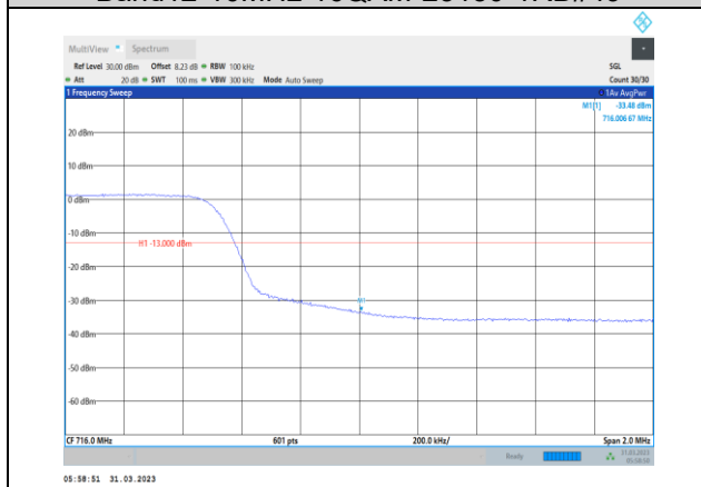
Band12-10MHz-16QAM-23130-50RB#0
