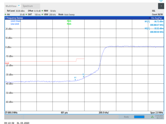
Band12-5MHz-16QAM-23035-25RB#0
