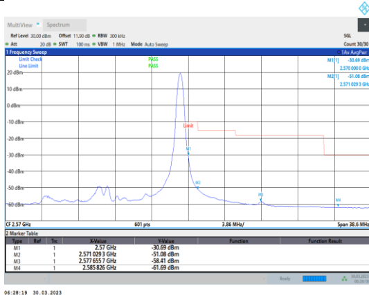
Band7-15MHz-QPSK-21375-1RB#74
