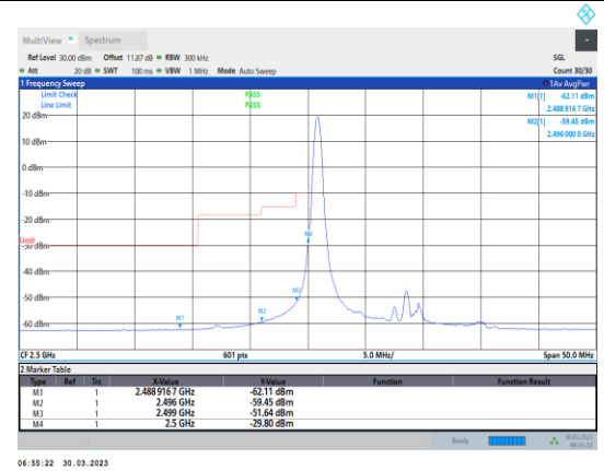
Band7-15MHz-16QAM-20825-1RB#0
