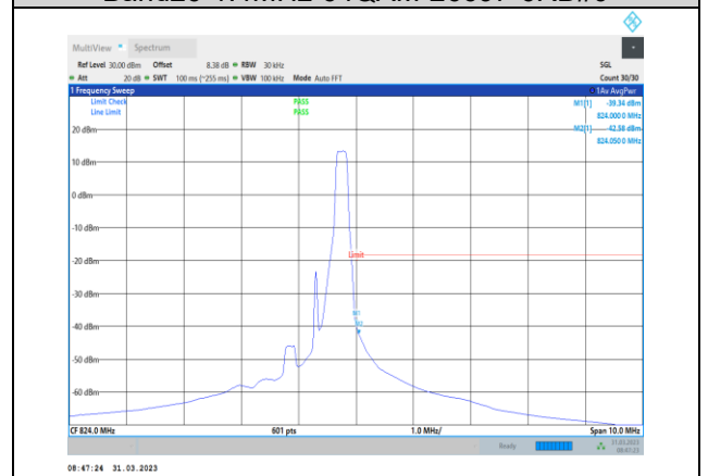
Band26-1.4MHz-64QAM-26783-1RB#5
