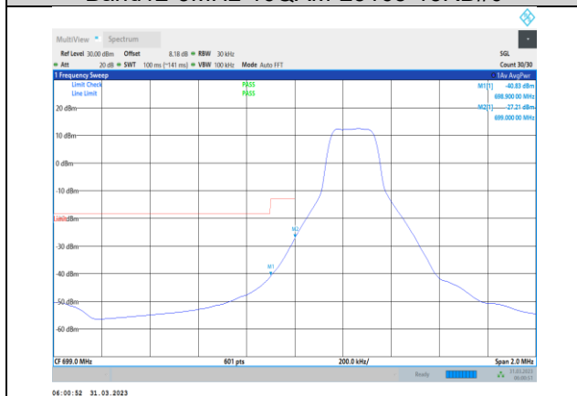
Band12-3MHz-64QAM-23025-1RB#0
