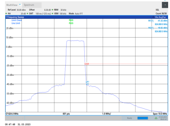
Band26-1.4MHz-QPSK-26783-6RB#0
