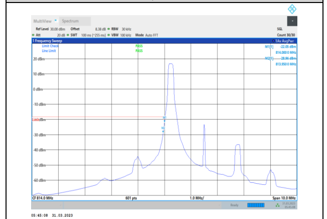
Band26-3MHz-16QAM-26705-1RB#0
