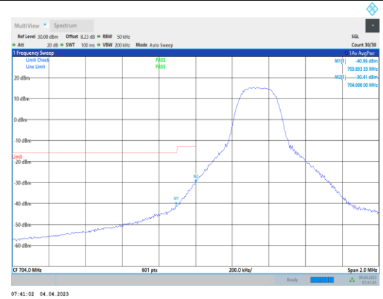
Band17-5MHz-16QAM-23755-1RB#0
