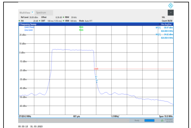
Band26-3MHz-QPSK-26775-15RB#0
