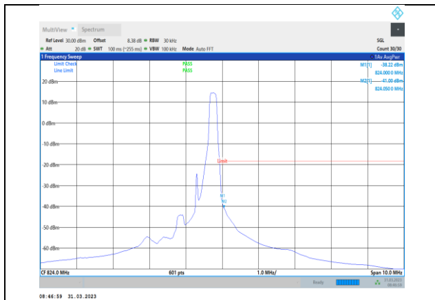
Band26-1.4MHz-16QAM-26783-1RB#5
