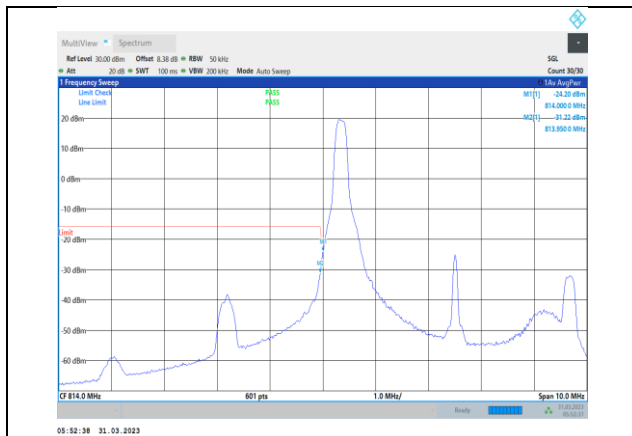
Band26-5MHz-QPSK-26715-1RB#0
