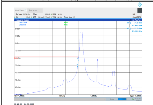
Band26-3MHz-64QAM-26705-1RB#0
