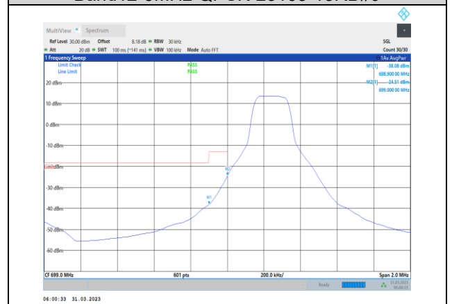
Band12-3MHz-16QAM-23025-1RB#0
