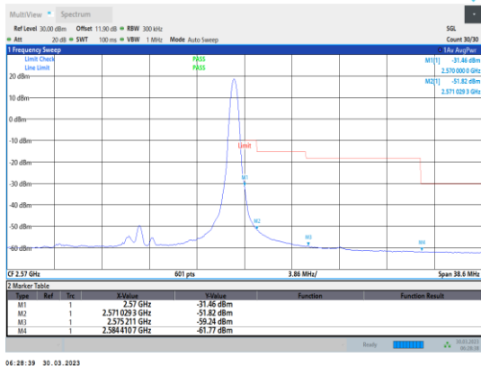
Band7-15MHz-16QAM-21375-1RB#74
