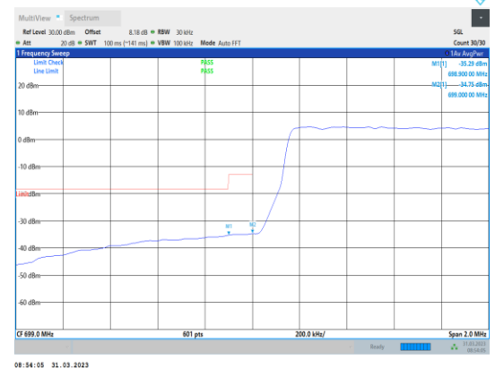
Band12-1.4MHz-16QAM-23017-6RB#0
