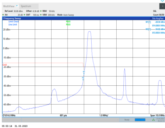
Band26-5MHz-64QAM-26715-1RB#0
