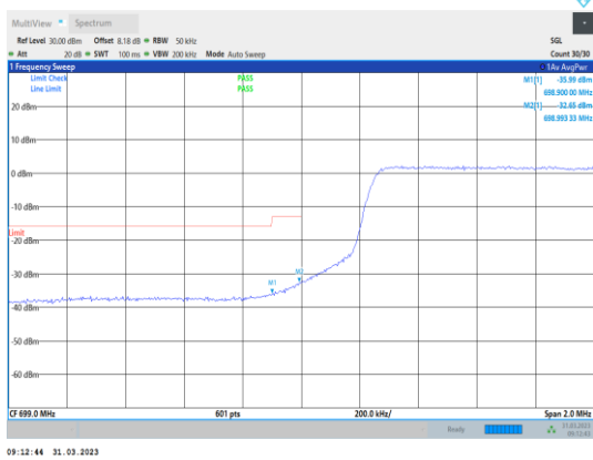
Band12-5MHz-QPSK-23035-25RB#0
