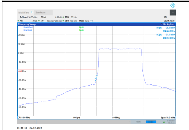
Band26-3MHz-QPSK-26705-15RB#0
