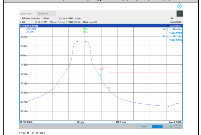
Band12-3MHz-64QAM-23165-1RB#14
