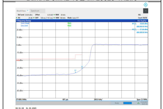
Band12-3MHz-16QAM-23025-15RB#0
