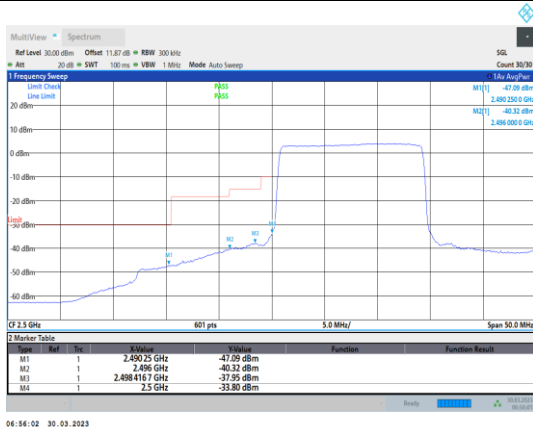
Band7-15MHz-QPSK-20825-75RB#0
