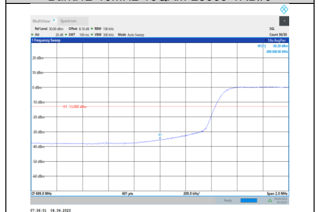
Band12-10MHz-16QAM-23060-50RB#0
