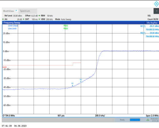
Band17-5MHz-QPSK-23755-25RB#0
