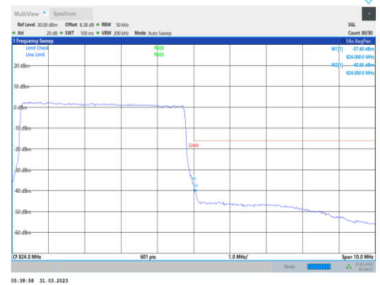
Band26-5MHz-64QAM-26765-25RB#0
