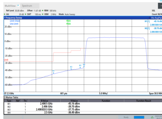
Band7-20MHz-64QAM-20850-100RB#0
