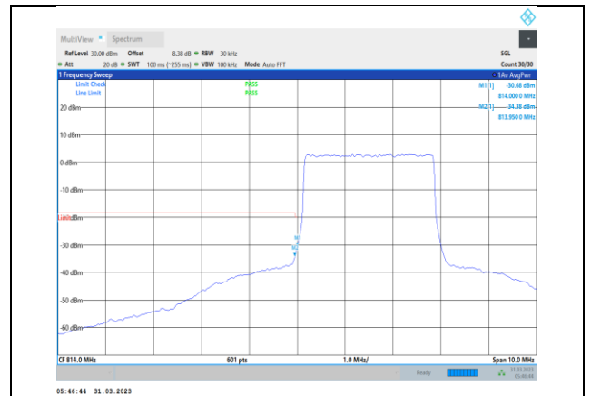
Band26-3MHz-64QAM-26705-15RB#0
