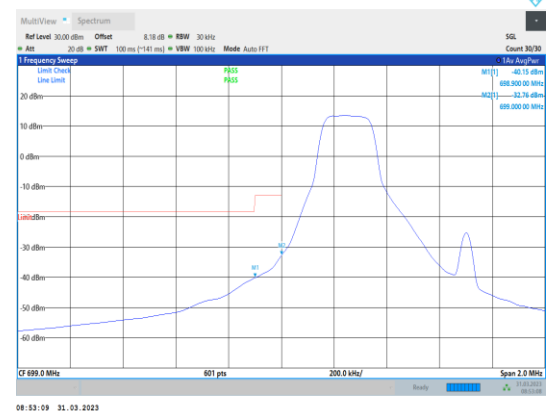
Band12-1.4MHz-16QAM-23017-1RB#0
