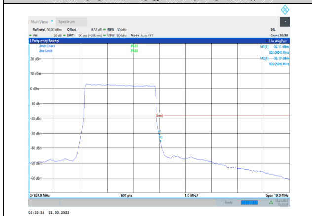
Band26-3MHz-16QAM-26775-15RB#0
