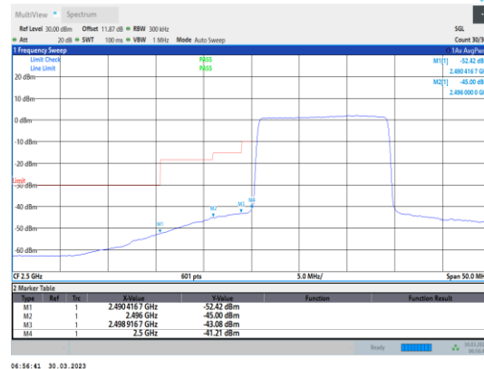
Band7-15MHz-64QAM-20825-75RB#0
