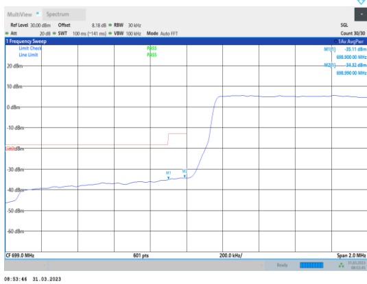
Band12-1.4MHz-QPSK-23017-6RB#0
