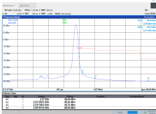
Band7-20MHz-16QAM-21350-1RB#99
