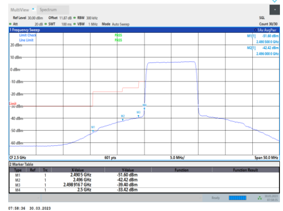
Band7-10MHz-64QAM-20800-50RB#0
