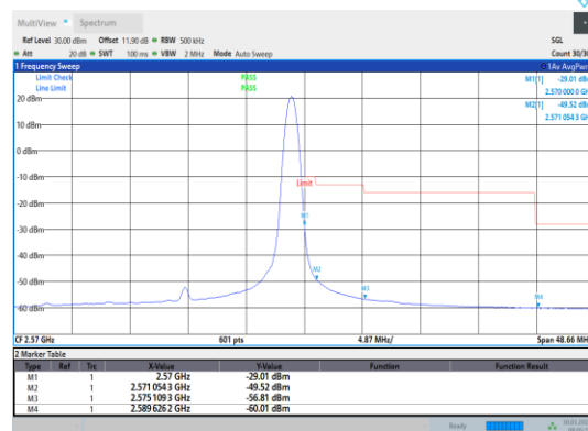
Band7-20MHz-64QAM-21350-1RB#99
