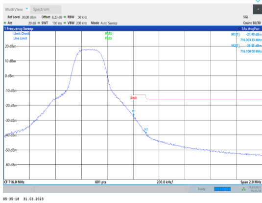
Band12-5MHz-16QAM-23155-1RB#24
