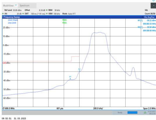
Band12-1.4MHz-QPSK-23017-1RB#0
