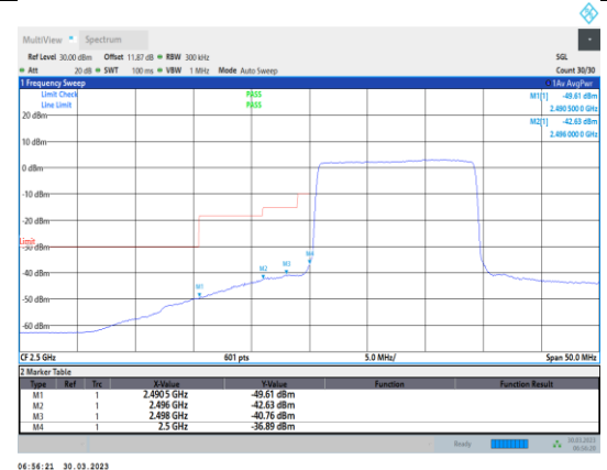
Band7-15MHz-16QAM-20825-75RB#0
