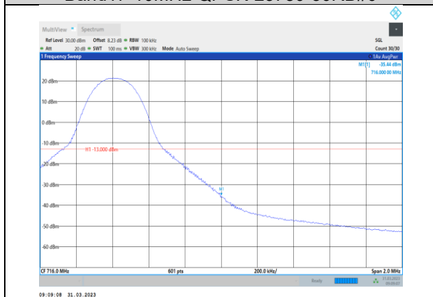
Band17-10MHz-QPSK-23800-1RB#49
