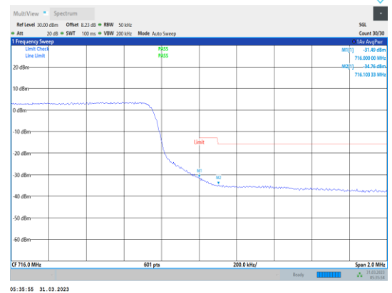
Band12-5MHz-QPSK-23155-25RB#0
