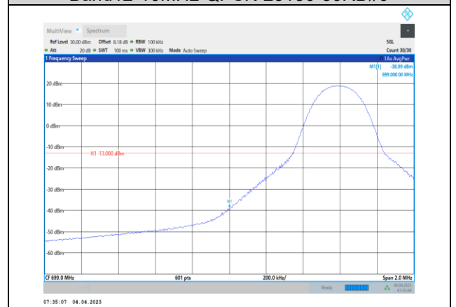
Band12-10MHz-16QAM-23060-1RB#0
