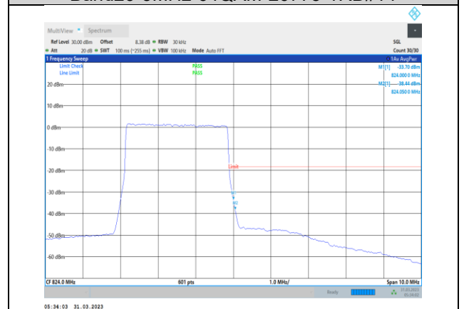
Band26-3MHz-64QAM-26775-15RB#0
