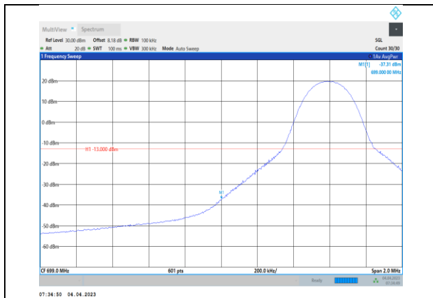
Band12-10MHz-QPSK-23060-1RB#0
