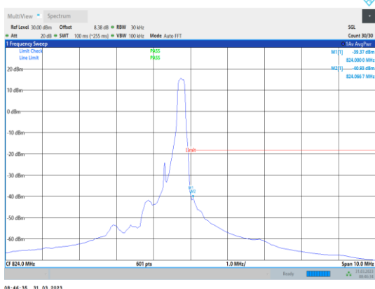
Band26-1.4MHz-QPSK-26783-1RB#5
