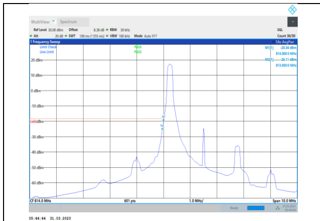
Band26-3MHz-QPSK-26705-1RB#0
