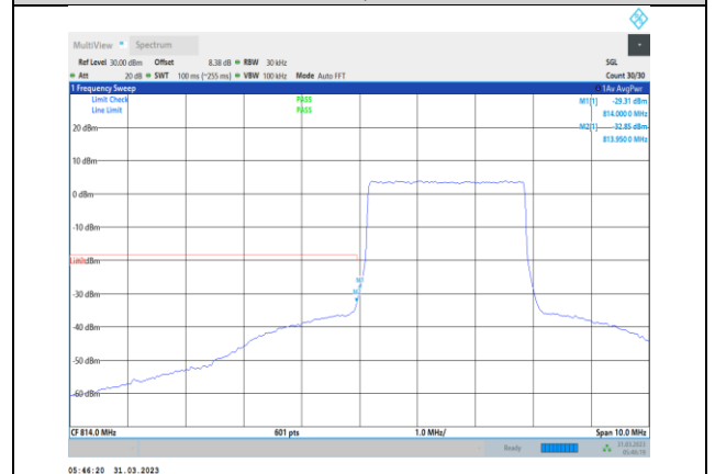
Band26-3MHz-16QAM-26705-15RB#0
