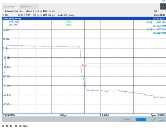
Band26-5MHz-16QAM-26765-25RB#0
