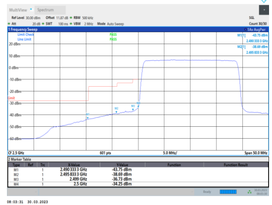
Band7-20MHz-16QAM-20850-100RB#0
