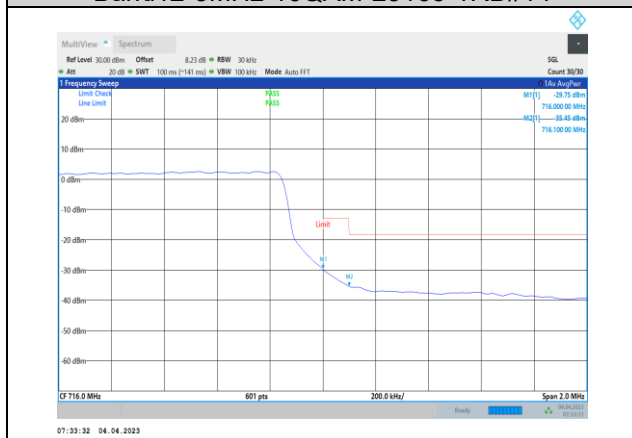
Band12-3MHz-16QAM-23165-15RB#0
