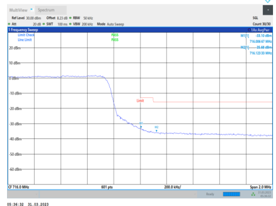
Band12-5MHz-64QAM-23155-25RB#0
