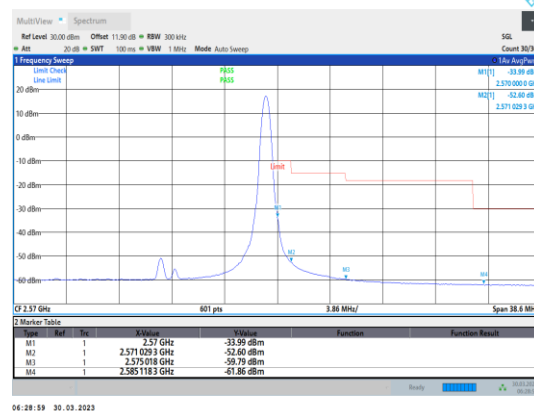
Band7-15MHz-64QAM-21375-1RB#74
