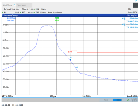
Band12-5MHz-QPSK-23155-1RB#24
