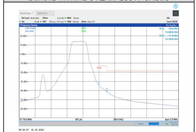
Band12-1.4MHz-64QAM-23173-1RB#5
