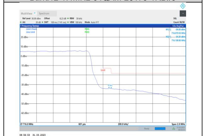
Band12-1.4MHz-64QAM-23173-6RB#0
