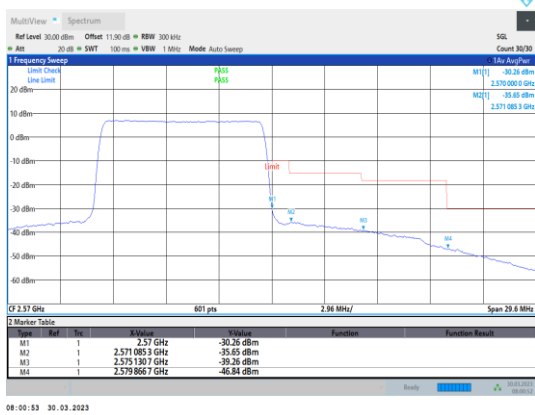
Band7-10MHz-16QAM-21400-50RB#0
