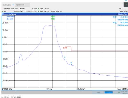
Band12-1.4MHz-QPSK-23173-1RB#5
