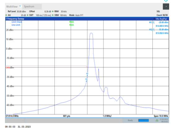
Band26-1.4MHz-16QAM-26697-1RB#0
