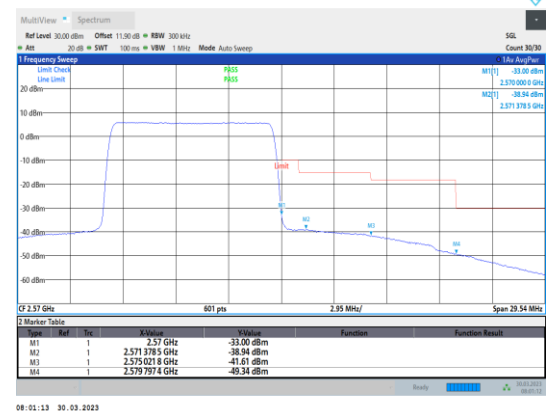
Band7-10MHz-64QAM-21400-50RB#0
