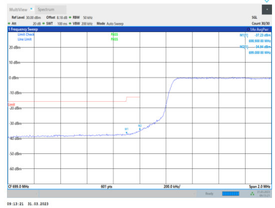
Band12-5MHz-64QAM-23035-25RB#0
