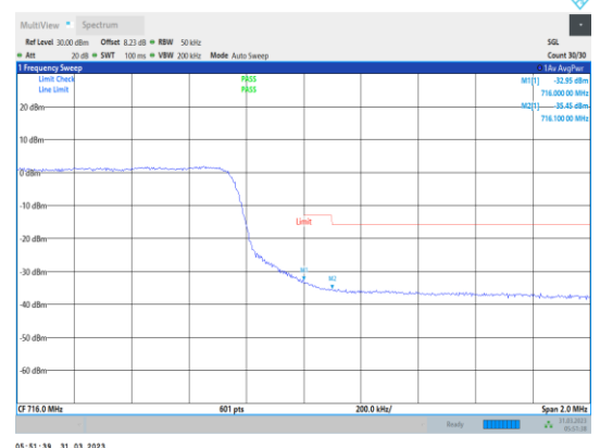
Band17-5MHz-64QAM-23825-25RB#0
