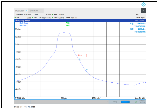
Band12-3MHz-16QAM-23165-1RB#14
