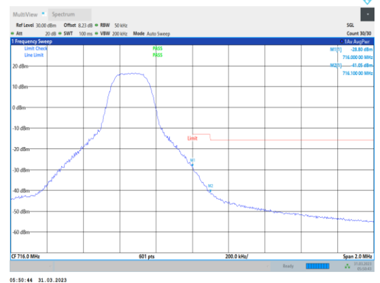
Band17-5MHz-64QAM-23825-1RB#24
