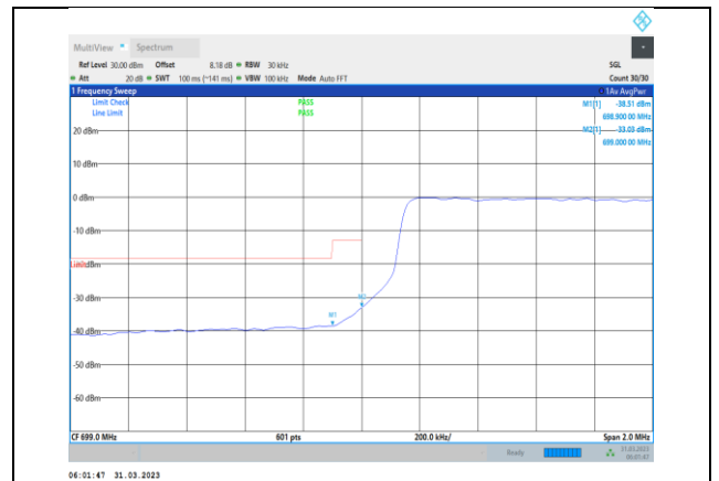
Band12-3MHz-64QAM-23025-15RB#0
