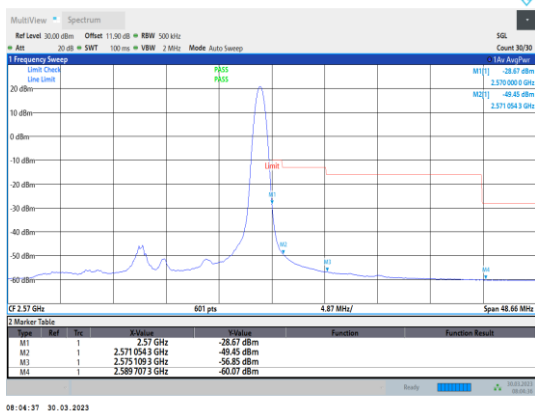
Band7-20MHz-QPSK-21350-1RB#99
