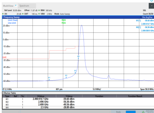
Band7-20MHz-64QAM-20850-1RB#0
