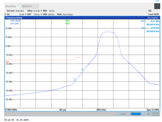
Band12-5MHz-16QAM-23035-1RB#0
