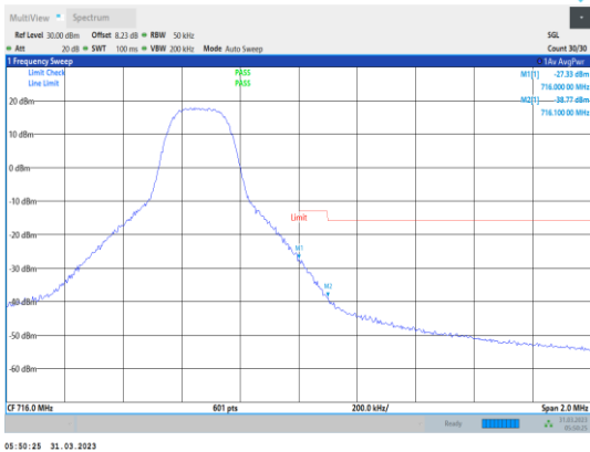
Band17-5MHz-16QAM-23825-1RB#24
