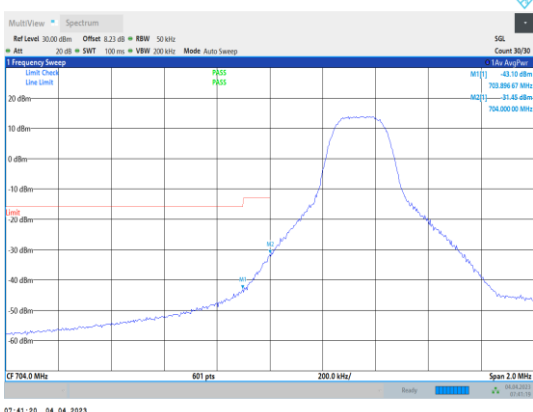
Band17-5MHz-64QAM-23755-1RB#0
