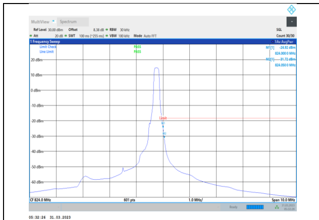
Band26-3MHz-16QAM-26775-1RB#14
