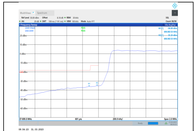
Band12-1.4MHz-64QAM-23017-6RB#0
