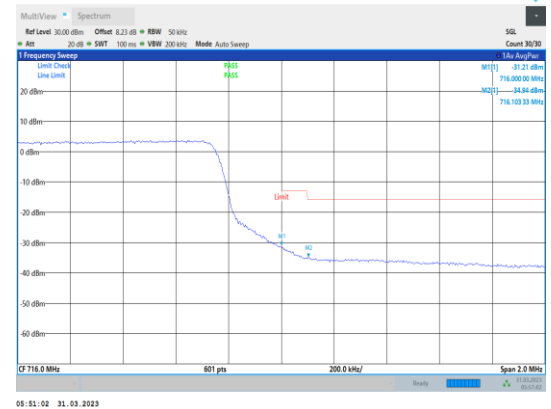
Band17-5MHz-QPSK-23825-25RB#0
