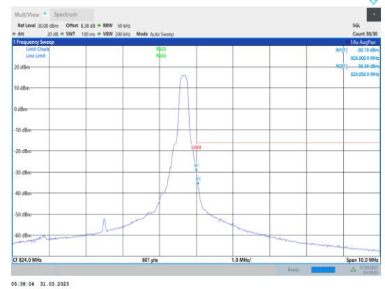
Band26-5MHz-64QAM-26765-1RB#24
