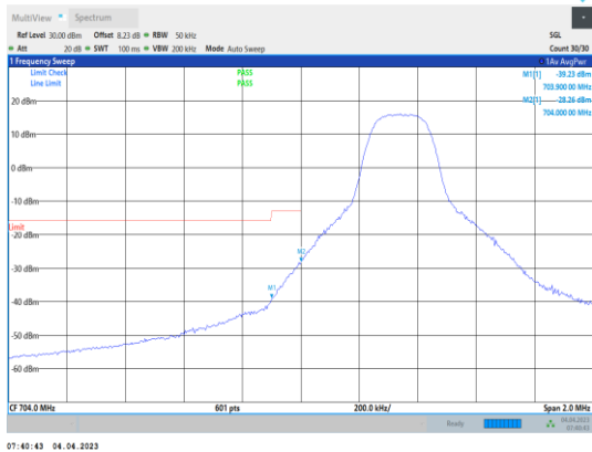
Band17-5MHz-QPSK-23755-1RB#0
