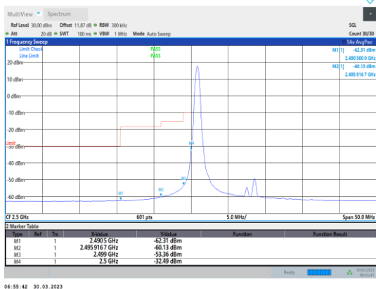
Band7-15MHz-64QAM-20825-1RB#0
