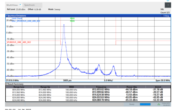
26(814-824)-10MHz-QPSK-26740-1RB#0
