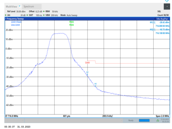
Band12-5MHz-64QAM-23155-1RB#24
