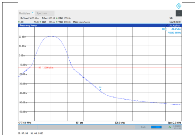
Band12-10MHz-16QAM-23130-1RB#49
