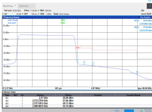
Band7-20MHz-16QAM-21350-100RB#0
