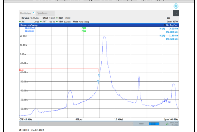
Band26-5MHz-16QAM-26715-1RB#0
