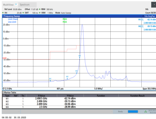
Band7-15MHz-QPSK-20825-1RB#0
