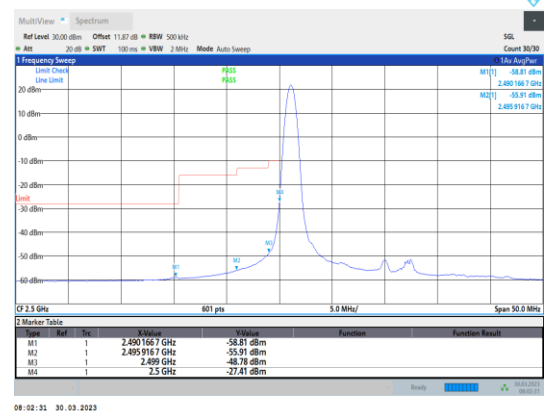
Band7-20MHz-16QAM-20850-1RB#0
