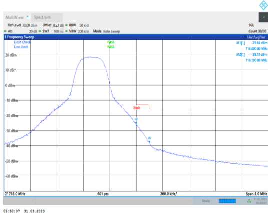
Band17-5MHz-QPSK-23825-1RB#24
