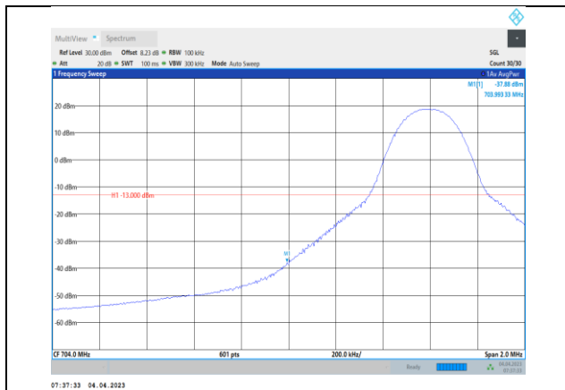
Band17-10MHz-QPSK-23780-1RB#0
