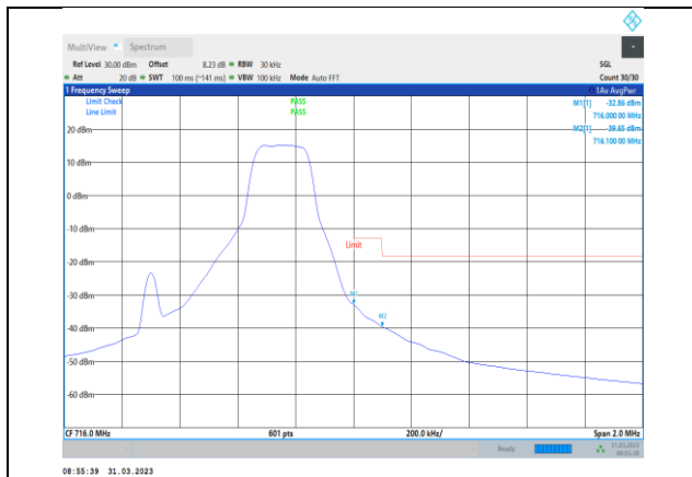
Band12-1.4MHz-16QAM-23173-1RB#5
