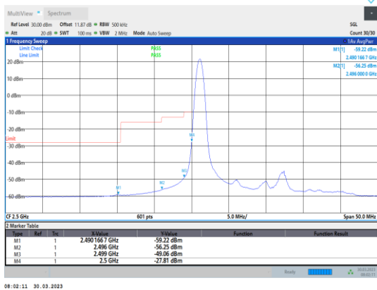
Band7-20MHz-QPSK-20850-1RB#0
