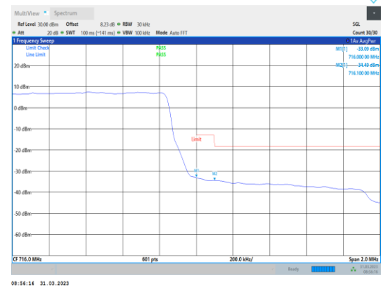
Band12-1.4MHz-QPSK-23173-6RB#0
