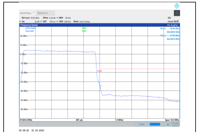
Band26-5MHz-QPSK-26765-25RB#0
