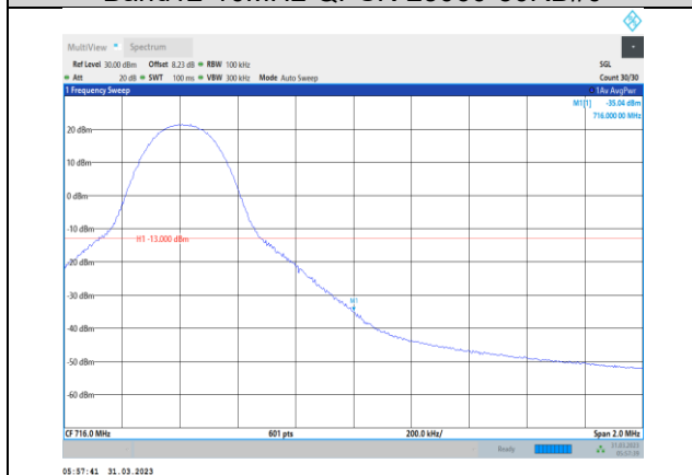
Band12-10MHz-QPSK-23130-1RB#49
