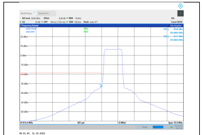
Band26-1.4MHz-64QAM-26697-6RB#0
