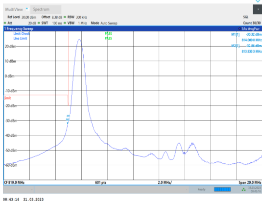
Band26-15MHz-QPSK-26765-1RB#0
