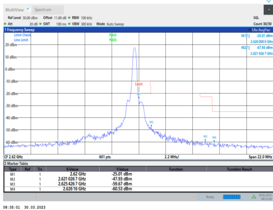
Band38-5MHz-16QAM-38225-1RB#24
