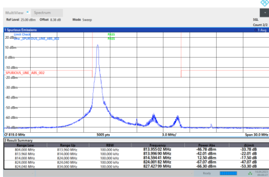
26(814-824)-10MHz-16QAM-26740-1RB#0
