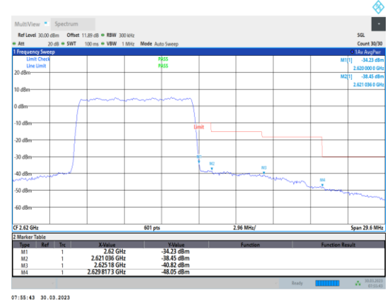
Band38-10MHz-64QAM-38200-50RB#0
