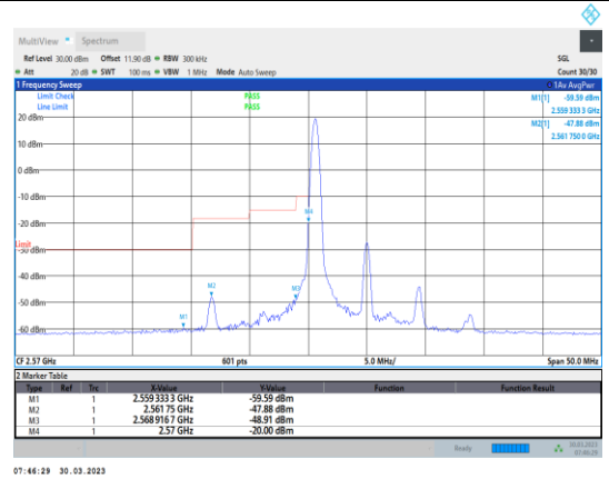
Band38-10MHz-16QAM-37800-1RB#0
