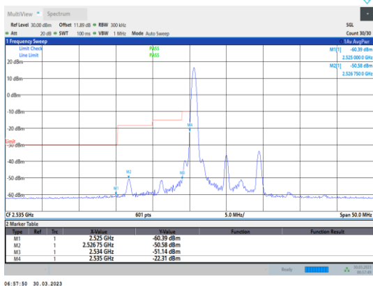
Band41-10MHz-QPSK-40090-1RB#0
