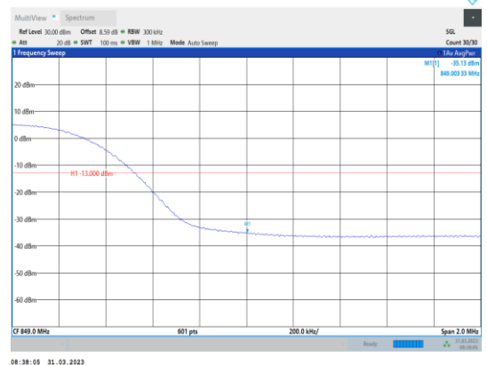
Band26-15MHz-16QAM-26965-75RB#0
