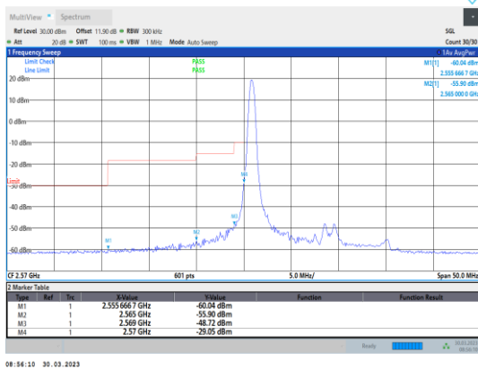
Band38-15MHz-QPSK-37825-1RB#0
