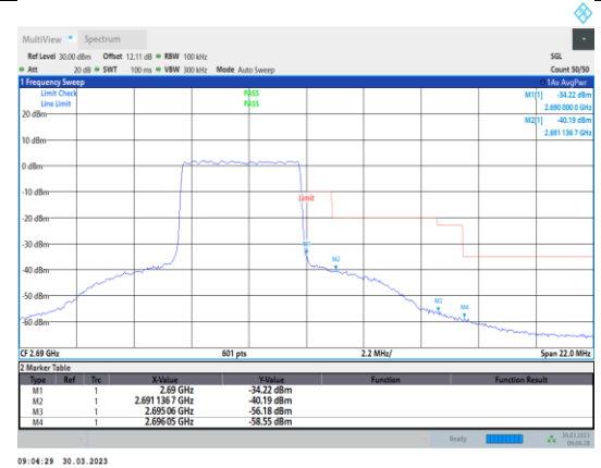
Band41-5MHz-64QAM-41565-25RB#0
