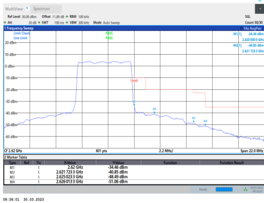
Band38-5MHz-16QAM-38225-25RB#0
