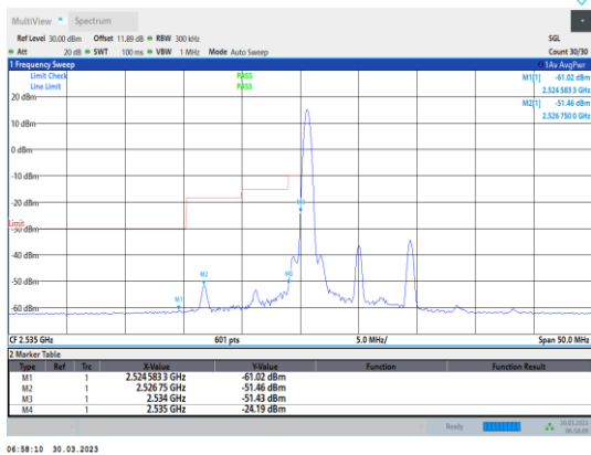
Band41-10MHz-16QAM-40090-1RB#0
