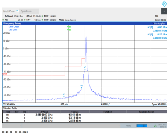
Band41-5MHz-64QAM-39675-1RB#0
