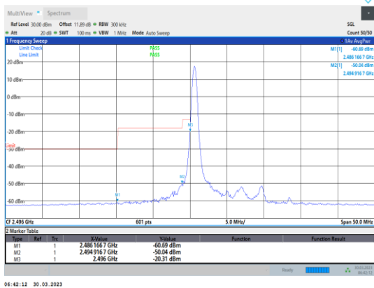
Band41-10MHz-QPSK-39700-1RB#0
