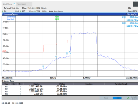
Band41-10MHz-16QAM-40090-50RB#0
