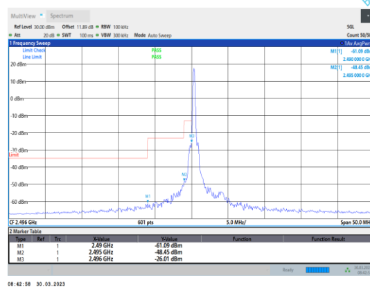
Band41-5MHz-16QAM-39675-1RB#0
