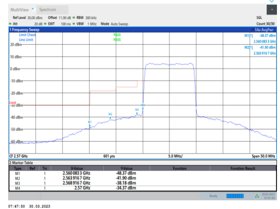
Band38-10MHz-64QAM-37800-50RB#0
