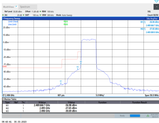
Band41-5MHz-QPSK-39675-25RB#0
