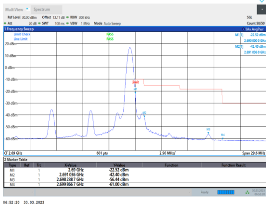
Band41-10MHz-16QAM-41540-1RB#49
