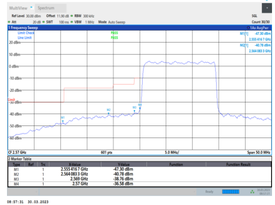
Band38-15MHz-16QAM-37825-75RB#0
