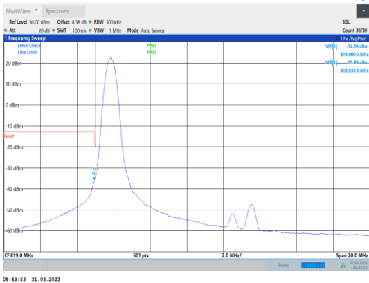
Band26-15MHz-64QAM-26765-1RB#0
