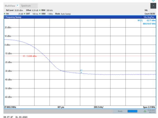
Band26-15MHz-QPSK-26965-75RB#0
