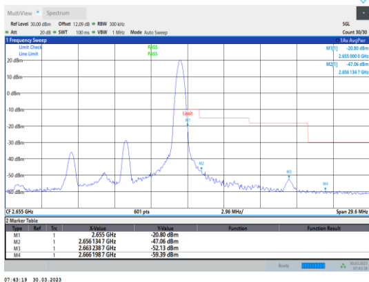
Band41-10MHz-QPSK-41190-1RB#49
