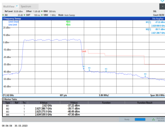
Band38-15MHz-16QAM-38175-75RB#0
