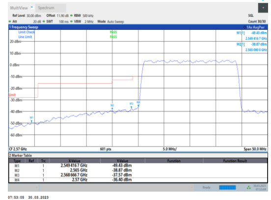
Band38-20MHz-64QAM-37850-100RB#0
