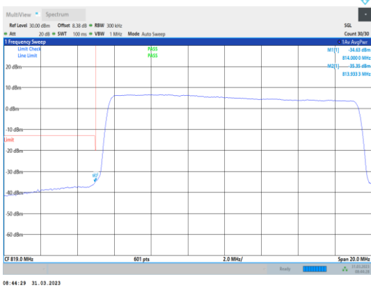
Band26-15MHz-16QAM-26765-75RB#0
