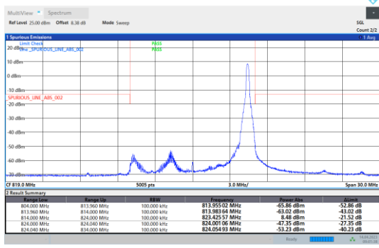
26(814-824)-10MHz-16QAM-26740-1RB#49
