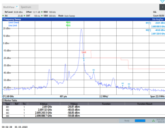
Band41-5MHz-QPSK-41565-1RB#24
