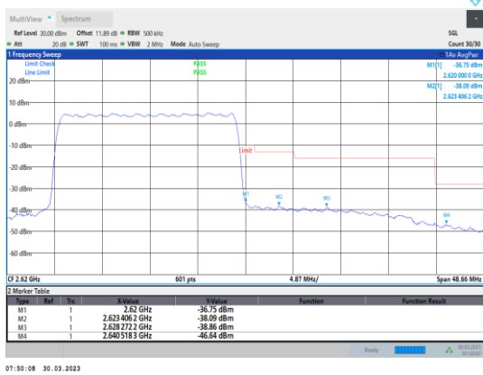
Band38-20MHz-16QAM-38150-100RB#0
