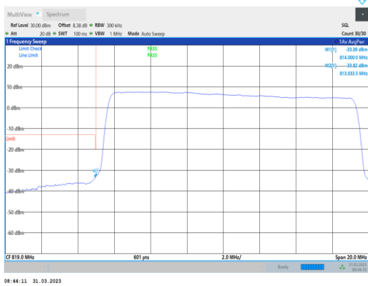
Band26-15MHz-QPSK-26765-75RB#0
