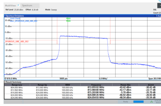
26(814-824)-10MHz-16QAM-26740-50RB#0
