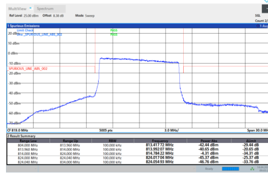
26(814-824)-10MHz-QPSK-26740-50RB#0
