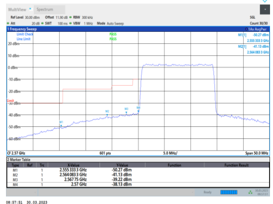
Band38-15MHz-64QAM-37825-75RB#0
