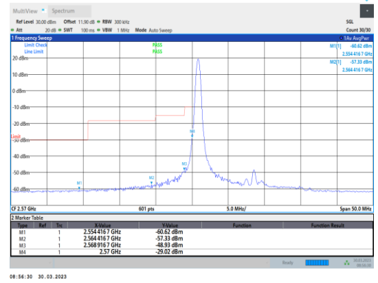
Band38-15MHz-16QAM-37825-1RB#0
