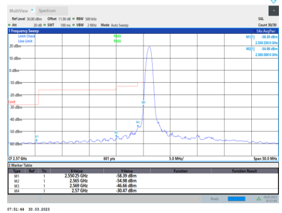
Band38-20MHz-16QAM-37850-1RB#0
