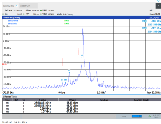
Band38-5MHz-QPSK-37775-1RB#0
