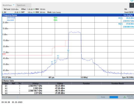
Band38-5MHz-QPSK-37775-25RB#0
