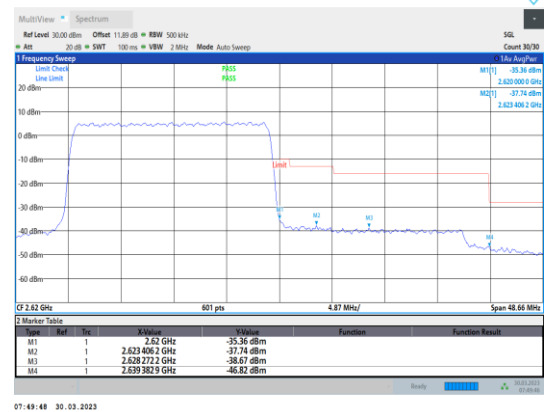
Band38-20MHz-QPSK-38150-100RB#0
