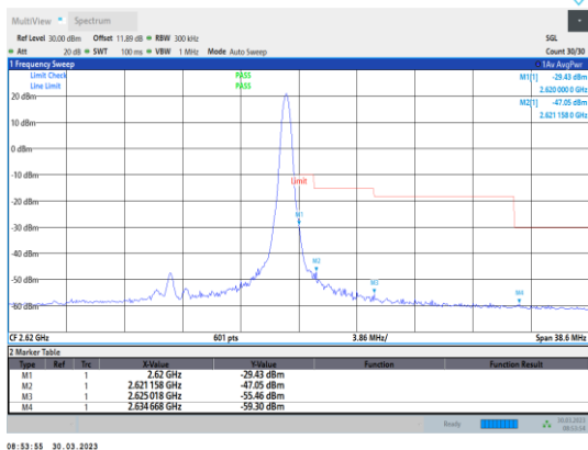
Band38-15MHz-16QAM-38175-1RB#74
