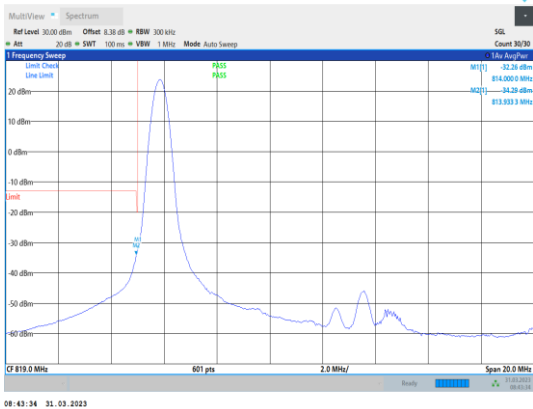
Band26-15MHz-16QAM-26765-1RB#0
