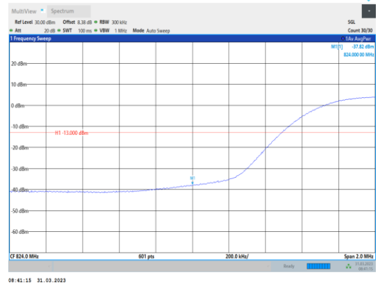
Band26-15MHz-16QAM-26865-75RB#0
