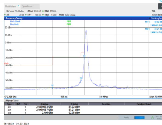
Band41-10MHz-16QAM-39700-1RB#0
