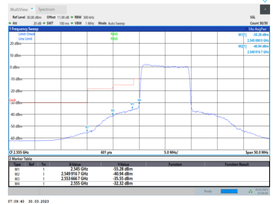
Band41-10MHz-16QAM-40290-50RB#0
