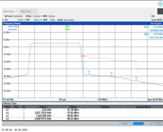
Band38-10MHz-16QAM-38200-50RB#0
