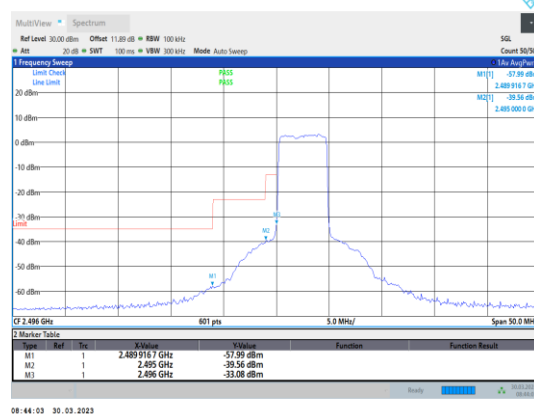
Band41-5MHz-16QAM-39675-25RB#0
