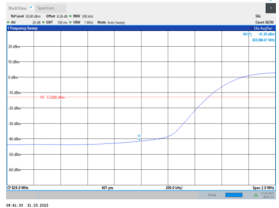
Band26-15MHz-64QAM-26865-75RB#0
