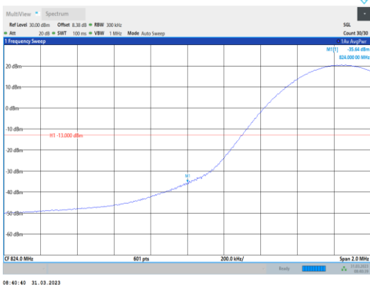
Band26-15MHz-64QAM-26865-1RB#0
