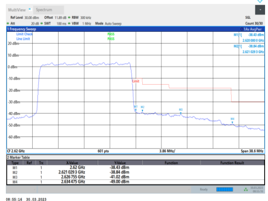
Band38-15MHz-64QAM-38175-75RB#0
