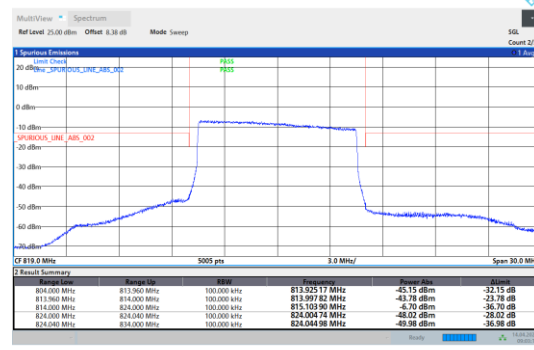
26(814-824)-10MHz-64QAM-26740-50RB#0
