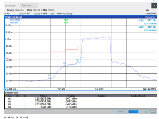
Band41-10MHz-QPSK-40090-50RB#0
