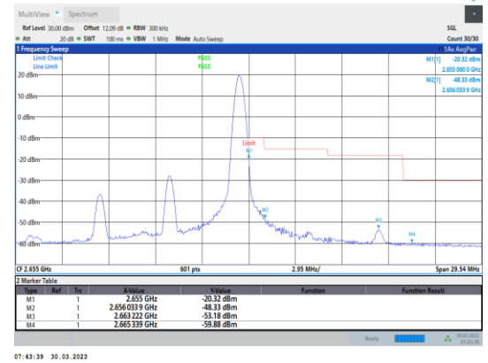
Band41-10MHz-16QAM-41190-1RB#49
