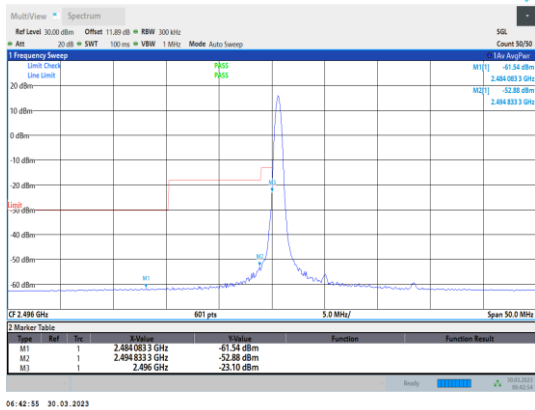
Band41-10MHz-64QAM-39700-1RB#0
