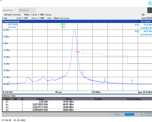
Band38-10MHz-QPSK-38200-1RB#49
