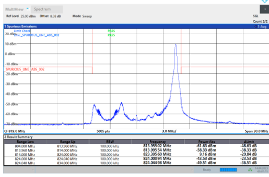
26(814-824)-10MHz-QPSK-26740-1RB#49
