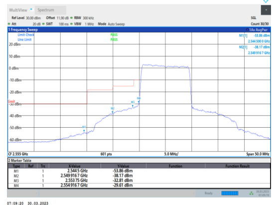
Band41-10MHz-QPSK-40290-50RB#0
