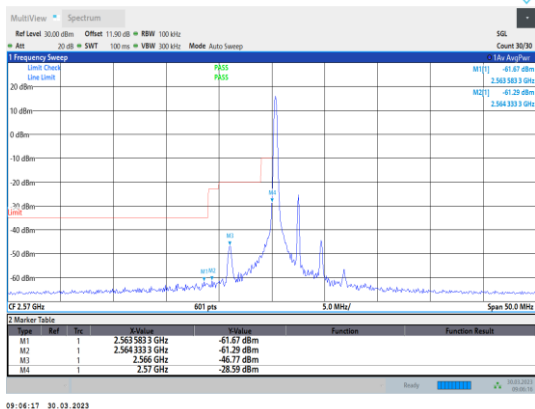
Band38-5MHz-64QAM-37775-1RB#0
