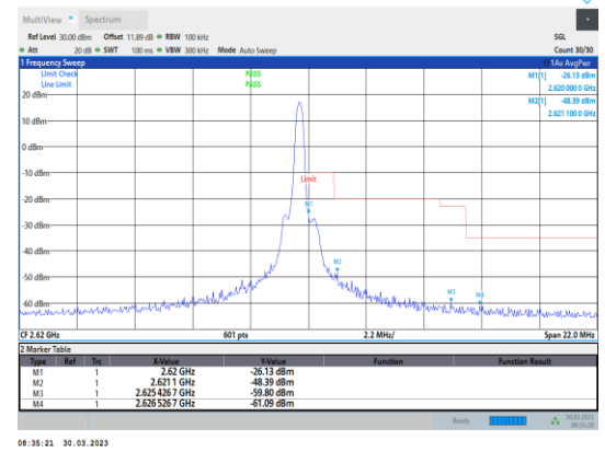
Band38-5MHz-64QAM-38225-1RB#24
