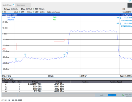
Band38-20MHz-QPSK-37850-100RB#0
