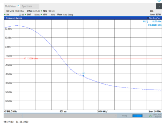
Band26-15MHz-16QAM-26965-1RB#74
