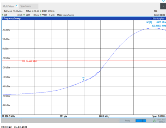
Band26-15MHz-16QAM-26865-1RB#0
