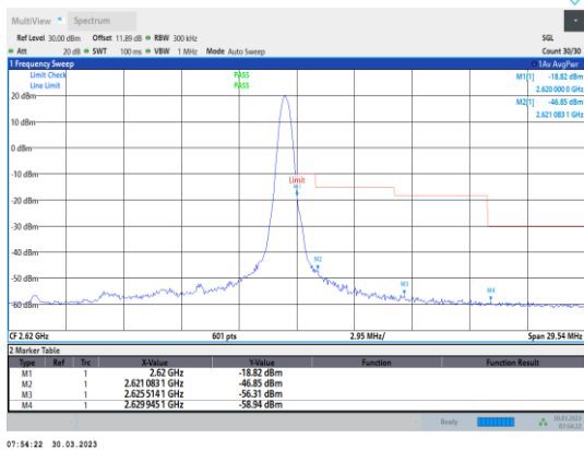
Band38-10MHz-16QAM-38200-1RB#49
