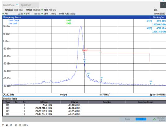
Band38-20MHz-16QAM-38150-1RB#99
