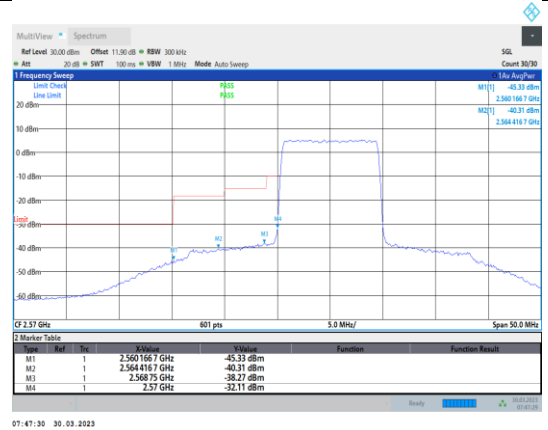
Band38-10MHz-16QAM-37800-50RB#0
