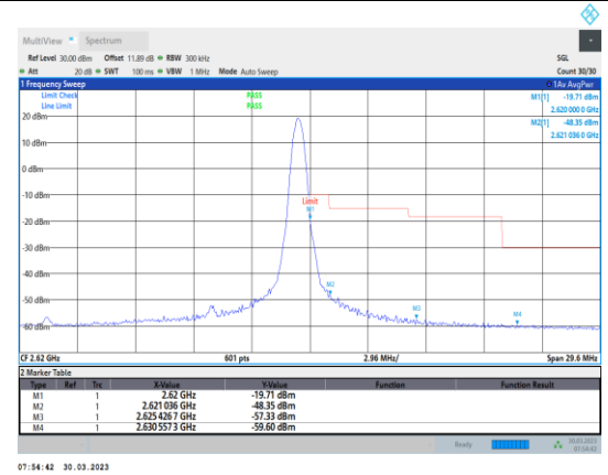
Band38-10MHz-64QAM-38200-1RB#49
