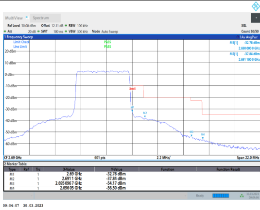
Band41-5MHz-16QAM-41565-25RB#0
