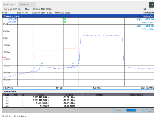
Band38-15MHz-QPSK-37825-75RB#0
