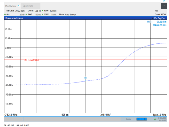
Band26-15MHz-QPSK-26865-75RB#0
