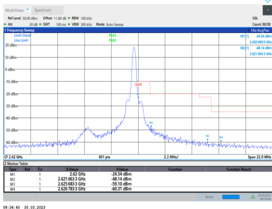
Band38-5MHz-QPSK-38225-1RB#24
