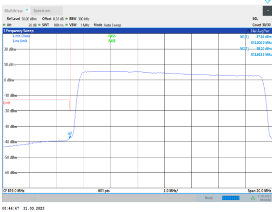
Band26-15MHz-64QAM-26765-75RB#0
