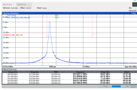
26(814-824)-10MHz-64QAM-26740-1RB#0
