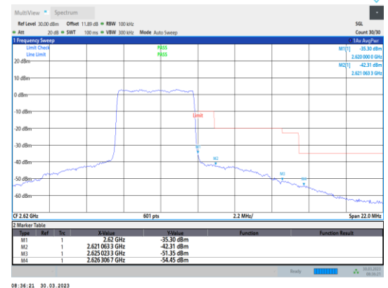
Band38-5MHz-64QAM-38225-25RB#0
