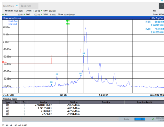
Band38-10MHz-QPSK-37800-1RB#0
