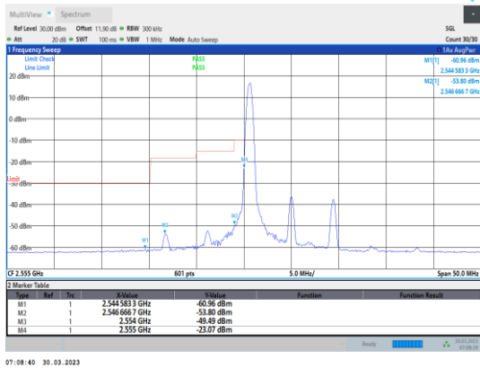
Band41-10MHz-16QAM-40290-1RB#0
