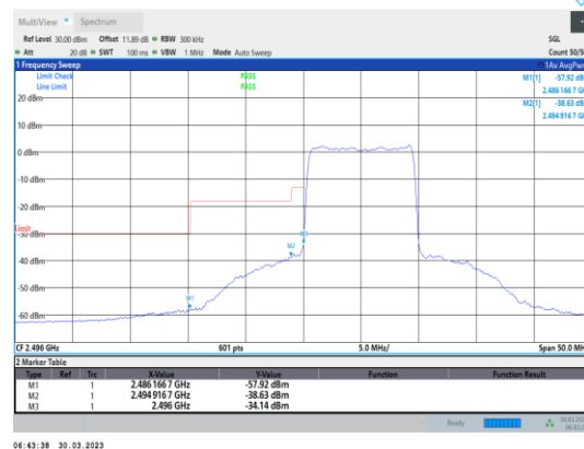
Band41-10MHz-16QAM-39700-50RB#0
