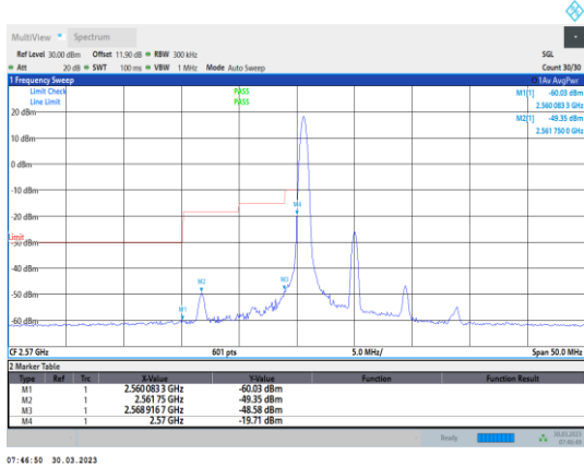
Band38-10MHz-64QAM-37800-1RB#0
