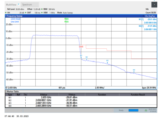
Band41-10MHz-16QAM-41190-50RB#0
