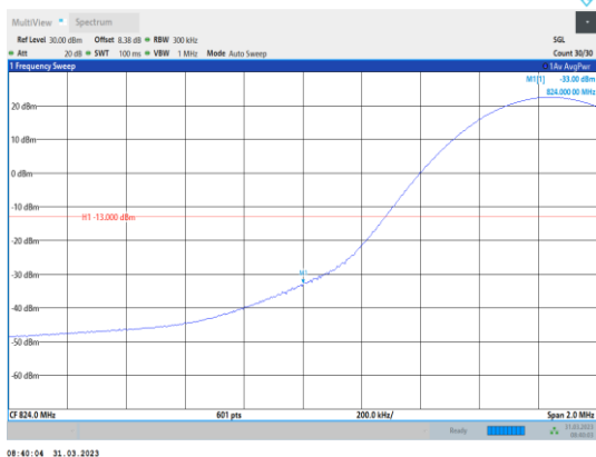
Band26-15MHz-QPSK-26865-1RB#0
