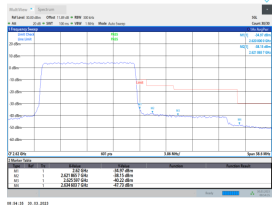
Band38-15MHz-QPSK-38175-75RB#0
