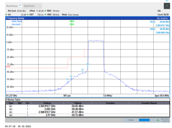
Band38-5MHz-64QAM-37775-25RB#0
