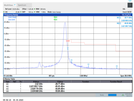
Band38-15MHz-64QAM-38175-1RB#74
