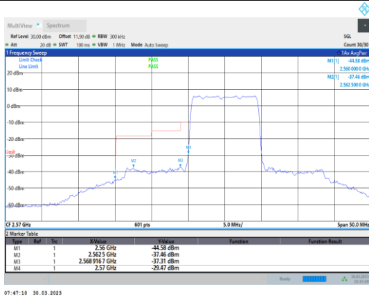
Band38-10MHz-QPSK-37800-50RB#0
