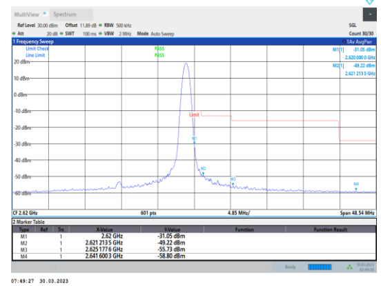
Band38-20MHz-64QAM-38150-1RB#99
