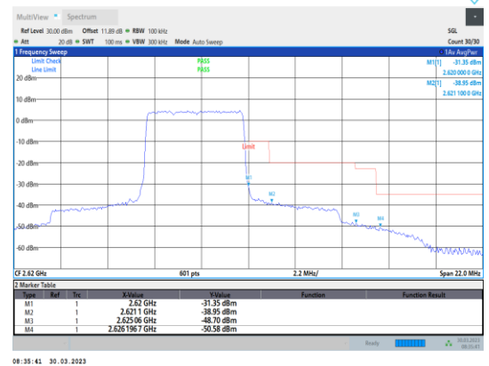
Band38-5MHz-QPSK-38225-25RB#0
