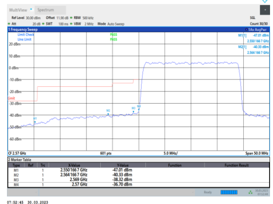
Band38-20MHz-16QAM-37850-100RB#0
