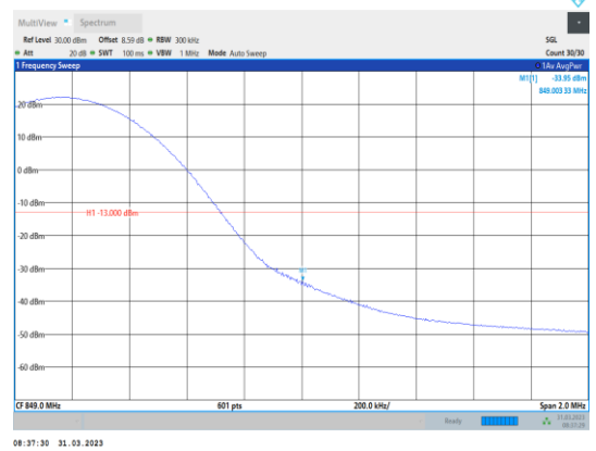
Band26-15MHz-64QAM-26965-1RB#74
