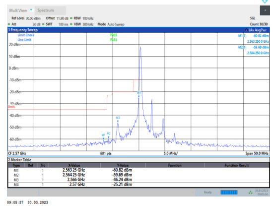
Band38-5MHz-16QAM-37775-1RB#0
