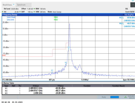
Band41-5MHz-QPSK-39675-1RB#0
