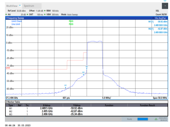
Band41-5MHz-64QAM-39675-25RB#0
