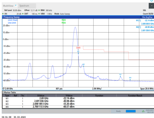
Band41-10MHz-QPSK-41540-1RB#49
