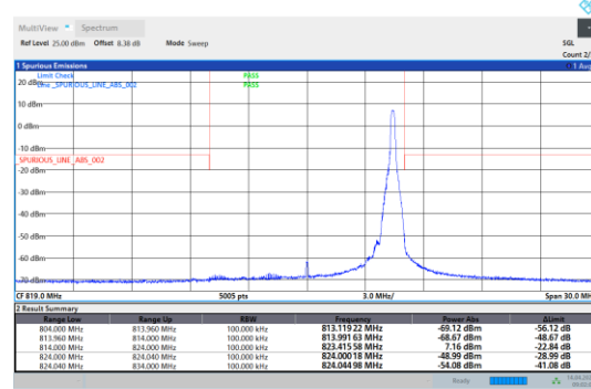
26(814-824)-10MHz-64QAM-26740-1RB#49
