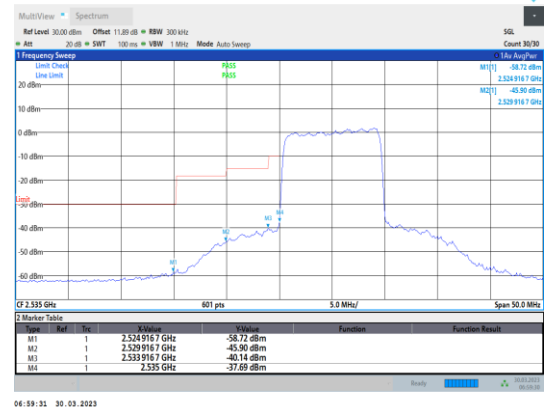
Band41-10MHz-64QAM-40090-50RB#0
