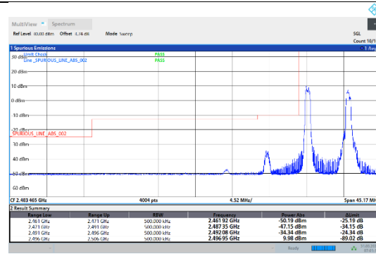
41-41-5MHz-20MHz-16QAM-16QAM-39683-39800-1RB#0-1RB#0
