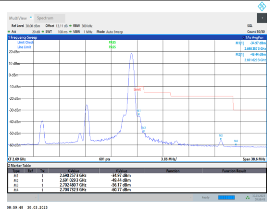
Band41-15MHz-64QAM-41515-1RB#74
