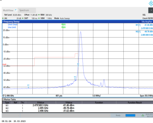
Band41-15MHz-64QAM-39725-1RB#0
