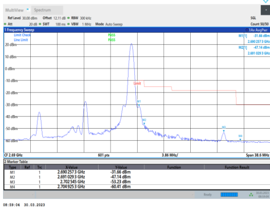
Band41-15MHz-QPSK-41515-1RB#74
