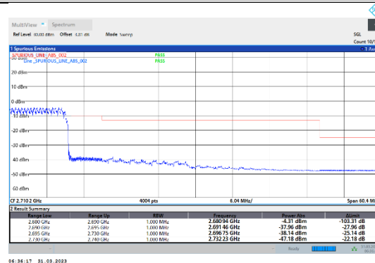
41-41-20MHz-20MHz-64QAM-64QAM-41292-41490-100RB#0-100RB#0
