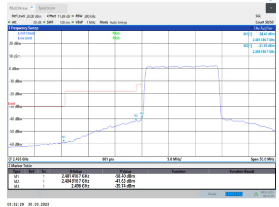
Band41-15MHz-64QAM-39725-75RB#0
