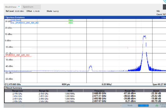
41-41-20MHz-20MHz-64QAM-64QAM-39750-39948-1RB#0-1RB#0
