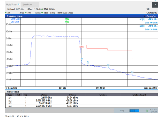
Band41-10MHz-64QAM-41190-50RB#0
