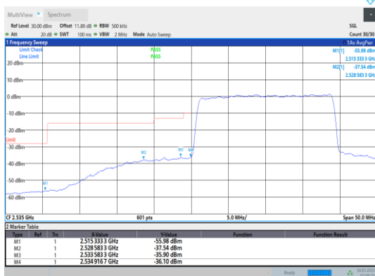
Band41-20MHz-16QAM-40140-100RB#0
