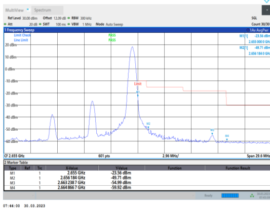
Band41-10MHz-64QAM-41190-1RB#49
