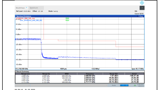
41-41-5MHz-20MHz-64QAM-64QAM-41373-41490-1RB#24-1RB#99
