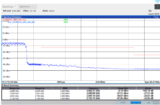
41-41-20MHz-20MHz-16QAM-16QAM-41292-41490-100RB#0-100RB#0
