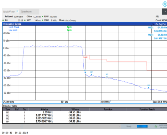
Band41-15MHz-16QAM-41515-75RB#0
