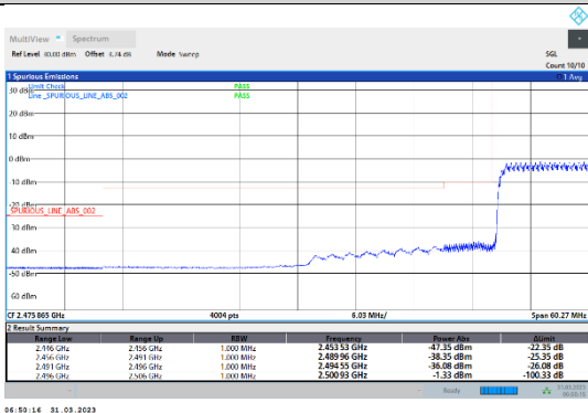
41-41-20MHz-20MHz-64QAM-64QAM-39750-39948-100RB#0-100RB#0
