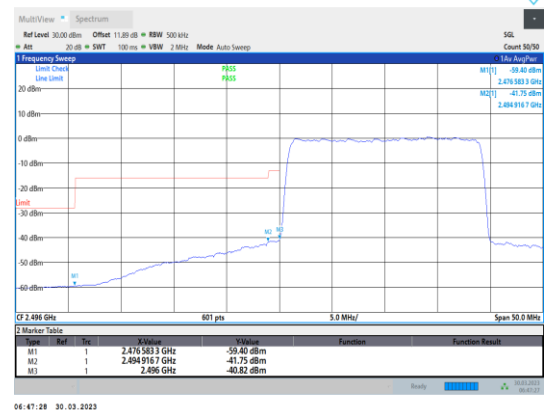
Band41-20MHz-64QAM-39750-100RB#0
