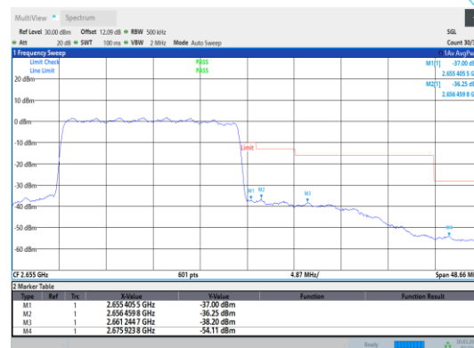
Band41-20MHz-16QAM-41140-100RB#0
