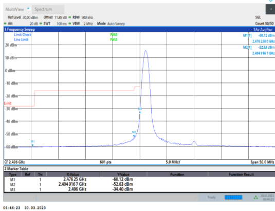
Band41-20MHz-64QAM-39750-1RB#0
