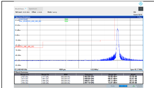
41-41-5MHz-20MHz-64QAM-64QAM-39683-39800-1RB#0-0RB#0
