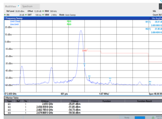
Band41-20MHz-16QAM-41140-1RB#99
