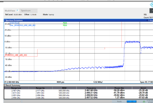
41-41-5MHz-20MHz-16QAM-16QAM-39683-39800-25RB#0-100RB#0
