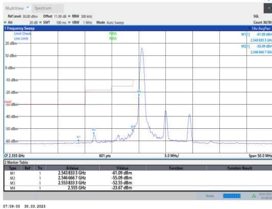
Band41-10MHz-64QAM-40290-1RB#0
