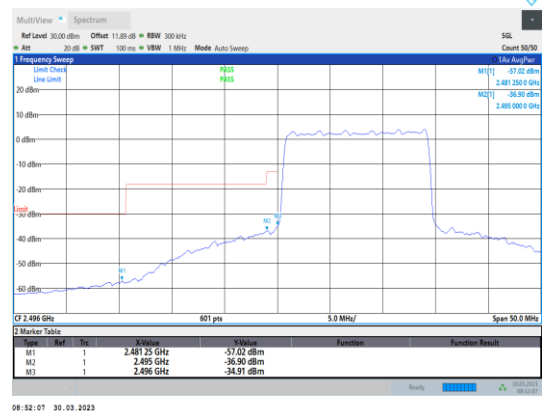
Band41-15MHz-16QAM-39725-75RB#0
