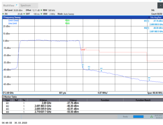
Band41-20MHz-16QAM-41490-100RB#0
