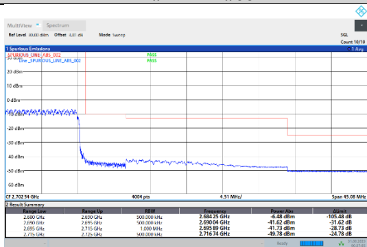
41-41-5MHz-20MHz-QPSK-QPSK-41373-41490-25RB#0-100RB#0
