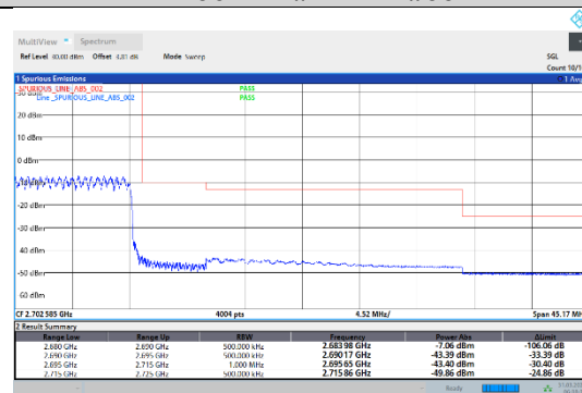
41-41-5MHz-20MHz-16QAM-16QAM-41373-41490-25RB#0-100RB#0
