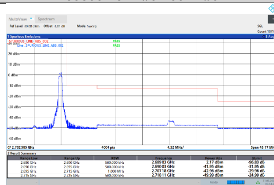
41-41-5MHz-20MHz-16QAM-16QAM-41373-41490-1RB#24-1RB#99
