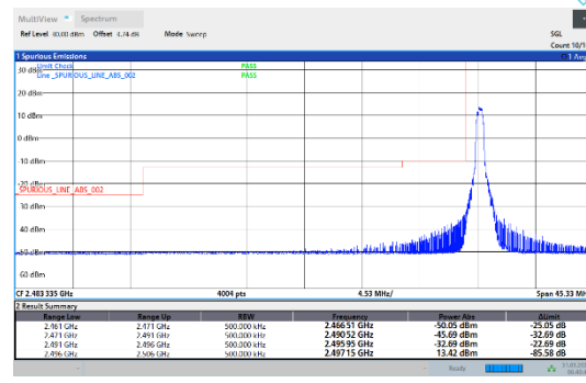
41-41-20MHz-5MHz-16QAM-16QAM-39750-39867-1RB#0-0RB#0
