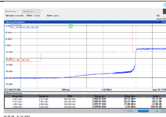
41-41-20MHz-5MHz-QPSK-QPSK-39750-39867-100RB#0-25RB#0
