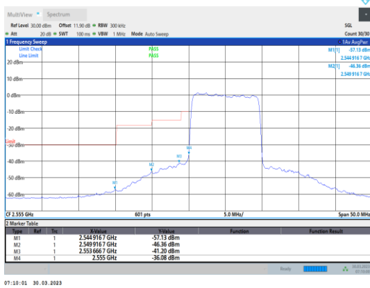
Band41-10MHz-64QAM-40290-50RB#0
