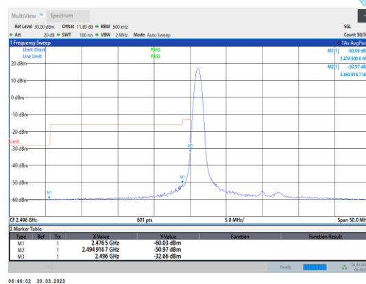
Band41-20MHz-16QAM-39750-1RB#0
