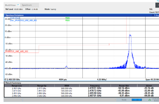
41-41-20MHz-5MHz-16QAM-16QAM-39750-39867-1RB#0-1RB#0
