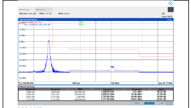
41-41-5MHz-20MHz-64QAM-64QAM-41373-41490-1RB#24-1RB#99
