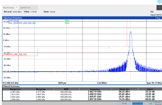
41-41-20MHz-5MHz-QPSK-QPSK-39750-39867-1RB#0-0RB#0
