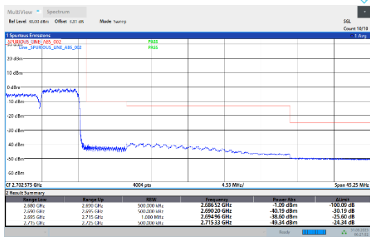
41-41-20MHz-5MHz-QPSK-QPSK-41440-41557-100RB#0-25RB#0
