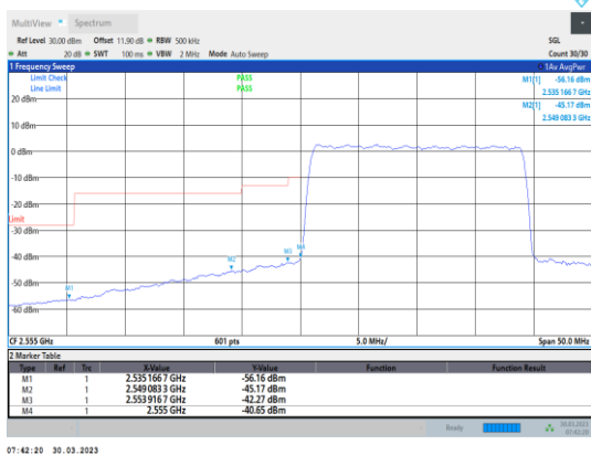
Band41-20MHz-64QAM-40340-100RB#0
