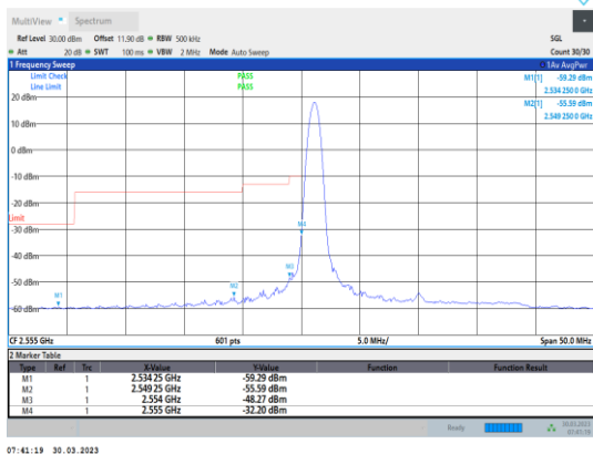
Band41-20MHz-64QAM-40340-1RB#0
