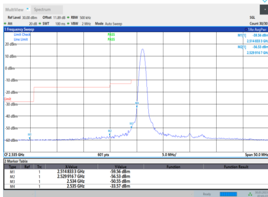
Band41-20MHz-16QAM-40140-1RB#0
