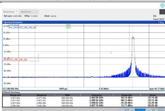
41-41-5MHz-20MHz-16QAM-16QAM-39683-39800-1RB#0-0RB#0
