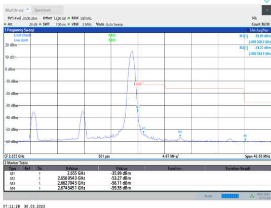
Band41-20MHz-64QAM-41140-1RB#99
