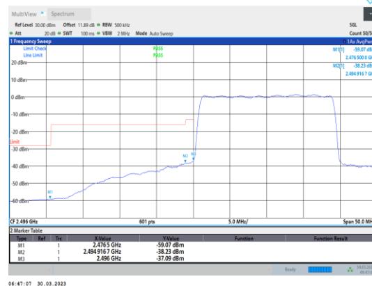
Band41-20MHz-16QAM-39750-100RB#0
