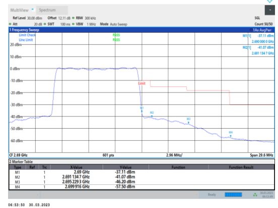
Band41-10MHz-64QAM-41540-50RB#0
