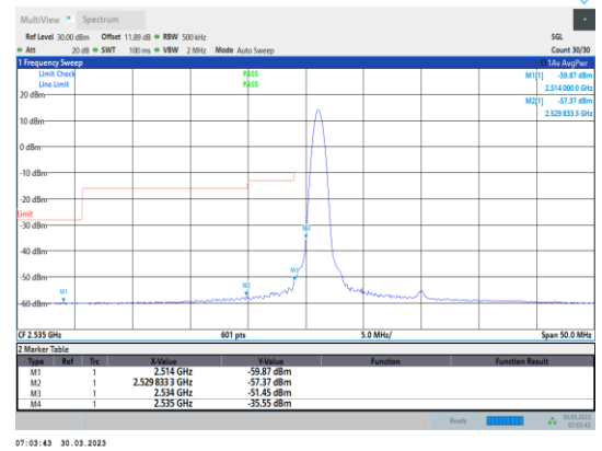
Band41-20MHz-64QAM-40140-1RB#0
