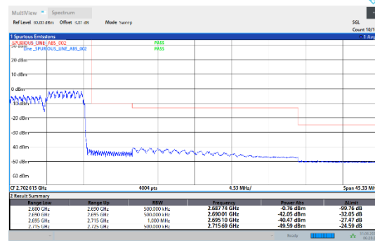
41-41-20MHz-5MHz-16QAM-16QAM-41440-41557-100RB#0-25RB#0
