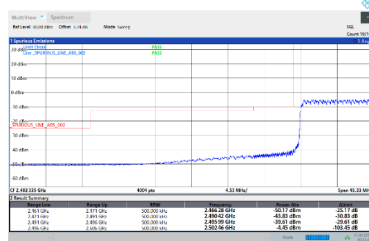
41-41-20MHz-5MHz-16QAM-16QAM-39750-39867-100RB#0-25RB#0
