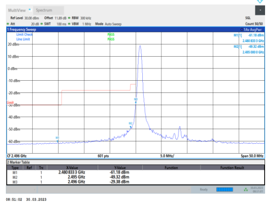
Band41-15MHz-16QAM-39725-1RB#0
