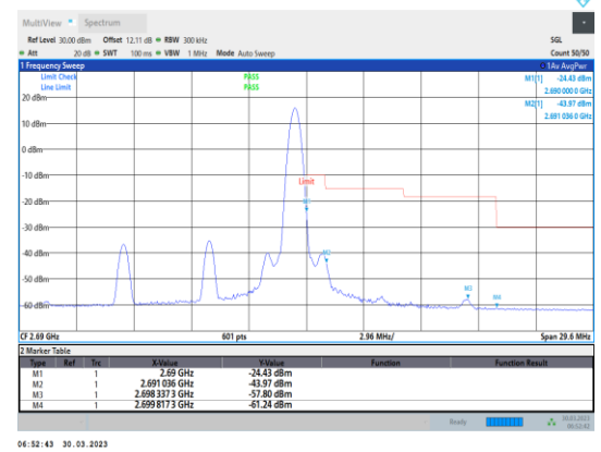
Band41-10MHz-64QAM-41540-1RB#49
