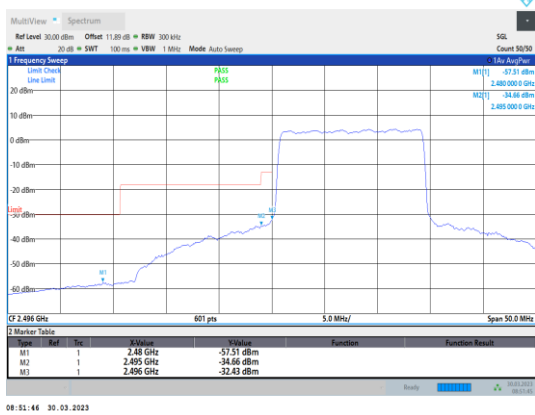
Band41-15MHz-QPSK-39725-75RB#0
