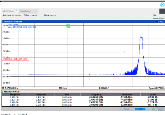
41-41-20MHz-20MHz-64QAM-64QAM-39750-39948-1RB#0-0RB#0
