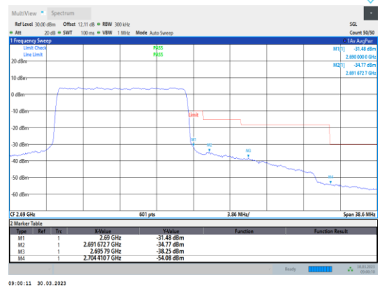
Band41-15MHz-QPSK-41515-75RB#0
