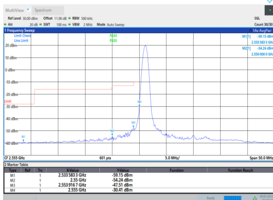
Band41-20MHz-16QAM-40340-1RB#0
