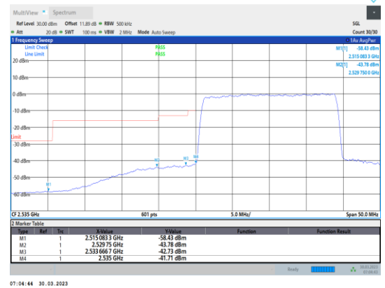
Band41-20MHz-64QAM-40140-100RB#0
