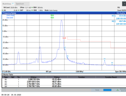
Band41-15MHz-16QAM-41515-1RB#74
