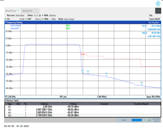
Band41-15MHz-64QAM-41515-75RB#0
