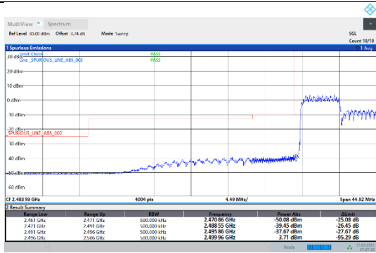
41-41-5MHz-20MHz-QPSK-QPSK-39683-39800-25RB#0-100RB#0
