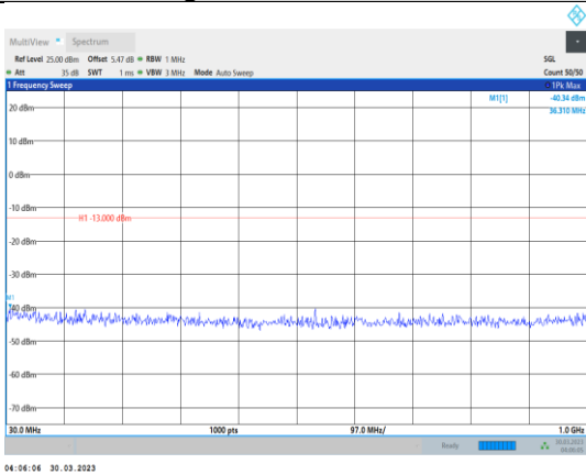
Band2-15MHz-QPSK-18900-1RB#0- Range1:30~1000MHz
