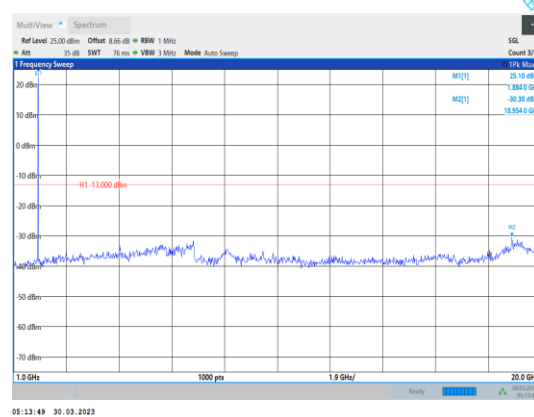
Band2-3MHz-16QAM-18900-1RB#0- Range2:1000~20000MHz
