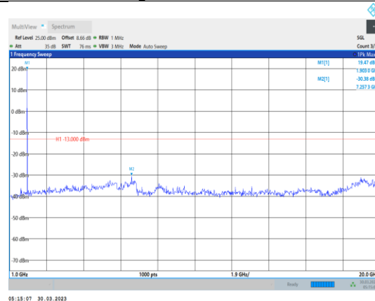
Band2-3MHz-16QAM-19185-1RB#0- Range2:1000~20000MHz
