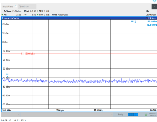
Band2-15MHz-64QAM-18675-1RB#0- Range1:30~1000MHz
