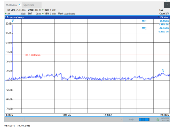
Band2-10MHz-16QAM-18900-1RB#0- Range2:1000~20000MHz
