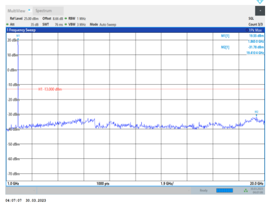
Band2-15MHz-64QAM-18900-1RB#0- Range2:1000~20000MHz
