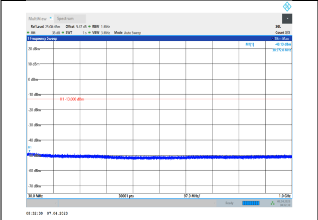
Band2-9538-30~1000MHz
