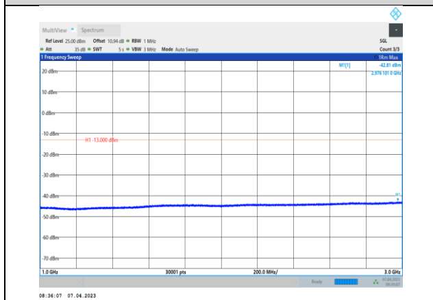
Band5-4132-1000~3000MHz
