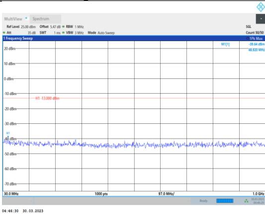
Band2-20MHz-64QAM-18900-1RB#0- Range1:30~1000MHz
