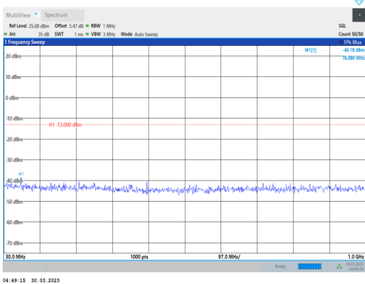
Band2-5MHz-16QAM-18625-1RB#0- Range1:30~1000MHz
