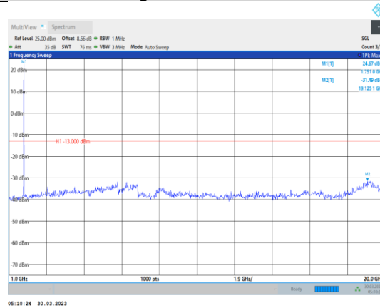
Band4-1.4MHz-16QAM-20393-1RB#0- Range2:1000~20000MHz
