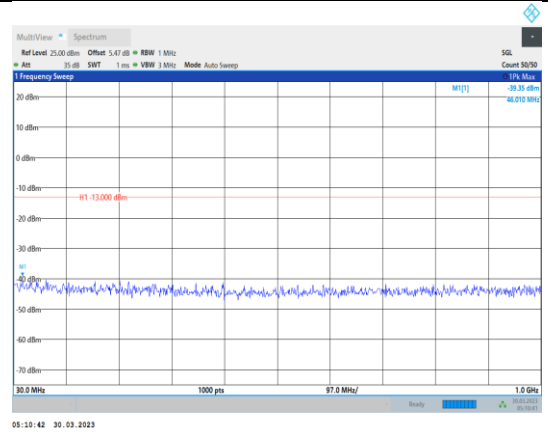
Band4-1.4MHz-64QAM-20393-1RB#0- Range1:30~1000MHz
