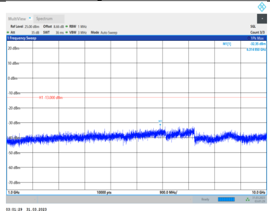
Band5-1.4MHz-QPSK-20643-1RB#0- Range2:1000~10000MHz
