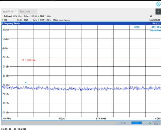
Band4-15MHz-16QAM-20175-1RB#0- Range1:30~1000MHz
