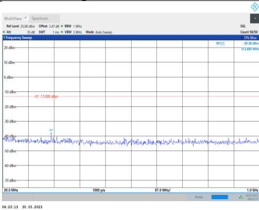
Band4-5MHz-64QAM-20175-1RB#0- Range1:30~1000MHz
