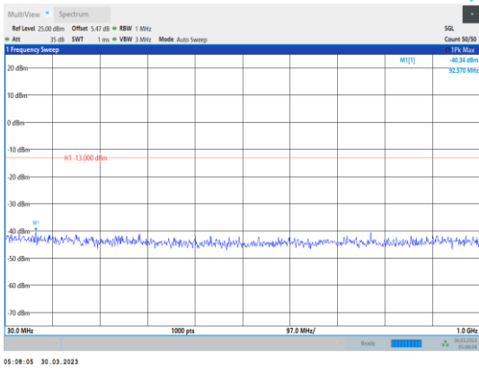
Band4-1.4MHz-64QAM-19957-1RB#0- Range1:30~1000MHz
