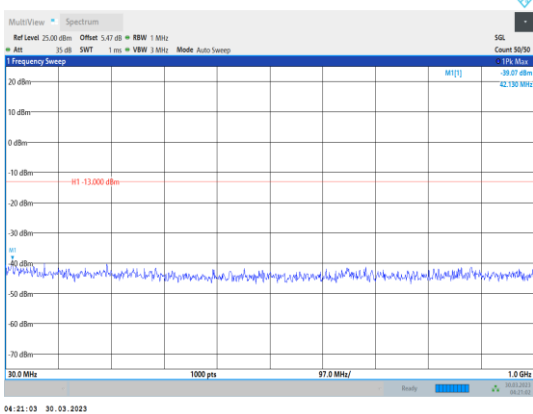
Band4-5MHz-QPSK-19975-1RB#0- Range1:30~1000MHz
