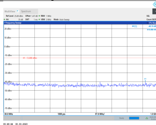
Band4-15MHz-16QAM-20325-1RB#0- Range1:30~1000MHz
