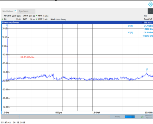
Band4-15MHz-64QAM-20025-1RB#0- Range2:1000~20000MHz
