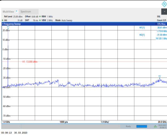
Band4-1.4MHz-64QAM-19957-1RB#0- Range2:1000~20000MHz
