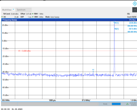
Band5-1.4MHz-QPSK-20525-1RB#0- Range1:30~1000MHz
