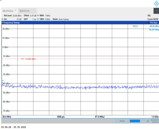
Band4-3MHz-QPSK-20175-1RB#0- Range1:30~1000MHz
