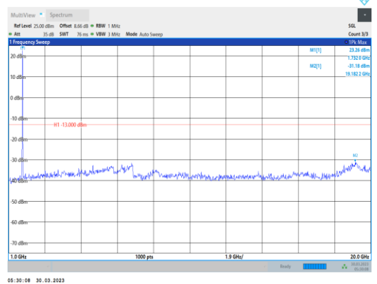
Band4-20MHz-16QAM-20175-1RB#0- Range2:1000~20000MHz
