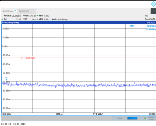
Band4-1.4MHz-64QAM-20175-1RB#0- Range1:30~1000MHz
