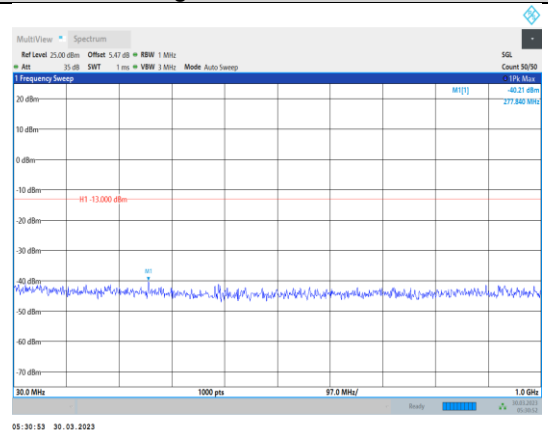
Band4-20MHz-QPSK-20300-1RB#0-Range1:30~1000MHz
