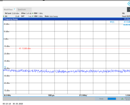
Band4-1.4MHz-16QAM-20393-1RB#0- Range1:30~1000MHz
