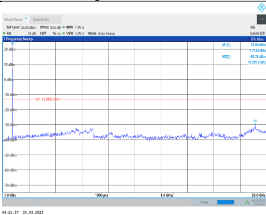
Band4-5MHz-16QAM-19975-1RB#0- Range2:1000~20000MHz
