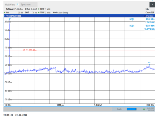
Band4-3MHz-64QAM-20175-1RB#0- Range2:1000~20000MHz
