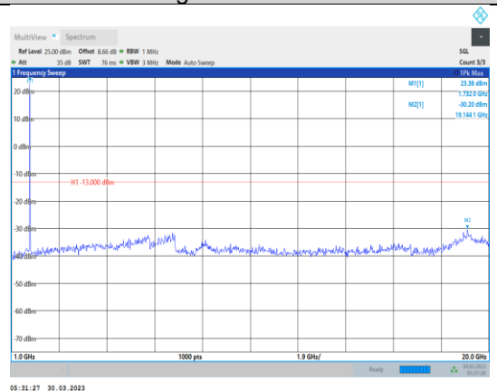
Band4-20MHz-16QAM-20300-1RB#0- Range2:1000~20000MHz
