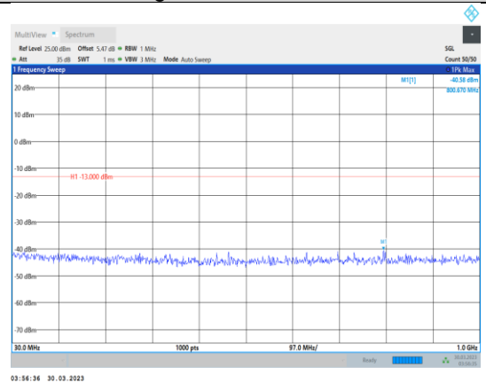
Band4-3MHz-64QAM-20385-1RB#0- Range1:30~1000MHz
