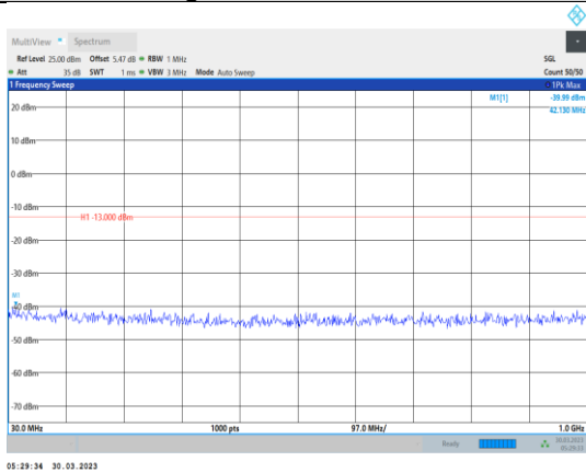
Band4-20MHz-QPSK-20175-1RB#0-Range1:30~1000MHz
