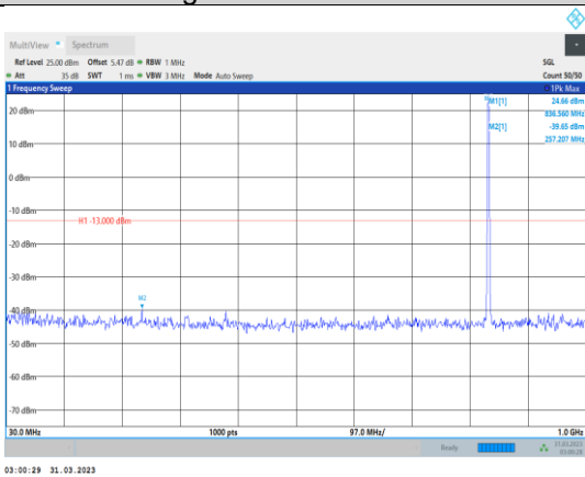
Band5-1.4MHz-16QAM-20525-1RB#0- Range1:30~1000MHz
