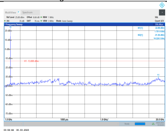
Band4-3MHz-64QAM-20385-1RB#0- Range2:1000~20000MHz
