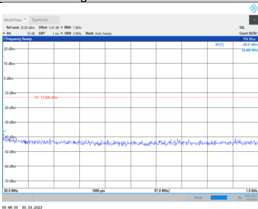
Band4-15MHz-QPSK-20175-1RB#0- Range1:30~1000MHz
