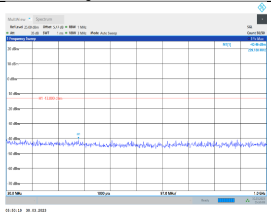
Band4-15MHz-64QAM-20325-1RB#0- Range1:30~1000MHz
