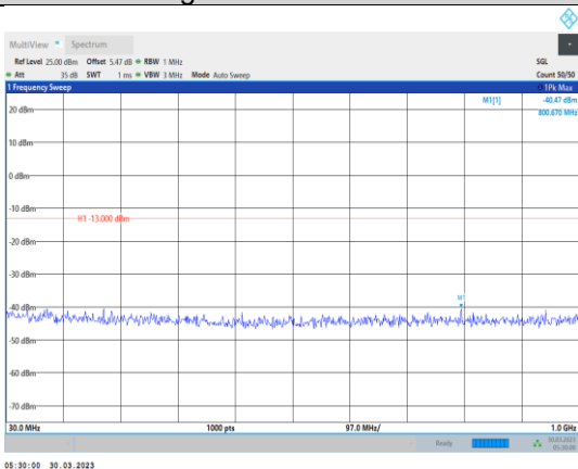
Band4-20MHz-16QAM-20175-1RB#0- Range1:30~1000MHz
