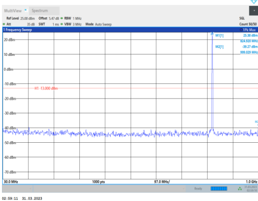
Band5-1.4MHz-16QAM-20407-1RB#0- Range1:30~1000MHz
