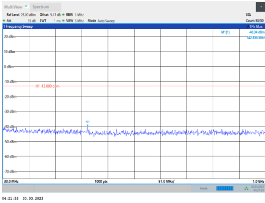
Band4-5MHz-64QAM-19975-1RB#0- Range1:30~1000MHz
