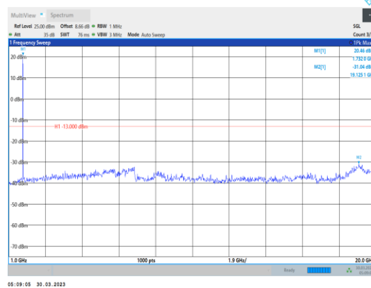
Band4-1.4MHz-16QAM-20175-1RB#0- Range2:1000~20000MHz
