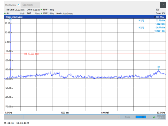
Band4-1.4MHz-64QAM-20175-1RB#0- Range2:1000~20000MHz
