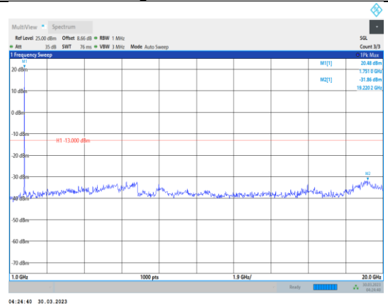
Band4-5MHz-64QAM-20375-1RB#0- Range2:1000~20000MHz
