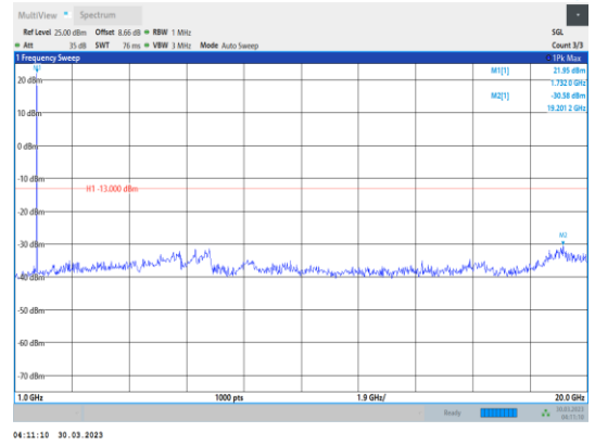
Band4-10MHz-16QAM-20175-1RB#0- Range2:1000~20000MHz
