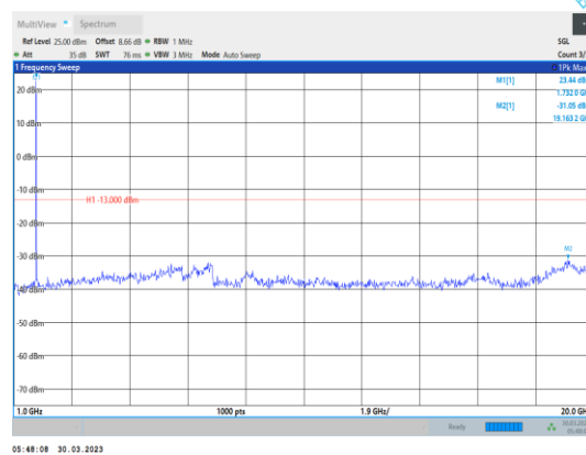
Band4-15MHz-QPSK-20175-1RB#0- Range2:1000~20000MHz
