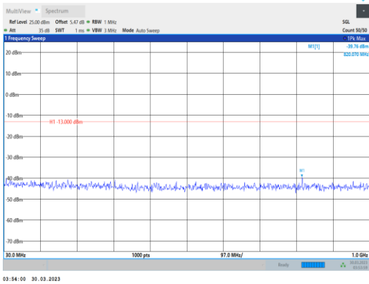
Band4-3MHz-64QAM-19965-1RB#0- Range1:30~1000MHz
