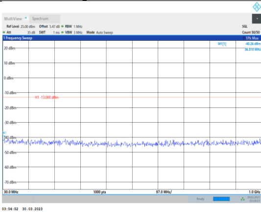
Band4-3MHz-16QAM-20175-1RB#0- Range1:30~1000MHz
