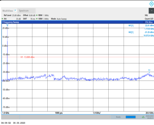
Band4-10MHz-16QAM-20000-1RB#0- Range2:1000~20000MHz
