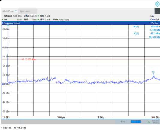
Band4-5MHz-64QAM-19975-1RB#0- Range2:1000~20000MHz
