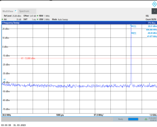
Band5-1.4MHz-64QAM-20525-1RB#0- Range1:30~1000MHz
