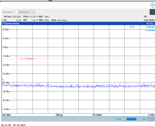
Band4-10MHz-64QAM-20175-1RB#0- Range1:30~1000MHz
