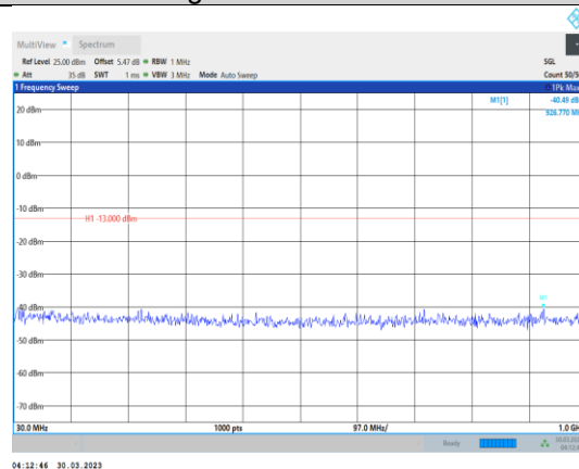
Band4-10MHz-64QAM-20350-1RB#0- Range1:30~1000MHz
