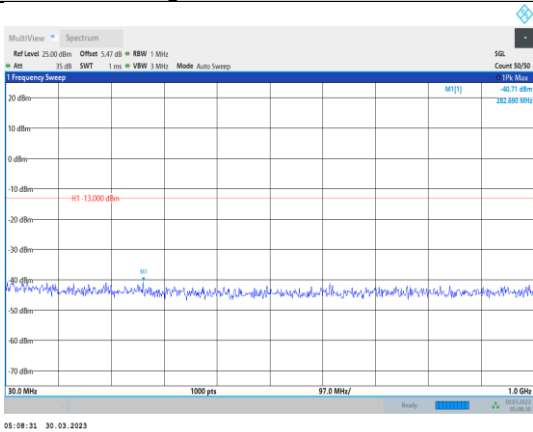
Band4-1.4MHz-QPSK-20175-1RB#0- Range1:30~1000MHz
