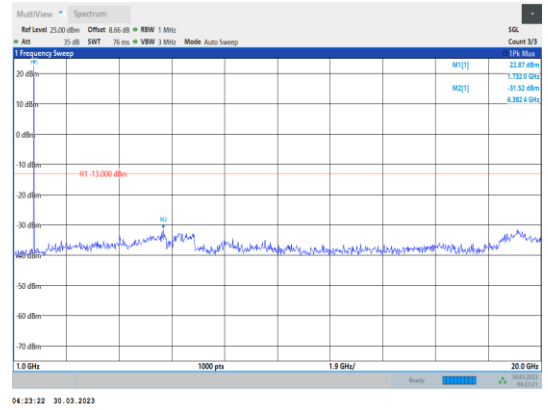
Band4-5MHz-64QAM-20175-1RB#0- Range2:1000~20000MHz
