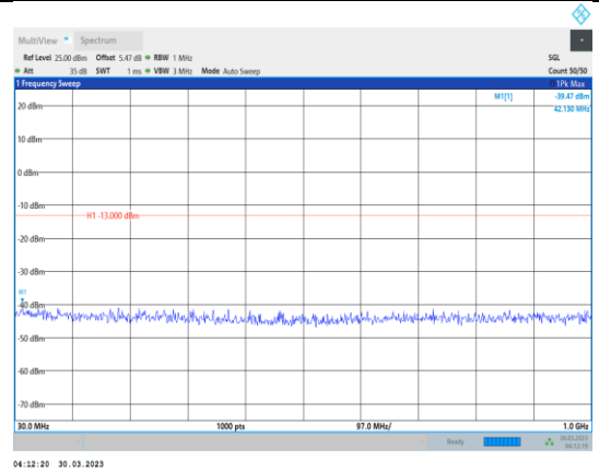
Band4-10MHz-16QAM-20350-1RB#0- Range1:30~1000MHz
