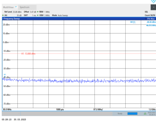
Band4-20MHz-QPSK-20050-1RB#0-Range1:30~1000MHz
