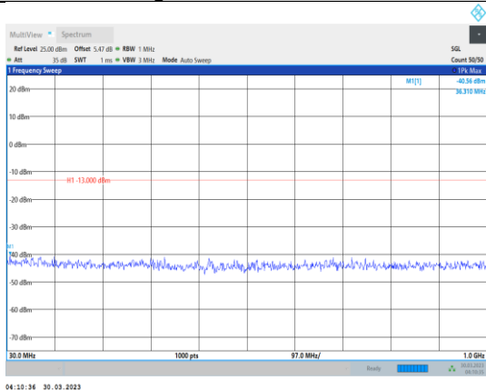
Band4-10MHz-QPSK-20175-1RB#0- Range1:30~1000MHz
