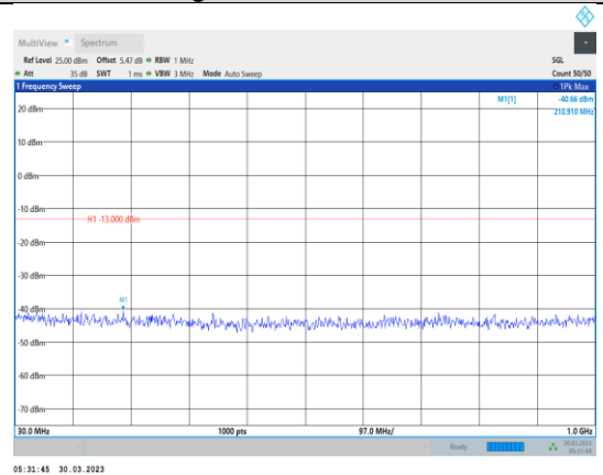
Band4-20MHz-64QAM-20300-1RB#0- Range1:30~1000MHz
