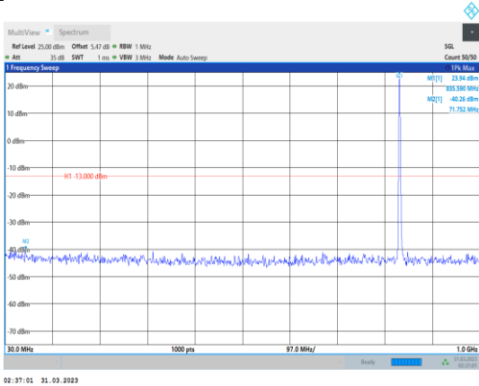
Band5-3MHz-QPSK-20525-1RB#0- Range1:30~1000MHz
