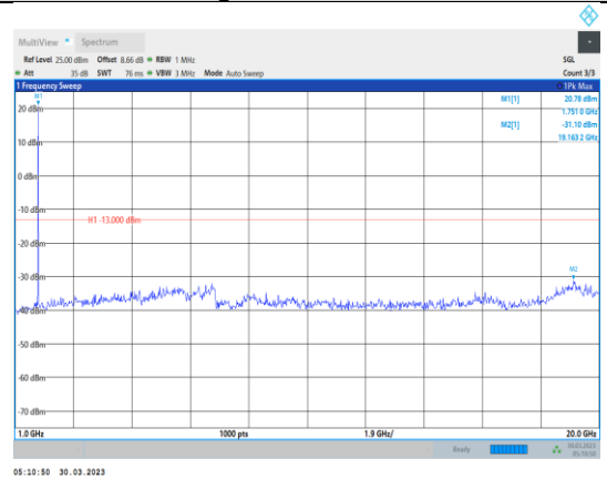
Band4-1.4MHz-64QAM-20393-1RB#0- Range2:1000~20000MHz
