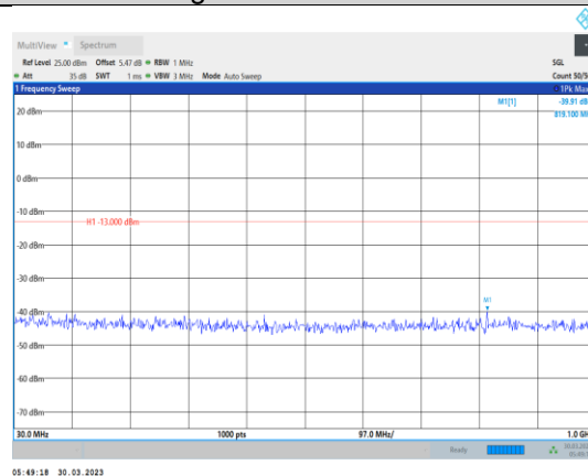
Band4-15MHz-QPSK-20325-1RB#0- Range1:30~1000MHz
