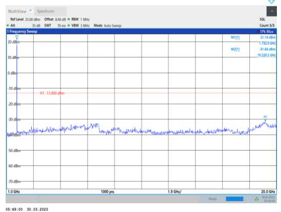
Band4-15MHz-64QAM-20175-1RB#0- Range2:1000~20000MHz
