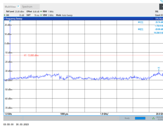
Band4-3MHz-16QAM-20175-1RB#0- Range2:1000~20000MHz
