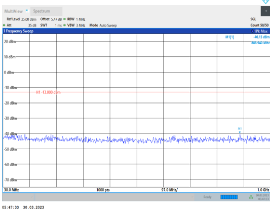
Band4-15MHz-64QAM-20025-1RB#0- Range1:30~1000MHz
