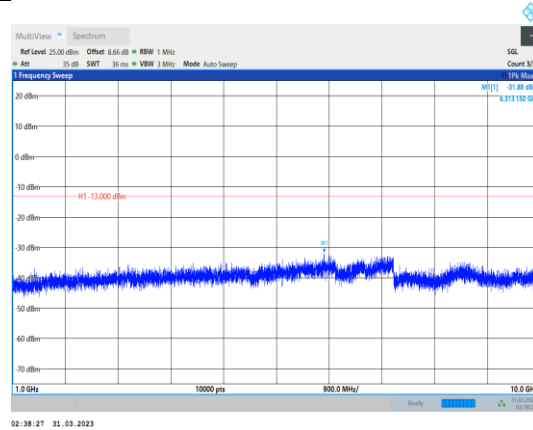
Band5-3MHz-QPSK-20635-1RB#0- Range2:1000~10000MHz
