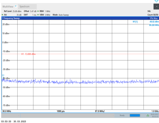
Band4-3MHz-16QAM-19965-1RB#0- Range1:30~1000MHz
