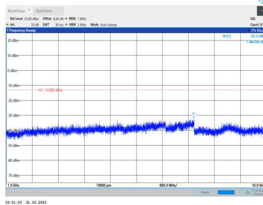
Band5-1.4MHz-64QAM-20525-1RB#0- Range2:1000~10000MHz
