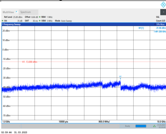
Band5-1.4MHz-64QAM-20407-1RB#0- Range2:1000~10000MHz
