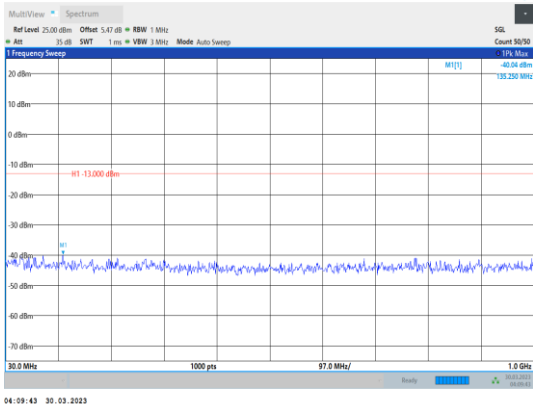
Band4-10MHz-16QAM-20000-1RB#0- Range1:30~1000MHz
