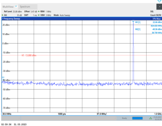
Band5-1.4MHz-64QAM-20407-1RB#0- Range1:30~1000MHz
