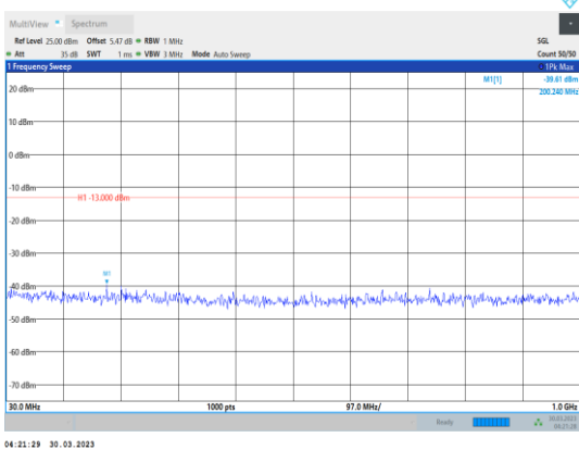
Band4-5MHz-16QAM-19975-1RB#0- Range1:30~1000MHz
