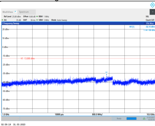
Band5-1.4MHz-16QAM-20407-1RB#0- Range2:1000~10000MHz
