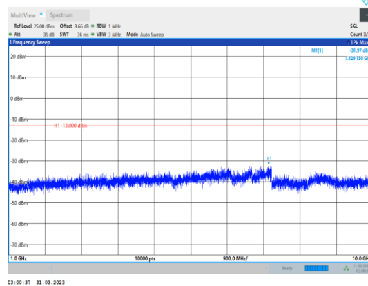
Band5-1.4MHz-16QAM-20525-1RB#0- Range2:1000~10000MHz
