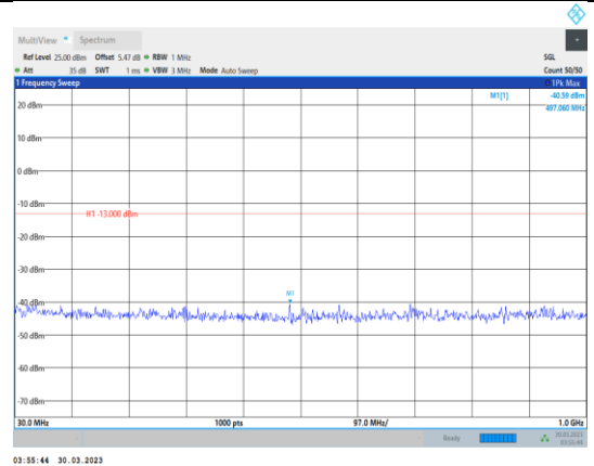
Band4-3MHz-QPSK-20385-1RB#0- Range1:30~1000MHz
