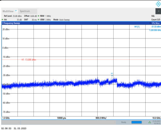
Band5-1.4MHz-QPSK-20407-1RB#0- Range2:1000~10000MHz
