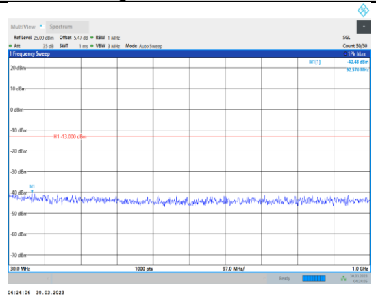
Band4-5MHz-16QAM-20375-1RB#0- Range1:30~1000MHz
