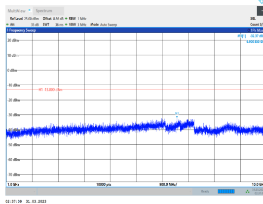
Band5-3MHz-QPSK-20525-1RB#0- Range2:1000~10000MHz
