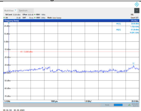
Band4-20MHz-64QAM-20300-1RB#0- Range2:1000~20000MHz
