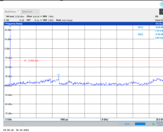
Band4-3MHz-16QAM-20385-1RB#0- Range2:1000~20000MHz
