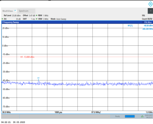
Band4-5MHz-QPSK-20175-1RB#0- Range1:30~1000MHz
