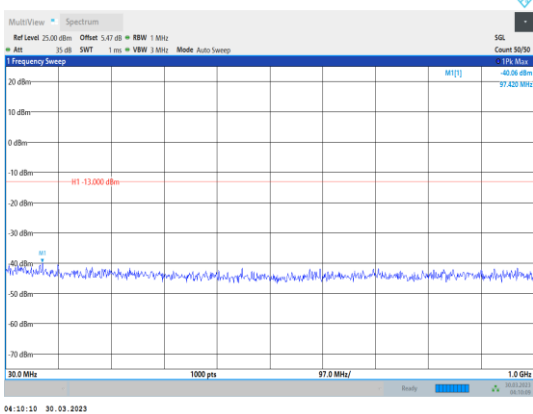
Band4-10MHz-64QAM-20000-1RB#0- Range1:30~1000MHz
