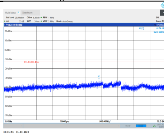
Band5-1.4MHz-16QAM-20643-1RB#0- Range2:1000~10000MHz
