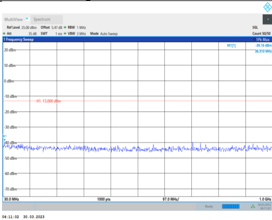
Band4-10MHz-16QAM-20175-1RB#0- Range1:30~1000MHz
