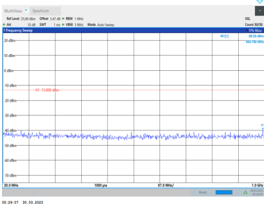
Band4-20MHz-64QAM-20050-1RB#0- Range1:30~1000MHz
