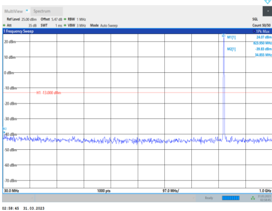
Band5-1.4MHz-QPSK-20407-1RB#0- Range1:30~1000MHz
