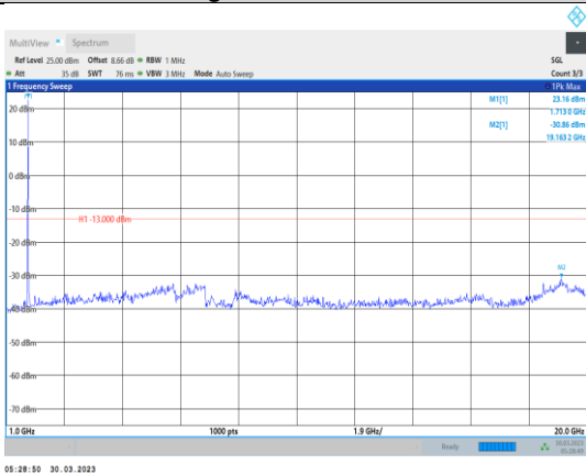
Band4-20MHz-16QAM-20050-1RB#0- Range2:1000~20000MHz
