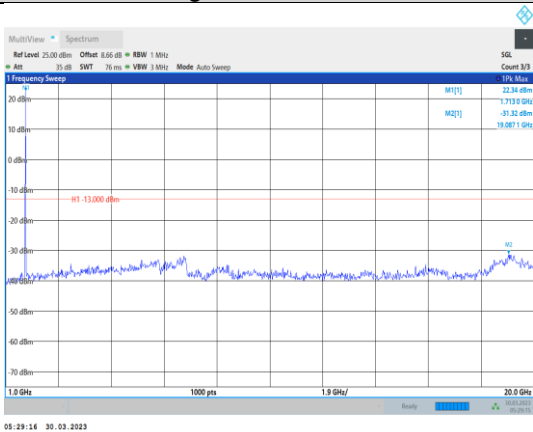
Band4-20MHz-64QAM-20050-1RB#0- Range2:1000~20000MHz
