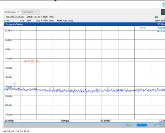
Band4-3MHz-16QAM-20385-1RB#0- Range1:30~1000MHz
