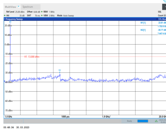
Band4-15MHz-16QAM-20175-1RB#0- Range2:1000~20000MHz
