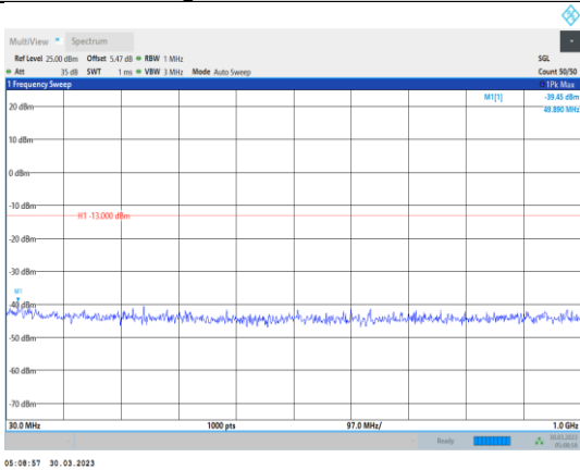
Band4-1.4MHz-16QAM-20175-1RB#0- Range1:30~1000MHz
