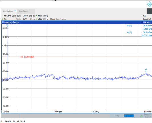
Band4-3MHz-64QAM-19965-1RB#0- Range2:1000~20000MHz
