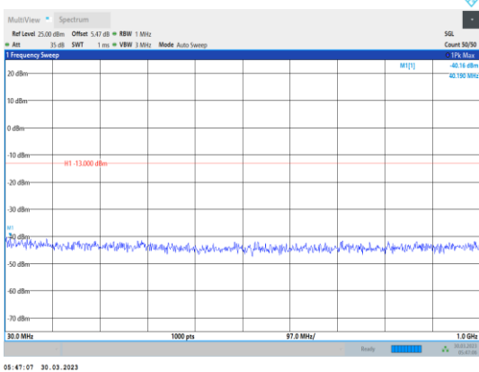
Band4-15MHz-16QAM-20025-1RB#0- Range1:30~1000MHz
