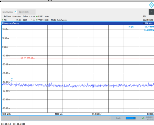
Band4-3MHz-64QAM-20175-1RB#0- Range1:30~1000MHz
