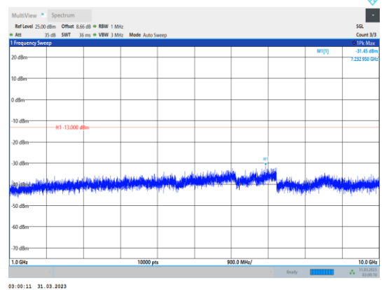
Band5-1.4MHz-QPSK-20525-1RB#0- Range2:1000~10000MHz
