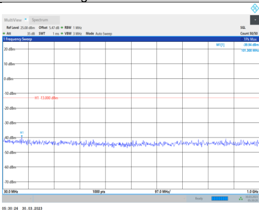
Band4-20MHz-64QAM-20175-1RB#0- Range1:30~1000MHz
