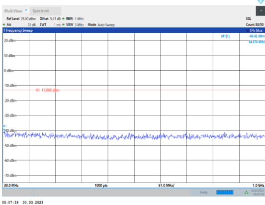
Band4-1.4MHz-16QAM-19957-1RB#0- Range1:30~1000MHz
