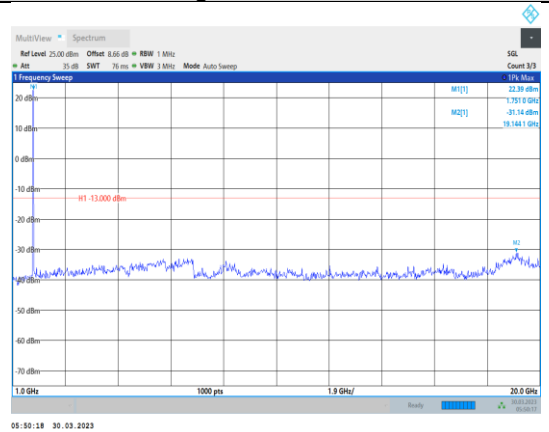
Band4-15MHz-64QAM-20325-1RB#0- Range2:1000~20000MHz
