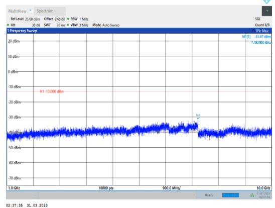
Band5-3MHz-16QAM-20525-1RB#0- Range2:1000~10000MHz
