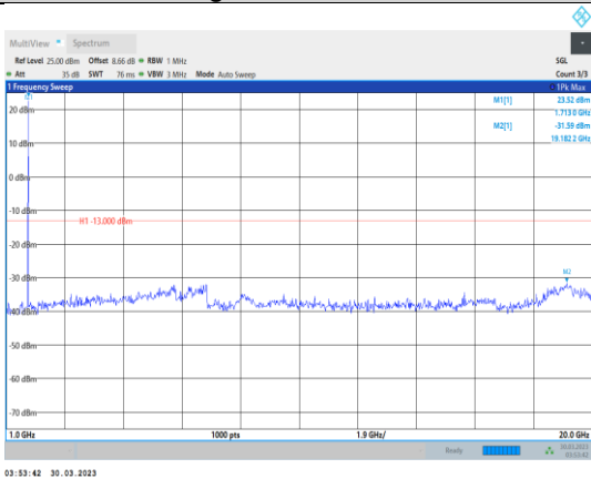
Band4-3MHz-16QAM-19965-1RB#0- Range2:1000~20000MHz
