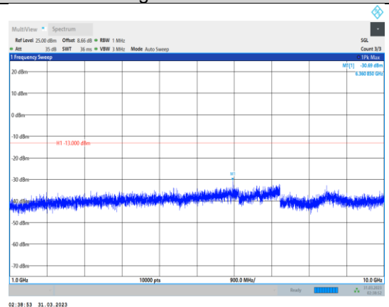
Band5-3MHz-16QAM-20635-1RB#0- Range2:1000~10000MHz
