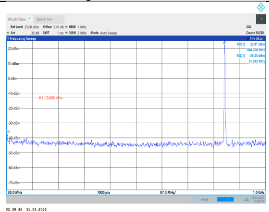
Band5-3MHz-16QAM-20635-1RB#0- Range1:30~1000MHz
