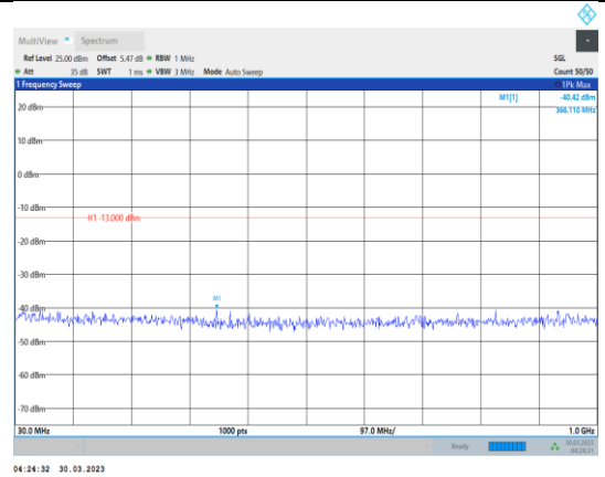
Band4-5MHz-64QAM-20375-1RB#0- Range1:30~1000MHz
