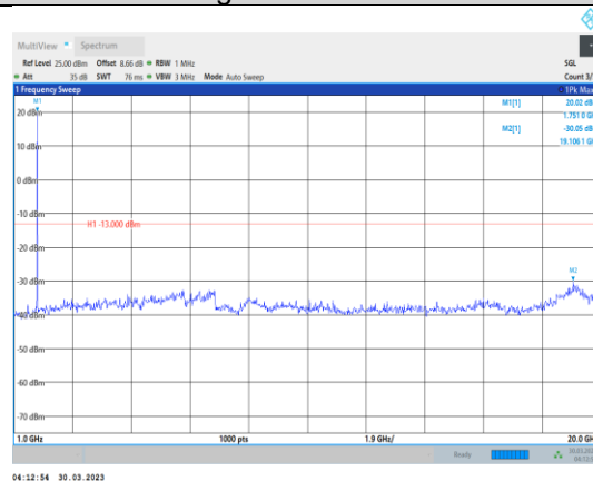
Band4-10MHz-64QAM-20350-1RB#0- Range2:1000~20000MHz
