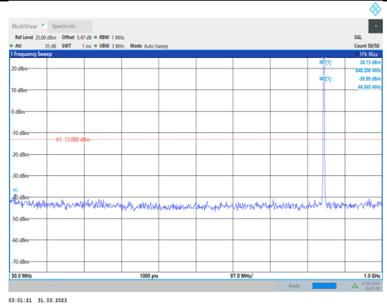
Band5-1.4MHz-QPSK-20643-1RB#0- Range1:30~1000MHz
