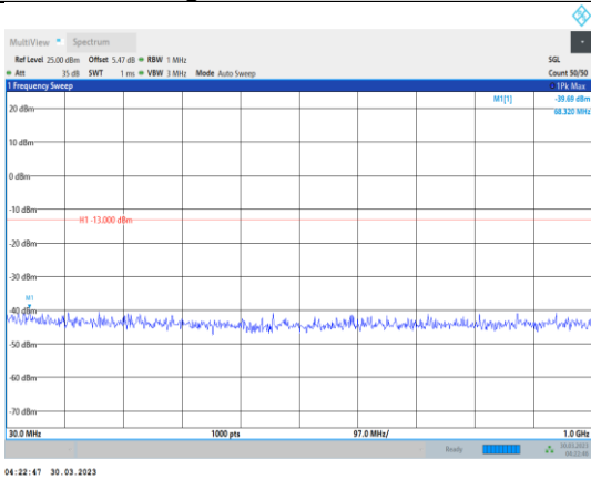
Band4-5MHz-16QAM-20175-1RB#0- Range1:30~1000MHz
