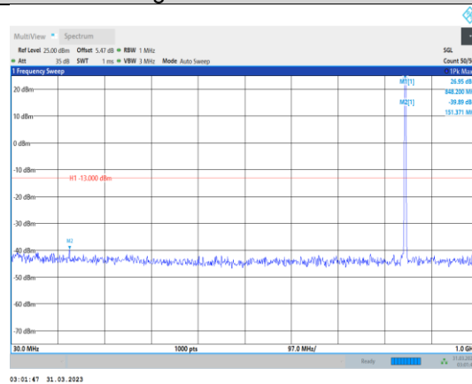
Band5-1.4MHz-16QAM-20643-1RB#0- Range1:30~1000MHz
