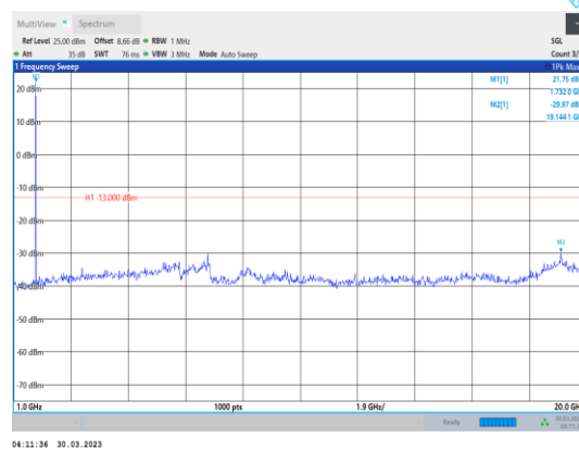
Band4-10MHz-64QAM-20175-1RB#0- Range2:1000~20000MHz
