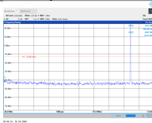
Band5-1.4MHz-64QAM-20643-1RB#0- Range1:30~1000MHz
