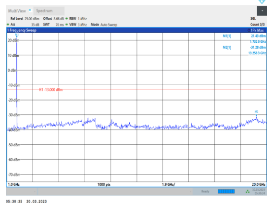
Band4-20MHz-64QAM-20175-1RB#0- Range2:1000~20000MHz
