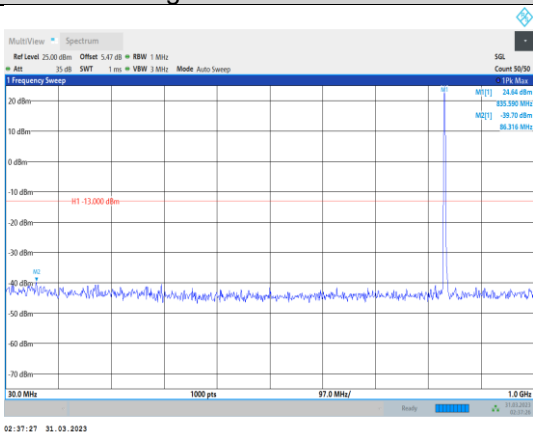
Band5-3MHz-16QAM-20525-1RB#0- Range1:30~1000MHz
