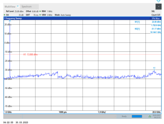
Band4-5MHz-16QAM-20175-1RB#0- Range2:1000~20000MHz
