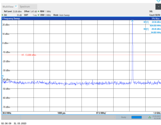
Band5-3MHz-16QAM-20415-1RB#0- Range1:30~1000MHz
