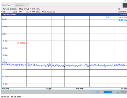
Band4-1.4MHz-QPSK-19957-1RB#0- Range1:30~1000MHz
