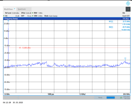
Band4-10MHz-16QAM-20350-1RB#0- Range2:1000~20000MHz
