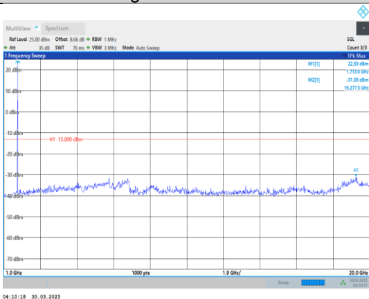
Band4-10MHz-64QAM-20000-1RB#0- Range2:1000~20000MHz
