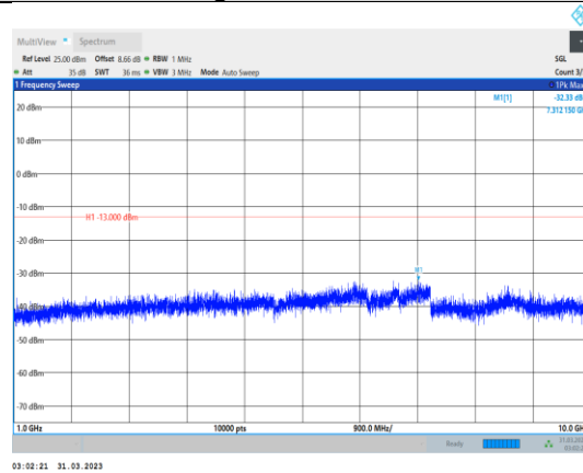
Band5-1.4MHz-64QAM-20643-1RB#0- Range2:1000~10000MHz
