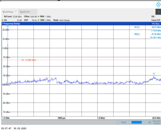
Band4-1.4MHz-16QAM-19957-1RB#0- Range2:1000~20000MHz
