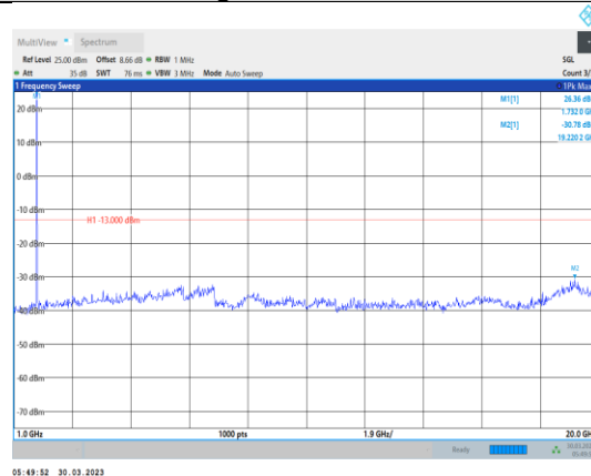
Band4-15MHz-16QAM-20325-1RB#0- Range2:1000~20000MHz
