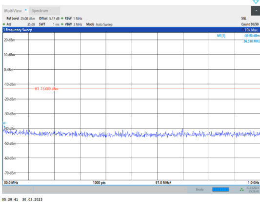
Band4-20MHz-16QAM-20050-1RB#0- Range1:30~1000MHz
