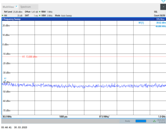
Band4-15MHz-QPSK-20025-1RB#0- Range1:30~1000MHz
