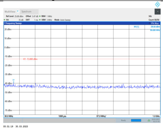
Band4-20MHz-16QAM-20300-1RB#0- Range1:30~1000MHz
