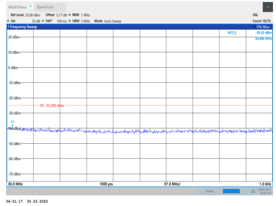
Band7-15MHz-64QAM-21100-1RB#0- Range1:30~1000MHz
