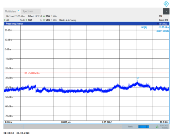
Band7-5MHz-16QAM-20775-1RB#0- Range3:3000~26500MHz
