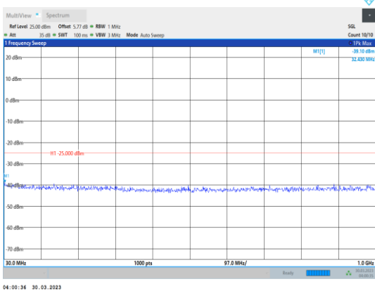
Band7-15MHz-16QAM-21100-1RB#0- Range1:30~1000MHz
