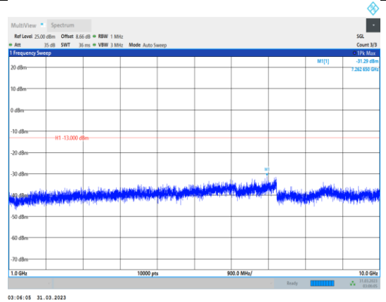
Band5-10MHz-QPSK-20600-1RB#0- Range2:1000~10000MHz
