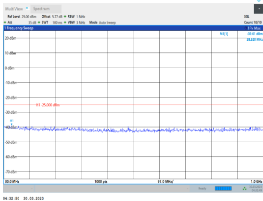
Band7-5MHz-QPSK-20775-1RB#0- Range1:30~1000MHz
