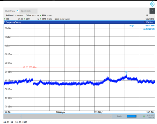
Band7-15MHz-64QAM-21100-1RB#0- Range3:3000~26500MHz
