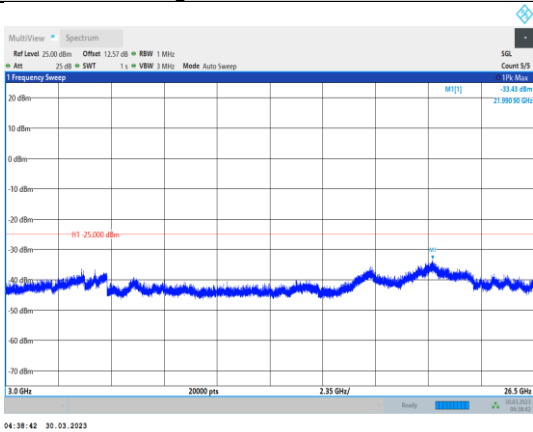
Band7-5MHz-64QAM-21425-1RB#0- Range3:3000~26500MHz
