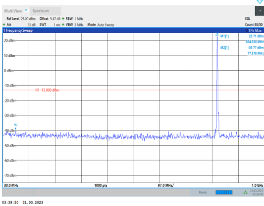
Band5-5MHz-64QAM-20425-1RB#0- Range1:30~1000MHz
