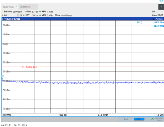
Band7-15MHz-QPSK-20825-1RB#0- Range1:30~1000MHz
