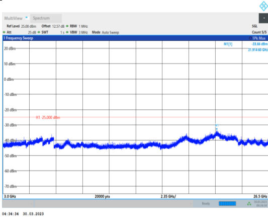
Band7-5MHz-64QAM-20775-1RB#0- Range3:3000~26500MHz
