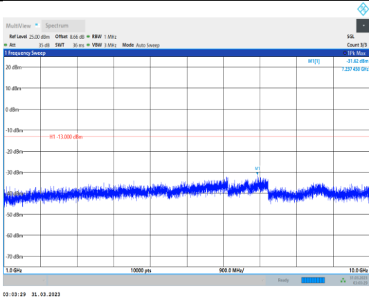
Band5-10MHz-QPSK-20450-1RB#0- Range2:1000~10000MHz
