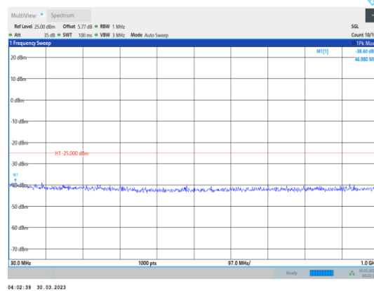
Band7-15MHz-16QAM-21375-1RB#0- Range1:30~1000MHz
