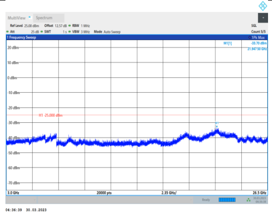
Band7-5MHz-64QAM-21100-1RB#0- Range3:3000~26500MHz
