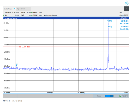
Band5-10MHz-16QAM-20600-1RB#0- Range1:30~1000MHz
