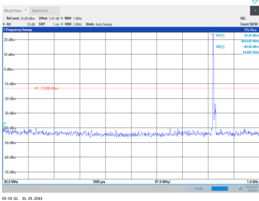
Band5-10MHz-QPSK-20450-1RB#0- Range1:30~1000MHz
