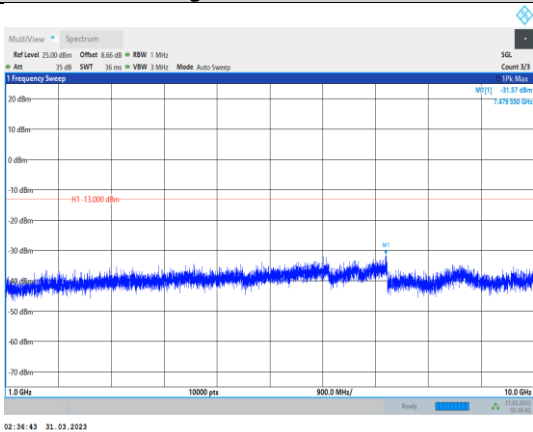
Band5-3MHz-64QAM-20415-1RB#0- Range2:1000~10000MHz
