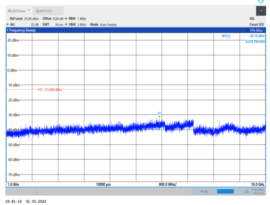
Band5-5MHz-64QAM-20525-1RB#0- Range2:1000~10000MHz
