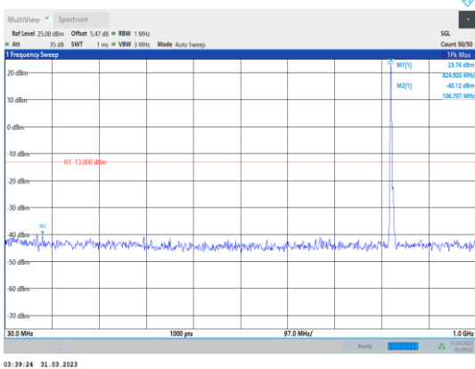
Band5-5MHz-16QAM-20425-1RB#0- Range1:30~1000MHz
