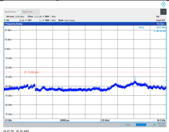
Band7-10MHz-64QAM-20800-1RB#0- Range3:3000~26500MHz
