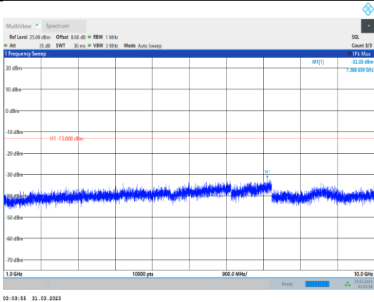
Band5-10MHz-16QAM-20450-1RB#0- Range2:1000~10000MHz
