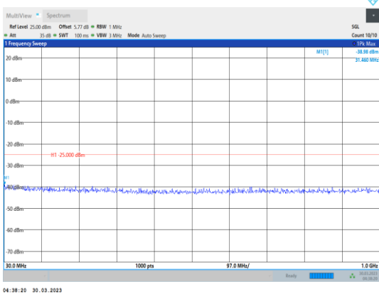
Band7-5MHz-64QAM-21425-1RB#0- Range1:30~1000MHz
