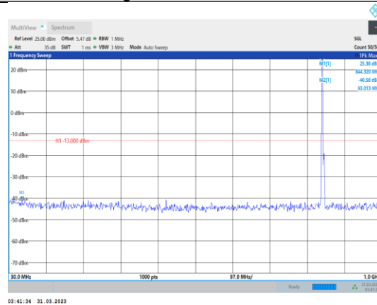
Band5-5MHz-QPSK-20625-1RB#0- Range1:30~1000MHz
