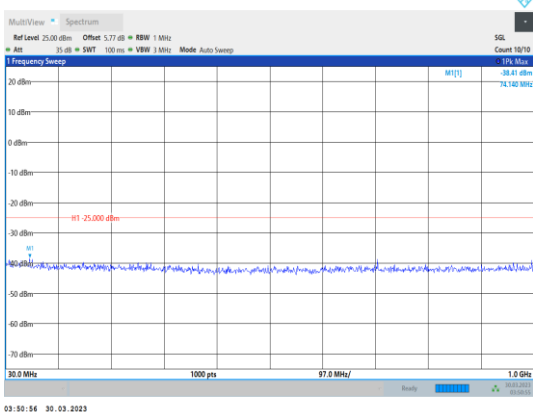
Band7-10MHz-16QAM-21400-1RB#0- Range1:30~1000MHz
