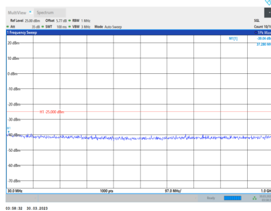
Band7-15MHz-16QAM-20825-1RB#0-Range1:30~1000MHz
