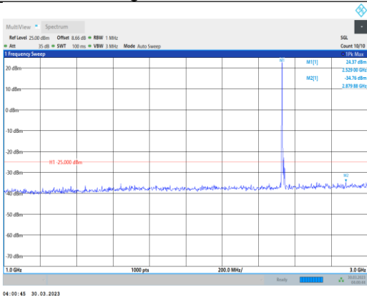
Band7-15MHz-16QAM-21100-1RB#0- Range2:1000~3000MHz
