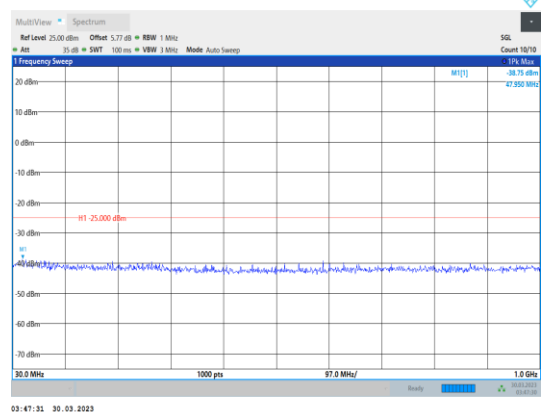
Band7-10MHz-64QAM-20800-1RB#0- Range1:30~1000MHz
