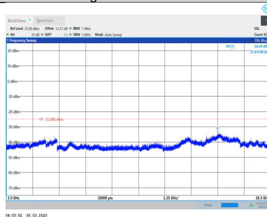
Band7-15MHz-16QAM-21375-1RB#0- Range3:3000~26500MHz
