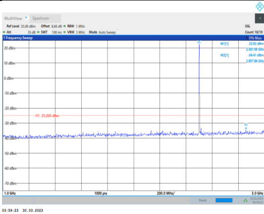
Band7-15MHz-64QAM-20825-1RB#0- Range2:1000~3000MHz
