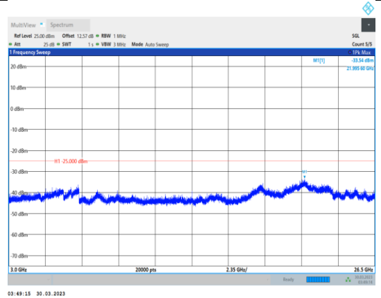
Band7-10MHz-16QAM-21100-1RB#0- Range3:3000~26500MHz
