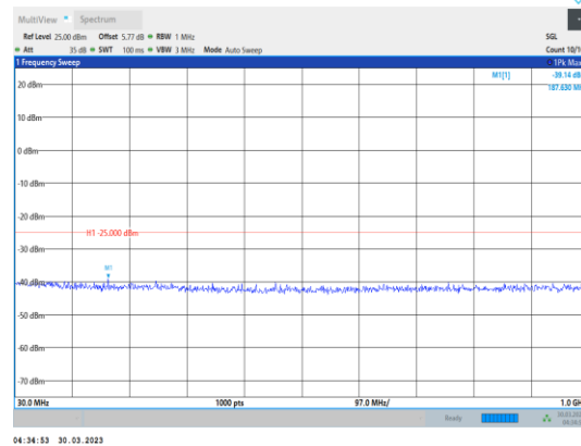
Band7-5MHz-QPSK-21100-1RB#0- Range1:30~1000MHz
