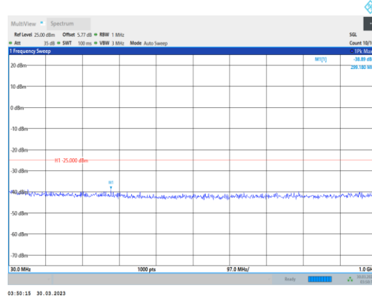
Band7-10MHz-QPSK-21400-1RB#0- Range1:30~1000MHz
