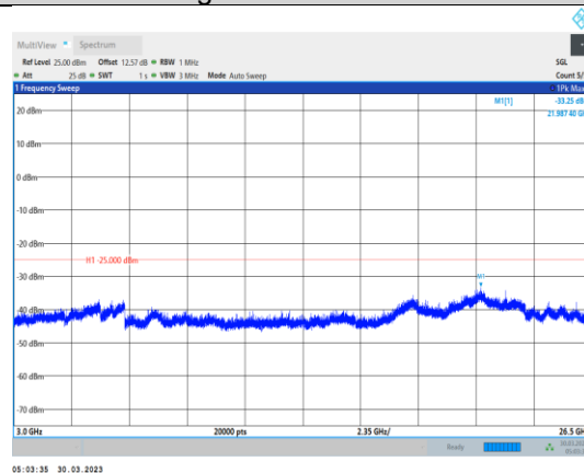
Band7-20MHz-16QAM-21100-1RB#0- Range3:3000~26500MHz
