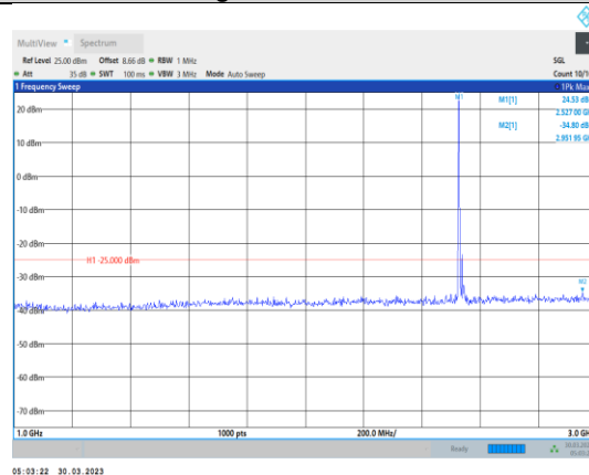
Band7-20MHz-16QAM-21100-1RB#0- Range2:1000~3000MHz
