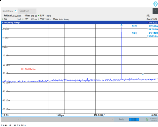
Band7-10MHz-64QAM-21100-1RB#0- Range2:1000~3000MHz
