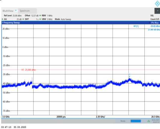
Band7-10MHz-16QAM-20800-1RB#0- Range3:3000~26500MHz
