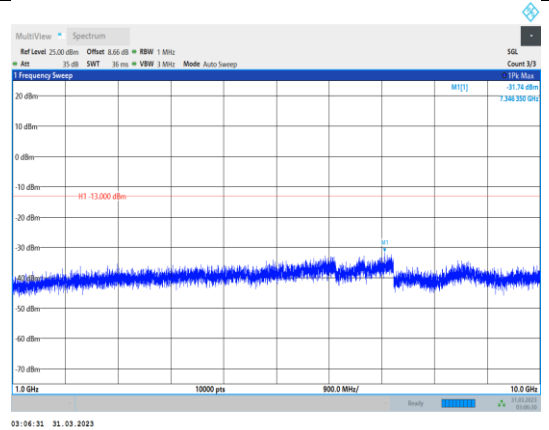
Band5-10MHz-16QAM-20600-1RB#0- Range2:1000~10000MHz
