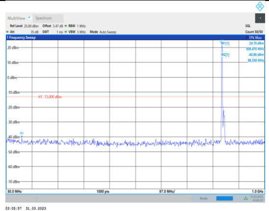
Band5-10MHz-QPSK-20600-1RB#0- Range1:30~1000MHz
