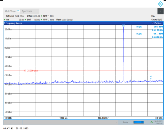
Band7-10MHz-64QAM-20800-1RB#0- Range2:1000~3000MHz
