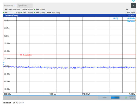
Band7-5MHz-64QAM-21100-1RB#0- Range1:30~1000MHz
