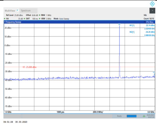
Band7-15MHz-64QAM-21100-1RB#0- Range2:1000~3000MHz
