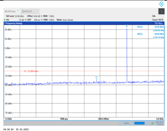
Band7-5MHz-64QAM-21100-1RB#0- Range2:1000~3000MHz
