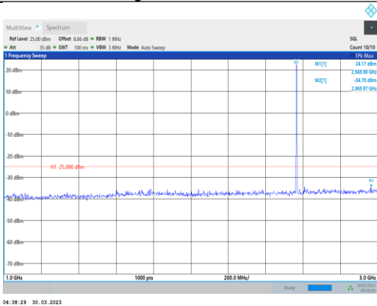
Band7-5MHz-64QAM-21425-1RB#0- Range2:1000~3000MHz
