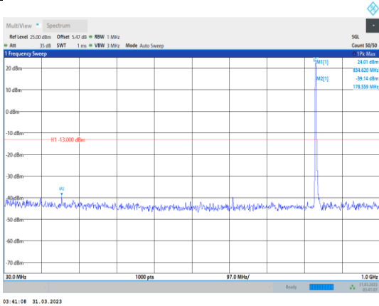
Band5-5MHz-64QAM-20525-1RB#0- Range1:30~1000MHz
