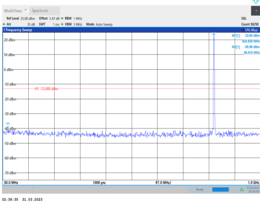
Band5-3MHz-64QAM-20415-1RB#0- Range1:30~1000MHz
