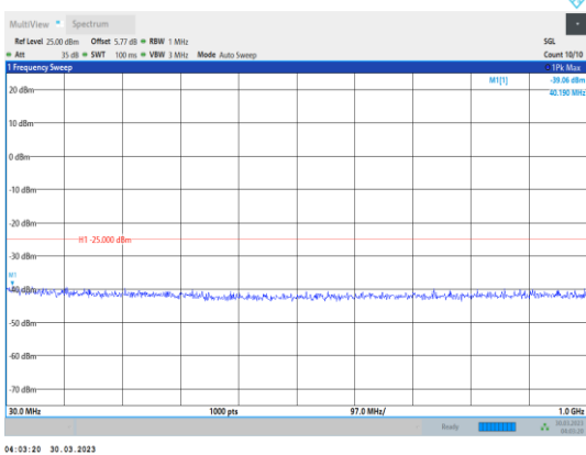
Band7-15MHz-64QAM-21375-1RB#0- Range1:30~1000MHz
