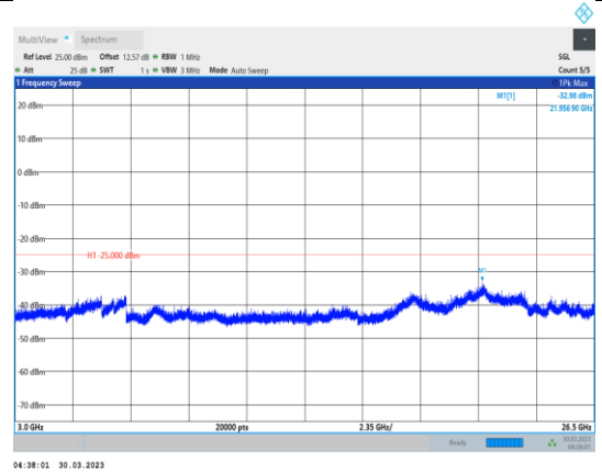
Band7-5MHz-16QAM-21425-1RB#0- Range3:3000~26500MHz
