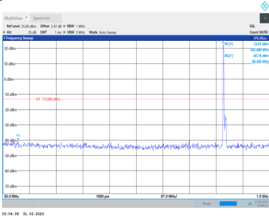
Band5-10MHz-QPSK-20525-1RB#0- Range1:30~1000MHz
