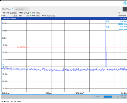
Band5-5MHz-QPSK-20525-1RB#0- Range1:30~1000MHz
