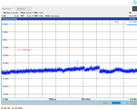
Band5-5MHz-64QAM-20425-1RB#0- Range2:1000~10000MHz
