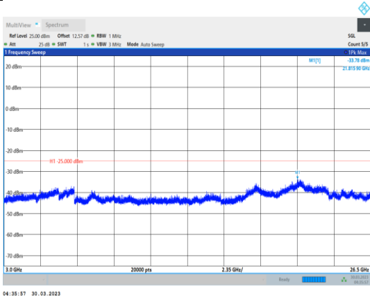
Band7-5MHz-16QAM-21100-1RB#0- Range3:3000~26500MHz
