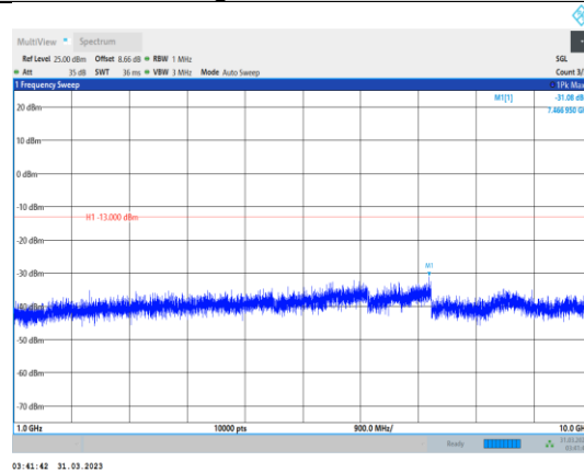
Band5-5MHz-QPSK-20625-1RB#0- Range2:1000~10000MHz
