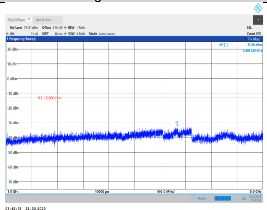
Band5-5MHz-16QAM-20625-1RB#0- Range2:1000~10000MHz
