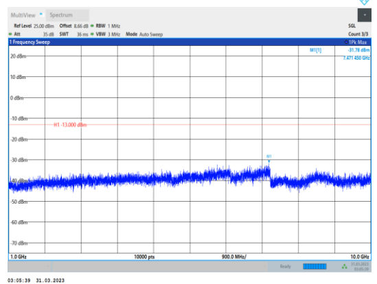
Band5-10MHz-64QAM-20525-1RB#0- Range2:1000~10000MHz
