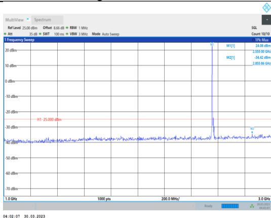
Band7-15MHz-QPSK-21375-1RB#0-Range2:1000~3000MHz
