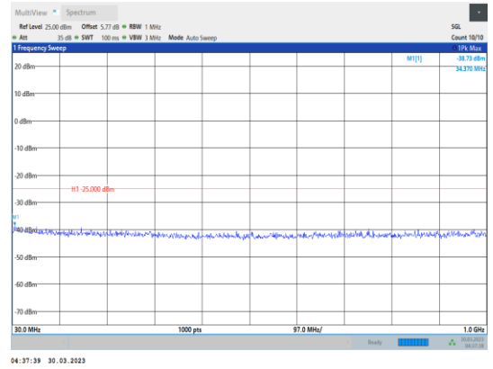
Band7-5MHz-16QAM-21425-1RB#0- Range1:30~1000MHz
