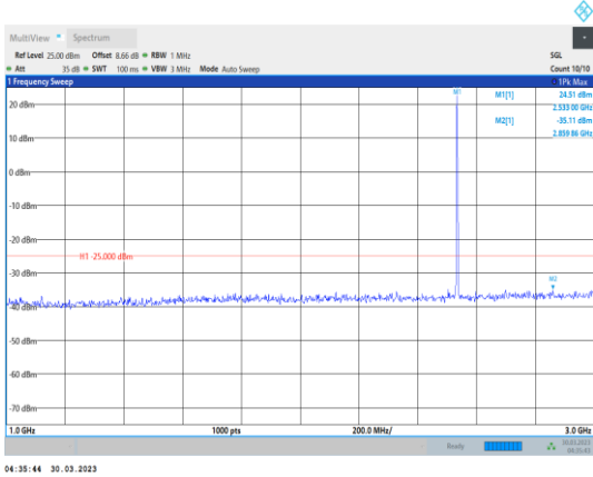
Band7-5MHz-16QAM-21100-1RB#0- Range2:1000~3000MHz
