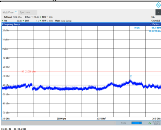
Band7-20MHz-16QAM-20850-1RB#0- Range3:3000~26500MHz
