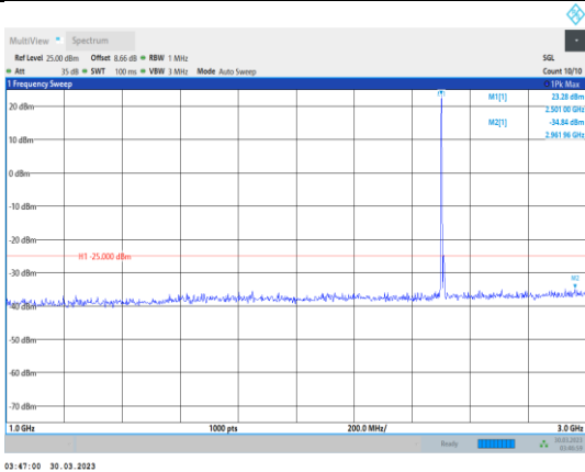
Band7-10MHz-16QAM-20800-1RB#0- Range2:1000~3000MHz
