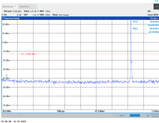
Band5-5MHz-QPSK-20425-1RB#0- Range1:30~1000MHz
