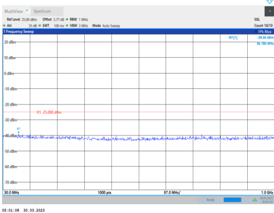
Band7-20MHz-16QAM-20850-1RB#0- Range1:30~1000MHz
