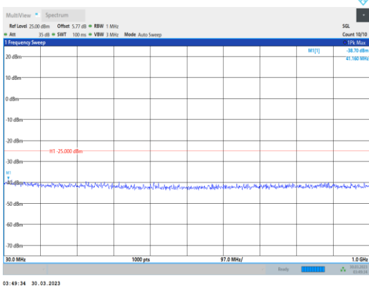
Band7-10MHz-64QAM-21100-1RB#0- Range1:30~1000MHz
