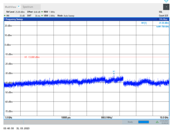
Band5-5MHz-16QAM-20525-1RB#0- Range2:1000~10000MHz
