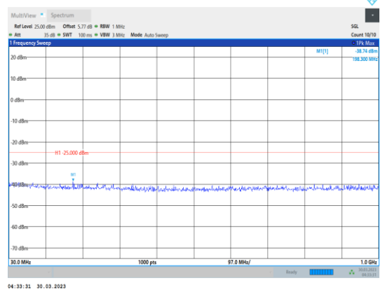
Band7-5MHz-16QAM-20775-1RB#0- Range1:30~1000MHz
