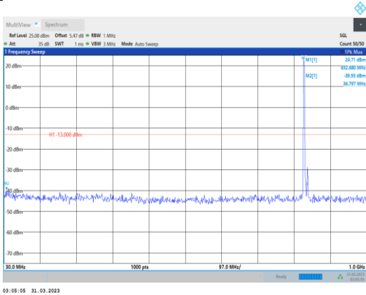
Band5-10MHz-16QAM-20525-1RB#0- Range1:30~1000MHz
