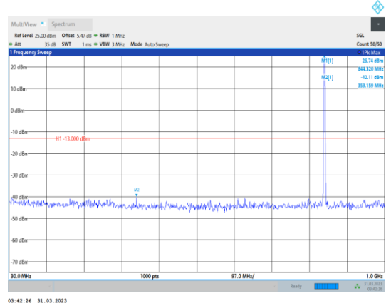
Band5-5MHz-64QAM-20625-1RB#0- Range1:30~1000MHz
