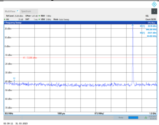
Band5-3MHz-64QAM-20635-1RB#0- Range1:30~1000MHz
