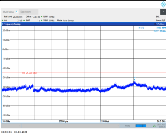
Band7-15MHz-64QAM-20825-1RB#0- Range3:3000~26500MHz
