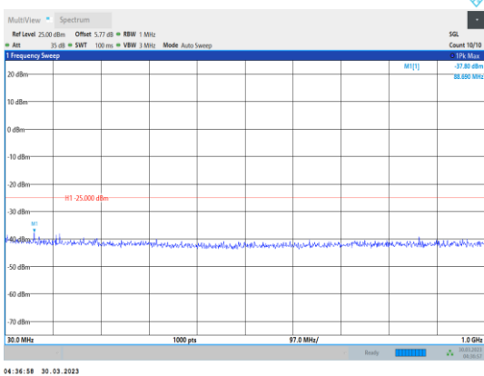
Band7-5MHz-QPSK-21425-1RB#0- Range1:30~1000MHz
