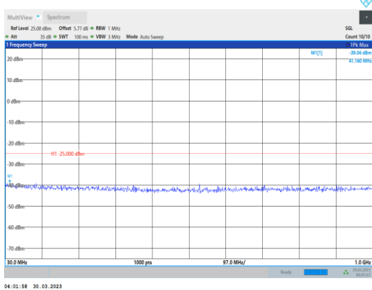
Band7-15MHz-QPSK-21375-1RB#0-Range1:30~1000MHz
