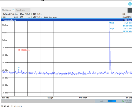
Band5-5MHz-16QAM-20525-1RB#0- Range1:30~1000MHz
