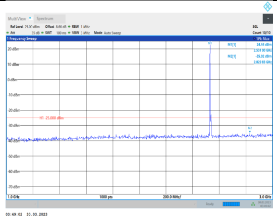
Band7-10MHz-16QAM-21100-1RB#0- Range2:1000~3000MHz
