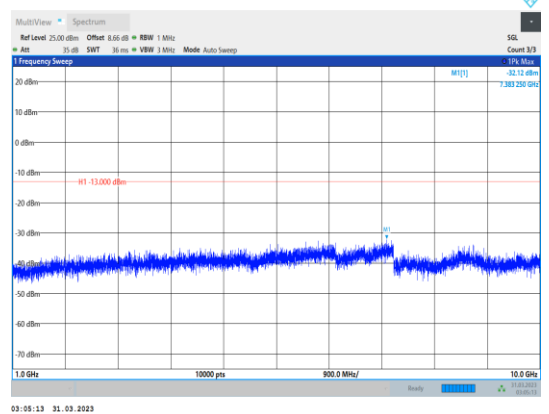
Band5-10MHz-16QAM-20525-1RB#0- Range2:1000~10000MHz
