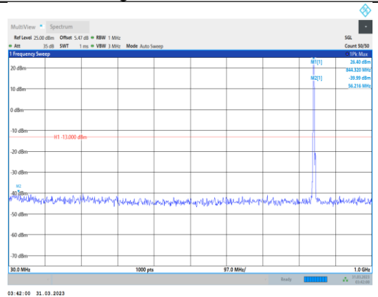
Band5-5MHz-16QAM-20625-1RB#0- Range1:30~1000MHz
