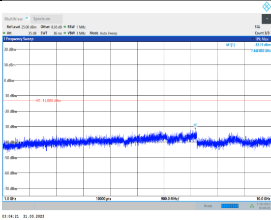
Band5-10MHz-64QAM-20450-1RB#0- Range2:1000~10000MHz
