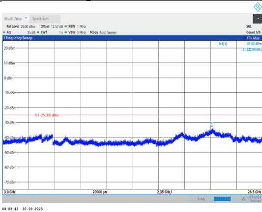
Band7-15MHz-64QAM-21375-1RB#0- Range3:3000~26500MHz
