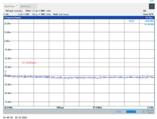
Band7-10MHz-16QAM-21100-1RB#0- Range1:30~1000MHz
