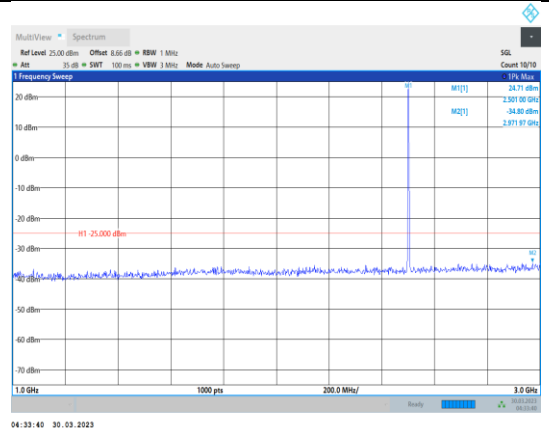
Band7-5MHz-16QAM-20775-1RB#0- Range2:1000~3000MHz
