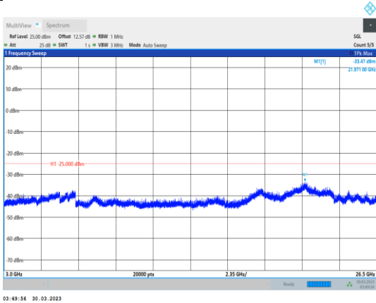
Band7-10MHz-64QAM-21100-1RB#0- Range3:3000~26500MHz
