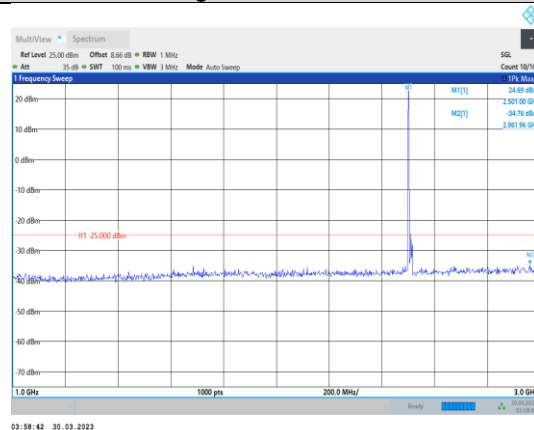
Band7-15MHz-16QAM-20825-1RB#0-Range2:1000~3000MHz
