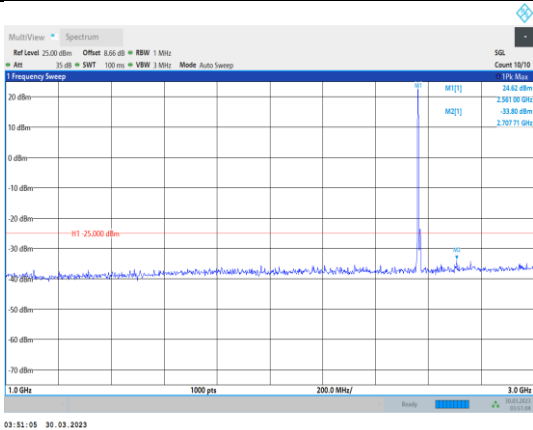
Band7-10MHz-16QAM-21400-1RB#0- Range2:1000~3000MHz
