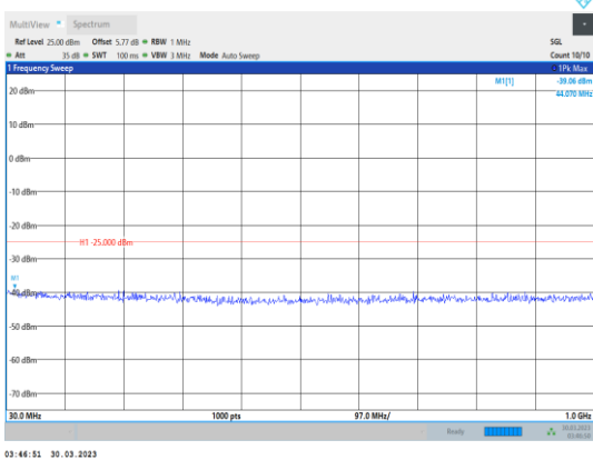
Band7-10MHz-16QAM-20800-1RB#0- Range1:30~1000MHz
