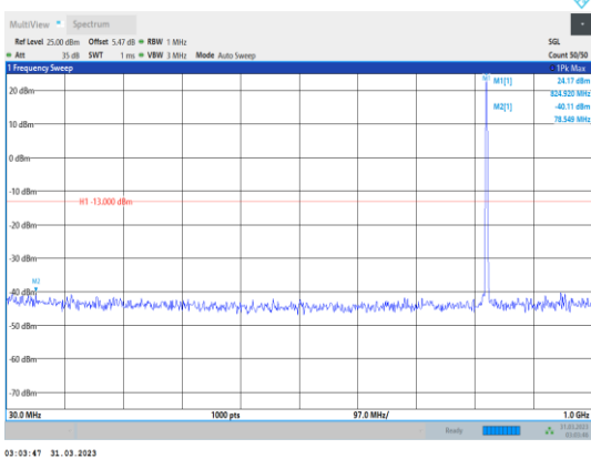
Band5-10MHz-16QAM-20450-1RB#0- Range1:30~1000MHz
