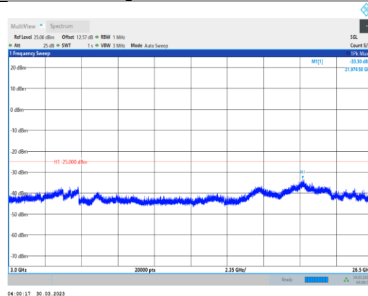
Band7-15MHz-QPSK-21100-1RB#0- Range3:3000~26500MHz
