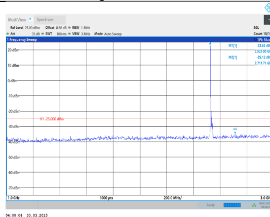
Band7-15MHz-QPSK-21100-1RB#0- Range2:1000~3000MHz
