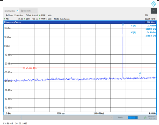
Band7-10MHz-64QAM-21400-1RB#0- Range2:1000~3000MHz
