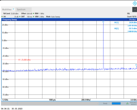
Band7-5MHz-64QAM-20775-1RB#0- Range2:1000~3000MHz
