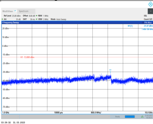
Band5-5MHz-16QAM-20425-1RB#0- Range2:1000~10000MHz
