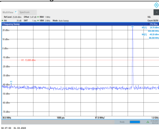
Band5-3MHz-64QAM-20525-1RB#0- Range1:30~1000MHz
