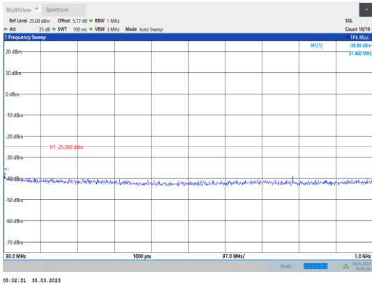
Band7-20MHz-QPSK-21100-1RB#0- Range1:30~1000MHz
