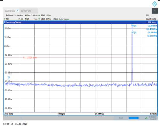
Band5-10MHz-64QAM-20600-1RB#0- Range1:30~1000MHz
