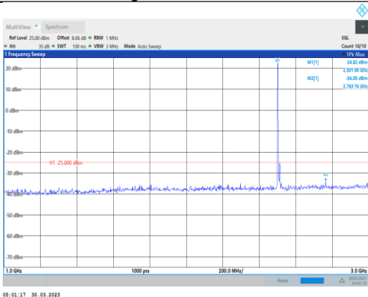
Band7-20MHz-16QAM-20850-1RB#0- Range2:1000~3000MHz
