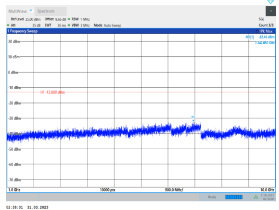
Band5-3MHz-64QAM-20525-1RB#0- Range2:1000~10000MHz
