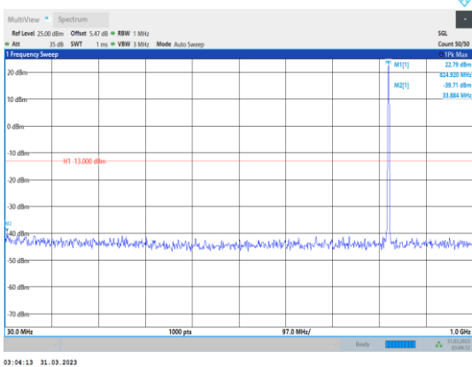
Band5-10MHz-64QAM-20450-1RB#0- Range1:30~1000MHz
