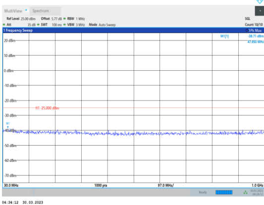
Band7-5MHz-64QAM-20775-1RB#0- Range1:30~1000MHz
