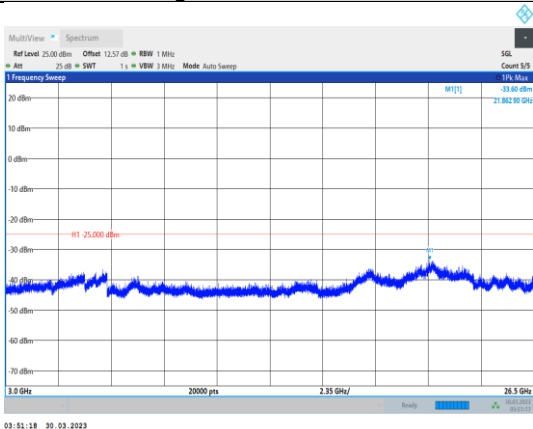
Band7-10MHz-16QAM-21400-1RB#0- Range3:3000~26500MHz
