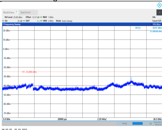
Band7-15MHz-QPSK-21375-1RB#0-Range3:3000~26500MHz
