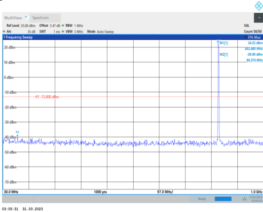
Band5-10MHz-64QAM-20525-1RB#0- Range1:30~1000MHz
