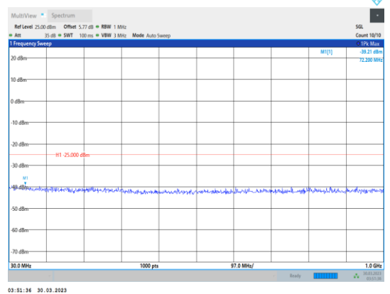
Band7-10MHz-64QAM-21400-1RB#0- Range1:30~1000MHz
