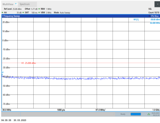
Band7-5MHz-16QAM-21100-1RB#0- Range1:30~1000MHz
