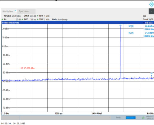
Band7-15MHz-64QAM-21375-1RB#0- Range2:1000~3000MHz
