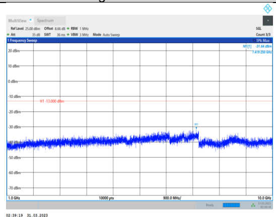
Band5-3MHz-64QAM-20635-1RB#0- Range2:1000~10000MHz
