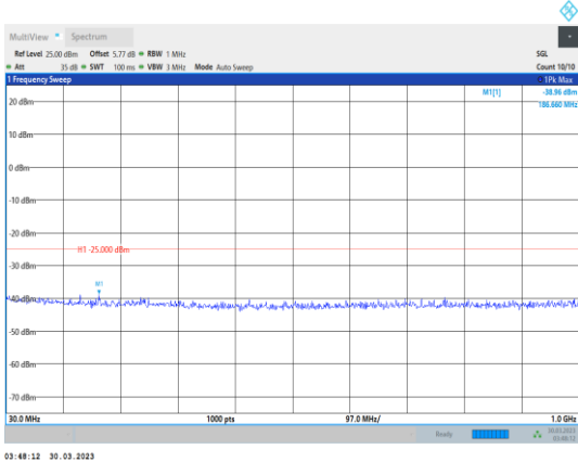
Band7-10MHz-QPSK-21100-1RB#0- Range1:30~1000MHz
