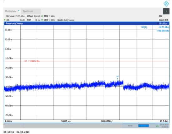
Band5-5MHz-64QAM-20625-1RB#0- Range2:1000~10000MHz
