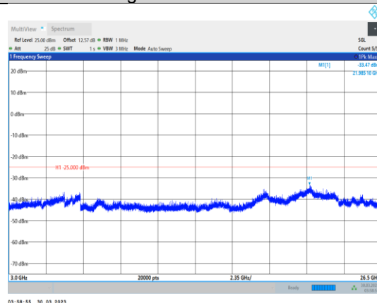
Band7-15MHz-16QAM-20825-1RB#0-Range3:3000~26500MHz
