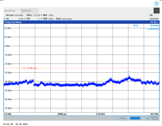
Band7-10MHz-64QAM-21400-1RB#0- Range3:3000~26500MHz
