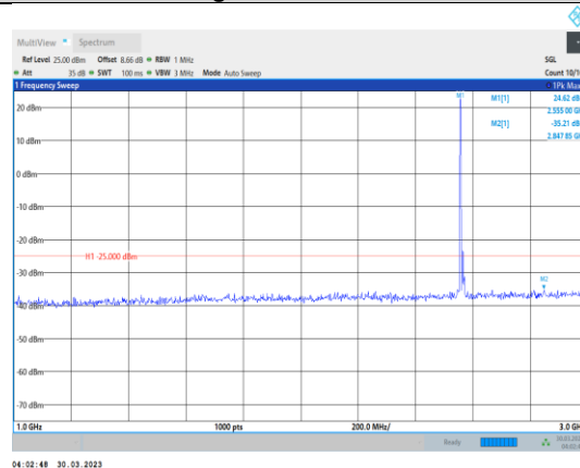
Band7-15MHz-16QAM-21375-1RB#0- Range2:1000~3000MHz
