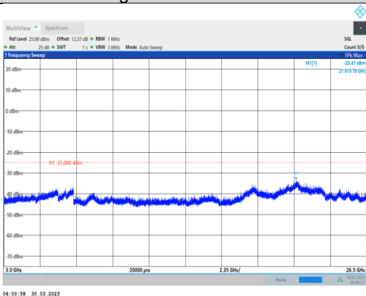
Band7-15MHz-16QAM-21100-1RB#0- Range3:3000~26500MHz
