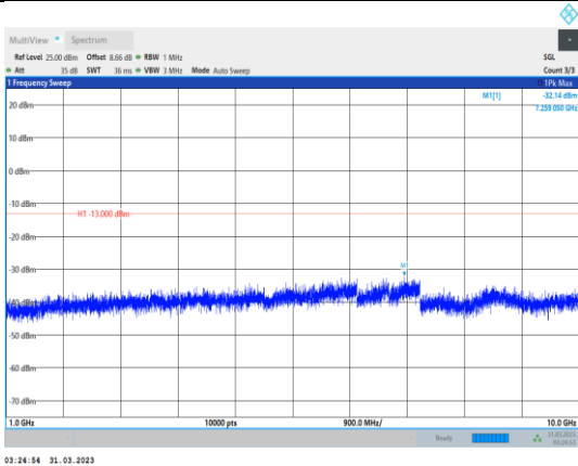
Band12-3MHz-16QAM-23025-1RB#0- Range2:1000~10000MHz
