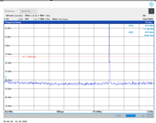
Band12-5MHz-QPSK-23155-1RB#0- Range1:30~1000MHz
