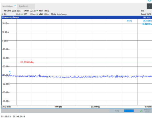
Band7-20MHz-64QAM-21100-1RB#0- Range1:30~1000MHz
