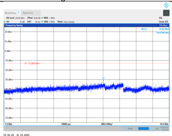
Band17-5MHz-QPSK-23825-1RB#0- Range2:1000~10000MHz
