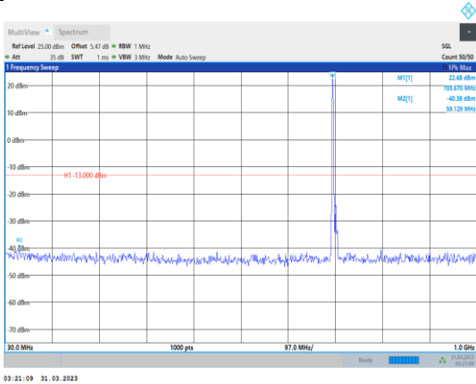
Band12-10MHz-QPSK-23095-1RB#0- Range1:30~1000MHz
