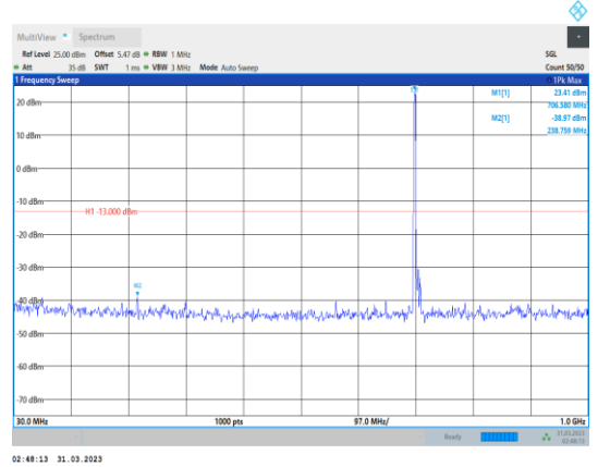
Band17-10MHz-16QAM-23800-1RB#0- Range1:30~1000MHz
