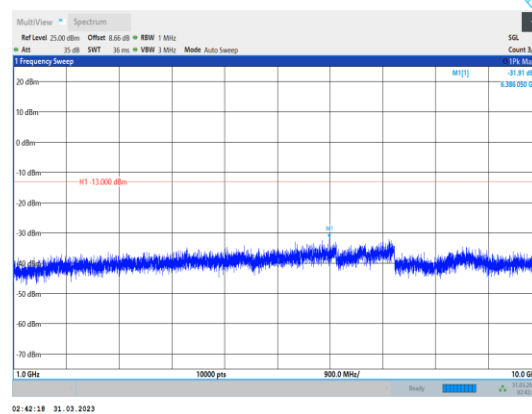
Band12-5MHz-16QAM-23095-1RB#0- Range2:1000~10000MHz
