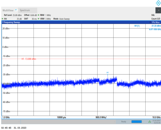
Band17-10MHz-16QAM-23780-1RB#0- Range2:1000~10000MHz
