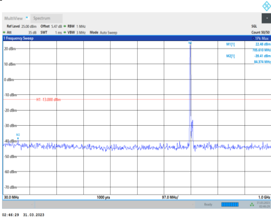
Band17-10MHz-QPSK-23790-1RB#0- Range1:30~1000MHz
