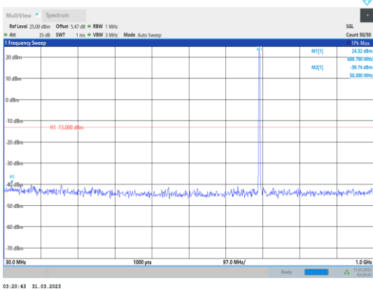
Band12-10MHz-64QAM-23060-1RB#0- Range1:30~1000MHz
