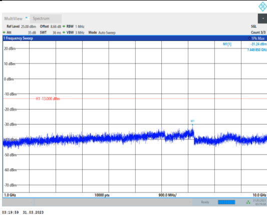
Band12-10MHz-QPSK-23060-1RB#0- Range2:1000~10000MHz
