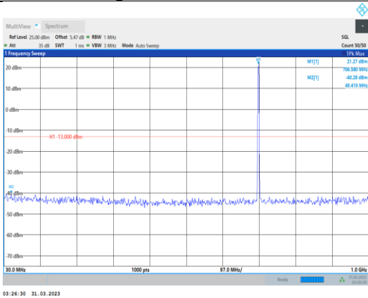
Band12-3MHz-64QAM-23095-1RB#0- Range1:30~1000MHz
