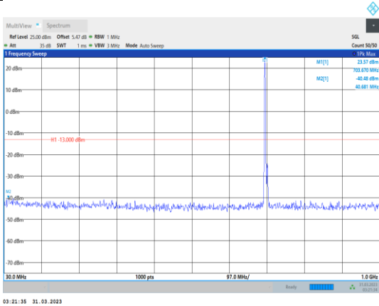
Band12-10MHz-16QAM-23095-1RB#0- Range1:30~1000MHz
