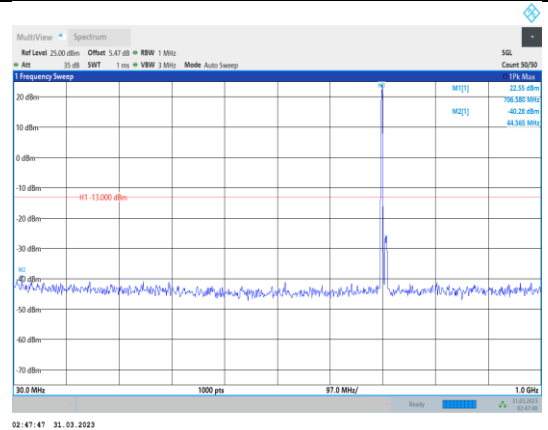
Band17-10MHz-QPSK-23800-1RB#0- Range1:30~1000MHz
