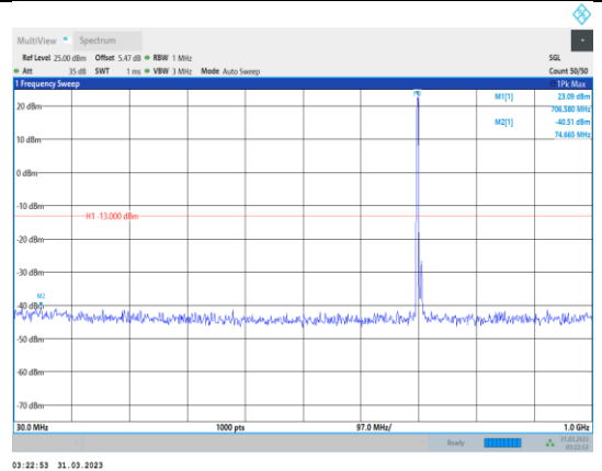
Band12-10MHz-16QAM-23130-1RB#0- Range1:30~1000MHz
