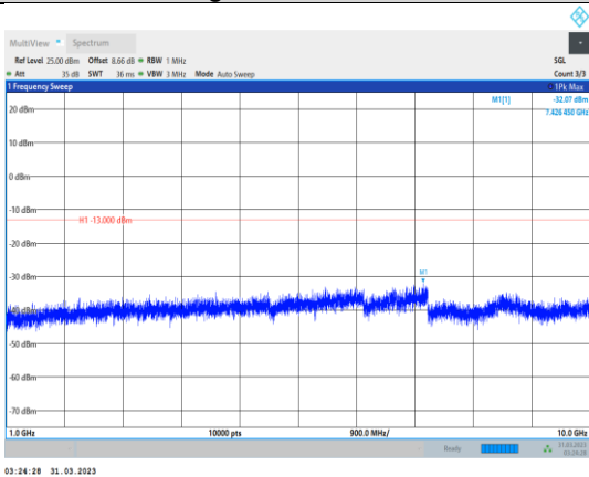
Band12-3MHz-QPSK-23025-1RB#0- Range2:1000~10000MHz
