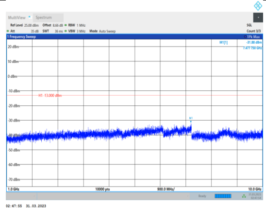
Band17-10MHz-QPSK-23800-1RB#0- Range2:1000~10000MHz
