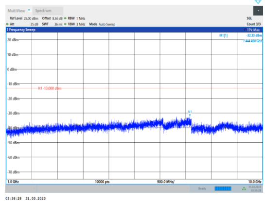
Band12-1.4MHz-64QAM-23095-1RB#0- Range2:1000~10000MHz
