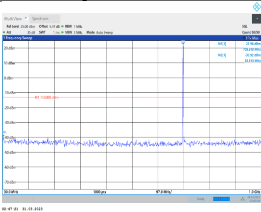
Band17-10MHz-64QAM-23790-1RB#0- Range1:30~1000MHz
