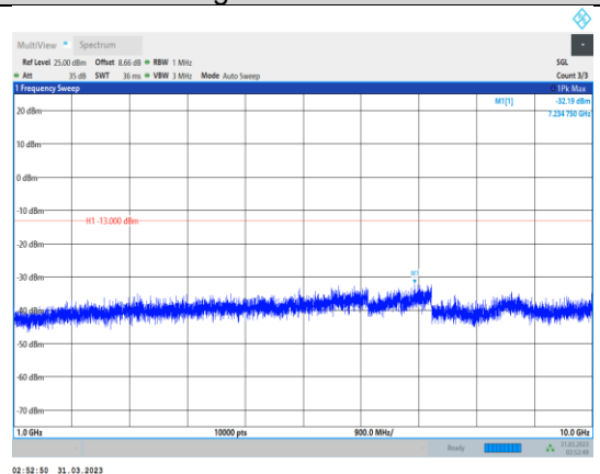
Band26-1.4MHz-16QAM-26783-1RB#0- Range2:1000~10000MHz
