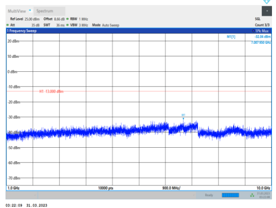
Band12-10MHz-64QAM-23095-1RB#0- Range2:1000~10000MHz
