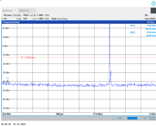
Band17-10MHz-16QAM-23790-1RB#0- Range1:30~1000MHz
