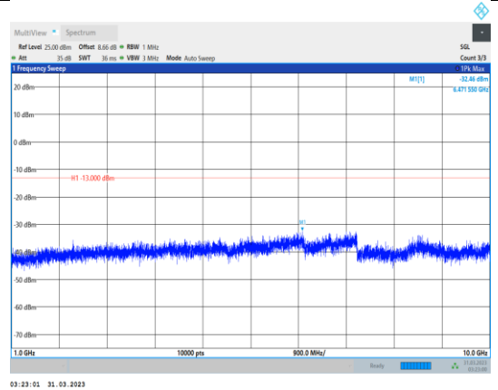
Band12-10MHz-16QAM-23130-1RB#0- Range2:1000~10000MHz
