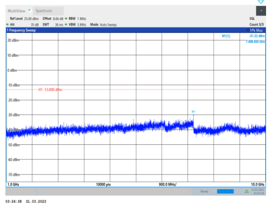
Band12-3MHz-64QAM-23095-1RB#0- Range2:1000~10000MHz
