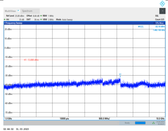
Band12-5MHz-64QAM-23155-1RB#0- Range2:1000~10000MHz
