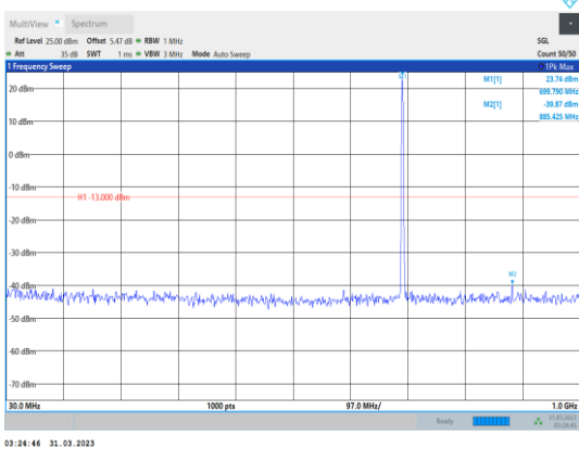
Band12-3MHz-16QAM-23025-1RB#0- Range1:30~1000MHz
