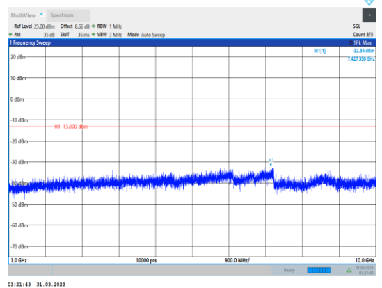
Band12-10MHz-16QAM-23095-1RB#0- Range2:1000~10000MHz
