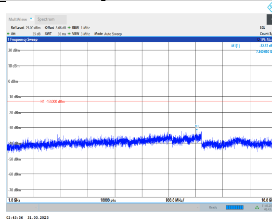
Band12-5MHz-16QAM-23155-1RB#0- Range2:1000~10000MHz
