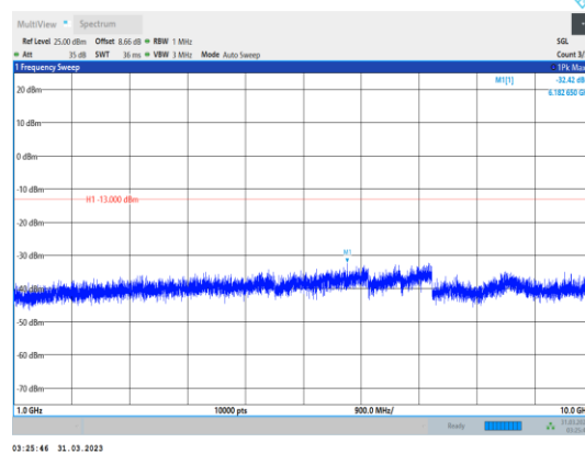
Band12-3MHz-QPSK-23095-1RB#0- Range2:1000~10000MHz
