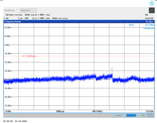
Band12-1.4MHz-QPSK-23173-1RB#0- Range2:1000~10000MHz
