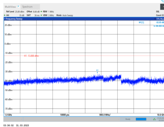
Band12-1.4MHz-16QAM-23095-1RB#0- Range2:1000~10000MHz
