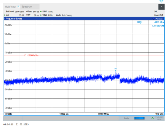
Band12-3MHz-16QAM-23095-1RB#0- Range2:1000~10000MHz
