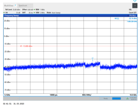
Band12-5MHz-QPSK-23095-1RB#0- Range2:1000~10000MHz
