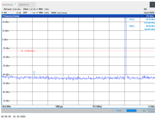
Band26-1.4MHz-16QAM-26697-1RB#0- Range1:30~1000MHz
