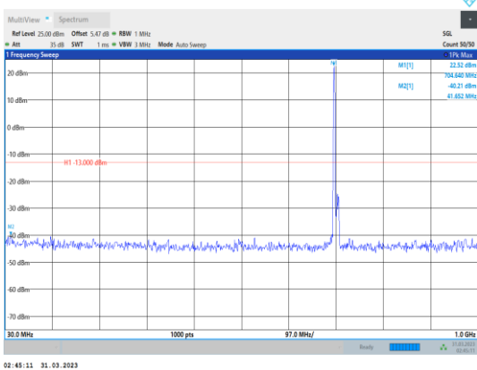
Band17-10MHz-QPSK-23780-1RB#0- Range1:30~1000MHz
