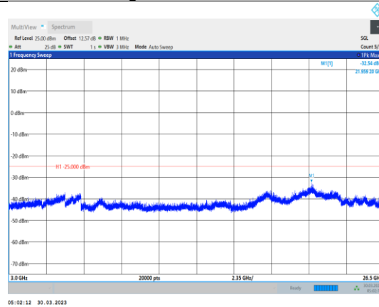
Band7-20MHz-64QAM-20850-1RB#0- Range3:3000~26500MHz
