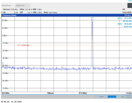
Band12-5MHz-QPSK-23035-1RB#0- Range1:30~1000MHz
