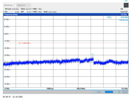
Band17-10MHz-QPSK-23790-1RB#0- Range2:1000~10000MHz
