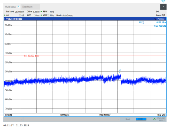
Band12-10MHz-QPSK-23095-1RB#0- Range2:1000~10000MHz
