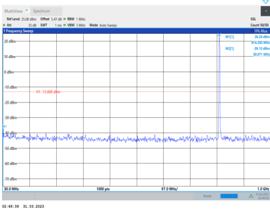
Band26-1.4MHz-QPSK-26697-1RB#0- Range1:30~1000MHz
