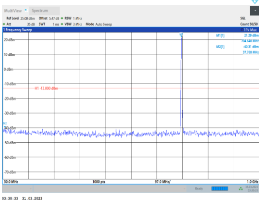
Band17-5MHz-64QAM-23755-1RB#0- Range1:30~1000MHz
