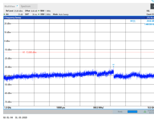
Band26-1.4MHz-QPSK-26740-1RB#0- Range2:1000~10000MHz
