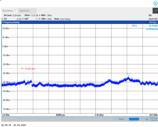
Band7-20MHz-64QAM-21100-1RB#0- Range3:3000~26500MHz
