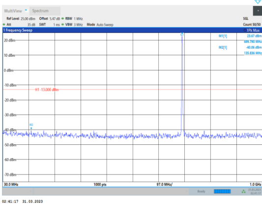
Band12-5MHz-64QAM-23035-1RB#0- Range1:30~1000MHz
