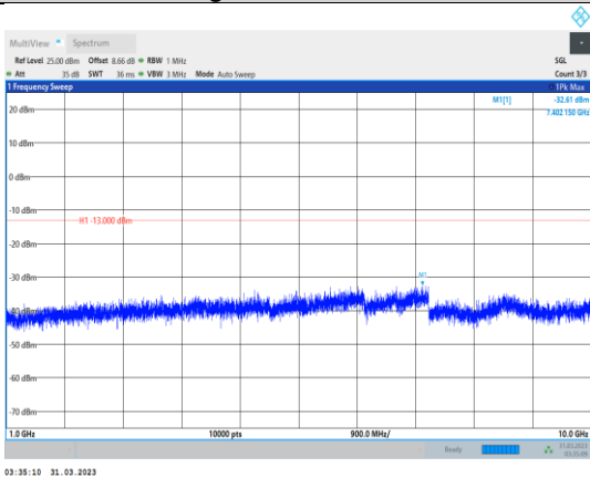
Band12-1.4MHz-64QAM-23017-1RB#0- Range2:1000~10000MHz
