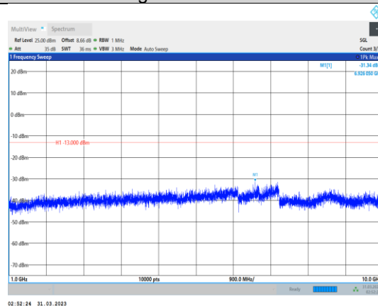
Band26-1.4MHz-QPSK-26783-1RB#0- Range2:1000~10000MHz
