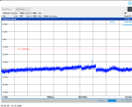
Band12-10MHz-16QAM-23060-1RB#0- Range2:1000~10000MHz
