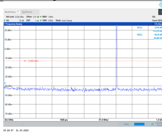
Band12-3MHz-QPSK-23165-1RB#0- Range1:30~1000MHz
