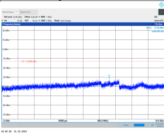
Band12-5MHz-QPSK-23035-1RB#0- Range2:1000~10000MHz
