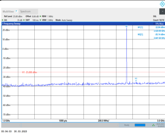
Band7-20MHz-64QAM-21100-1RB#0- Range2:1000~3000MHz
