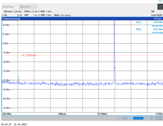
Band17-5MHz-16QAM-23755-1RB#0- Range1:30~1000MHz
