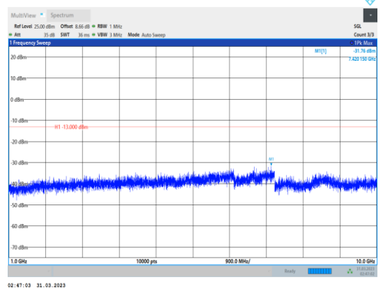
Band17-10MHz-16QAM-23790-1RB#0- Range2:1000~10000MHz
