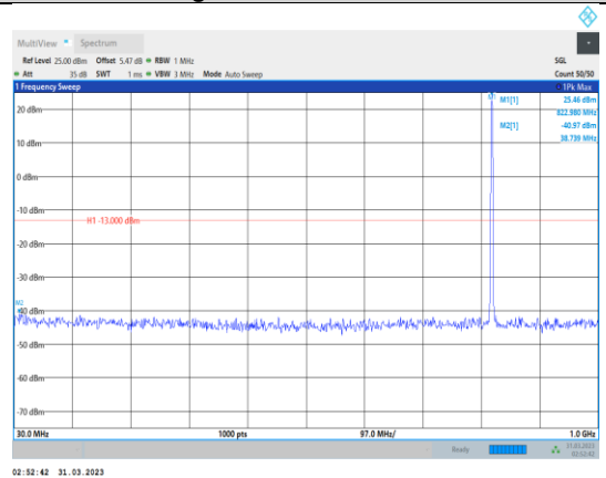
Band26-1.4MHz-16QAM-26783-1RB#0- Range1:30~1000MHz
