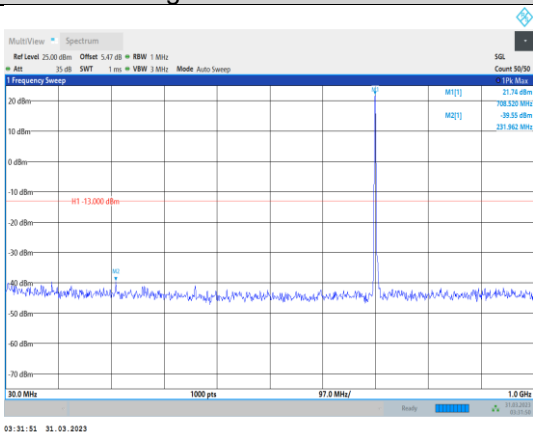
Band17-5MHz-64QAM-23790-1RB#0- Range1:30~1000MHz
