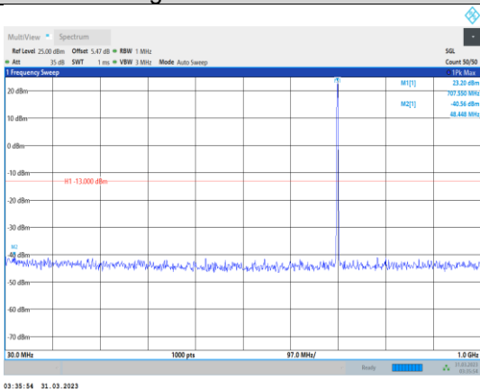
Band12-1.4MHz-16QAM-23095-1RB#0- Range1:30~1000MHz
