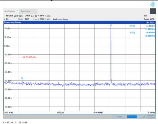
Band12-1.4MHz-64QAM-23173-1RB#0- Range1:30~1000MHz
