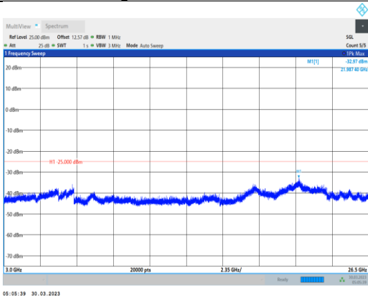
Band7-20MHz-16QAM-21350-1RB#0- Range3:3000~26500MHz
