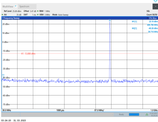
Band12-3MHz-QPSK-23025-1RB#0- Range1:30~1000MHz
