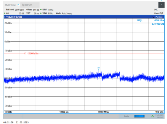
Band17-5MHz-QPSK-23790-1RB#0- Range2:1000~10000MHz
