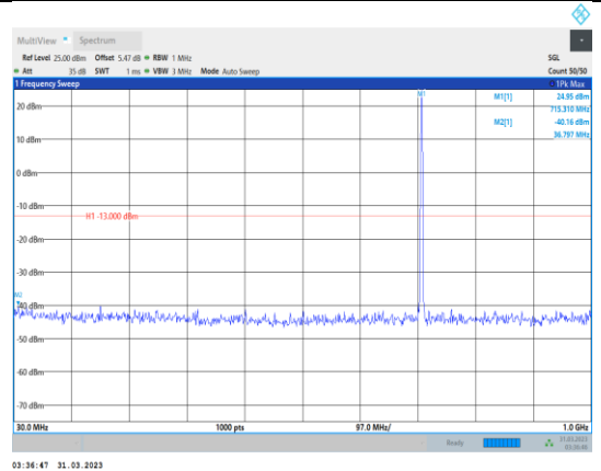
Band12-1.4MHz-QPSK-23173-1RB#0- Range1:30~1000MHz
