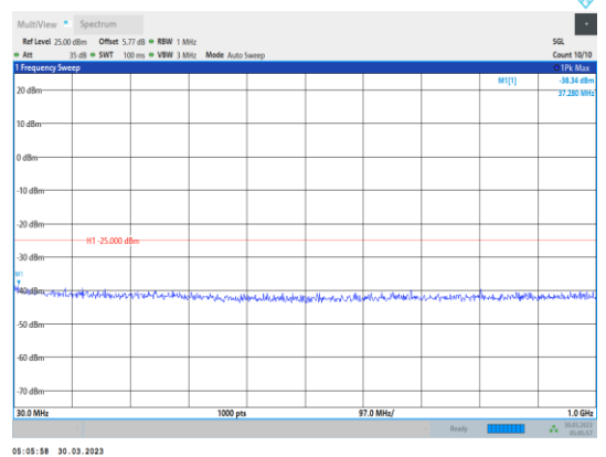
Band7-20MHz-64QAM-21350-1RB#0- Range1:30~1000MHz
