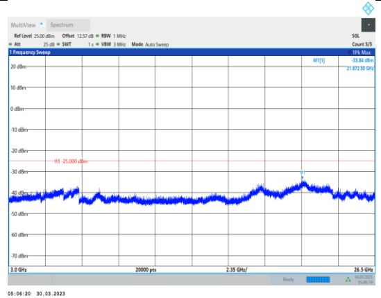
Band7-20MHz-64QAM-21350-1RB#0- Range3:3000~26500MHz
