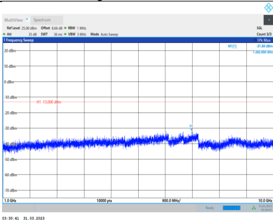
Band17-5MHz-64QAM-23755-1RB#0- Range2:1000~10000MHz
