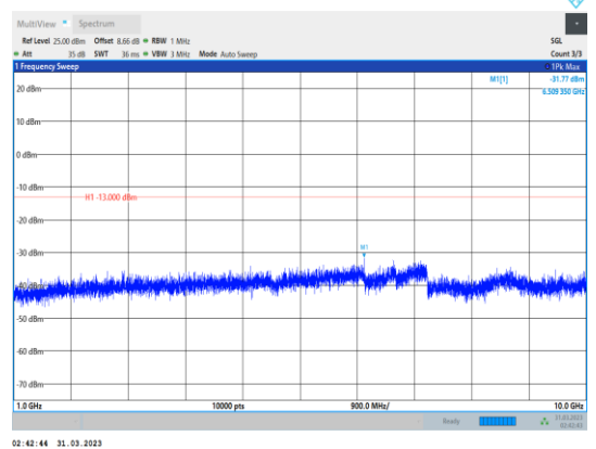
Band12-5MHz-64QAM-23095-1RB#0- Range2:1000~10000MHz
