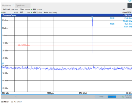
Band17-10MHz-16QAM-23780-1RB#0- Range1:30~1000MHz
