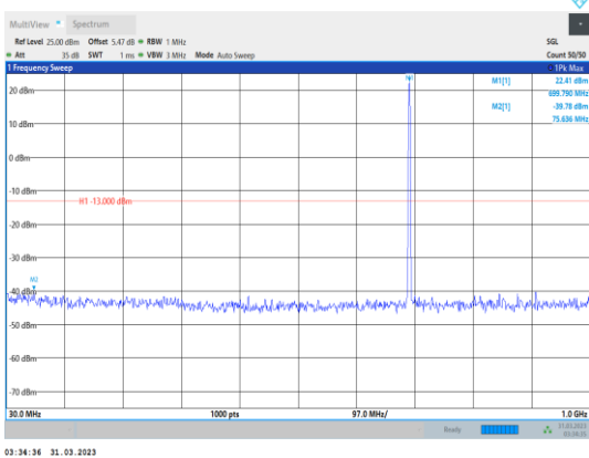
Band12-1.4MHz-16QAM-23017-1RB#0- Range1:30~1000MHz
