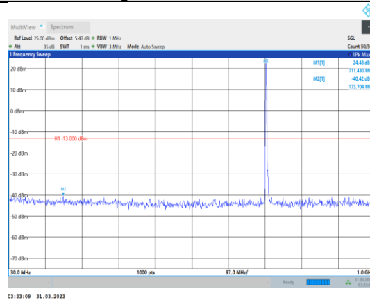
Band17-5MHz-64QAM-23825-1RB#0- Range1:30~1000MHz
