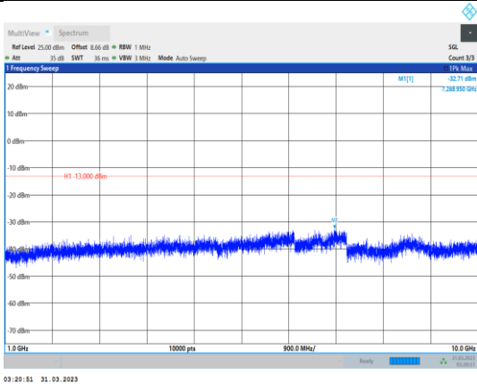
Band12-10MHz-64QAM-23060-1RB#0- Range2:1000~10000MHz
