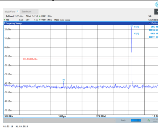
Band26-1.4MHz-QPSK-26783-1RB#0- Range1:30~1000MHz
