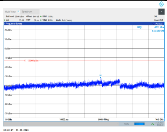
Band17-10MHz-64QAM-23800-1RB#0- Range2:1000~10000MHz
