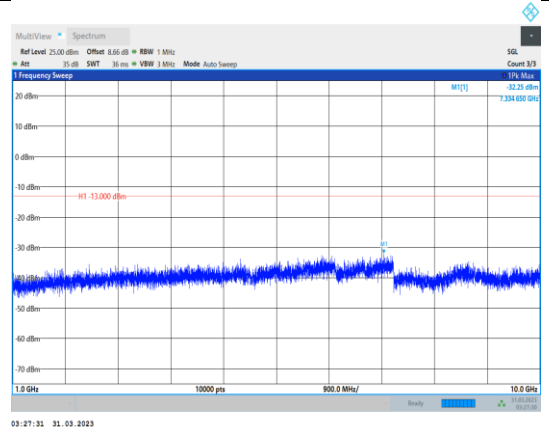
Band12-3MHz-16QAM-23165-1RB#0- Range2:1000~10000MHz
