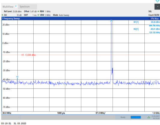
Band12-10MHz-QPSK-23060-1RB#0- Range1:30~1000MHz
