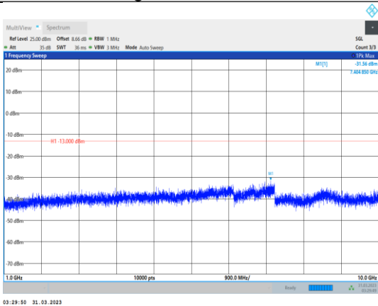
Band17-5MHz-QPSK-23755-1RB#0- Range2:1000~10000MHz
