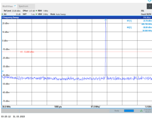
Band12-3MHz-64QAM-23025-1RB#0- Range1:30~1000MHz
