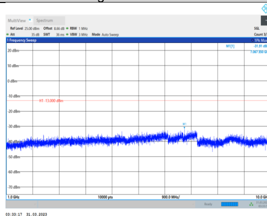
Band17-5MHz-64QAM-23825-1RB#0- Range2:1000~10000MHz
