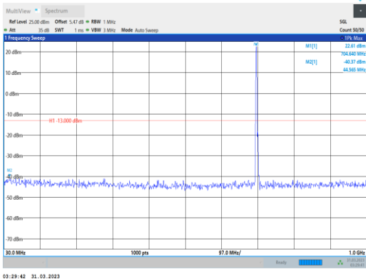
Band17-5MHz-QPSK-23755-1RB#0- Range1:30~1000MHz
