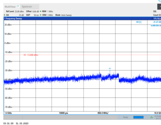
Band17-5MHz-64QAM-23790-1RB#0- Range2:1000~10000MHz
