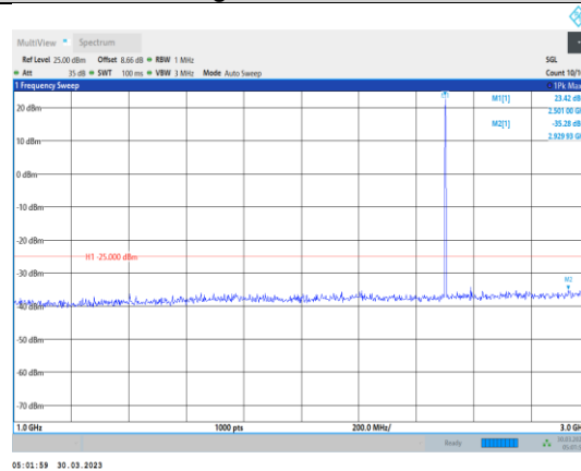
Band7-20MHz-64QAM-20850-1RB#0- Range2:1000~3000MHz
