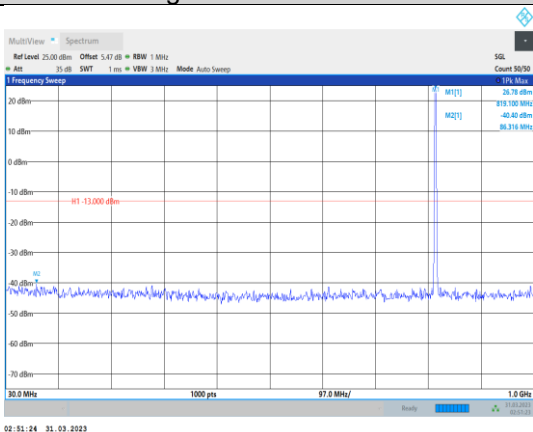
Band26-1.4MHz-16QAM-26740-1RB#0- Range1:30~1000MHz
