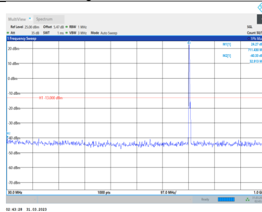
Band12-5MHz-16QAM-23155-1RB#0- Range1:30~1000MHz
