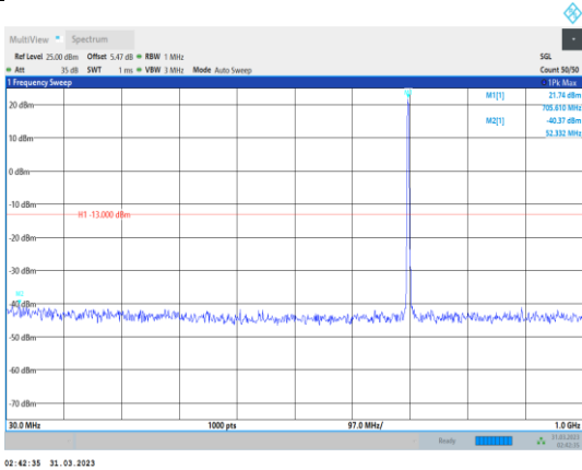
Band12-5MHz-64QAM-23095-1RB#0- Range1:30~1000MHz
