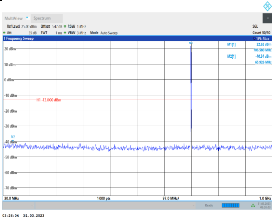
Band12-3MHz-16QAM-23095-1RB#0- Range1:30~1000MHz
