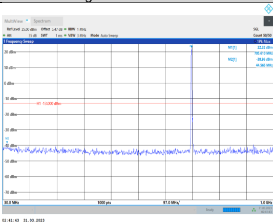
Band12-5MHz-QPSK-23095-1RB#0- Range1:30~1000MHz
