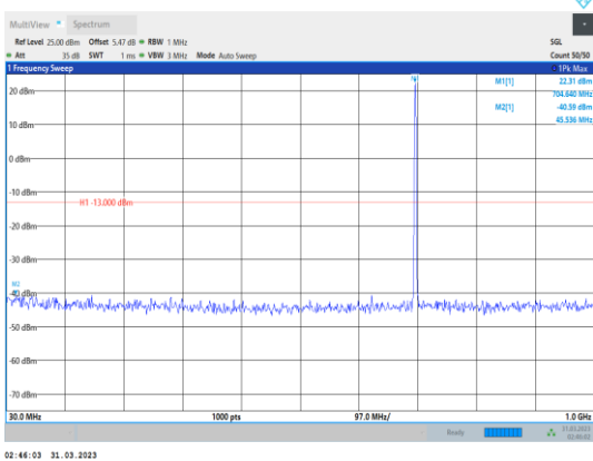
Band17-10MHz-64QAM-23780-1RB#0- Range1:30~1000MHz
