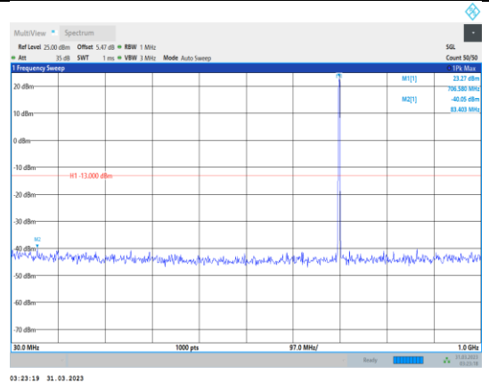
Band12-10MHz-64QAM-23130-1RB#0- Range1:30~1000MHz
