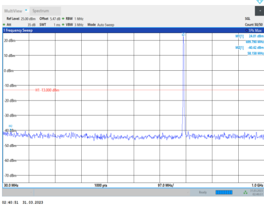
Band12-5MHz-16QAM-23035-1RB#0- Range1:30~1000MHz
