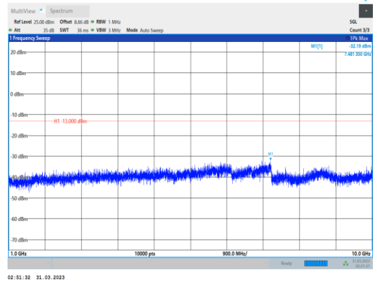
Band26-1.4MHz-16QAM-26740-1RB#0- Range2:1000~10000MHz
