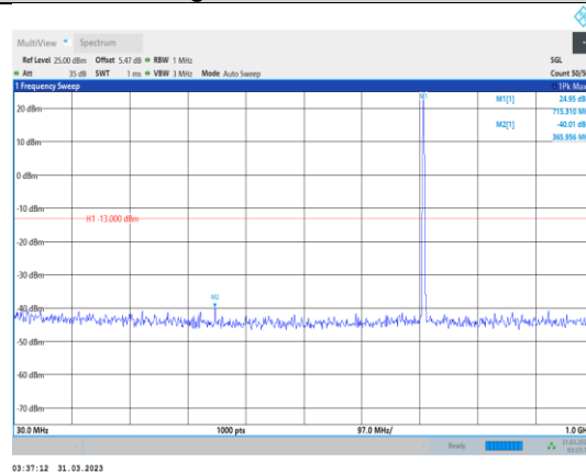
Band12-1.4MHz-16QAM-23173-1RB#0- Range1:30~1000MHz
