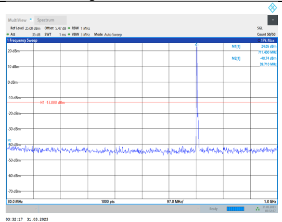
Band17-5MHz-QPSK-23825-1RB#0- Range1:30~1000MHz
