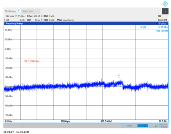
Band12-10MHz-64QAM-23130-1RB#0- Range2:1000~10000MHz
