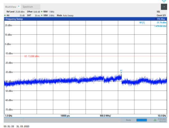
Band17-5MHz-16QAM-23790-1RB#0- Range2:1000~10000MHz
