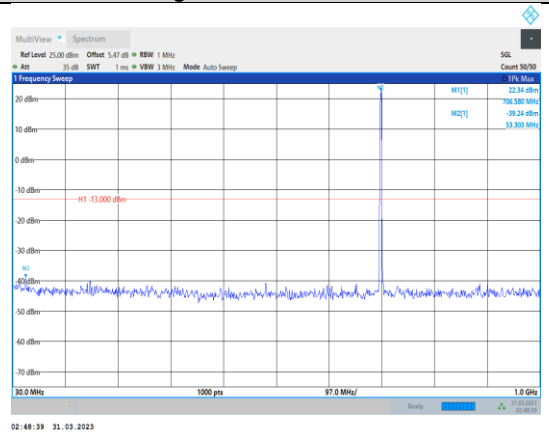
Band17-10MHz-64QAM-23800-1RB#0- Range1:30~1000MHz
