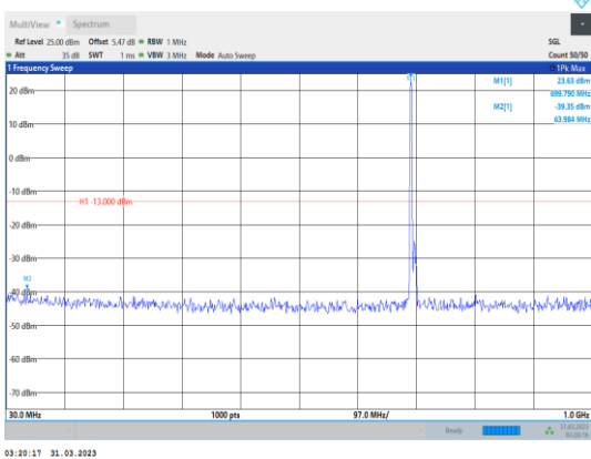
Band12-10MHz-16QAM-23060-1RB#0- Range1:30~1000MHz
