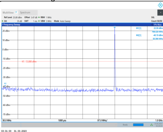
Band17-5MHz-QPSK-23790-1RB#0- Range1:30~1000MHz
