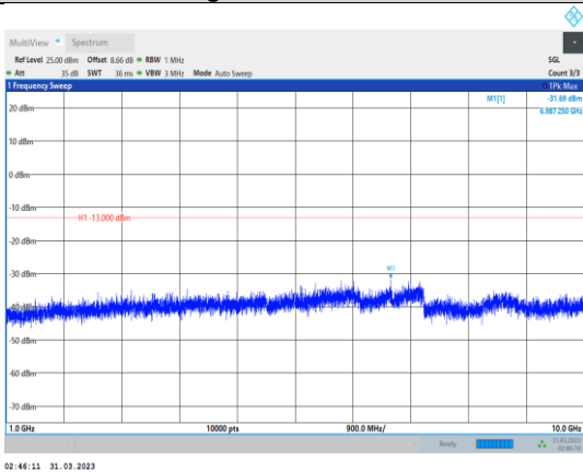
Band17-10MHz-64QAM-23780-1RB#0- Range2:1000~10000MHz
