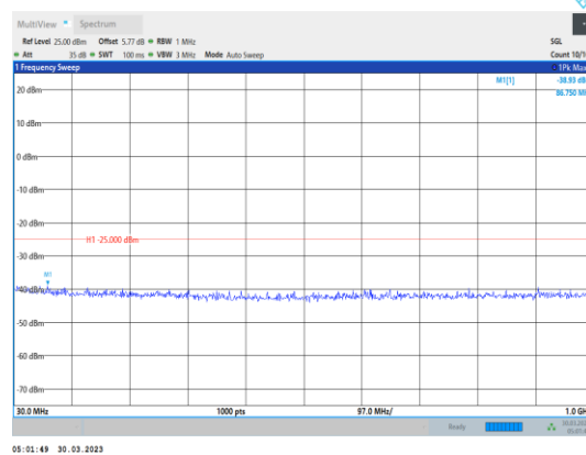
Band7-20MHz-64QAM-20850-1RB#0- Range1:30~1000MHz
