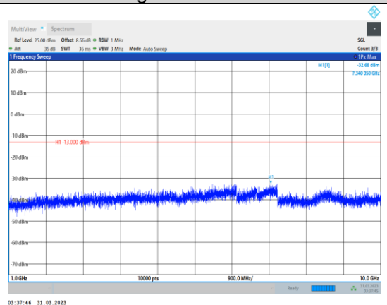
Band12-1.4MHz-64QAM-23173-1RB#0- Range2:1000~10000MHz
