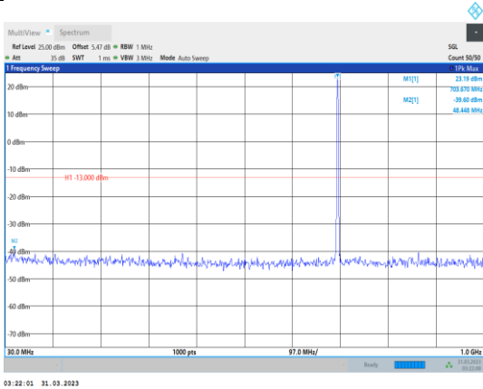
Band12-10MHz-64QAM-23095-1RB#0- Range1:30~1000MHz
