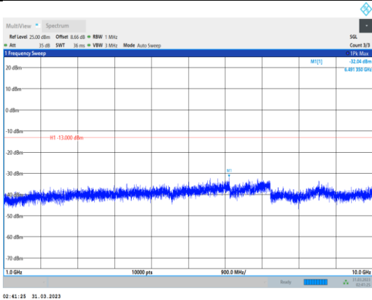
Band12-5MHz-64QAM-23035-1RB#0- Range2:1000~10000MHz
