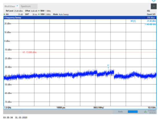
Band12-1.4MHz-QPSK-23095-1RB#0- Range2:1000~10000MHz
