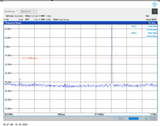
Band12-3MHz-64QAM-23165-1RB#0- Range1:30~1000MHz
