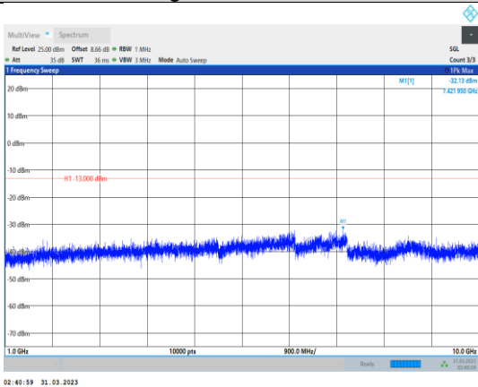
Band12-5MHz-16QAM-23035-1RB#0- Range2:1000~10000MHz
