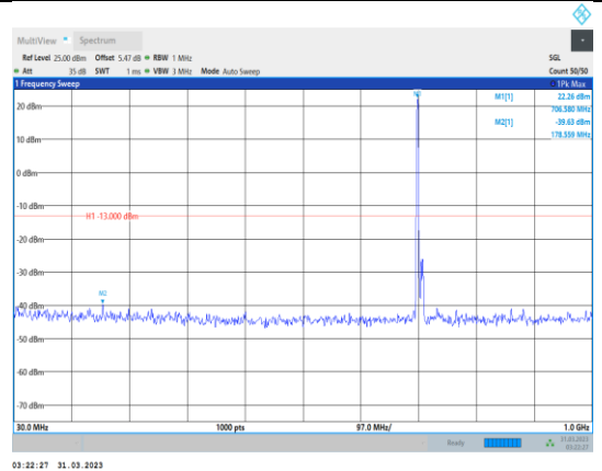
Band12-10MHz-QPSK-23130-1RB#0- Range1:30~1000MHz
