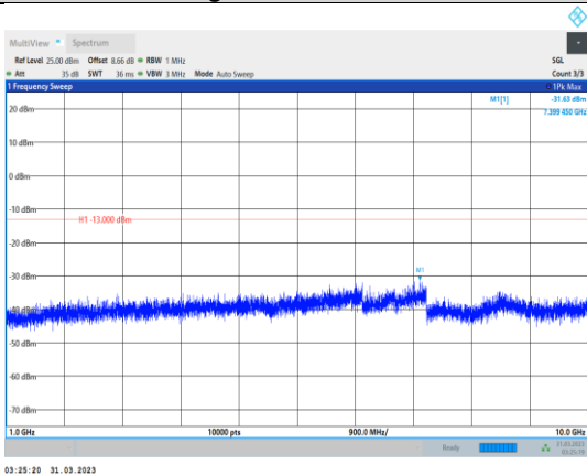
Band12-3MHz-64QAM-23025-1RB#0- Range2:1000~10000MHz
