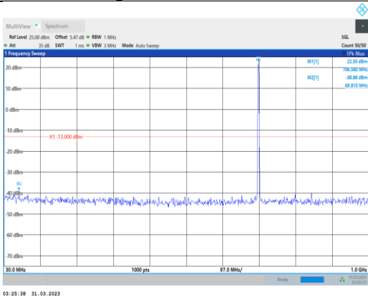
Band12-3MHz-QPSK-23095-1RB#0- Range1:30~1000MHz
