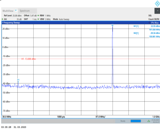
Band12-1.4MHz-QPSK-23095-1RB#0- Range1:30~1000MHz
