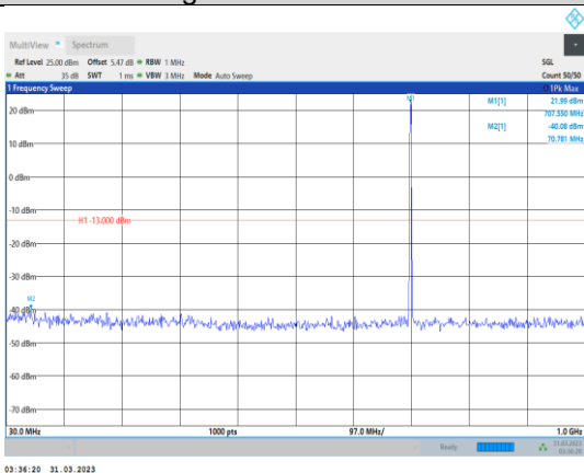
Band12-1.4MHz-64QAM-23095-1RB#0- Range1:30~1000MHz
