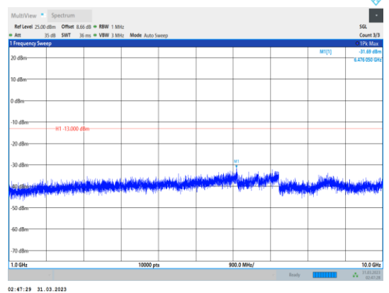
Band17-10MHz-64QAM-23790-1RB#0- Range2:1000~10000MHz
