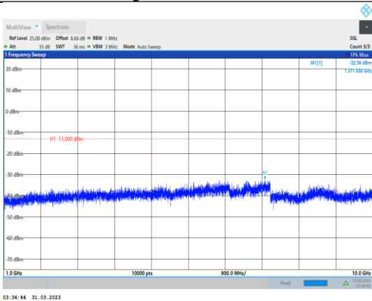
Band12-1.4MHz-16QAM-23017-1RB#0- Range2:1000~10000MHz
