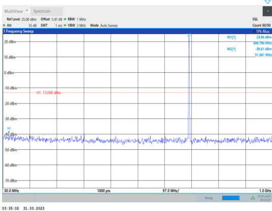
Band12-1.4MHz-64QAM-23017-1RB#0- Range1:30~1000MHz
