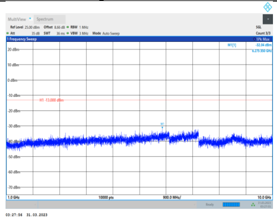
Band12-3MHz-64QAM-23165-1RB#0- Range2:1000~10000MHz
