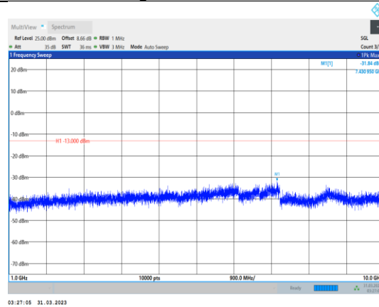
Band12-3MHz-QPSK-23165-1RB#0- Range2:1000~10000MHz
