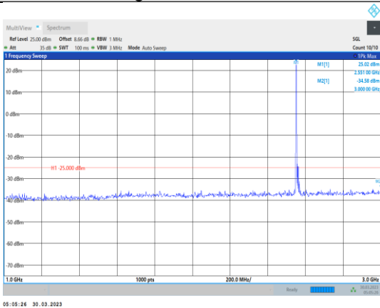
Band7-20MHz-16QAM-21350-1RB#0- Range2:1000~3000MHz
