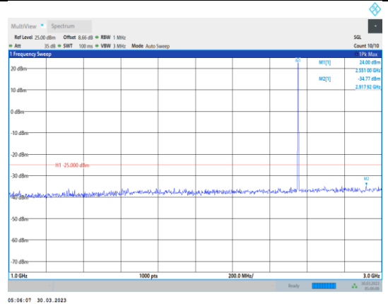
Band7-20MHz-64QAM-21350-1RB#0- Range2:1000~3000MHz
