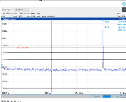
Band26-1.4MHz-QPSK-26740-1RB#0- Range1:30~1000MHz
