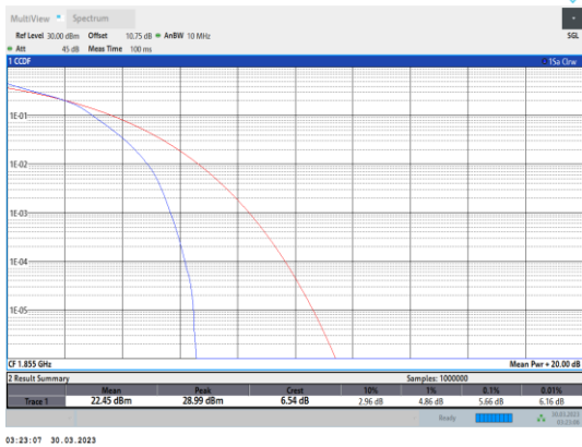
Band2-10MHz-16QAM-18650-50RB#0
