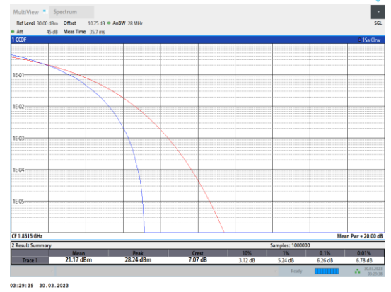
Band2-3MHz-64QAM-18615-15RB#0
