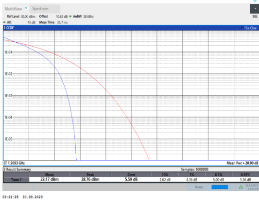
Band2-1.4MHz-QPSK-19193-6RB#0
