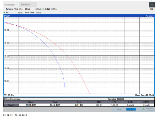
Band2-10MHz-64QAM-18900-50RB#0
