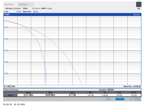
Band2-5MHz-16QAM-18625-25RB#0
