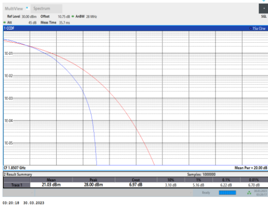
Band2-1.4MHz-64QAM-18607-6RB#0
