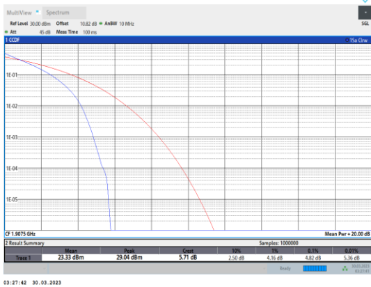
Band2-5MHz-QPSK-19175-25RB#0
