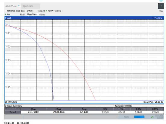
Band2-10MHz-QPSK-19150-50RB#0
