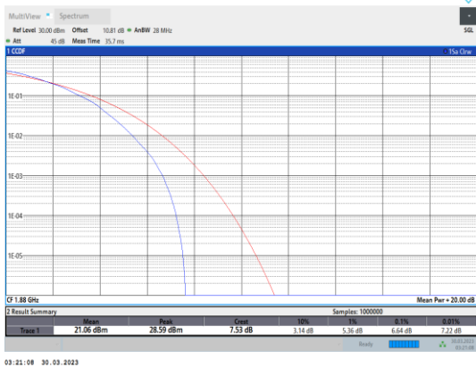
Band2-1.4MHz-64QAM-18900-6RB#0
