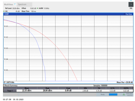
Band2-5MHz-16QAM-19175-25RB#0
