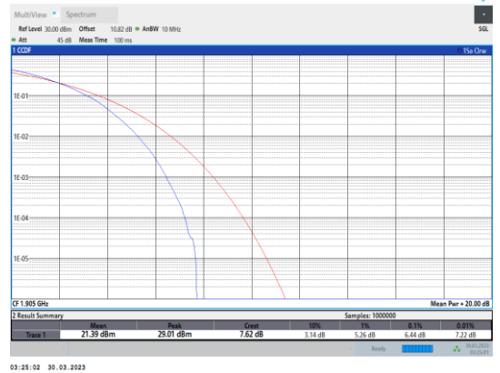
Band2-10MHz-64QAM-19150-50RB#0
