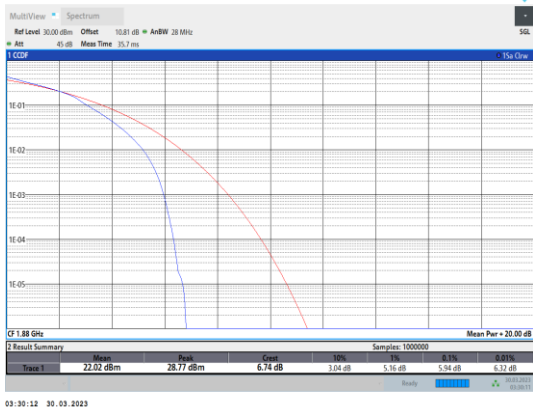
Band2-3MHz-16QAM-18900-15RB#0
