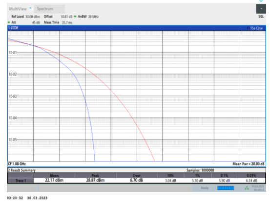
Band2-1.4MHz-16QAM-18900-6RB#0
