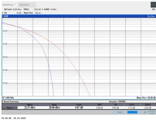
Band2-10MHz-16QAM-19150-50RB#0
