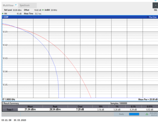
Band2-1.4MHz-64QAM-19193-6RB#0
