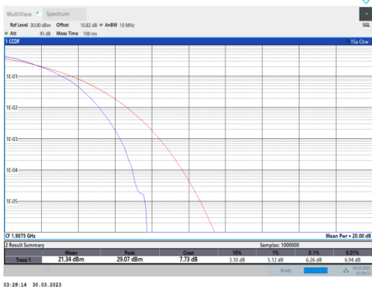
Band2-5MHz-64QAM-19175-25RB#0
