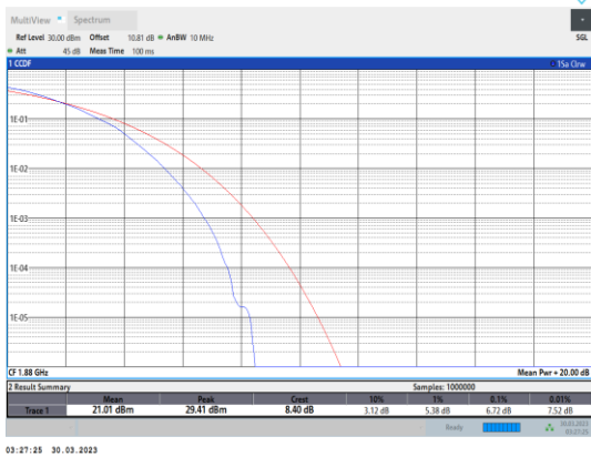
Band2-5MHz-64QAM-18900-25RB#0
