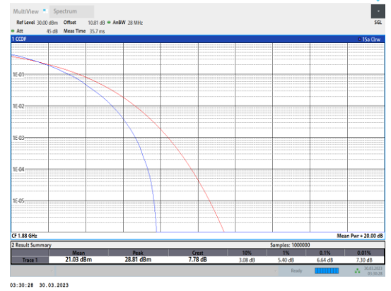
Band2-3MHz-64QAM-18900-15RB#0
