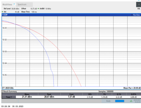
Band2-5MHz-64QAM-18625-25RB#0
