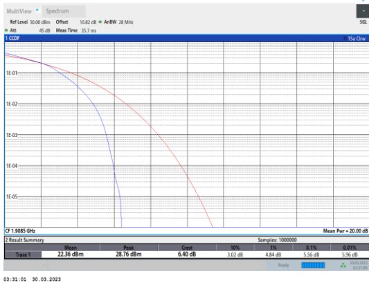
Band2-3MHz-16QAM-19185-15RB#0
