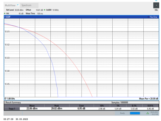
Band2-5MHz-16QAM-18900-25RB#0
