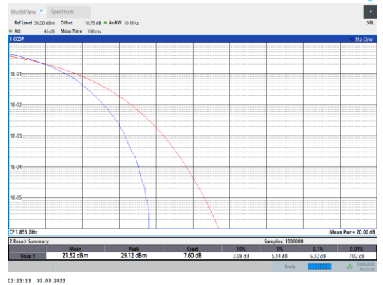
Band2-10MHz-64QAM-18650-50RB#0
