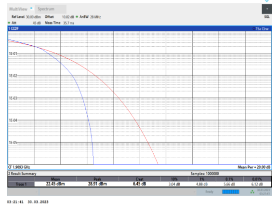
Band2-1.4MHz-16QAM-19193-6RB#0
