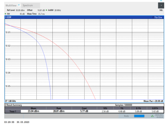
Band2-3MHz-QPSK-18900-15RB#0
