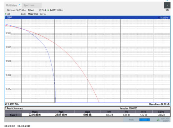
Band2-1.4MHz-16QAM-18607-6RB#0
