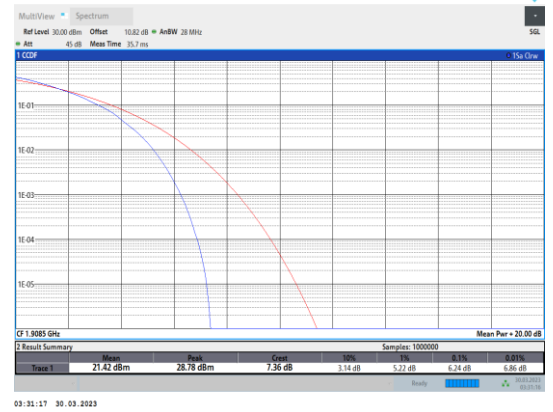
Band2-3MHz-64QAM-19185-15RB#0
