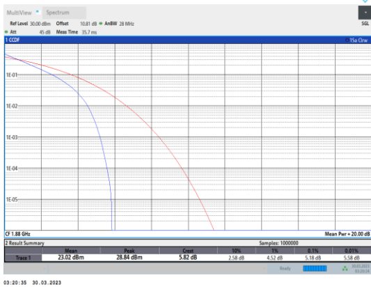
Band2-1.4MHz-QPSK-18900-6RB#0
