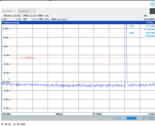
Band26-5MHz-16QAM-26740-1RB#0- Range1:30~1000MHz
