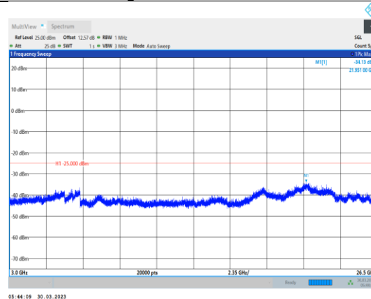
Band38-10MHz-QPSK-38200-1RB#0- Range3:3000~26500MHz
