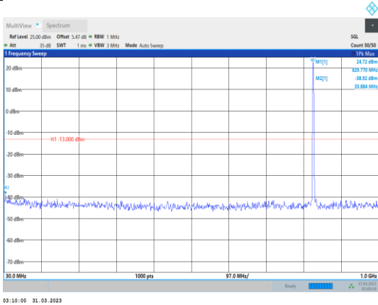
Band26-15MHz-64QAM-26915-1RB#0- Range1:30~1000MHz
