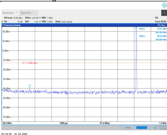
Band26-3MHz-16QAM-26740-1RB#0- Range1:30~1000MHz
