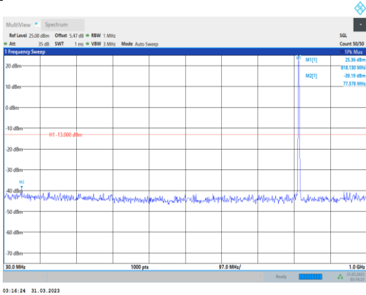
Band26-3MHz-QPSK-26740-1RB#0- Range1:30~1000MHz
