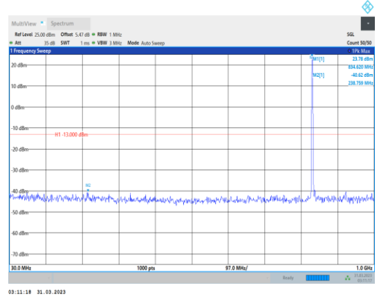
Band26-15MHz-64QAM-26965-1RB#0- Range1:30~1000MHz
