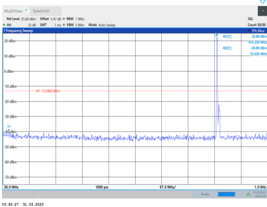
Band26-10MHz-QPSK-26740-1RB#0- Range1:30~1000MHz
