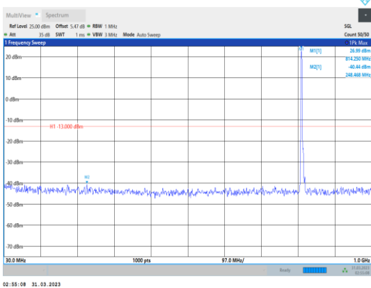
Band26-5MHz-64QAM-26715-1RB#0- Range1:30~1000MHz
