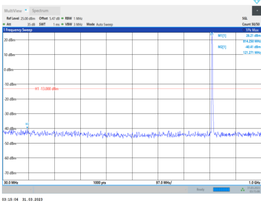
Band26-3MHz-QPSK-26705-1RB#0- Range1:30~1000MHz
