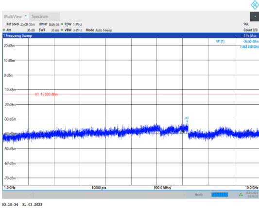
Band26-15MHz-QPSK-26965-1RB#0- Range2:1000~10000MHz
