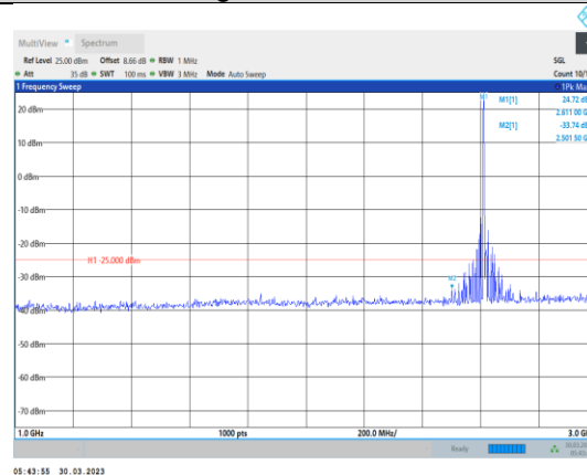
Band38-10MHz-QPSK-38200-1RB#0- Range2:1000~3000MHz
