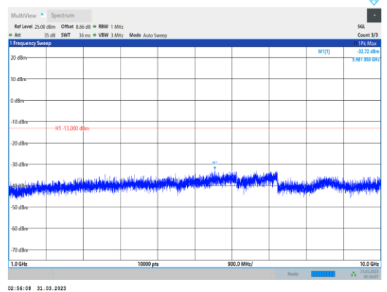
Band26-5MHz-16QAM-26740-1RB#0- Range2:1000~10000MHz
