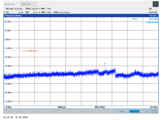
Band26-15MHz-16QAM-26765-1RB#0- Range2:1000~10000MHz
