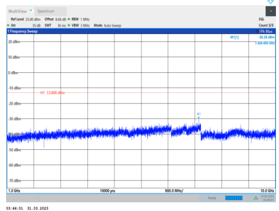
Band26-10MHz-16QAM-26740-1RB#0- Range2:1000~10000MHz
