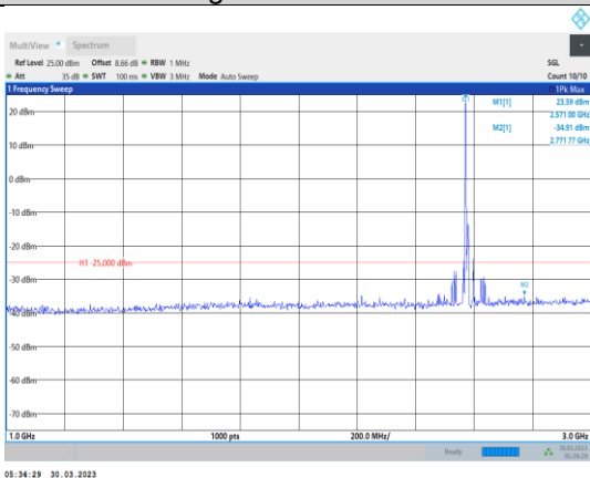
Band38-5MHz-64QAM-37775-1RB#0- Range2:1000~3000MHz
