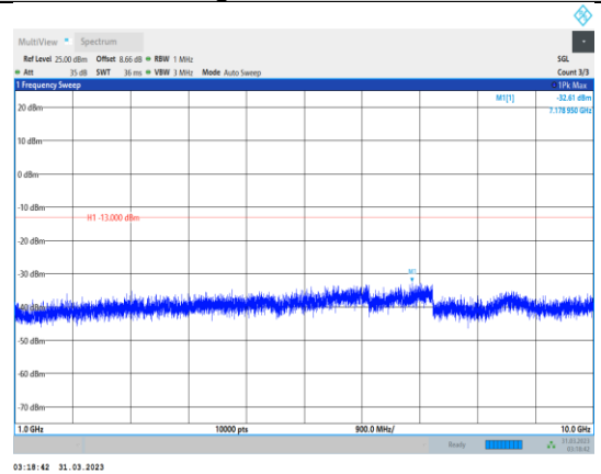
Band26-3MHz-64QAM-26775-1RB#0- Range2:1000~10000MHz
