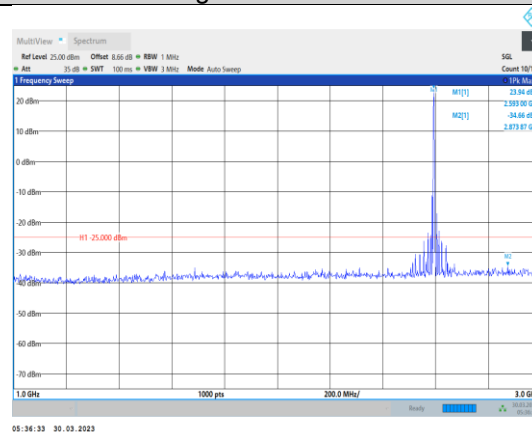
Band38-5MHz-64QAM-38000-1RB#0- Range2:1000~3000MHz
