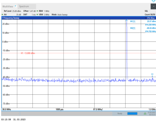
Band26-3MHz-64QAM-26705-1RB#0- Range1:30~1000MHz
