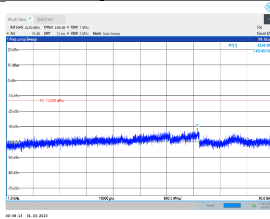
Band26-15MHz-QPSK-26915-1RB#0- Range2:1000~10000MHz
