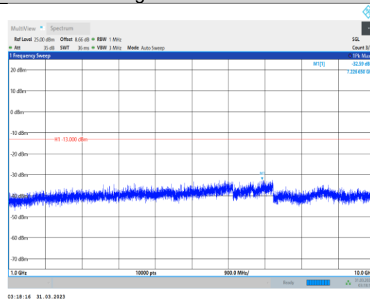
Band26-3MHz-16QAM-26775-1RB#0- Range2:1000~10000MHz
