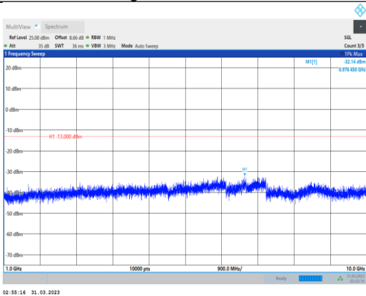
Band26-5MHz-64QAM-26715-1RB#0- Range2:1000~10000MHz
