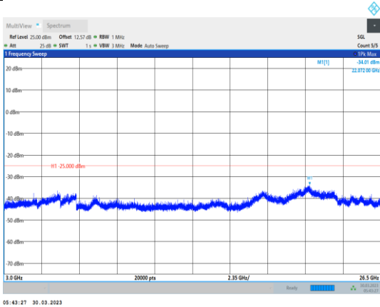
Band38-10MHz-64QAM-38000-1RB#0-Range3:3000~26500MHz
