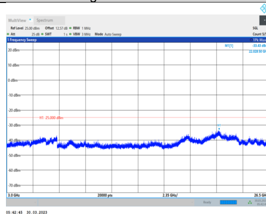
Band38-10MHz-16QAM-38000-1RB#0-Range3:3000~26500MHz
