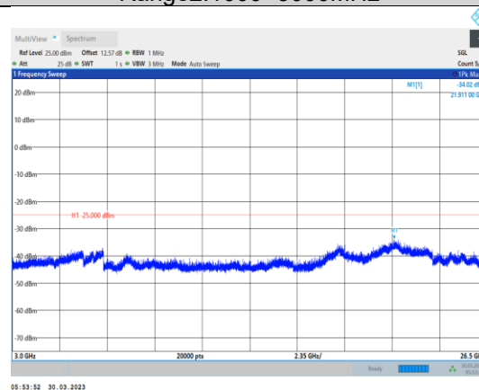
Band38-15MHz-QPSK-38000-1RB#0- Range3:3000~26500MHz
