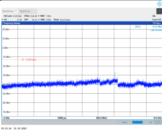
Band26-3MHz-QPSK-26705-1RB#0- Range2:1000~10000MHz
