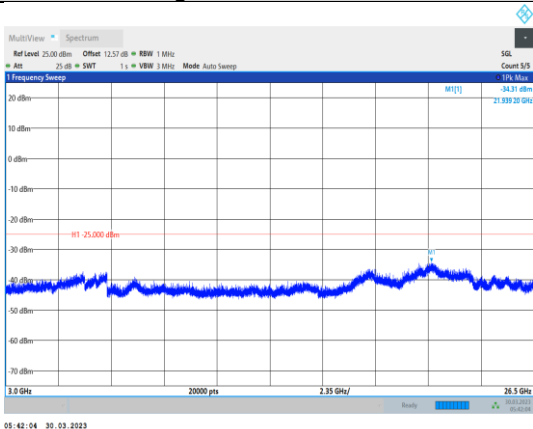
Band38-10MHz-QPSK-38000-1RB#0- Range3:3000~26500MHz
