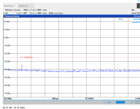
Band38-5MHz-16QAM-38225-1RB#0- Range1:30~1000MHz
