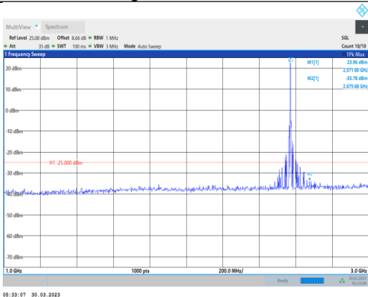
Band38-5MHz-QPSK-37775-1RB#0- Range2:1000~3000MHz
