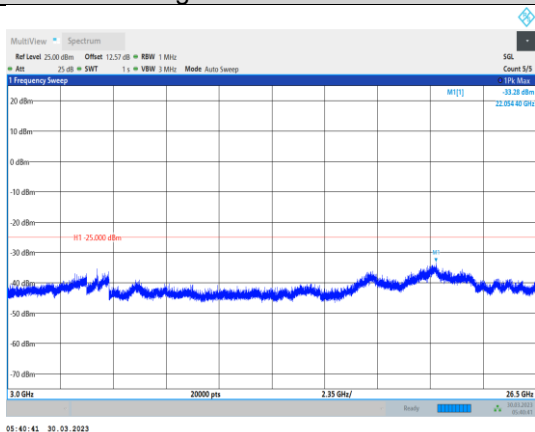
Band38-10MHz-16QAM-37800-1RB#0-Range3:3000~26500MHz
