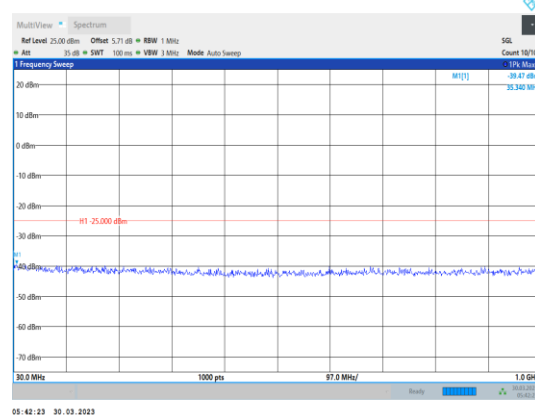
Band38-10MHz-16QAM-38000-1RB#0-Range1:30~1000MHz
