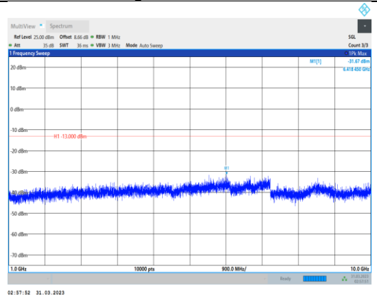
Band26-5MHz-64QAM-26765-1RB#0- Range2:1000~10000MHz
