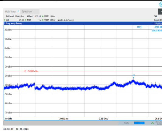
Band38-5MHz-16QAM-38225-1RB#0- Range3:3000~26500MHz
