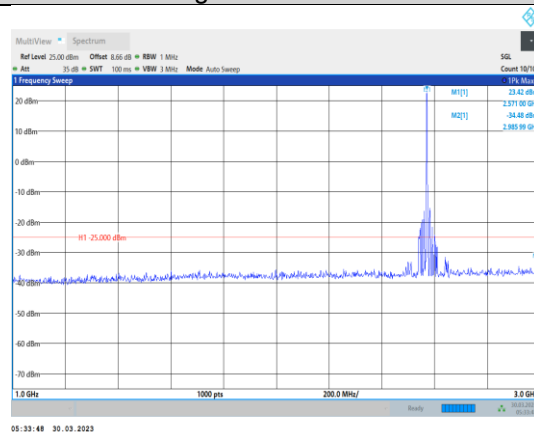
Band38-5MHz-16QAM-37775-1RB#0- Range2:1000~3000MHz
