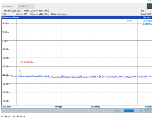
Band38-10MHz-QPSK-38000-1RB#0- Range1:30~1000MHz
