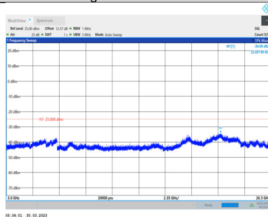
Band38-5MHz-16QAM-37775-1RB#0- Range3:3000~26500MHz
