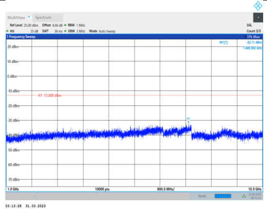
Band26-15MHz-64QAM-26765-1RB#0- Range2:1000~10000MHz
