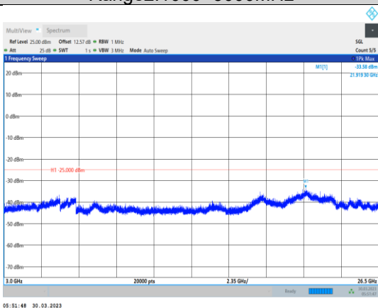
Band38-15MHz-QPSK-37825-1RB#0- Range3:3000~26500MHz
