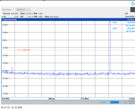
Band26-3MHz-64QAM-26740-1RB#0- Range1:30~1000MHz
