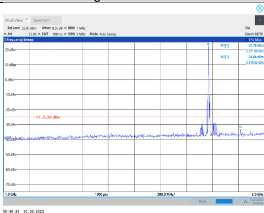
Band38-10MHz-16QAM-37800-1RB#0-Range2:1000~3000MHz
