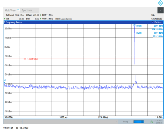
Band26-15MHz-16QAM-26865-1RB#0- Range1:30~1000MHz
