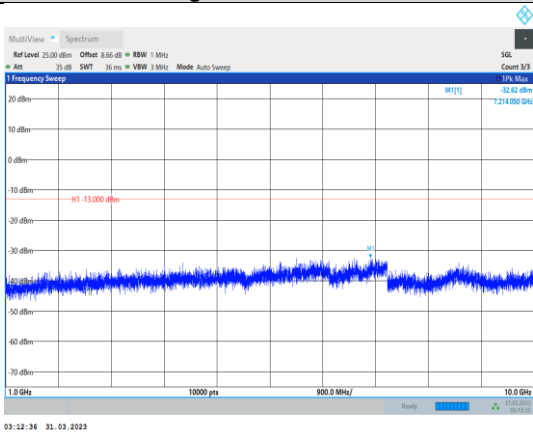
Band26-15MHz-QPSK-26765-1RB#0- Range2:1000~10000MHz
