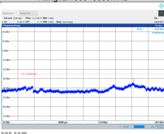
Band38-5MHz-64QAM-37775-1RB#0- Range3:3000~26500MHz
