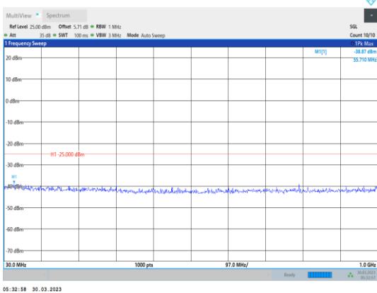
Band38-5MHz-QPSK-37775-1RB#0- Range1:30~1000MHz
