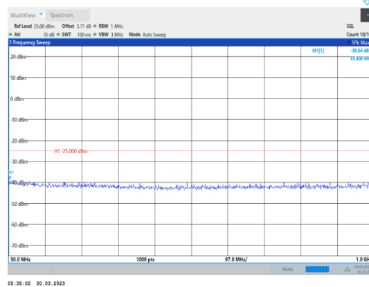
Band38-5MHz-QPSK-38000-1RB#0- Range1:30~1000MHz
