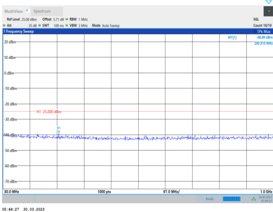
Band38-10MHz-16QAM-38200-1RB#0-Range1:30~1000MHz
