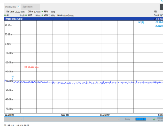
Band38-5MHz-64QAM-38000-1RB#0- Range1:30~1000MHz
