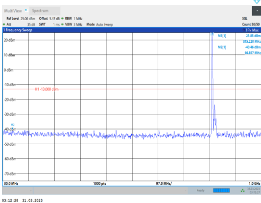
Band26-15MHz-QPSK-26765-1RB#0- Range1:30~1000MHz
