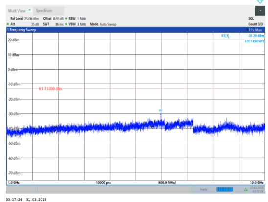
Band26-3MHz-64QAM-26740-1RB#0- Range2:1000~10000MHz
