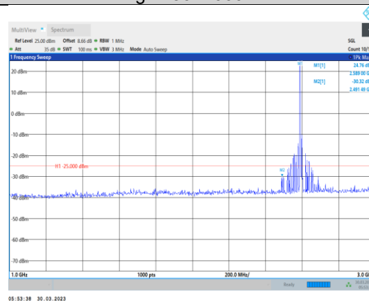
Band38-15MHz-QPSK-38000-1RB#0- Range2:1000~3000MHz
