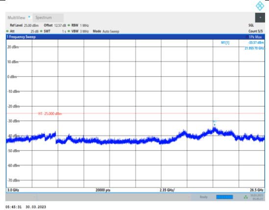
Band38-10MHz-64QAM-38200-1RB#0-Range3:3000~26500MHz
