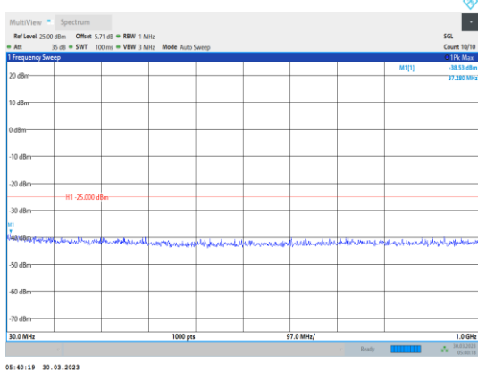
Band38-10MHz-16QAM-37800-1RB#0-Range1:30~1000MHz
