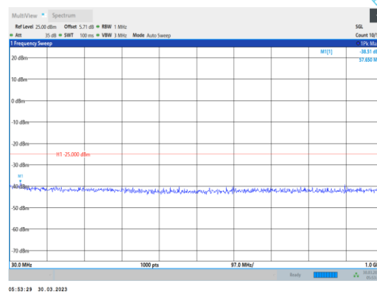
Band38-15MHz-QPSK-38000-1RB#0- Range1:30~1000MHz
