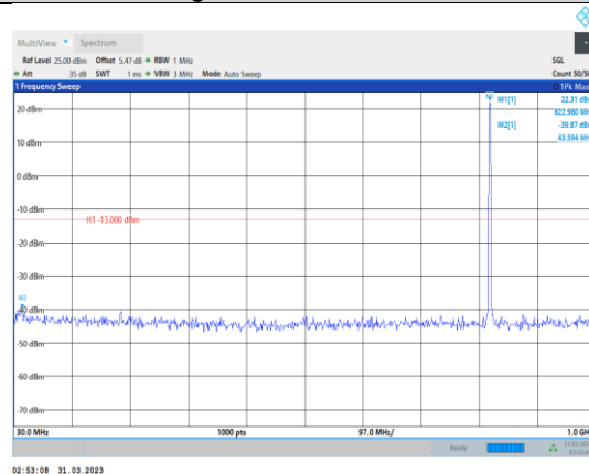
Band26-1.4MHz-64QAM-26783-1RB#0- Range1:30~1000MHz
