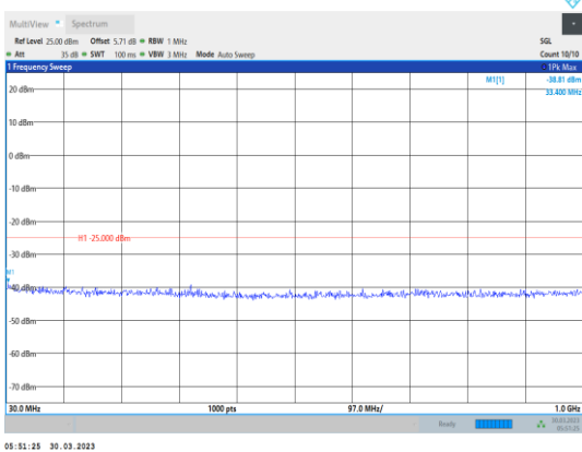
Band38-15MHz-QPSK-37825-1RB#0- Range1:30~1000MHz
