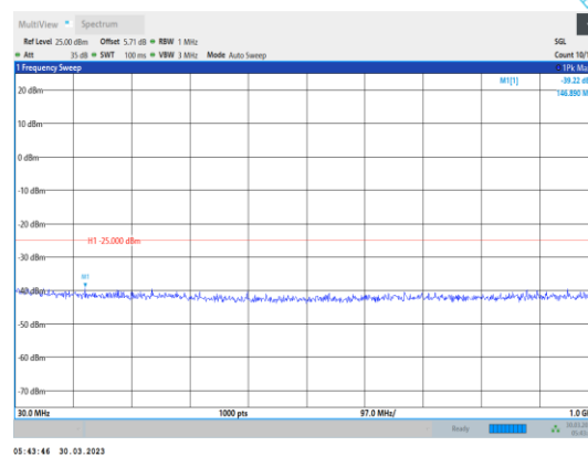
Band38-10MHz-QPSK-38200-1RB#0- Range1:30~1000MHz
