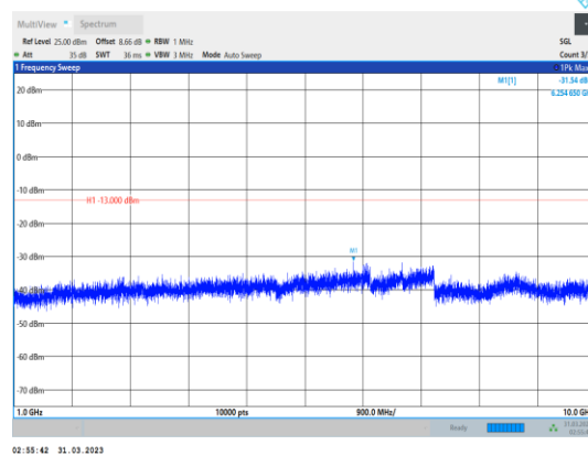
Band26-5MHz-QPSK-26740-1RB#0- Range2:1000~10000MHz
