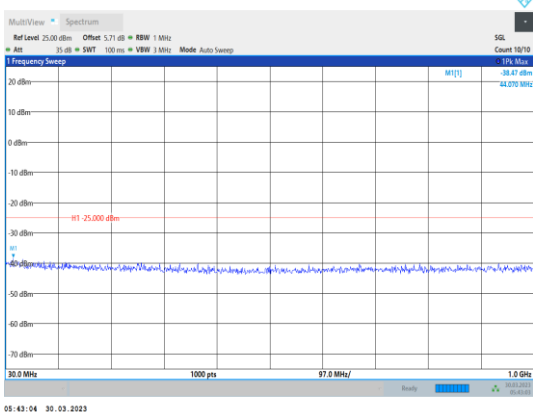
Band38-10MHz-64QAM-38000-1RB#0-Range1:30~1000MHz
