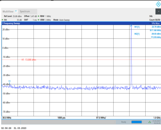
Band26-5MHz-64QAM-26740-1RB#0- Range1:30~1000MHz
