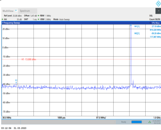
Band26-15MHz-16QAM-26765-1RB#0- Range1:30~1000MHz
