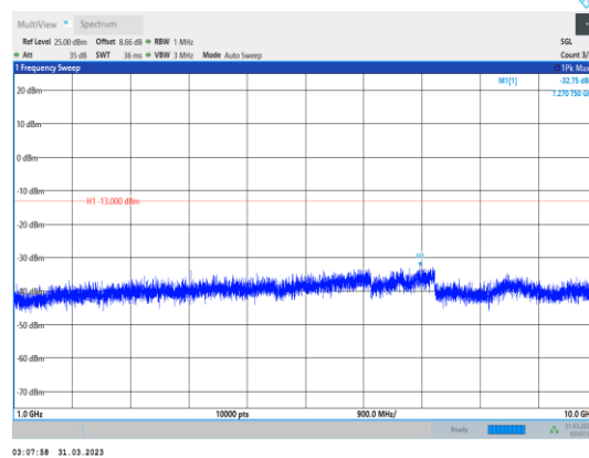
Band26-15MHz-QPSK-26865-1RB#0- Range2:1000~10000MHz
