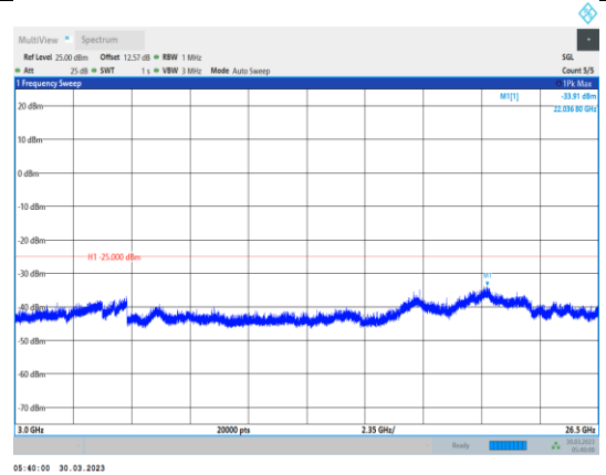
Band38-10MHz-QPSK-37800-1RB#0- Range3:3000~26500MHz
