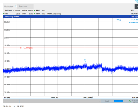
Band26-1.4MHz-64QAM-26740-1RB#0- Range2:1000~10000MHz
