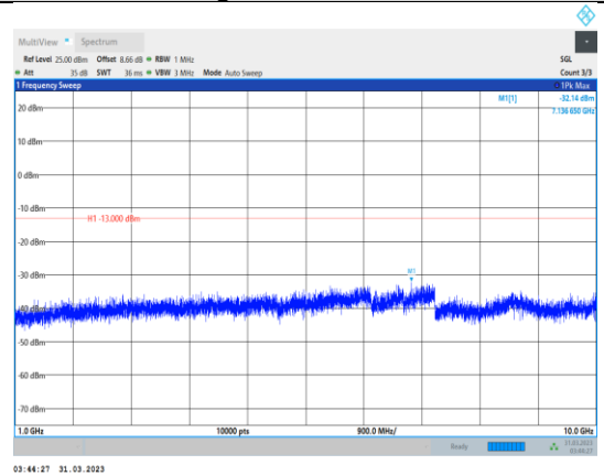
Band26-10MHz-64QAM-26740-1RB#0- Range2:1000~10000MHz
