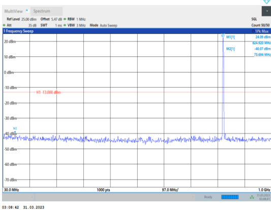
Band26-15MHz-64QAM-26865-1RB#0- Range1:30~1000MHz
