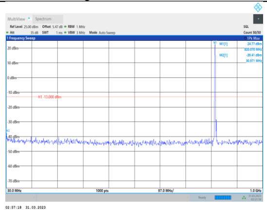
Band26-5MHz-16QAM-26765-1RB#0- Range1:30~1000MHz
