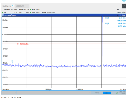
Band26-1.4MHz-64QAM-26697-1RB#0- Range1:30~1000MHz
