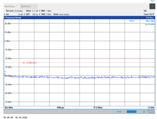
Band38-10MHz-QPSK-37800-1RB#0- Range1:30~1000MHz
