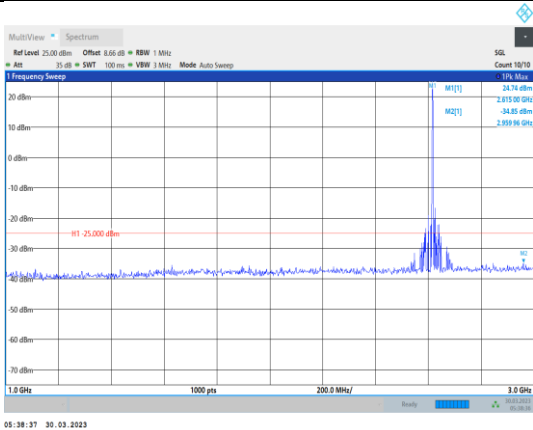
Band38-5MHz-64QAM-38225-1RB#0- Range2:1000~3000MHz
