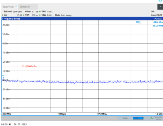
Band38-5MHz-16QAM-38000-1RB#0- Range1:30~1000MHz
