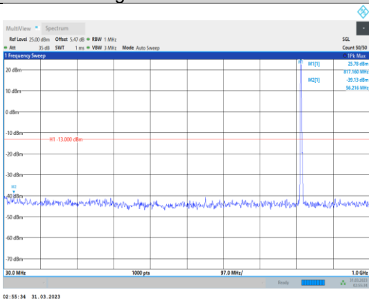
Band26-5MHz-QPSK-26740-1RB#0- Range1:30~1000MHz
