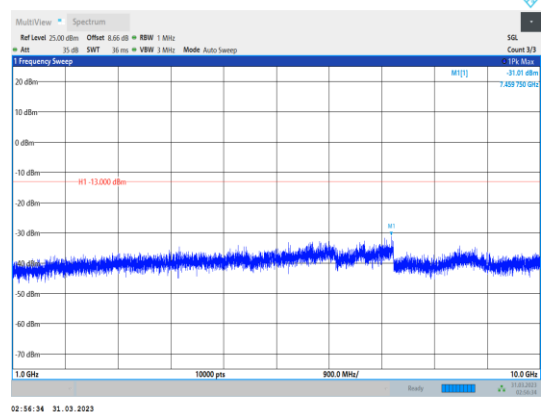
Band26-5MHz-64QAM-26740-1RB#0- Range2:1000~10000MHz
