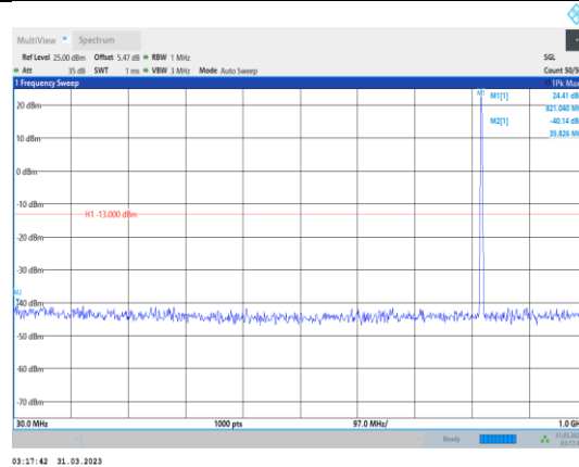
Band26-3MHz-QPSK-26775-1RB#0- Range1:30~1000MHz
