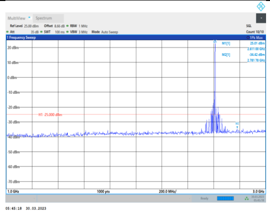
Band38-10MHz-64QAM-38200-1RB#0-Range2:1000~3000MHz
