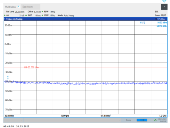
Band38-10MHz-64QAM-38200-1RB#0-Range1:30~1000MHz
