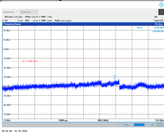
Band26-1.4MHz-64QAM-26697-1RB#0- Range2:1000~10000MHz
