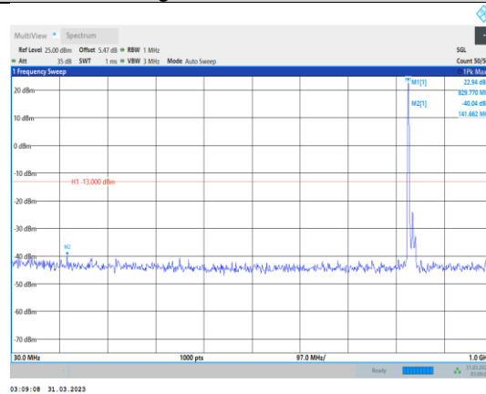
Band26-15MHz-QPSK-26915-1RB#0- Range1:30~1000MHz
