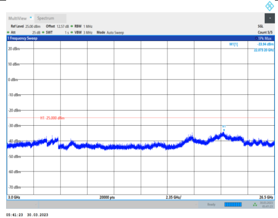
Band38-10MHz-64QAM-37800-1RB#0-Range3:3000~26500MHz
