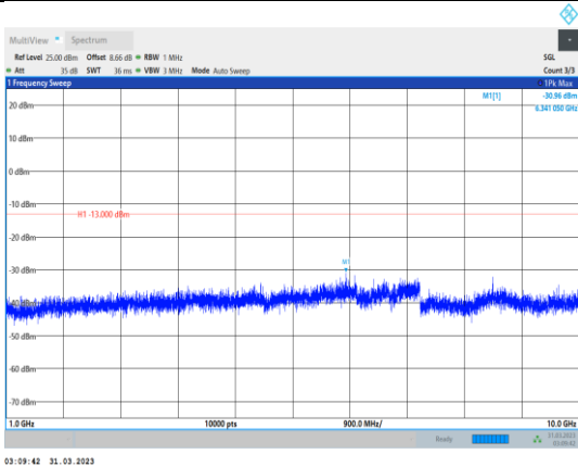
Band26-15MHz-16QAM-26915-1RB#0- Range2:1000~10000MHz
