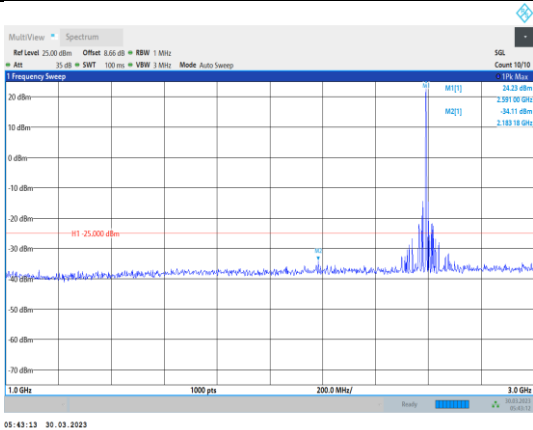
Band38-10MHz-64QAM-38000-1RB#0-Range2:1000~3000MHz
