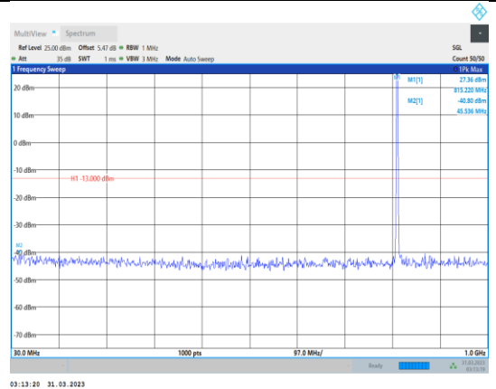
Band26-15MHz-64QAM-26765-1RB#0- Range1:30~1000MHz
