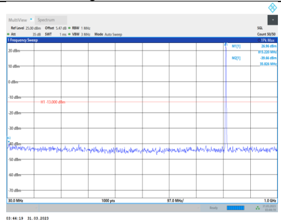
Band26-10MHz-64QAM-26740-1RB#0- Range1:30~1000MHz
