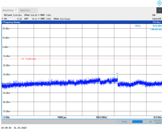
Band26-15MHz-64QAM-26865-1RB#0- Range2:1000~10000MHz
