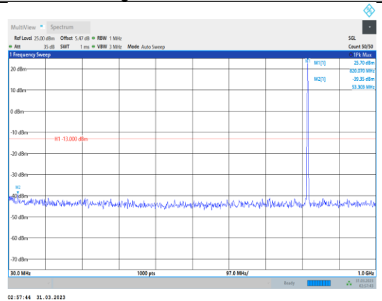
Band26-5MHz-64QAM-26765-1RB#0- Range1:30~1000MHz
