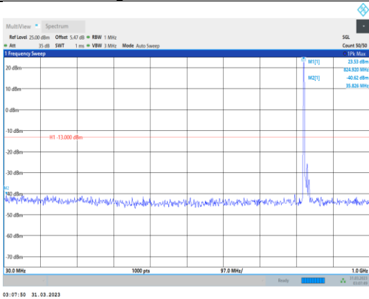
Band26-15MHz-QPSK-26865-1RB#0- Range1:30~1000MHz
