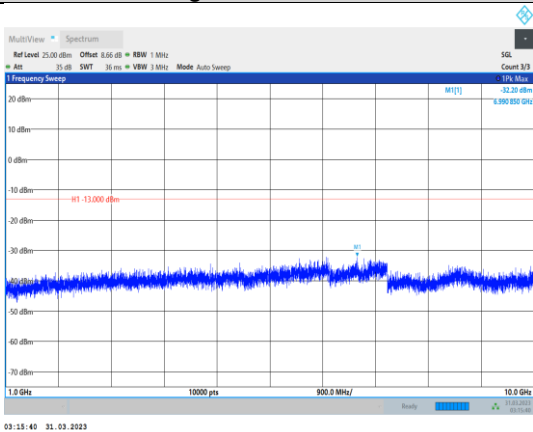
Band26-3MHz-16QAM-26705-1RB#0- Range2:1000~10000MHz
