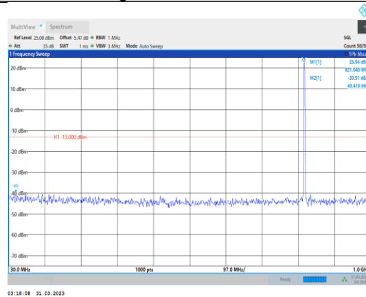
Band26-3MHz-16QAM-26775-1RB#0- Range1:30~1000MHz
