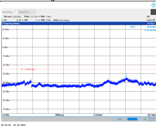
Band38-5MHz-QPSK-37775-1RB#0- Range3:3000~26500MHz
