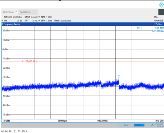
Band26-5MHz-16QAM-26715-1RB#0- Range2:1000~10000MHz
