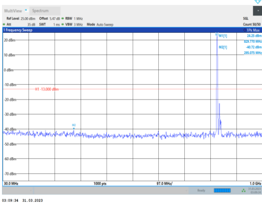
Band26-15MHz-16QAM-26915-1RB#0- Range1:30~1000MHz
