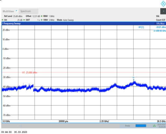
Band38-10MHz-16QAM-38200-1RB#0-Range3:3000~26500MHz
