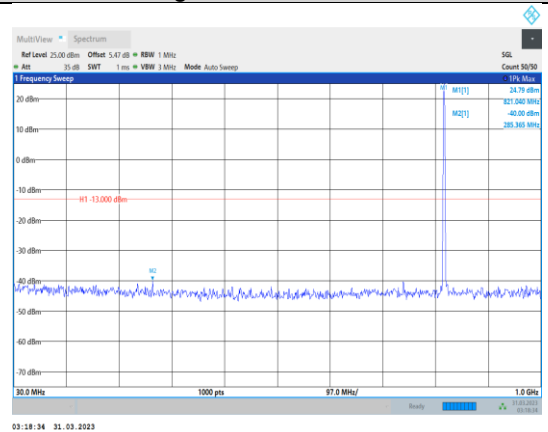
Band26-3MHz-64QAM-26775-1RB#0- Range1:30~1000MHz
