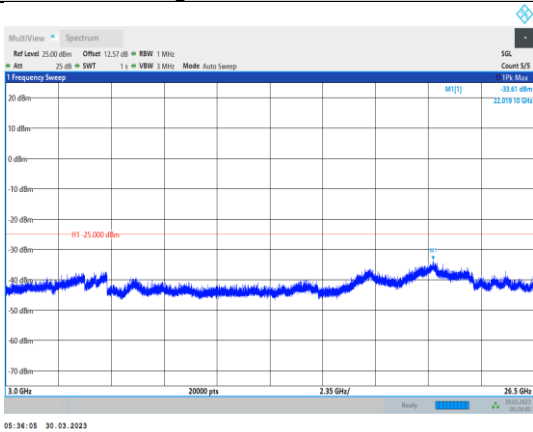
Band38-5MHz-16QAM-38000-1RB#0- Range3:3000~26500MHz
