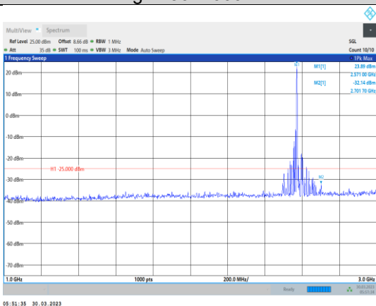
Band38-15MHz-QPSK-37825-1RB#0- Range2:1000~3000MHz
