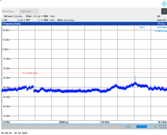
Band38-5MHz-64QAM-38225-1RB#0- Range3:3000~26500MHz
