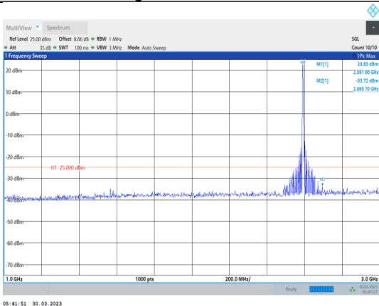
Band38-10MHz-QPSK-38000-1RB#0- Range2:1000~3000MHz
