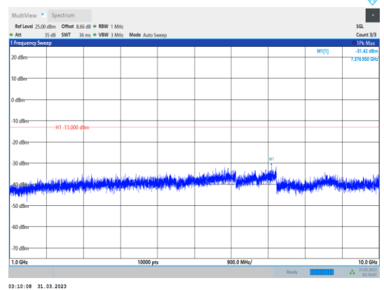
Band26-15MHz-64QAM-26915-1RB#0- Range2:1000~10000MHz
