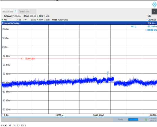
Band26-10MHz-QPSK-26740-1RB#0- Range2:1000~10000MHz
