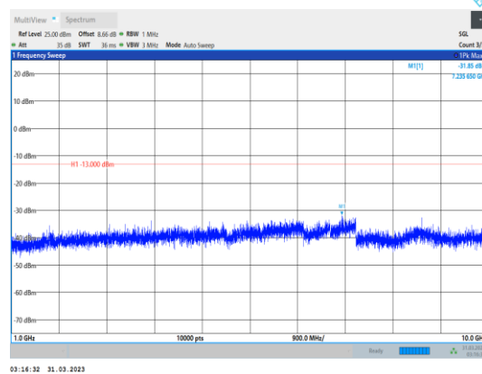
Band26-3MHz-QPSK-26740-1RB#0- Range2:1000~10000MHz
