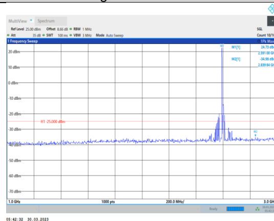
Band38-10MHz-16QAM-38000-1RB#0-Range2:1000~3000MHz
