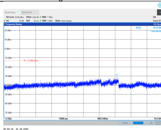
Band26-1.4MHz-64QAM-26783-1RB#0- Range2:1000~10000MHz
