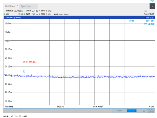
Band38-10MHz-64QAM-37800-1RB#0-Range1:30~1000MHz
