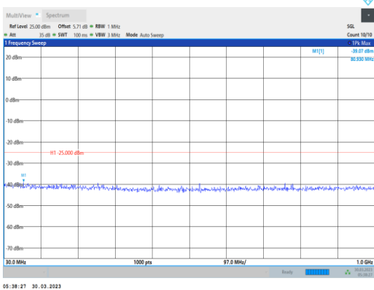
Band38-5MHz-64QAM-38225-1RB#0- Range1:30~1000MHz
