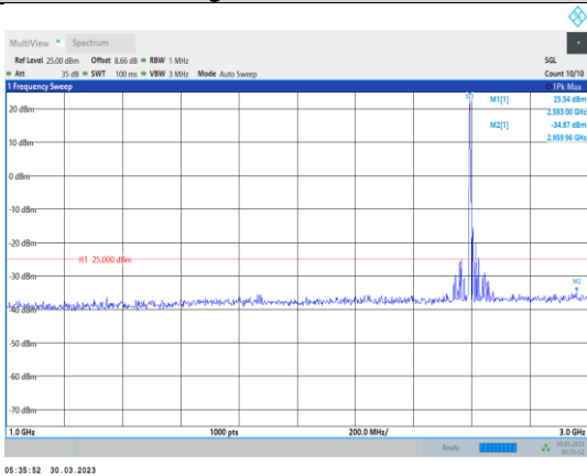
Band38-5MHz-16QAM-38000-1RB#0- Range2:1000~3000MHz
