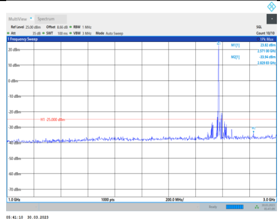
Band38-10MHz-64QAM-37800-1RB#0-Range2:1000~3000MHz
