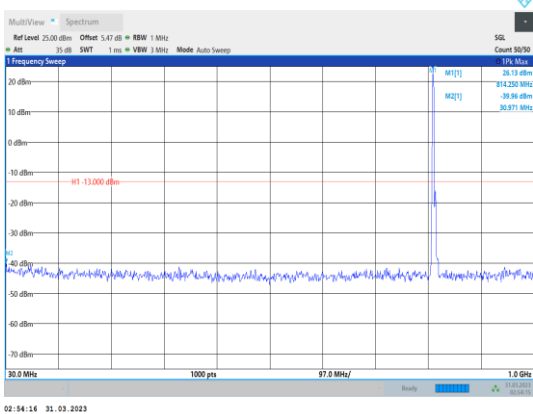
Band26-5MHz-QPSK-26715-1RB#0- Range1:30~1000MHz
