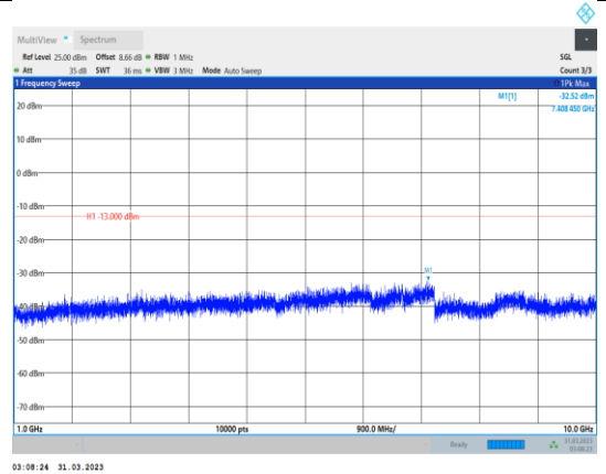
Band26-15MHz-16QAM-26865-1RB#0- Range2:1000~10000MHz
