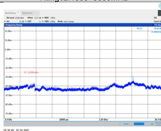
Band38-5MHz-64QAM-38000-1RB#0- Range3:3000~26500MHz
