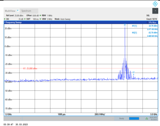
Band38-10MHz-QPSK-37800-1RB#0- Range2:1000~3000MHz
