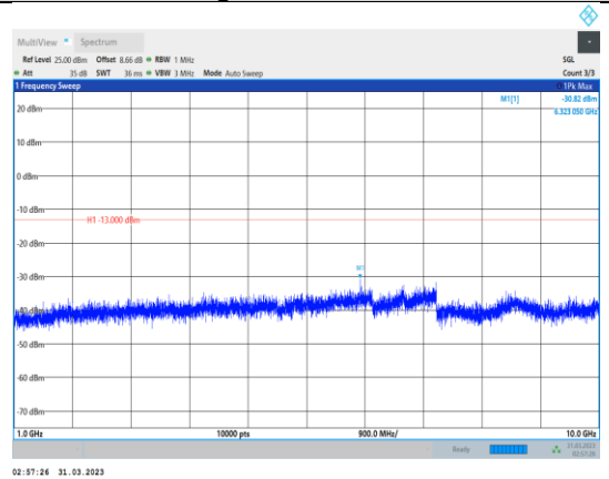
Band26-5MHz-16QAM-26765-1RB#0- Range2:1000~10000MHz
