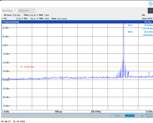
Band38-10MHz-16QAM-38200-1RB#0-Range2:1000~3000MHz
