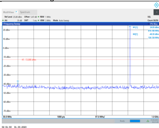
Band26-1.4MHz-64QAM-26740-1RB#0- Range1:30~1000MHz
