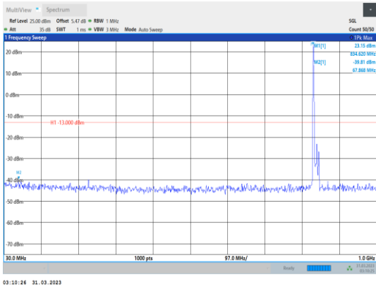
Band26-15MHz-QPSK-26965-1RB#0- Range1:30~1000MHz
