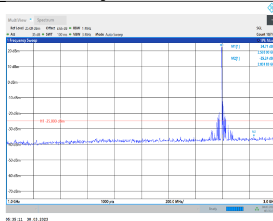
Band38-5MHz-QPSK-38000-1RB#0- Range2:1000~3000MHz
