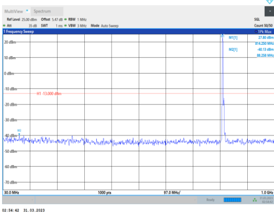
Band26-5MHz-16QAM-26715-1RB#0- Range1:30~1000MHz
