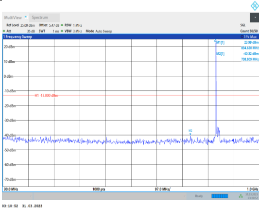
Band26-15MHz-16QAM-26965-1RB#0- Range1:30~1000MHz
