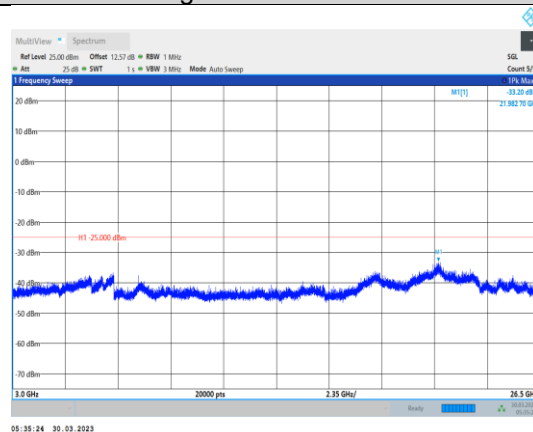
Band38-5MHz-QPSK-38000-1RB#0- Range3:3000~26500MHz
