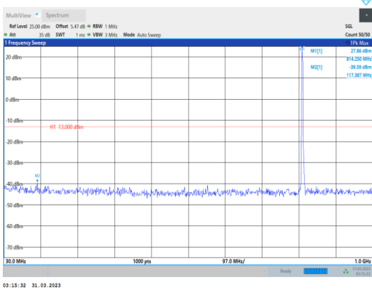
Band26-3MHz-16QAM-26705-1RB#0- Range1:30~1000MHz
