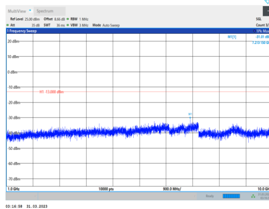
Band26-3MHz-16QAM-26740-1RB#0- Range2:1000~10000MHz
