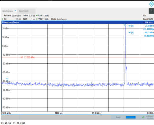
Band26-10MHz-16QAM-26740-1RB#0- Range1:30~1000MHz
