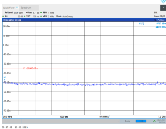
Band38-5MHz-QPSK-38225-1RB#0- Range1:30~1000MHz
