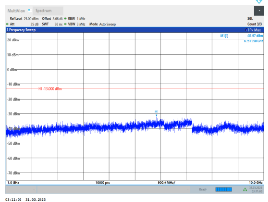
Band26-15MHz-16QAM-26965-1RB#0- Range2:1000~10000MHz
