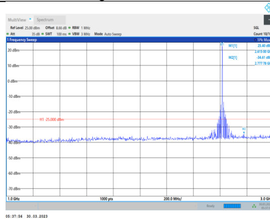
Band38-5MHz-16QAM-38225-1RB#0- Range2:1000~3000MHz
