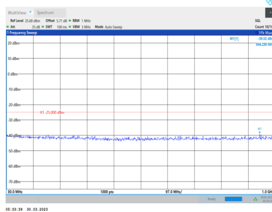
Band38-5MHz-16QAM-37775-1RB#0- Range1:30~1000MHz
