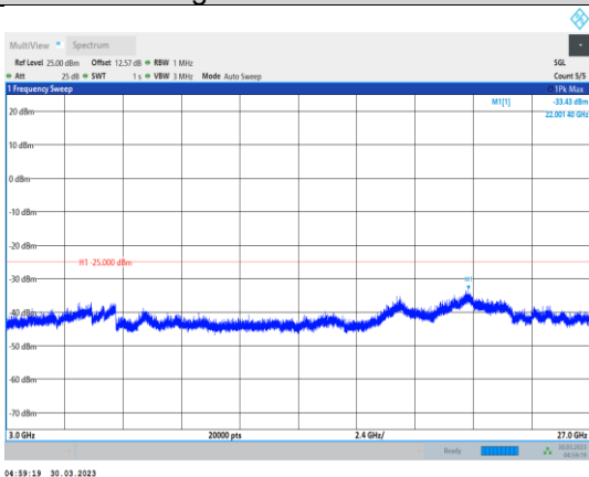
Band41-5MHz-64QAM-41565-1RB#0- Range3:3000~27000MHz
