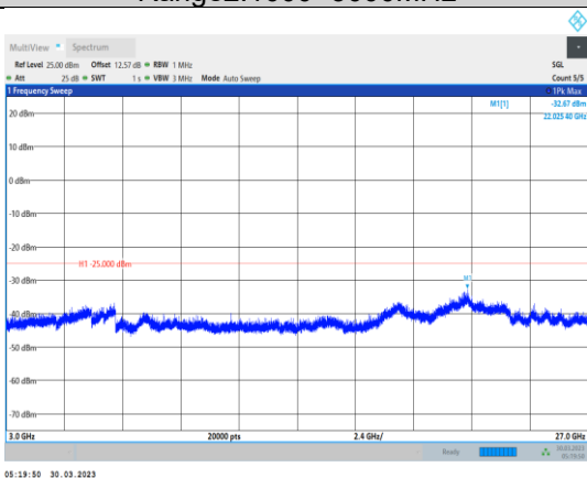
Band41-15MHz-16QAM-40620-1RB#0- Range3:3000~27000MHz
