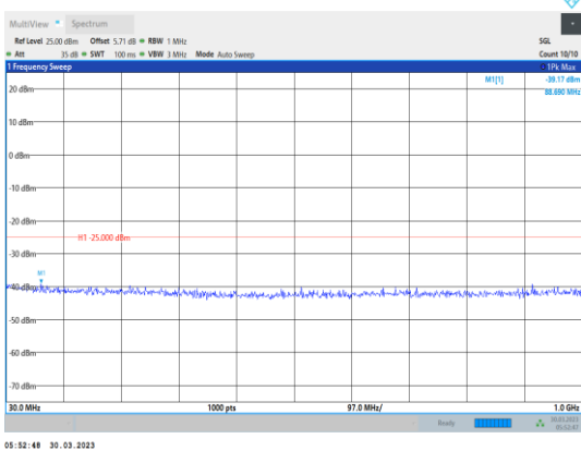
Band38-15MHz-64QAM-37825-1RB#0-Range1:30~1000MHz
