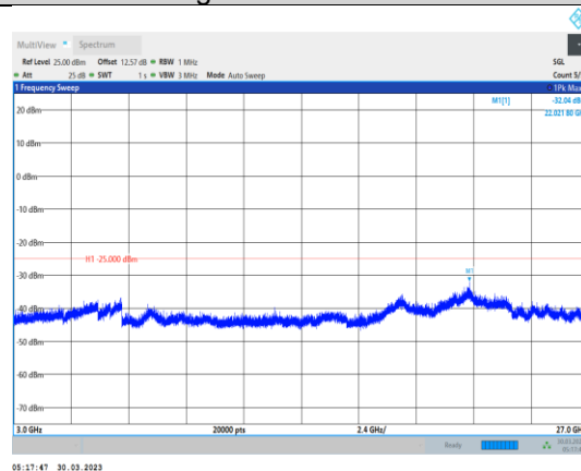
Band41-15MHz-16QAM-39725-1RB#0- Range3:3000~27000MHz
