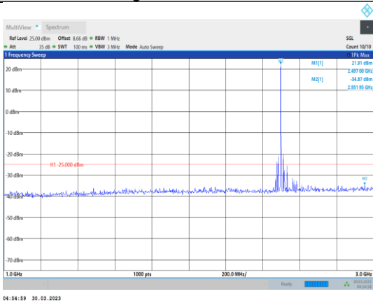
Band41-5MHz-64QAM-39675-1RB#0- Range2:1000~3000MHz
