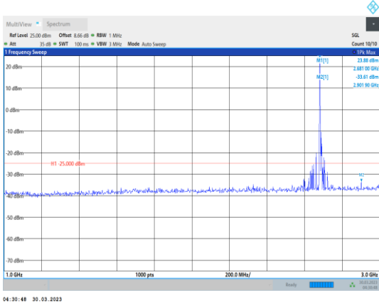
Band41-10MHz-16QAM-41540-1RB#0- Range2:1000~3000MHz
