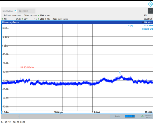
Band41-5MHz-64QAM-39675-1RB#0- Range3:3000~27000MHz
