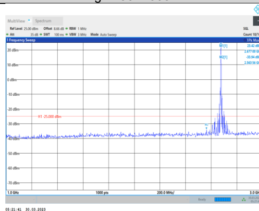
Band41-15MHz-16QAM-41515-1RB#0- Range2:1000~3000MHz
