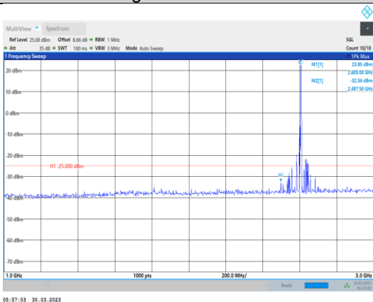
Band38-15MHz-64QAM-38175-1RB#0- Range2:1000~3000MHz
