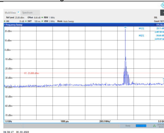
Band41-5MHz-16QAM-39675-1RB#0- Range2:1000~3000MHz
