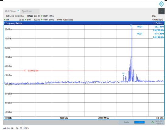
Band41-15MHz-64QAM-40620-1RB#0- Range2:1000~3000MHz
