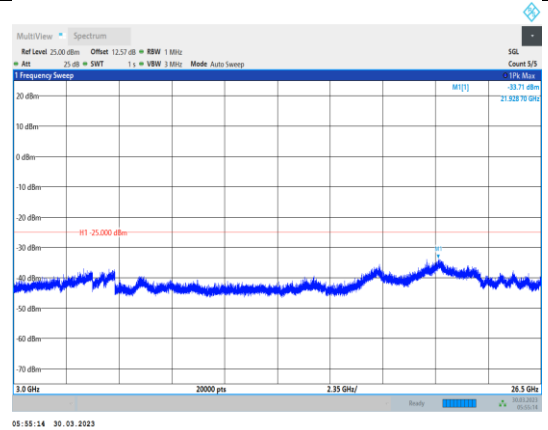
Band38-15MHz-64QAM-38000-1RB#0-Range3:3000~26500MHz
