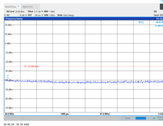
Band38-15MHz-16QAM-37825-1RB#0- Range1:30~1000MHz
