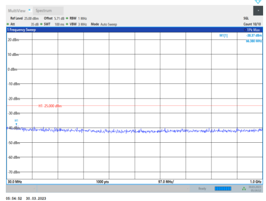
Band38-15MHz-64QAM-38000-1RB#0-Range1:30~1000MHz
