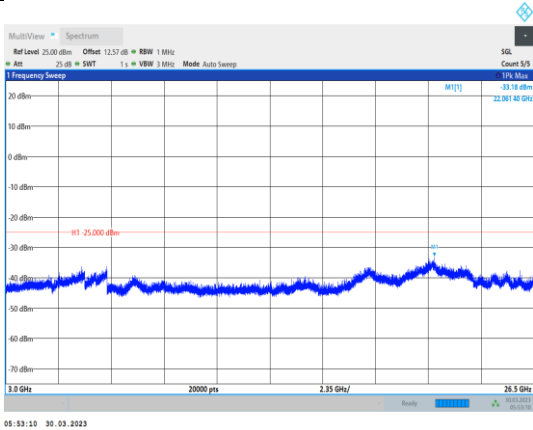
Band38-15MHz-64QAM-37825-1RB#0-Range3:3000~26500MHz
