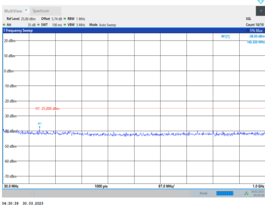
Band41-10MHz-16QAM-41540-1RB#0- Range1:30~1000MHz
