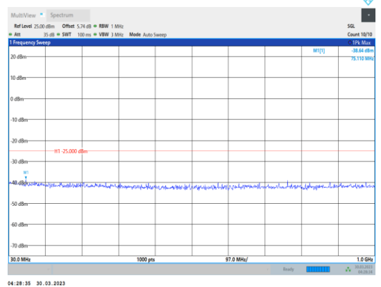
Band41-10MHz-16QAM-40620-1RB#0- Range1:30~1000MHz
