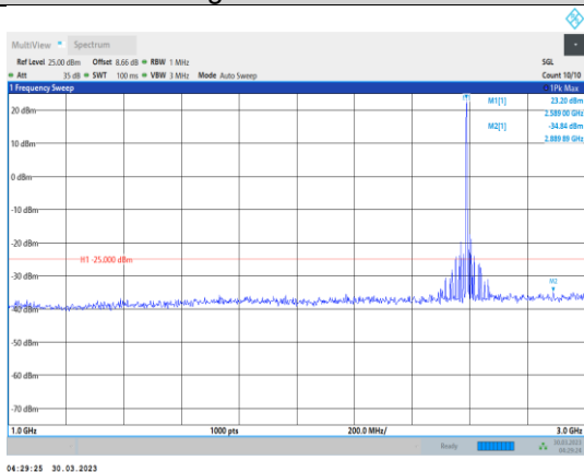
Band41-10MHz-64QAM-40620-1RB#0- Range2:1000~3000MHz
