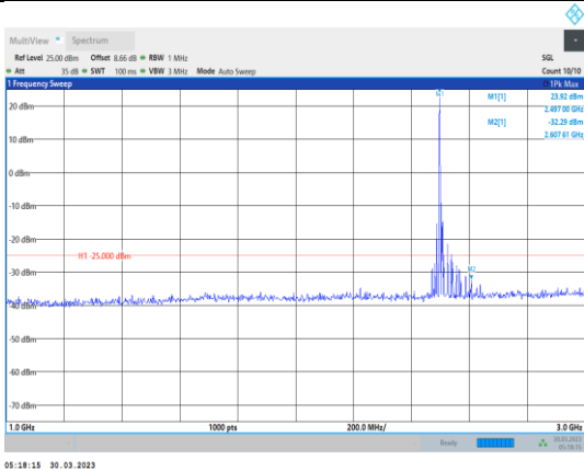
Band41-15MHz-64QAM-39725-1RB#0- Range2:1000~3000MHz
