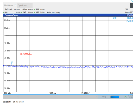
Band41-15MHz-QPSK-40620-1RB#0- Range1:30~1000MHz
