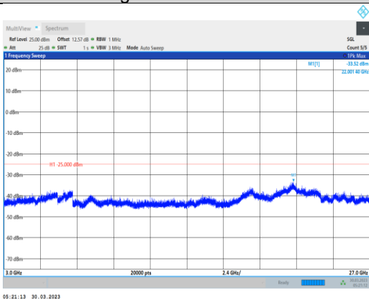
Band41-15MHz-QPSK-41515-1RB#0- Range3:3000~27000MHz
