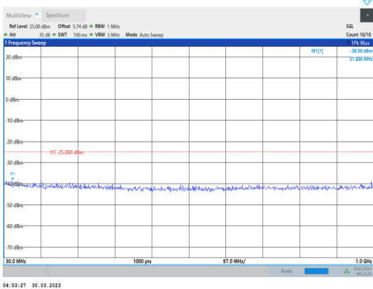
Band41-5MHz-QPSK-39675-1RB#0- Range1:30~1000MHz
