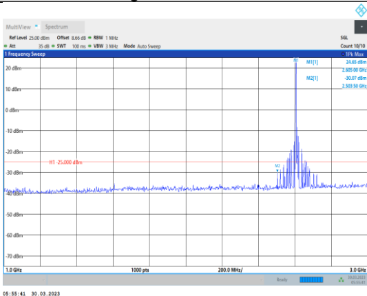
Band38-15MHz-QPSK-38175-1RB#0- Range2:1000~3000MHz
