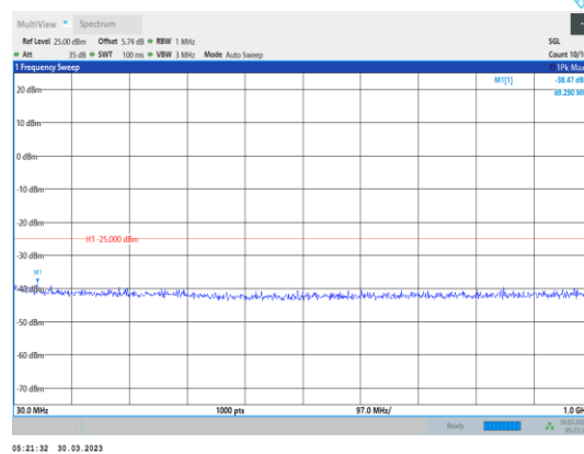
Band41-15MHz-16QAM-41515-1RB#0- Range1:30~1000MHz
