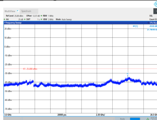
Band38-20MHz-64QAM-37850-1RB#0- Range3:3000~26500MHz
