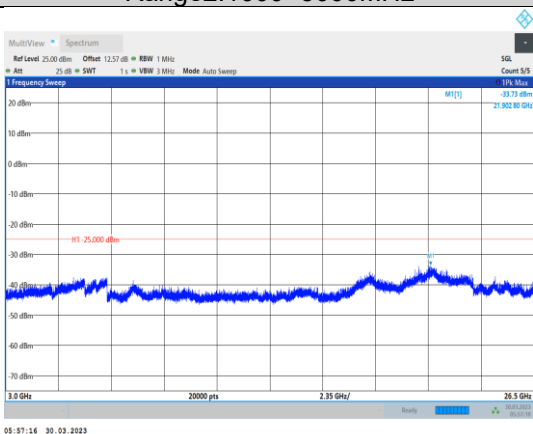
Band38-15MHz-64QAM-38175-1RB#0- Range3:3000~26500MHz
