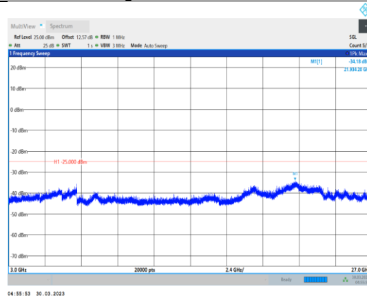
Band41-5MHz-QPSK-40620-1RB#0- Range3:3000~27000MHz
