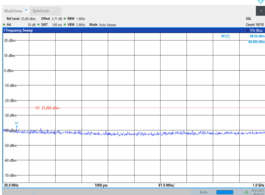
Band38-20MHz-16QAM-38150-1RB#0- Range1:30~1000MHz
