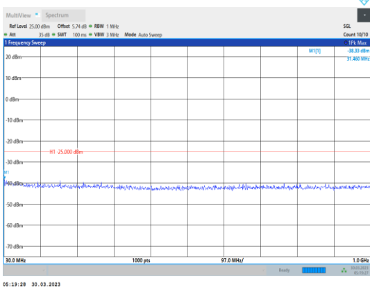
Band41-15MHz-16QAM-40620-1RB#0- Range1:30~1000MHz
