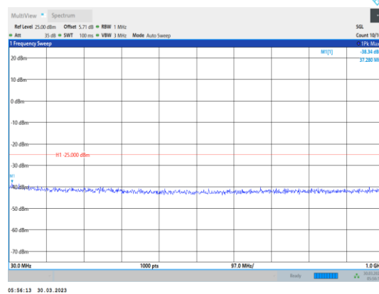
Band38-15MHz-16QAM-38175-1RB#0- Range1:30~1000MHz
