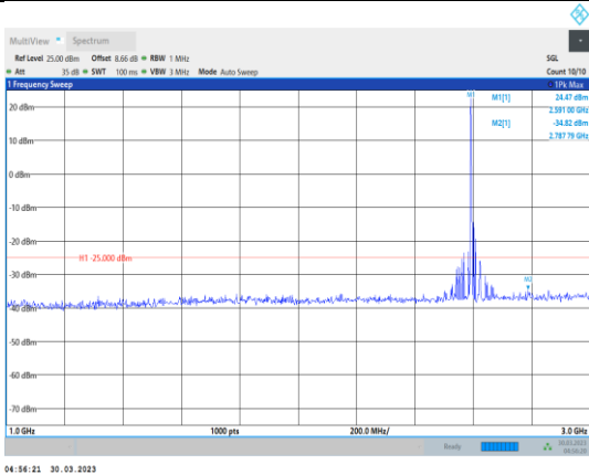
Band41-5MHz-16QAM-40620-1RB#0- Range2:1000~3000MHz
