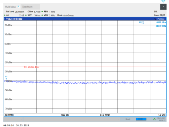
Band41-5MHz-16QAM-41565-1RB#0- Range1:30~1000MHz
