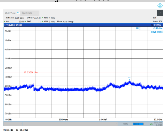
Band41-10MHz-64QAM-41540-1RB#0- Range3:3000~27000MHz
