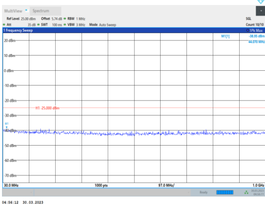
Band41-5MHz-16QAM-40620-1RB#0- Range1:30~1000MHz
