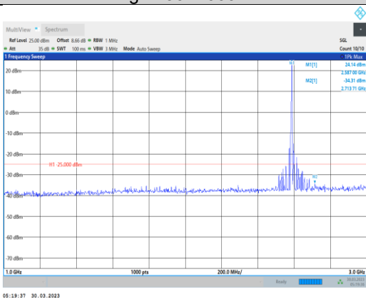
Band41-15MHz-16QAM-40620-1RB#0- Range2:1000~3000MHz
