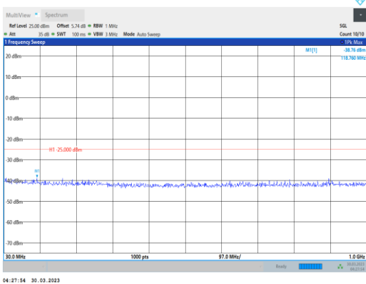
Band41-10MHz-QPSK-40620-1RB#0- Range1:30~1000MHz
