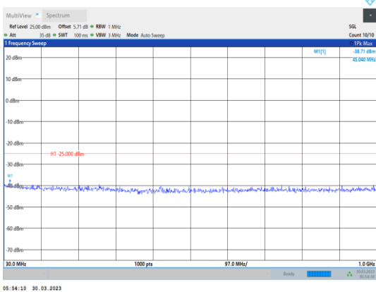
Band38-15MHz-16QAM-38000-1RB#0- Range1:30~1000MHz
