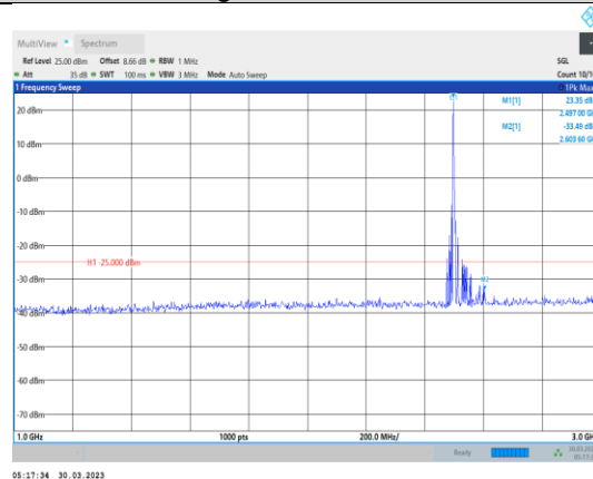
Band41-15MHz-16QAM-39725-1RB#0- Range2:1000~3000MHz
