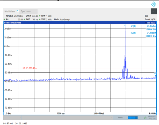
Band41-5MHz-64QAM-40620-1RB#0- Range2:1000~3000MHz
