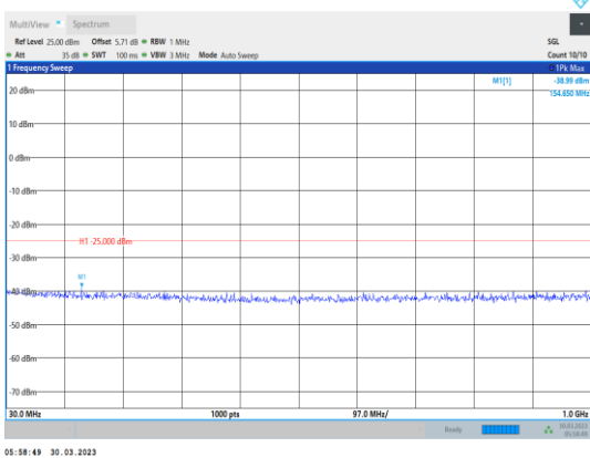
Band38-20MHz-16QAM-37850-1RB#0- Range1:30~1000MHz
