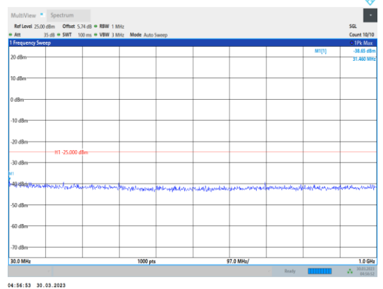
Band41-5MHz-64QAM-40620-1RB#0- Range1:30~1000MHz
