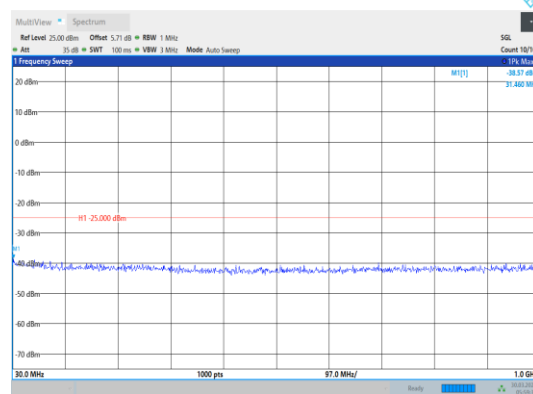
Band38-20MHz-64QAM-37850-1RB#0- Range1:30~1000MHz
