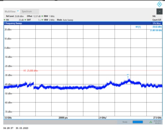
Band41-10MHz-16QAM-40620-1RB#0- Range3:3000~27000MHz
