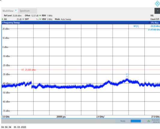
Band41-5MHz-16QAM-40620-1RB#0- Range3:3000~27000MHz
