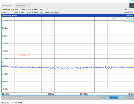
Band41-15MHz-QPSK-41515-1RB#0- Range1:30~1000MHz
