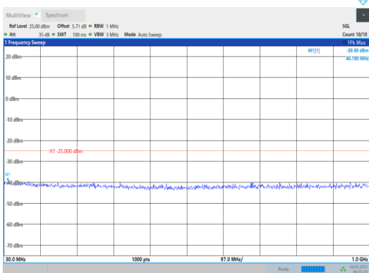
Band38-20MHz-64QAM-38000-1RB#0- Range1:30~1000MHz
