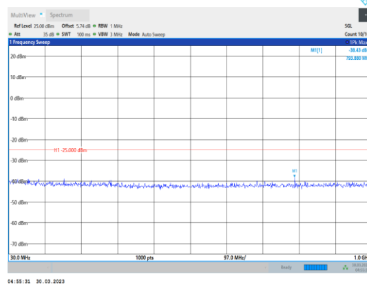
Band41-5MHz-QPSK-40620-1RB#0- Range1:30~1000MHz
