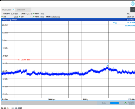
Band41-10MHz-QPSK-40620-1RB#0- Range3:3000~27000MHz
