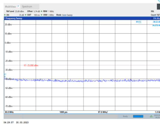
Band41-10MHz-QPSK-41540-1RB#0- Range1:30~1000MHz
