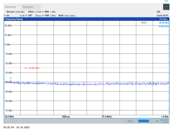
Band41-15MHz-64QAM-40620-1RB#0- Range1:30~1000MHz
