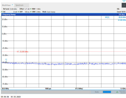
Band38-15MHz-64QAM-38175-1RB#0- Range1:30~1000MHz
