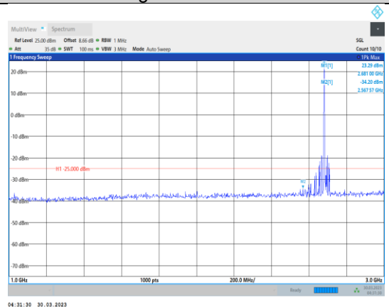
Band41-10MHz-64QAM-41540-1RB#0- Range2:1000~3000MHz
