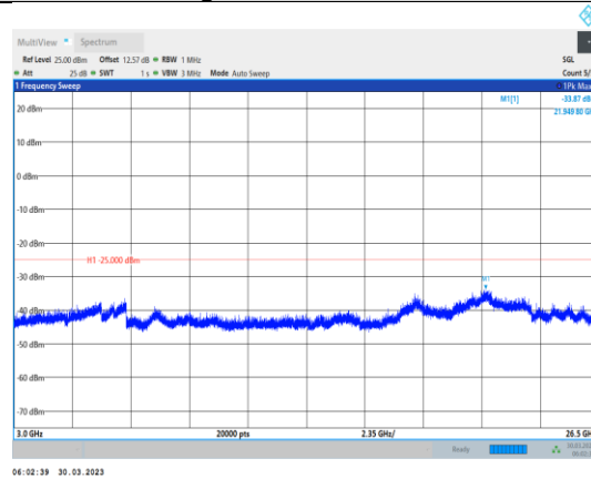
Band38-20MHz-QPSK-38150-1RB#0- Range3:3000~26500MHz
