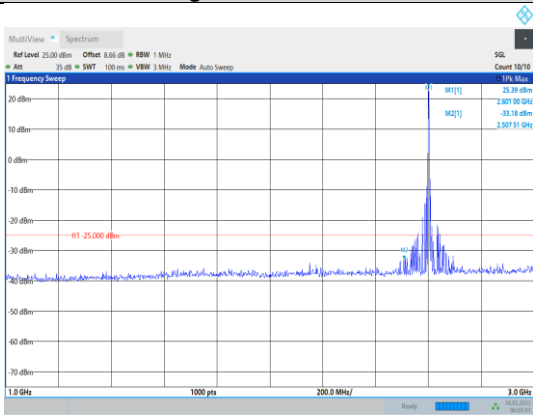
Band38-20MHz-16QAM-38150-1RB#0- Range2:1000~3000MHz
