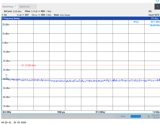
Band41-10MHz-16QAM-39700-1RB#0- Range1:30~1000MHz
