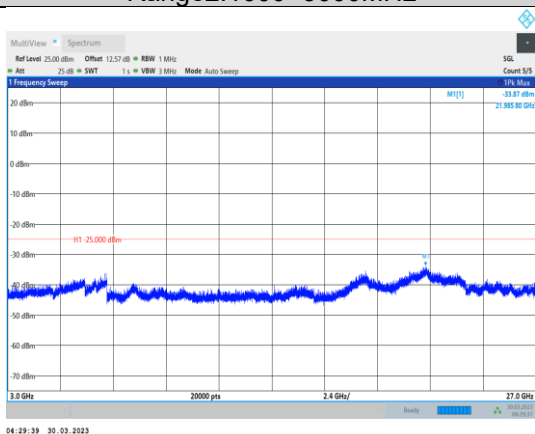
Band41-10MHz-64QAM-40620-1RB#0- Range3:3000~27000MHz
