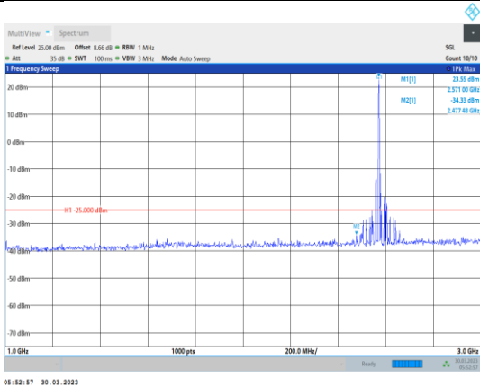
Band38-15MHz-64QAM-37825-1RB#0-Range2:1000~3000MHz
