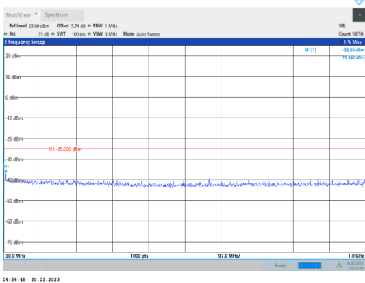
Band41-5MHz-64QAM-39675-1RB#0- Range1:30~1000MHz
