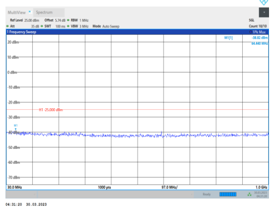
Band41-10MHz-64QAM-41540-1RB#0- Range1:30~1000MHz
