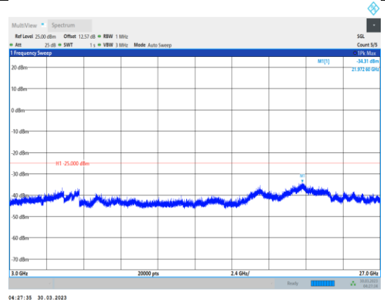
Band41-10MHz-64QAM-39700-1RB#0- Range3:3000~27000MHz
