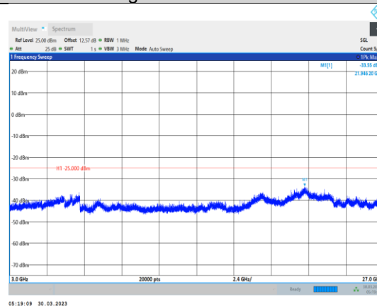
Band41-15MHz-QPSK-40620-1RB#0- Range3:3000~27000MHz
