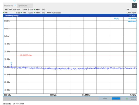
Band38-20MHz-16QAM-38000-1RB#0- Range1:30~1000MHz
