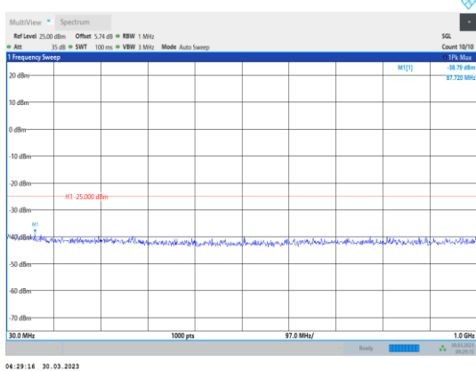
Band41-10MHz-64QAM-40620-1RB#0- Range1:30~1000MHz
