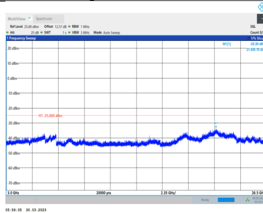
Band38-15MHz-16QAM-38175-1RB#0- Range3:3000~26500MHz
