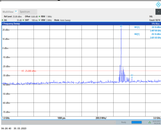
Band41-10MHz-16QAM-39700-1RB#0- Range2:1000~3000MHz
