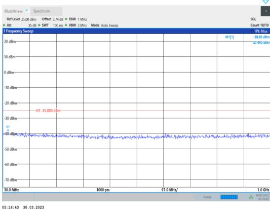
Band41-15MHz-QPSK-39725-1RB#0- Range1:30~1000MHz
