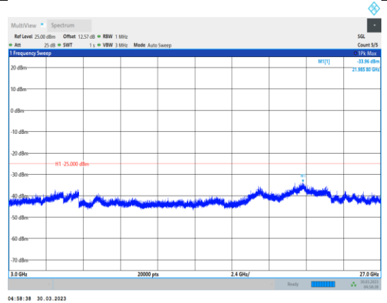
Band41-5MHz-16QAM-41565-1RB#0- Range3:3000~27000MHz
