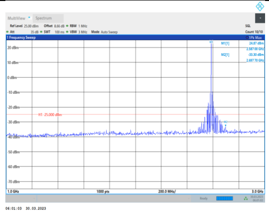
Band38-20MHz-16QAM-38000-1RB#0- Range2:1000~3000MHz
