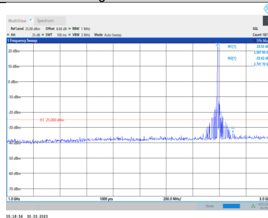
Band41-15MHz-QPSK-40620-1RB#0- Range2:1000~3000MHz
