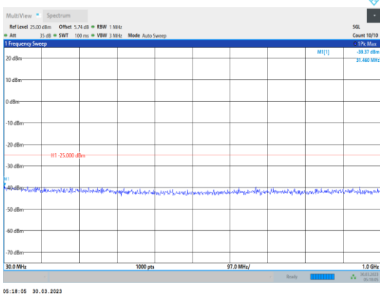
Band41-15MHz-64QAM-39725-1RB#0- Range1:30~1000MHz
