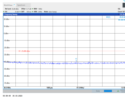
Band38-20MHz-QPSK-37850-1RB#0- Range1:30~1000MHz
