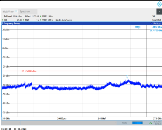
Band41-15MHz-64QAM-39725-1RB#0- Range3:3000~27000MHz
