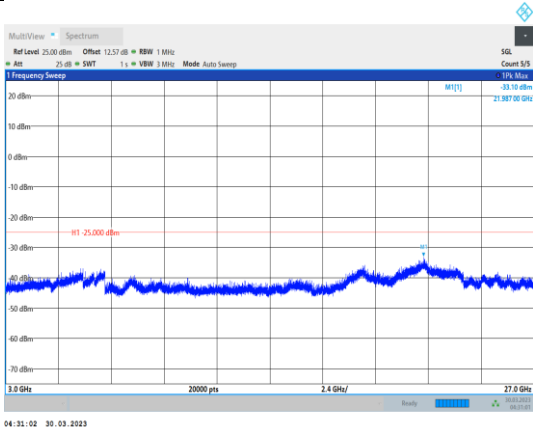
Band41-10MHz-16QAM-41540-1RB#0- Range3:3000~27000MHz
