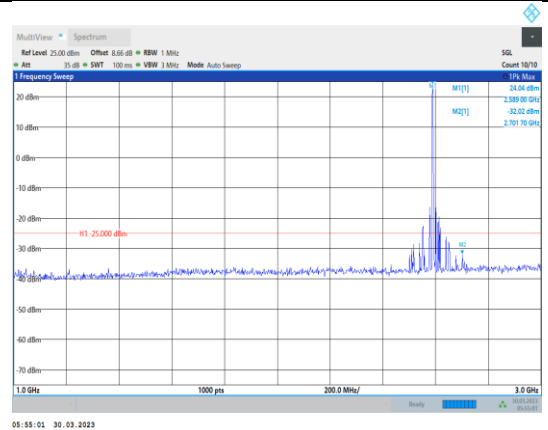
Band38-15MHz-64QAM-38000-1RB#0-Range2:1000~3000MHz
