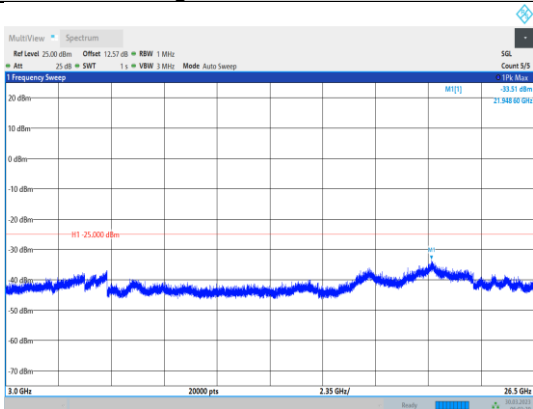
Band38-20MHz-16QAM-38150-1RB#0- Range3:3000~26500MHz
