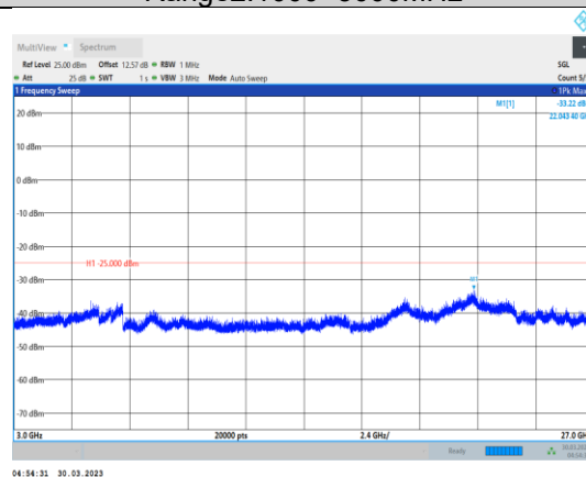
Band41-5MHz-16QAM-39675-1RB#0- Range3:3000~27000MHz
