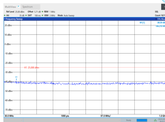
Band38-20MHz-64QAM-38150-1RB#0- Range1:30~1000MHz
