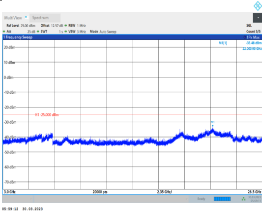
Band38-20MHz-16QAM-37850-1RB#0- Range3:3000~26500MHz
