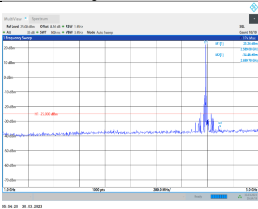
Band38-15MHz-16QAM-38000-1RB#0- Range2:1000~3000MHz
