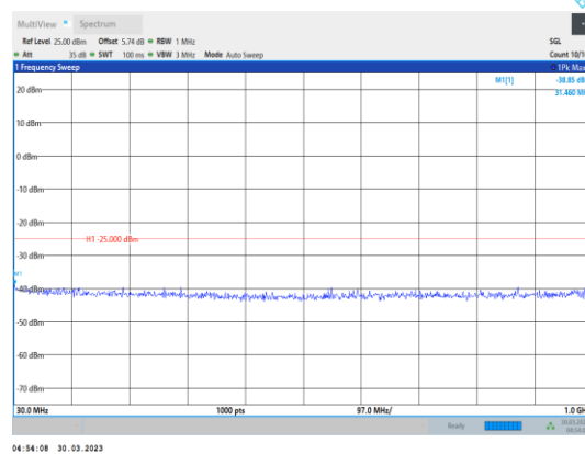
Band41-5MHz-16QAM-39675-1RB#0- Range1:30~1000MHz
