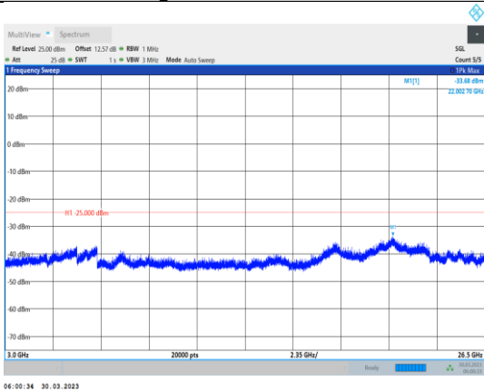
Band38-20MHz-QPSK-38000-1RB#0- Range3:3000~26500MHz
