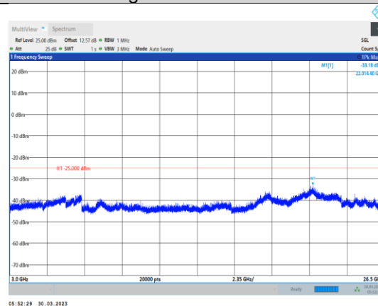
Band38-15MHz-16QAM-37825-1RB#0- Range3:3000~26500MHz
