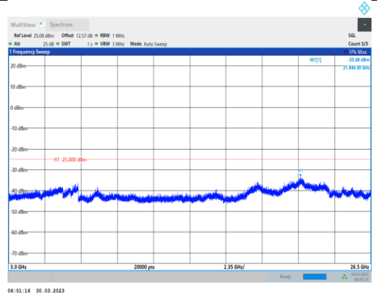
Band38-20MHz-16QAM-38000-1RB#0- Range3:3000~26500MHz
