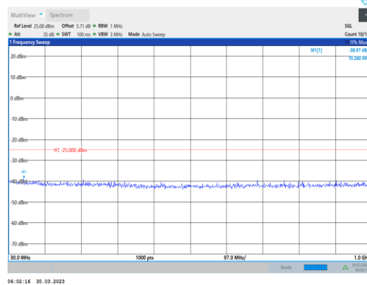
Band38-20MHz-QPSK-38150-1RB#0- Range1:30~1000MHz
