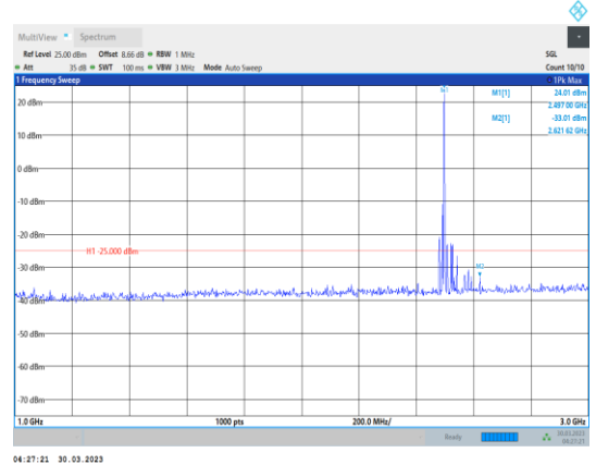
Band41-10MHz-64QAM-39700-1RB#0- Range2:1000~3000MHz
