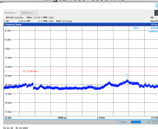
Band41-15MHz-16QAM-41515-1RB#0- Range3:3000~27000MHz
