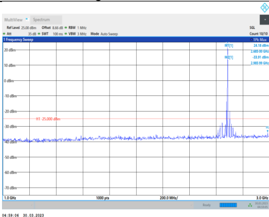
Band41-5MHz-64QAM-41565-1RB#0- Range2:1000~3000MHz
