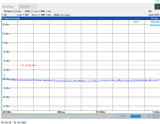
Band38-15MHz-QPSK-38175-1RB#0- Range1:30~1000MHz
