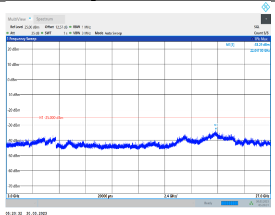
Band41-15MHz-64QAM-40620-1RB#0- Range3:3000~27000MHz
