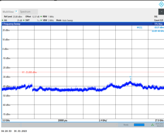
Band41-10MHz-16QAM-39700-1RB#0- Range3:3000~27000MHz
