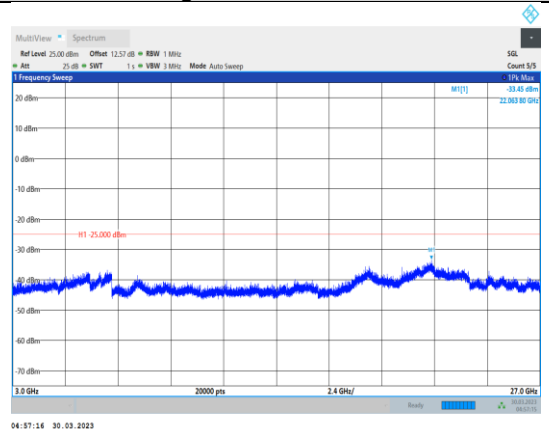
Band41-5MHz-64QAM-40620-1RB#0- Range3:3000~27000MHz
