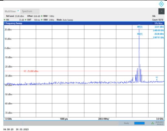
Band41-5MHz-16QAM-41565-1RB#0- Range2:1000~3000MHz
