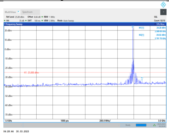
Band41-10MHz-16QAM-40620-1RB#0- Range2:1000~3000MHz
