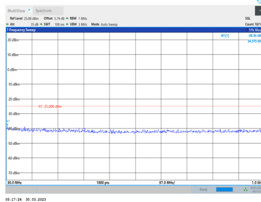
Band41-15MHz-16QAM-39725-1RB#0- Range1:30~1000MHz
