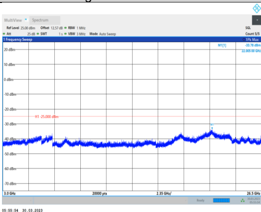
Band38-15MHz-QPSK-38175-1RB#0- Range3:3000~26500MHz
