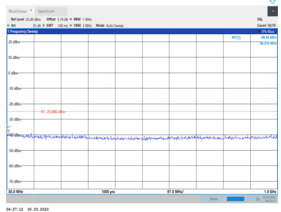
Band41-10MHz-64QAM-39700-1RB#0- Range1:30~1000MHz
