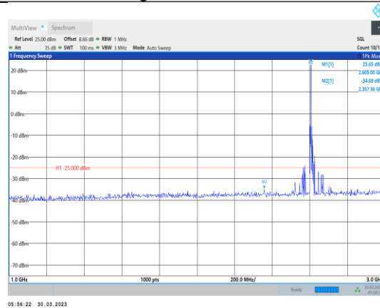
Band38-15MHz-16QAM-38175-1RB#0- Range2:1000~3000MHz
