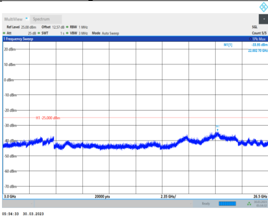
Band38-15MHz-16QAM-38000-1RB#0- Range3:3000~26500MHz
