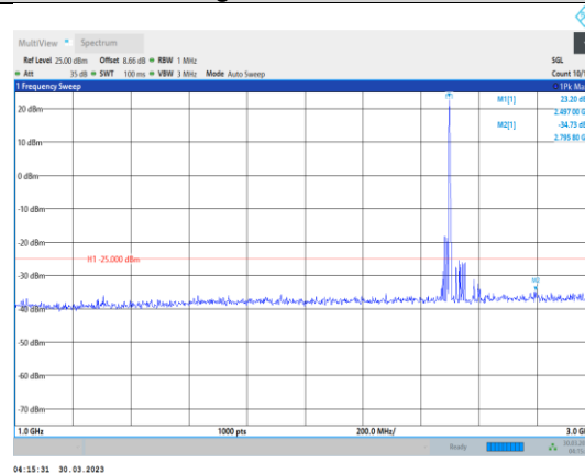
Band41-20MHz-64QAM-39750-1RB#0- Range2:1000~3000MHz
