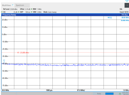
Band41-20MHz-16QAM-39750-1RB#0-Range1:30~1000MHz
