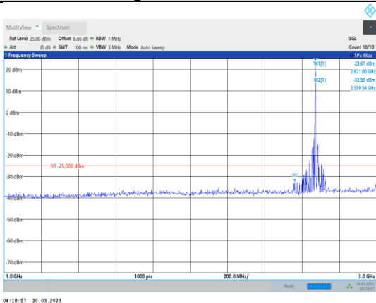
Band41-20MHz-16QAM-41490-1RB#0- Range2:1000~3000MHz
