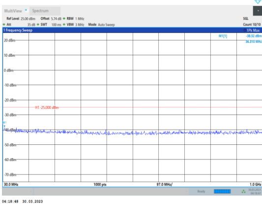
Band41-20MHz-16QAM-41490-1RB#0- Range1:30~1000MHz
