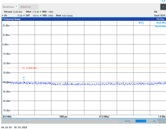
Band41-20MHz-QPSK-40620-1RB#0- Range1:30~1000MHz
