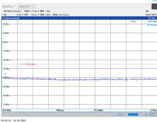
Band41-15MHz-64QAM-41515-1RB#0- Range1:30~1000MHz
