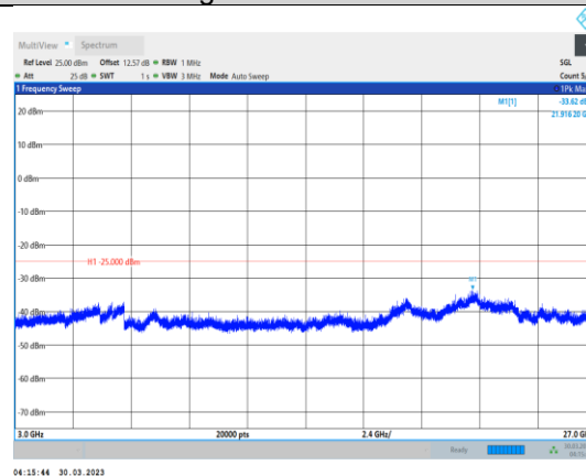
Band41-20MHz-64QAM-39750-1RB#0- Range3:3000~27000MHz
