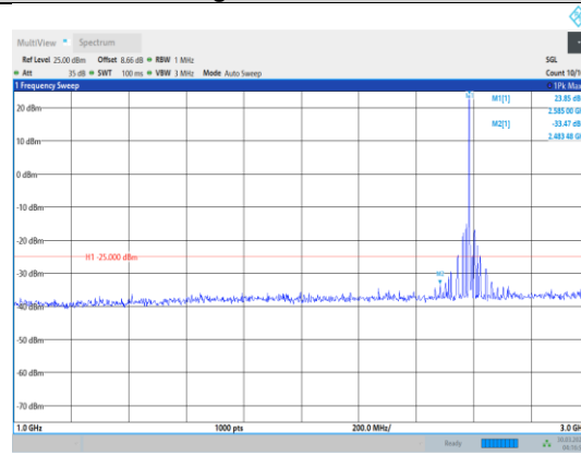
Band41-20MHz-16QAM-40620-1RB#0-Range2:1000~3000MHz
