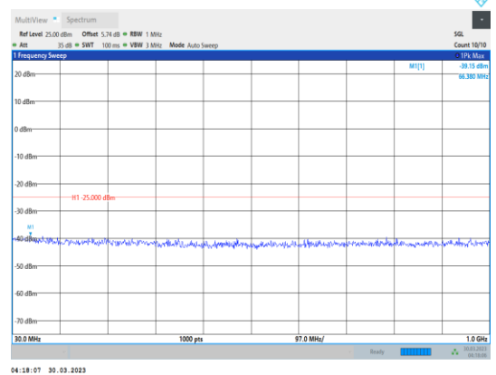
Band41-20MHz-QPSK-41490-1RB#0- Range1:30~1000MHz
