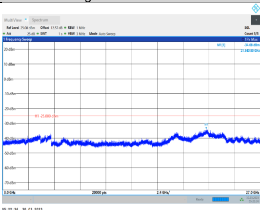
Band41-15MHz-64QAM-41515-1RB#0- Range3:3000~27000MHz
