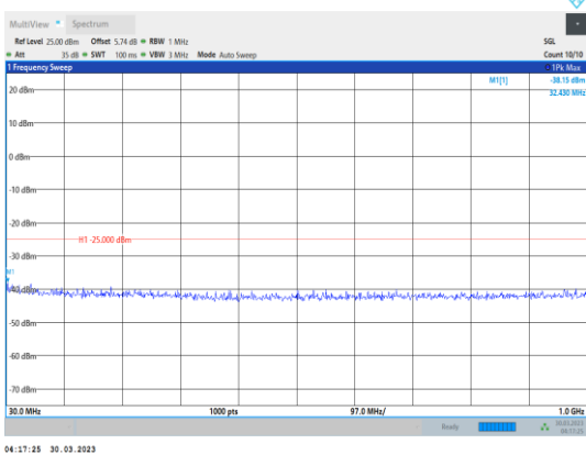
Band41-20MHz-64QAM-40620-1RB#0- Range1:30~1000MHz
