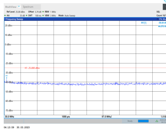
Band41-20MHz-QPSK-39750-1RB#0- Range1:30~1000MHz
