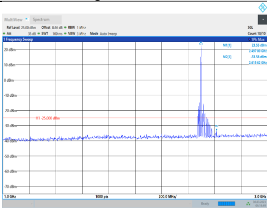
Band41-20MHz-16QAM-39750-1RB#0-Range2:1000~3000MHz
