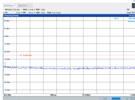
Band41-20MHz-16QAM-40620-1RB#0-Range1:30~1000MHz
