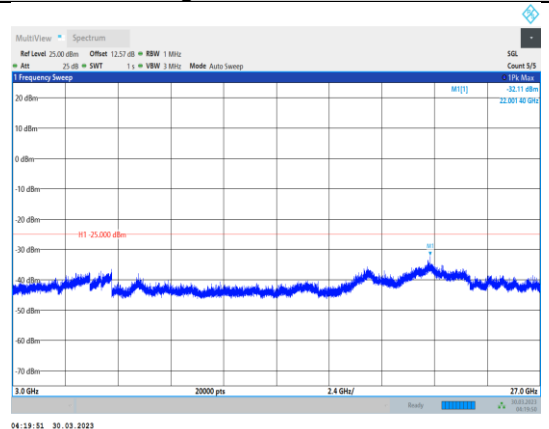
Band41-20MHz-64QAM-41490-1RB#0- Range3:3000~27000MHz
