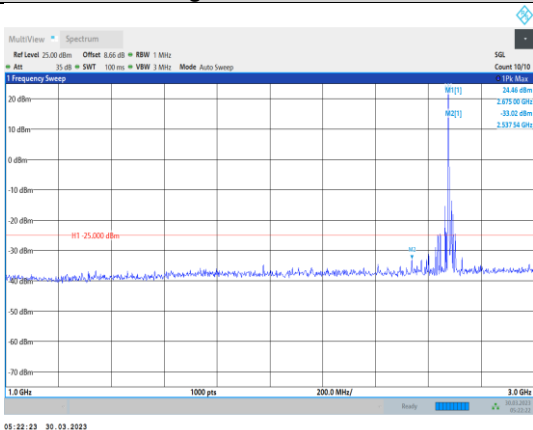
Band41-15MHz-64QAM-41515-1RB#0- Range2:1000~3000MHz
