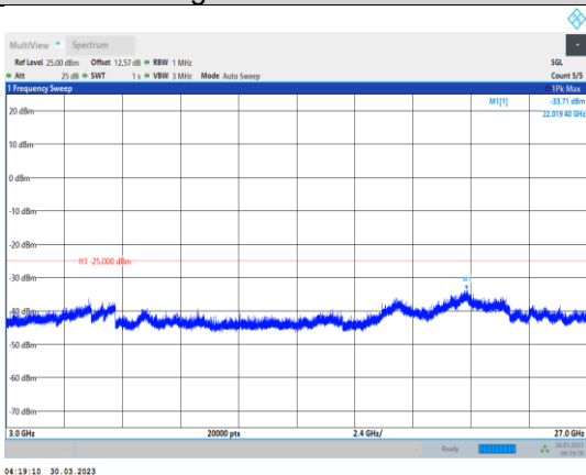
Band41-20MHz-16QAM-41490-1RB#0- Range3:3000~27000MHz
