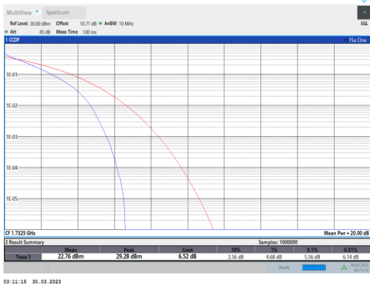
Band4-5MHz-QPSK-20175-25RB#0
