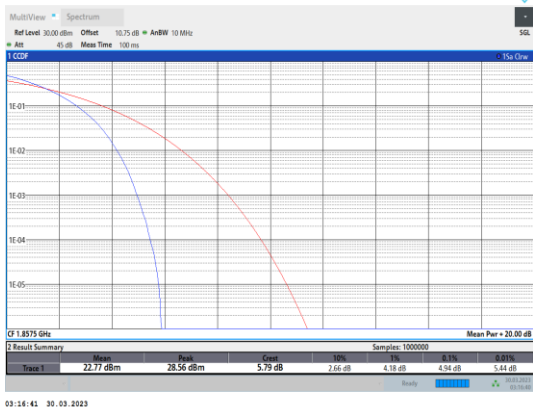
Band2-15MHz-QPSK-18675-75RB#0
