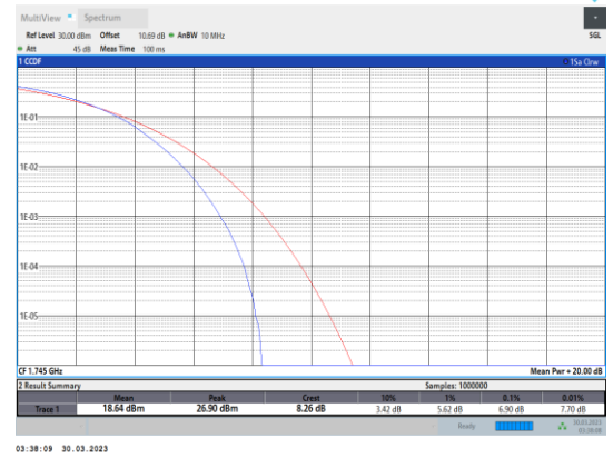
Band4-20MHz-64QAM-20300-100RB#0
