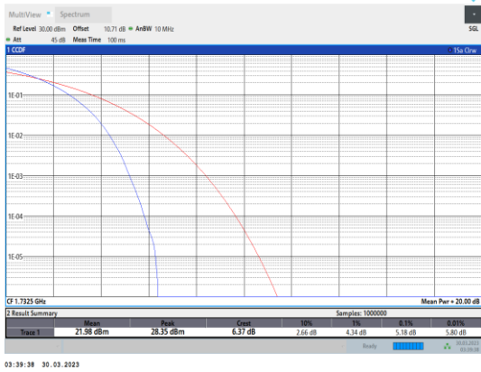
Band4-15MHz-QPSK-20175-75RB#0
