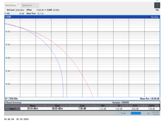
Band4-3MHz-64QAM-20385-15RB#0
