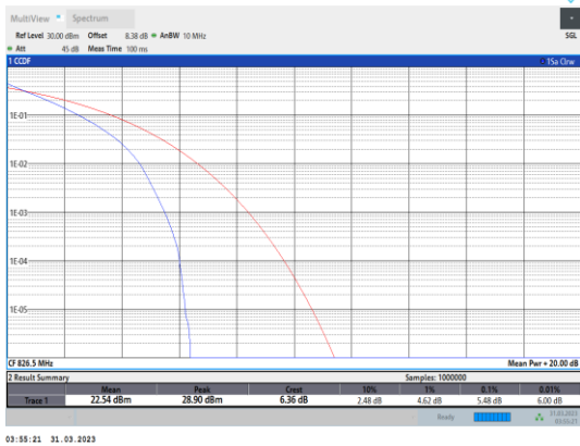
Band5-5MHz-QPSK-20425-25RB#0
