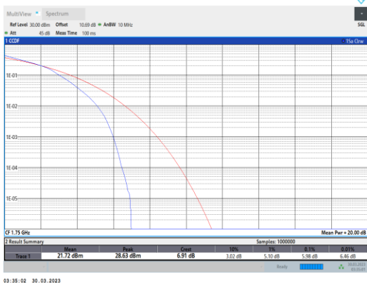
Band4-10MHz-16QAM-20350-50RB#0
