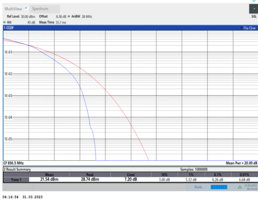
Band5-3MHz-16QAM-20525-15RB#0
