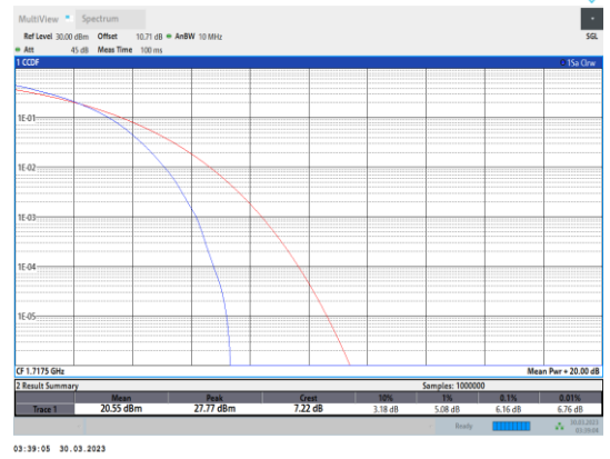
Band4-15MHz-16QAM-20025-75RB#0
