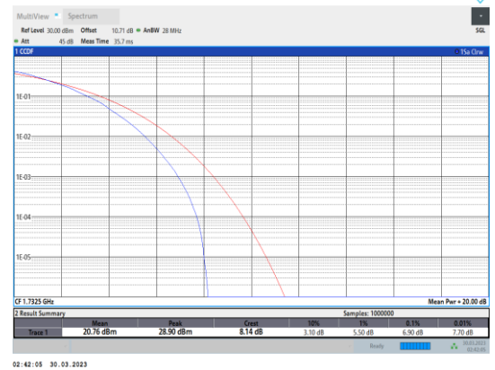
Band4-3MHz-64QAM-20175-15RB#0
