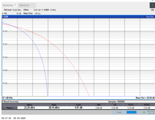
Band2-15MHz-QPSK-18900-75RB#0
