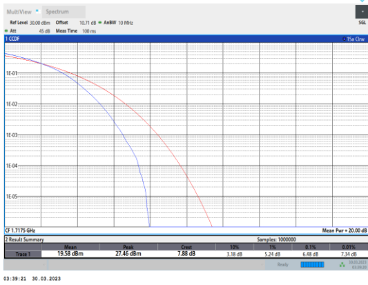
Band4-15MHz-64QAM-20025-75RB#0
