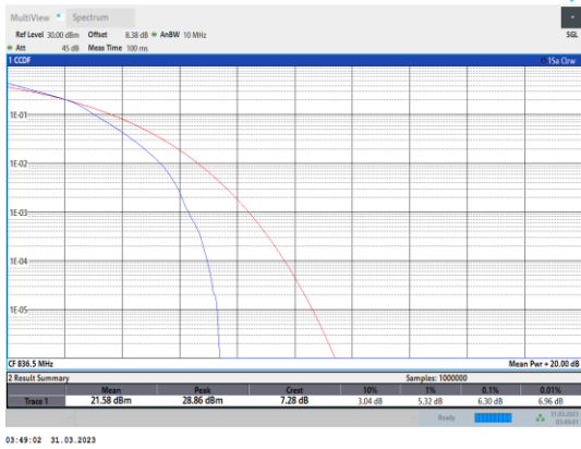
Band5-10MHz-16QAM-20525-50RB#0
