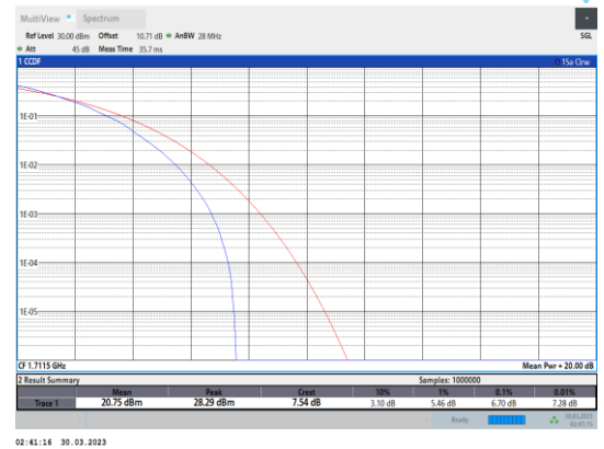
Band4-3MHz-64QAM-19965-15RB#0
