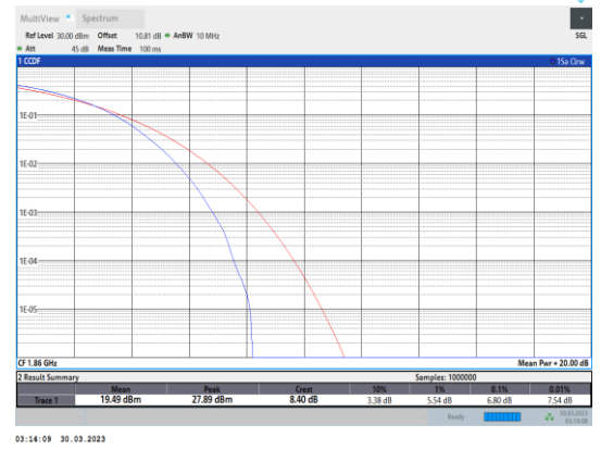
Band2-20MHz-64QAM-18700-100RB#0
