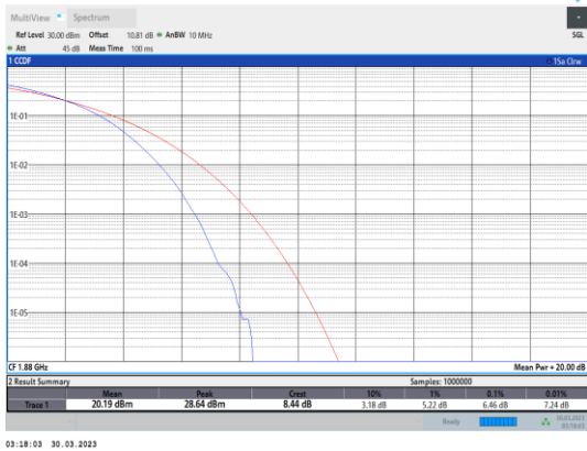
Band2-15MHz-64QAM-18900-75RB#0
