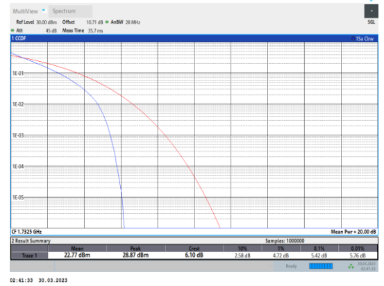
Band4-3MHz-QPSK-20175-15RB#0
