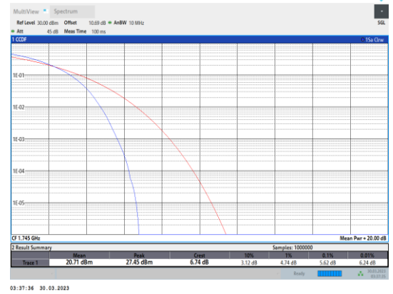
Band4-20MHz-QPSK-20300-100RB#0
