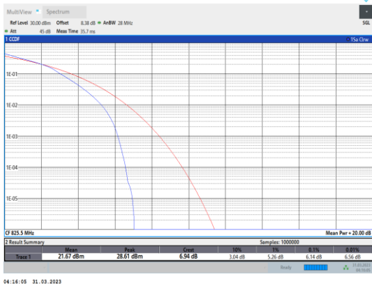
Band5-3MHz-16QAM-20415-15RB#0
