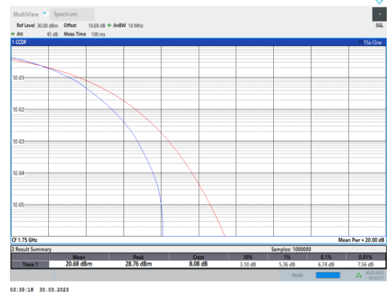
Band4-10MHz-64QAM-20350-50RB#0
