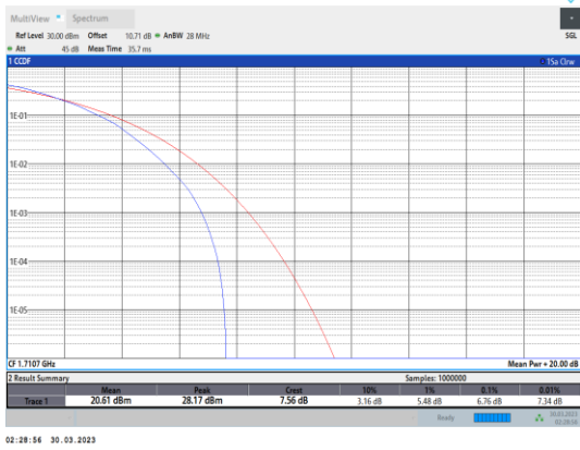
Band4-1.4MHz-64QAM-19957-6RB#0
