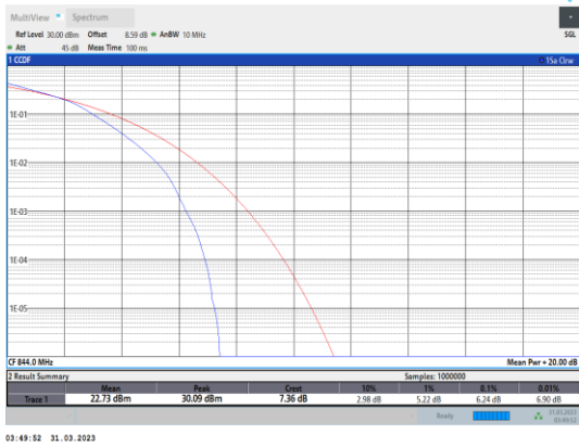
Band5-10MHz-16QAM-20600-50RB#0
