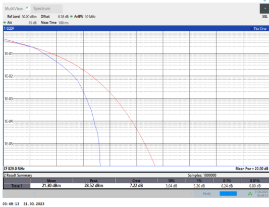
Band5-10MHz-16QAM-20450-50RB#0
