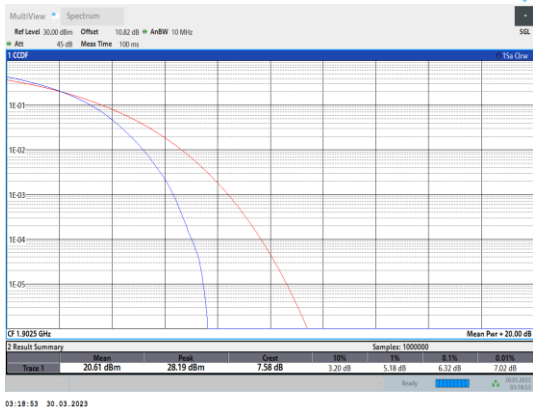
Band2-15MHz-64QAM-19125-75RB#0
