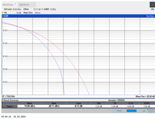
Band4-15MHz-64QAM-20175-75RB#0
