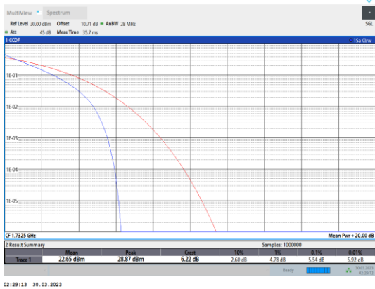
Band4-1.4MHz-QPSK-20175-6RB#0
