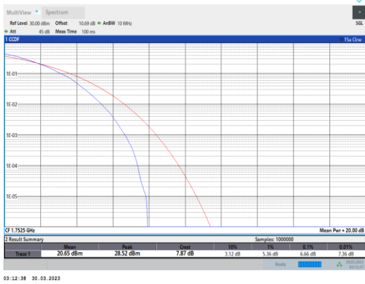
Band4-5MHz-64QAM-20375-25RB#0
