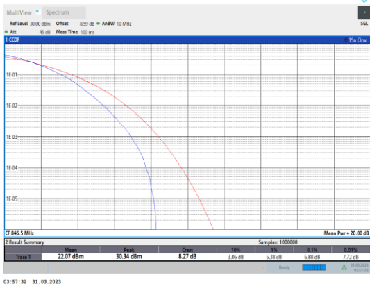
Band5-5MHz-64QAM-20625-25RB#0
