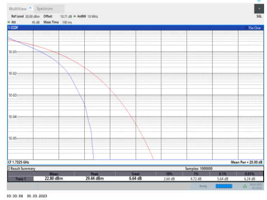
Band4-10MHz-QPSK-20175-50RB#0
