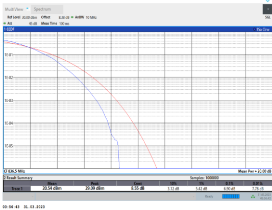
Band5-5MHz-64QAM-20525-25RB#0
