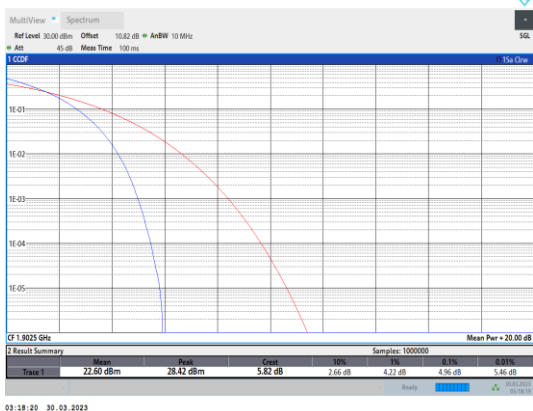
Band2-15MHz-QPSK-19125-75RB#0
