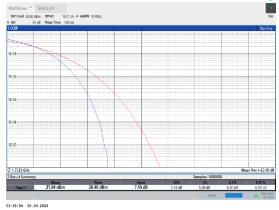
Band4-15MHz-16QAM-20175-75RB#0
