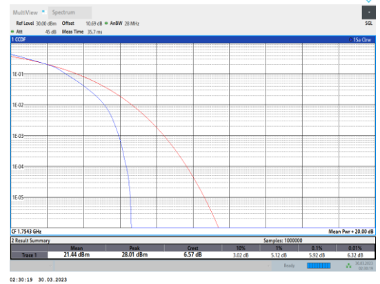
Band4-1.4MHz-16QAM-20393-6RB#0
