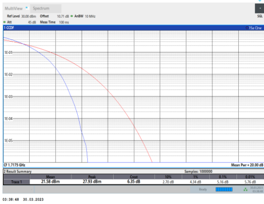
Band4-15MHz-QPSK-20025-75RB#0
