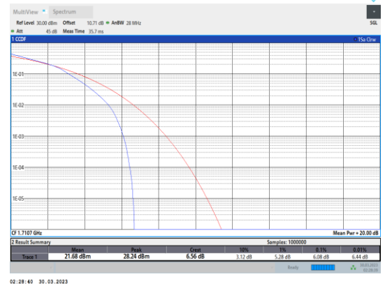
Band4-1.4MHz-16QAM-19957-6RB#0
