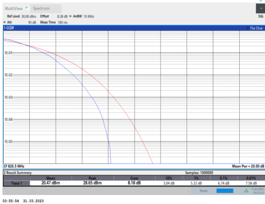
Band5-5MHz-64QAM-20425-25RB#0
