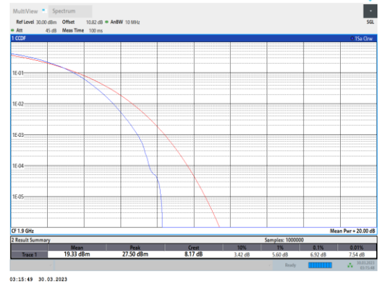
Band2-20MHz-64QAM-19100-100RB#0
