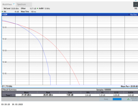
Band4-10MHz-16QAM-20000-50RB#0
