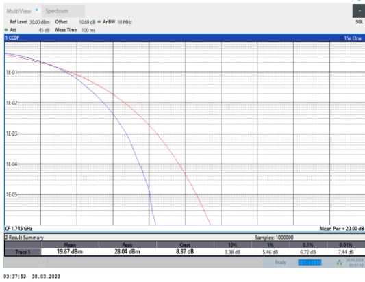
Band4-20MHz-16QAM-20300-100RB#0
