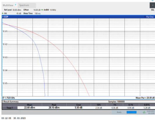
Band4-5MHz-QPSK-20375-25RB#0
