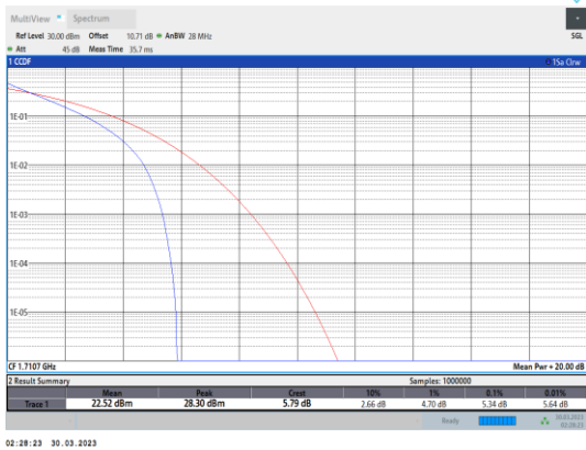
Band4-1.4MHz-QPSK-19957-6RB#0
