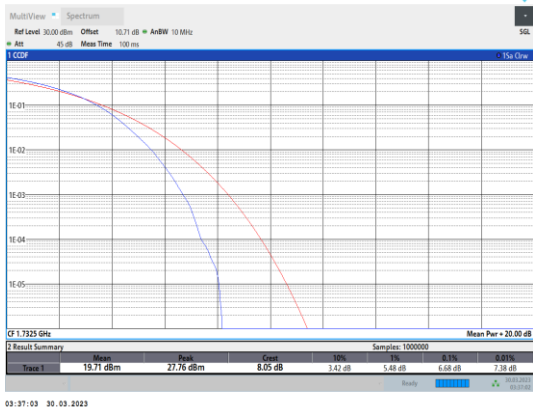
Band4-20MHz-16QAM-20175-100RB#0
