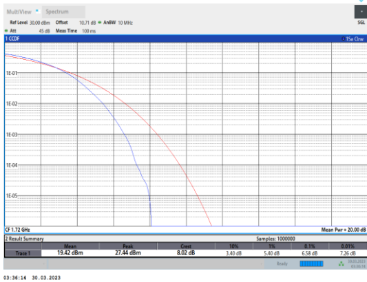
Band4-20MHz-16QAM-20050-100RB#0
