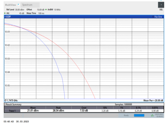
Band4-15MHz-16QAM-20325-75RB#0
