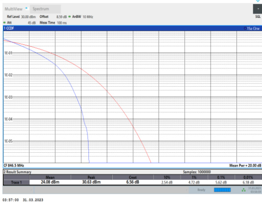
Band5-5MHz-QPSK-20625-25RB#0
