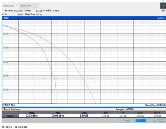
Band5-5MHz-QPSK-20525-25RB#0
