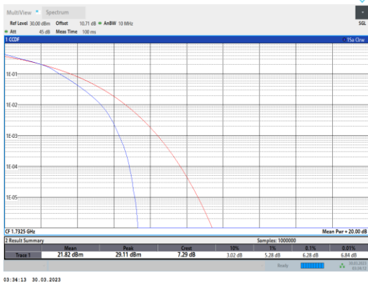
Band4-10MHz-16QAM-20175-50RB#0
