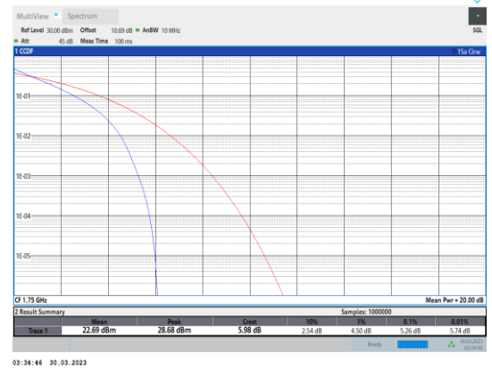
Band4-10MHz-QPSK-20350-50RB#0
