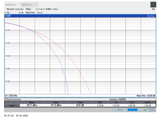
Band4-20MHz-64QAM-20175-100RB#0
