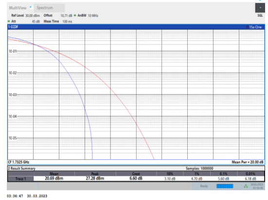
Band4-20MHz-QPSK-20175-100RB#0
