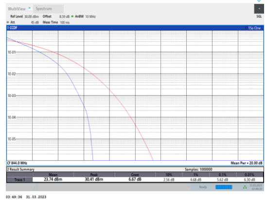
Band5-10MHz-QPSK-20600-50RB#0
