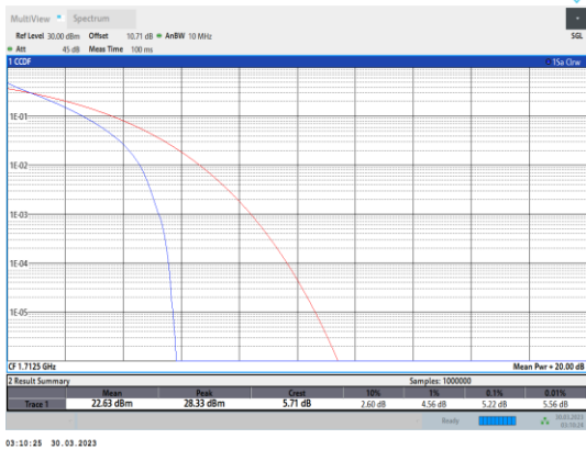
Band4-5MHz-QPSK-19975-25RB#0
