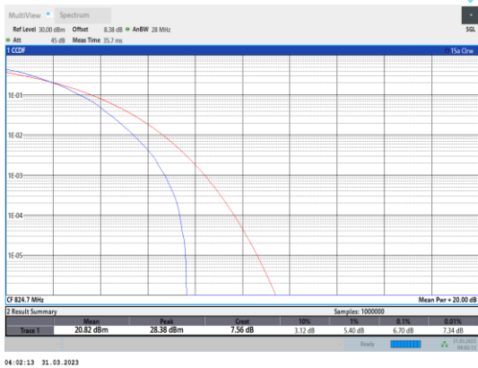
Band5-1.4MHz-64QAM-20407-6RB#0
