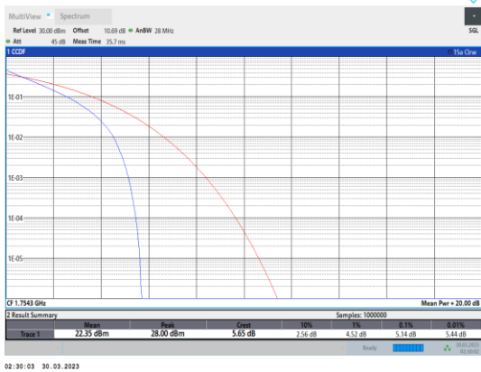
Band4-1.4MHz-QPSK-20393-6RB#0
