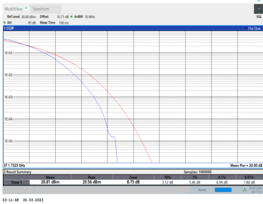
Band4-5MHz-64QAM-20175-25RB#0
