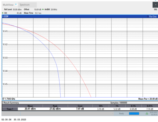
Band4-1.4MHz-64QAM-20393-6RB#0
