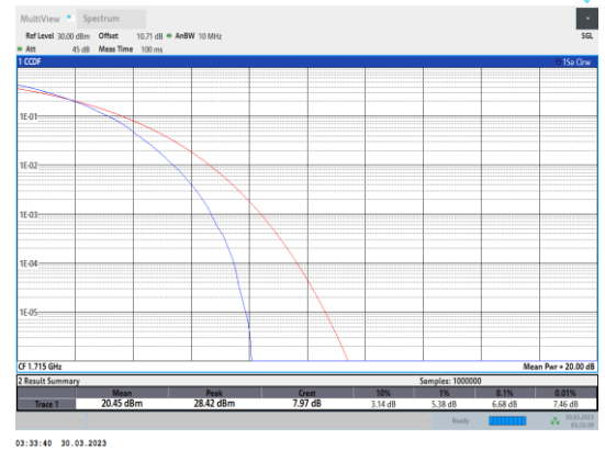
Band4-10MHz-64QAM-20000-50RB#0
