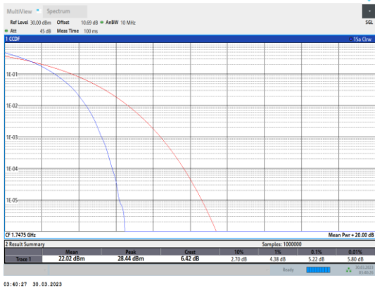
Band4-15MHz-QPSK-20325-75RB#0
