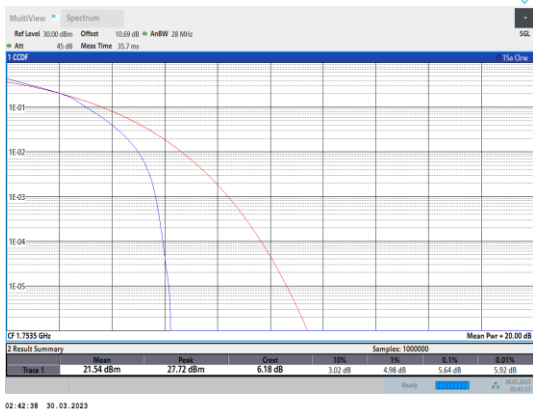
Band4-3MHz-16QAM-20385-15RB#0
