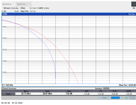
Band4-1.4MHz-64QAM-20175-6RB#0
