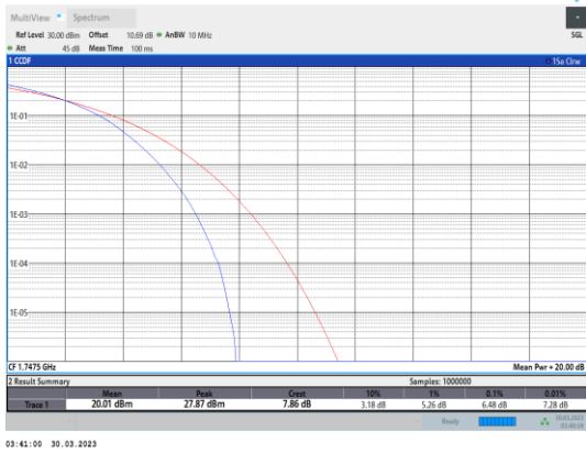
Band4-15MHz-64QAM-20325-75RB#0
