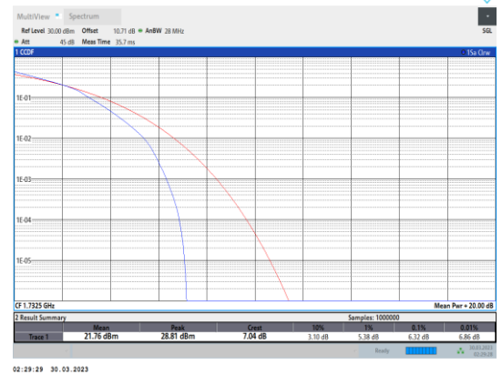
Band4-1.4MHz-16QAM-20175-6RB#0
