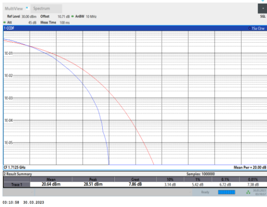
Band4-5MHz-64QAM-19975-25RB#0
