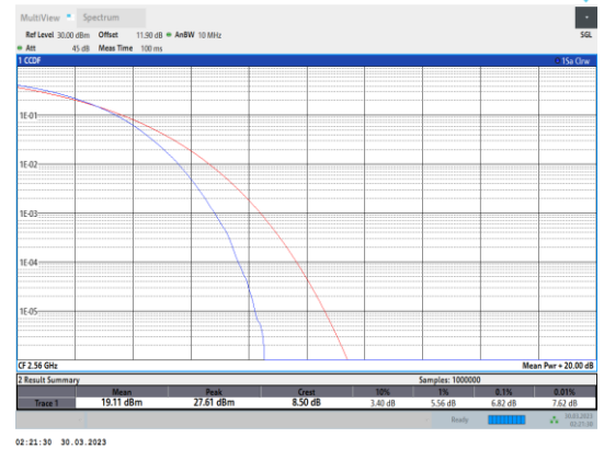
Band7-20MHz-64QAM-21350-100RB#0
