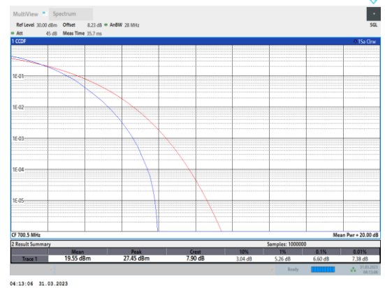
Band12-3MHz-64QAM-23025-15RB#0
