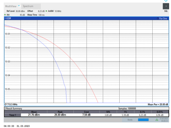
Band12-5MHz-16QAM-23155-25RB#0
