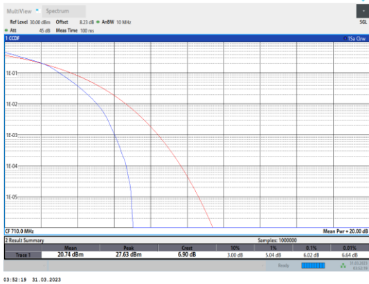
Band17-10MHz-16QAM-23790-50RB#0
