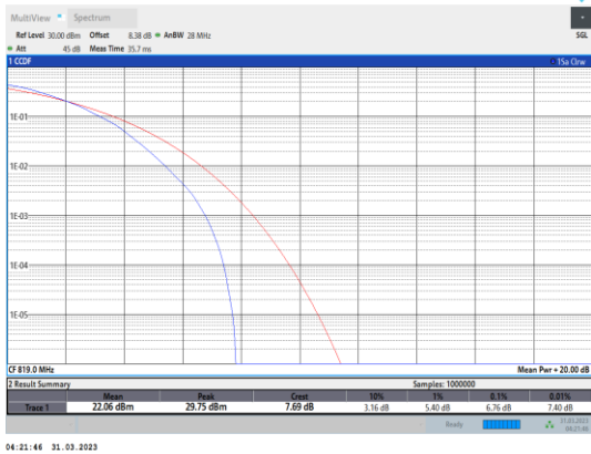
Band26-1.4MHz-64QAM-26740-6RB#0
