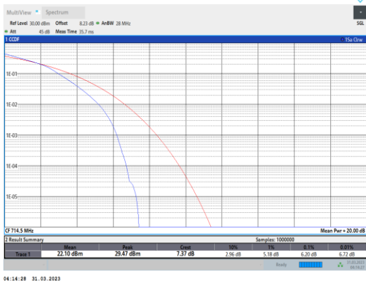
Band12-3MHz-16QAM-23165-15RB#0
