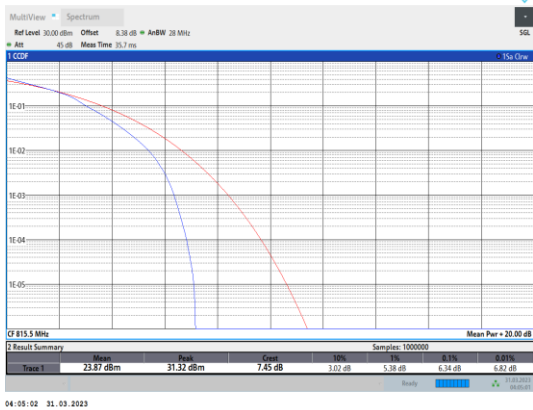
Band26-3MHz-16QAM-26705-15RB#0
