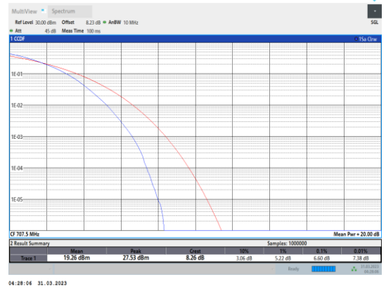
Band12-10MHz-64QAM-23095-50RB#0
