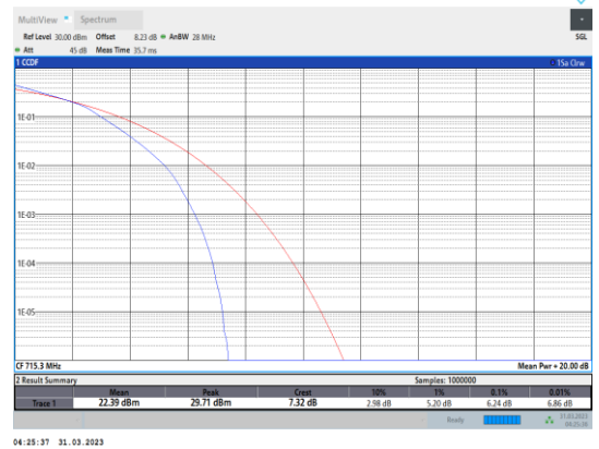
Band12-1.4MHz-16QAM-23173-6RB#0
