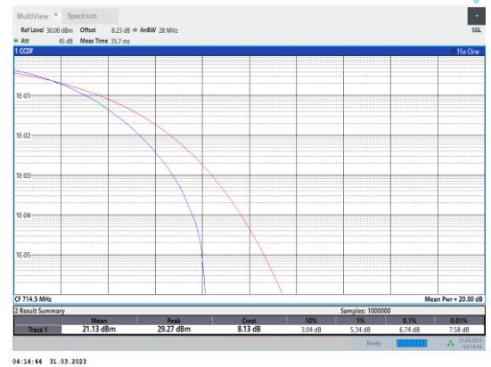
Band12-3MHz-64QAM-23165-15RB#0
