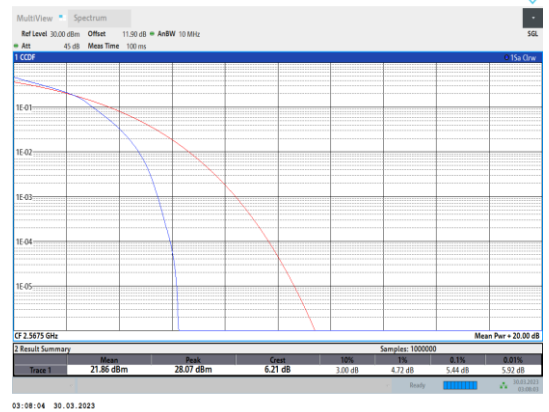
Band7-5MHz-16QAM-21425-25RB#0
