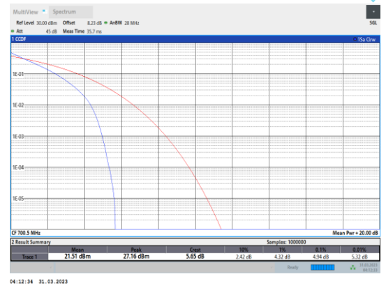
Band12-3MHz-QPSK-23025-15RB#0
