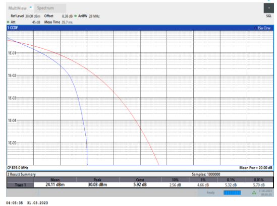
Band26-3MHz-QPSK-26740-15RB#0
