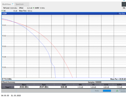
Band12-5MHz-64QAM-23155-25RB#0
