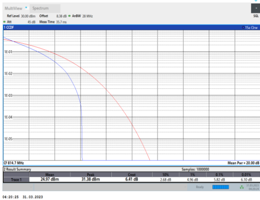
Band26-1.4MHz-QPSK-26697-6RB#0
