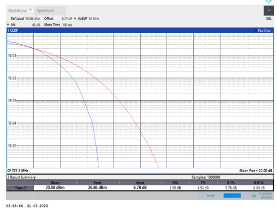
Band12-5MHz-16QAM-23095-25RB#0
