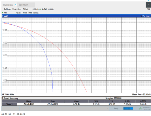
Band17-10MHz-16QAM-23780-50RB#0
