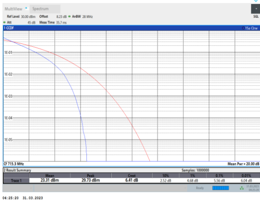
Band12-1.4MHz-QPSK-23173-6RB#0
