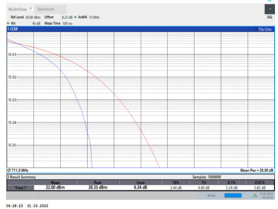
Band12-10MHz-QPSK-23130-50RB#0
