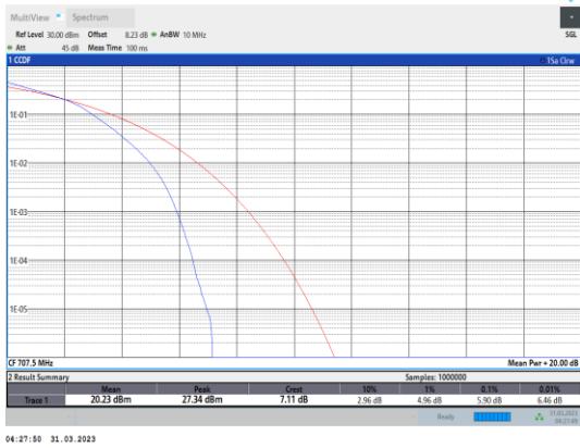
Band12-10MHz-16QAM-23095-50RB#0
