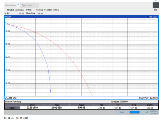
Band7-10MHz-QPSK-21400-50RB#0
