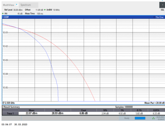
Band7-10MHz-16QAM-21100-50RB#0
