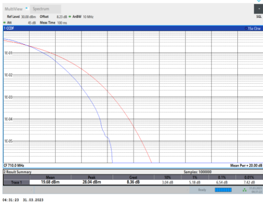
Band17-5MHz-64QAM-23790-25RB#0
