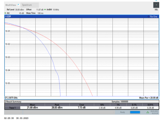
Band7-15MHz-16QAM-20825-75RB#0
