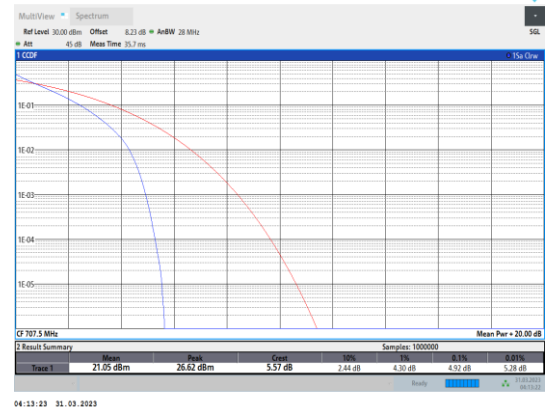
Band12-3MHz-QPSK-23095-15RB#0
