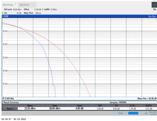
Band7-10MHz-16QAM-21400-50RB#0
