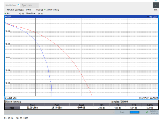
Band7-10MHz-QPSK-21100-50RB#0
