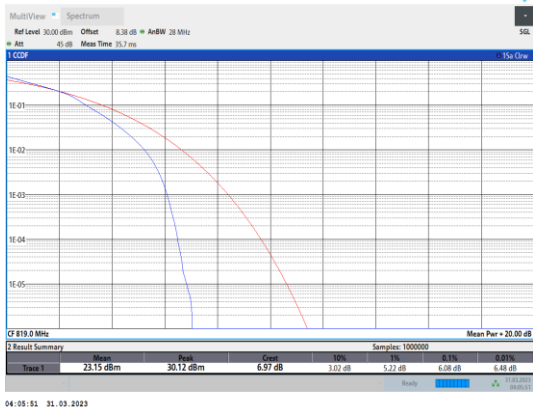
Band26-3MHz-16QAM-26740-15RB#0
