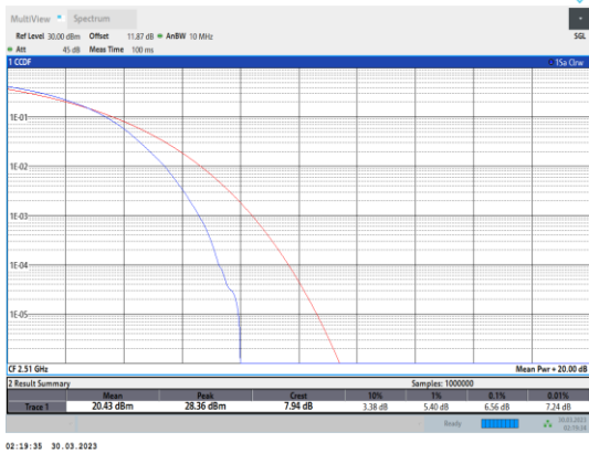
Band7-20MHz-16QAM-20850-100RB#0
