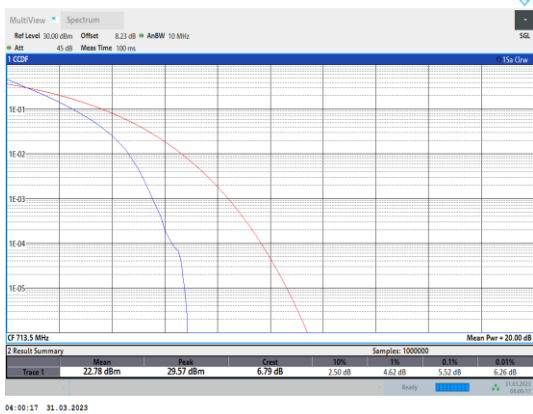
Band12-5MHz-QPSK-23155-25RB#0
