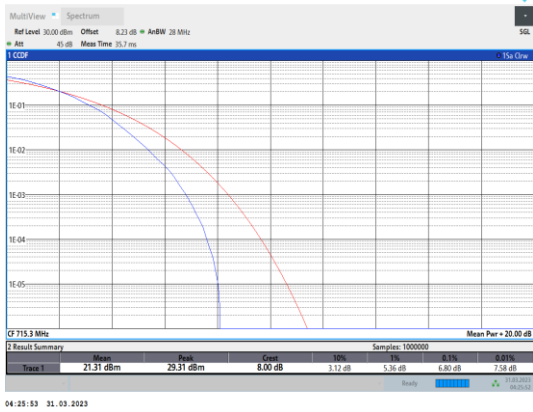
Band12-1.4MHz-64QAM-23173-6RB#0
