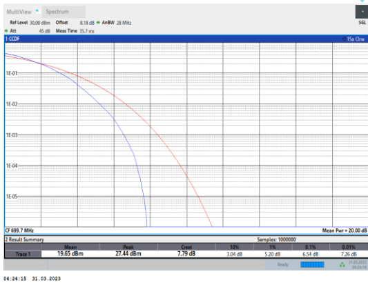
Band12-1.4MHz-64QAM-23017-6RB#0
