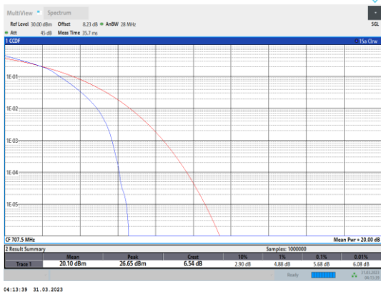
Band12-3MHz-16QAM-23095-15RB#0
