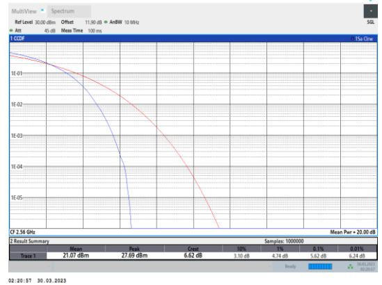
Band7-20MHz-QPSK-21350-100RB#0
