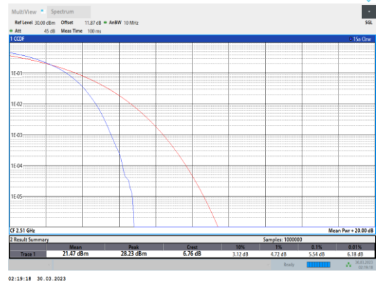
Band7-20MHz-QPSK-20850-100RB#0
