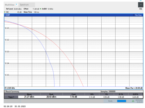
Band7-15MHz-16QAM-21100-75RB#0
