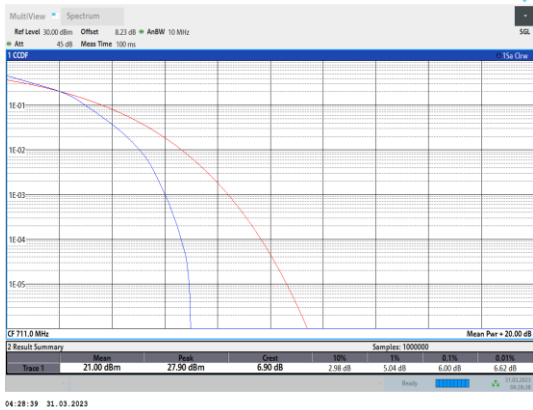
Band12-10MHz-16QAM-23130-50RB#0
