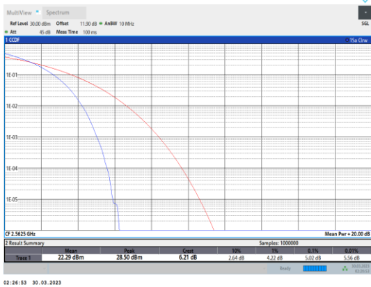
Band7-15MHz-QPSK-21375-75RB#0
