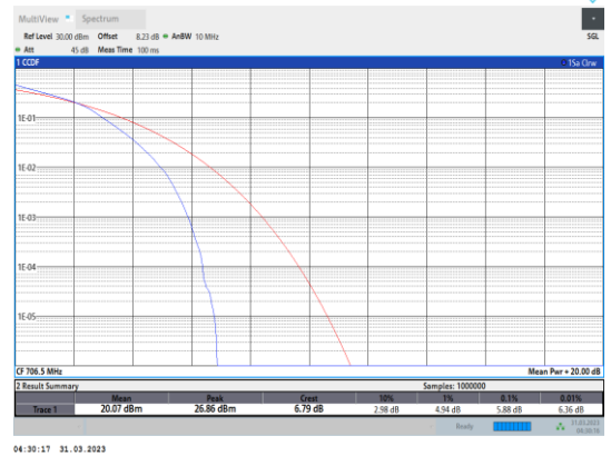
Band17-5MHz-16QAM-23755-25RB#0
