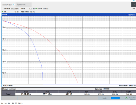
Band17-5MHz-QPSK-23790-25RB#0
