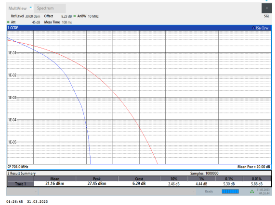
Band12-10MHz-QPSK-23060-50RB#0
