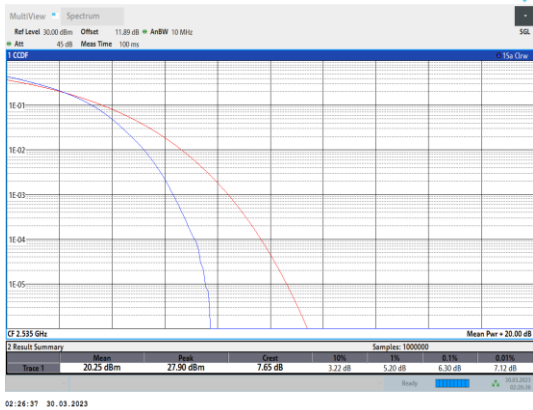
Band7-15MHz-64QAM-21100-75RB#0
