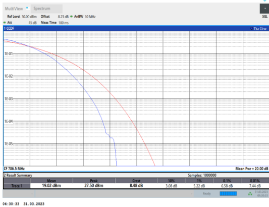
Band17-5MHz-64QAM-23755-25RB#0
