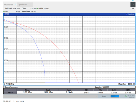
Band17-10MHz-QPSK-23790-50RB#0
