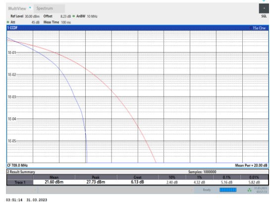
Band17-10MHz-QPSK-23780-50RB#0
