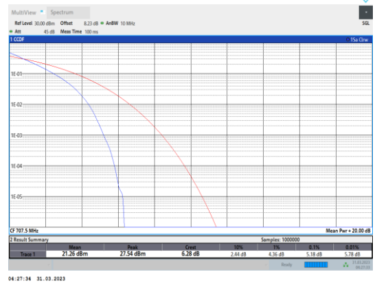
Band12-10MHz-QPSK-23095-50RB#0
