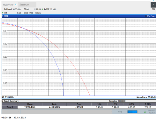
Band7-20MHz-16QAM-21100-100RB#0
