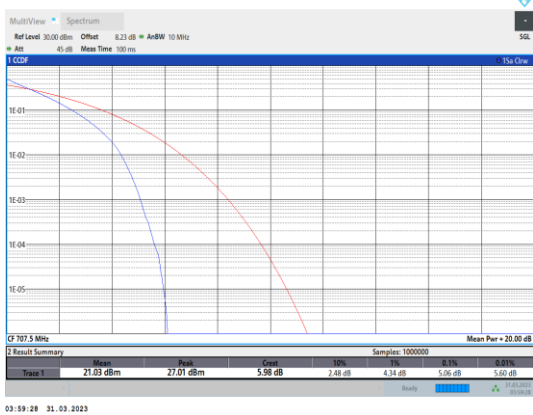
Band12-5MHz-QPSK-23095-25RB#0
