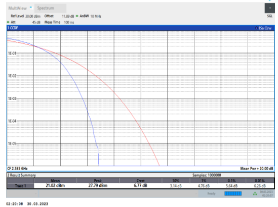
Band7-20MHz-QPSK-21100-100RB#0
