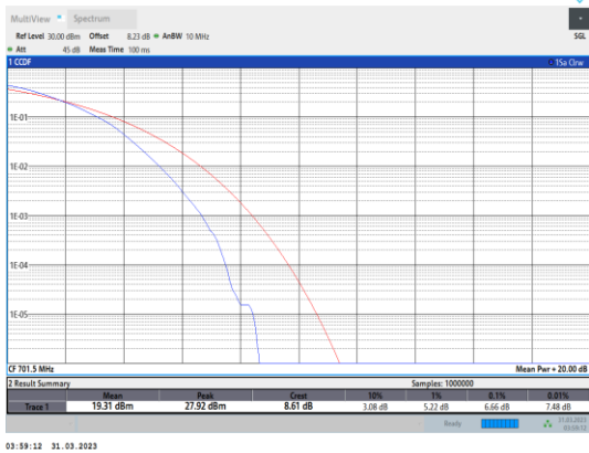
Band12-5MHz-64QAM-23035-25RB#0
