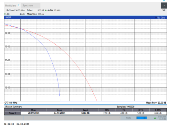
Band17-5MHz-16QAM-23790-25RB#0
