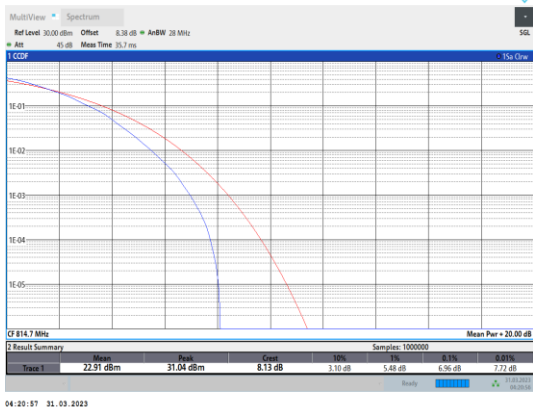
Band26-1.4MHz-64QAM-26697-6RB#0
