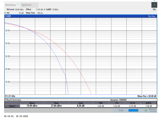
Band7-20MHz-64QAM-20850-100RB#0
