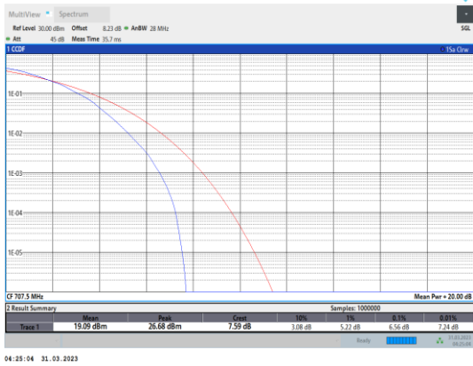
Band12-1.4MHz-64QAM-23095-6RB#0
