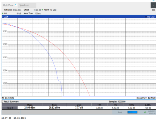
Band7-5MHz-64QAM-21100-25RB#0
