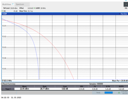
Band26-1.4MHz-QPSK-26783-6RB#0
