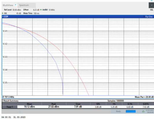
Band12-5MHz-64QAM-23095-25RB#0
