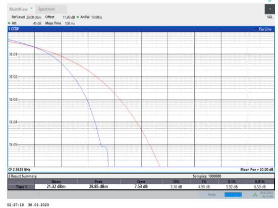
Band7-15MHz-16QAM-21375-75RB#0
