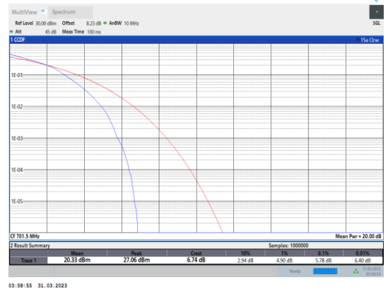
Band12-5MHz-16QAM-23035-25RB#0
