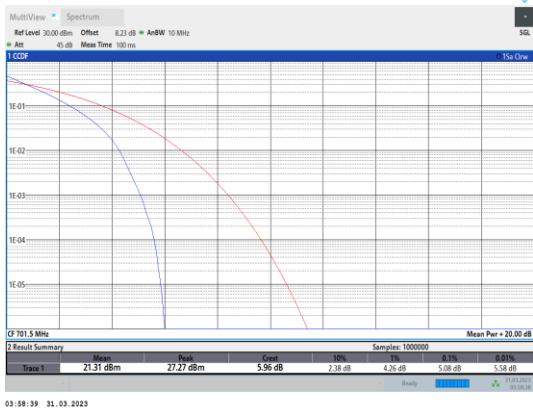
Band12-5MHz-QPSK-23035-25RB#0
