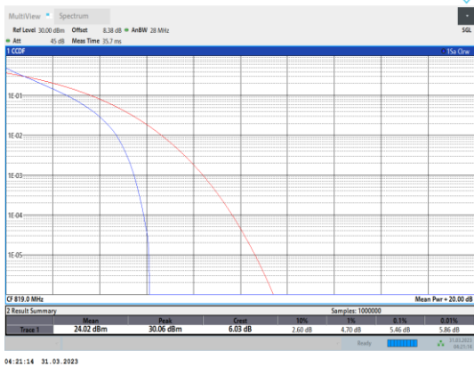
Band26-1.4MHz-QPSK-26740-6RB#0
