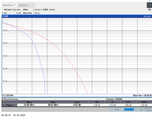
Band7-5MHz-QPSK-21100-25RB#0
