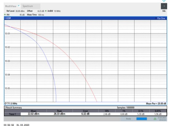
Band17-10MHz-QPSK-23800-50RB#0
