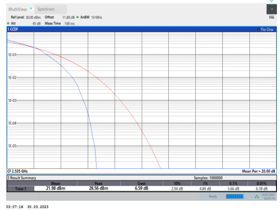
Band7-5MHz-16QAM-21100-25RB#0
