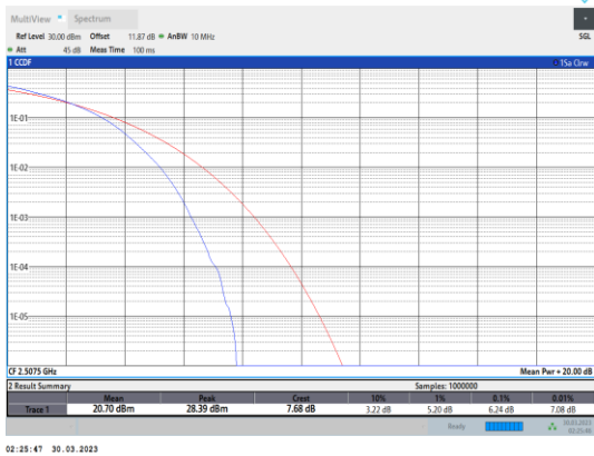
Band7-15MHz-64QAM-20825-75RB#0
