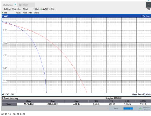
Band7-15MHz-QPSK-20825-75RB#0
