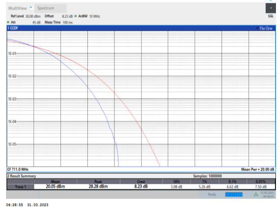
Band12-10MHz-64QAM-23130-50RB#0
