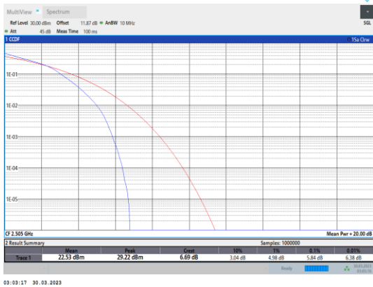
Band7-10MHz-16QAM-20800-50RB#0
