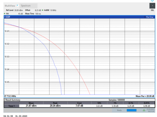
Band17-5MHz-16QAM-23825-25RB#0
