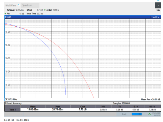
Band12-3MHz-64QAM-23095-15RB#0
