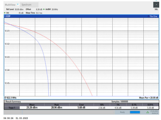
Band26-3MHz-QPSK-26775-15RB#0
