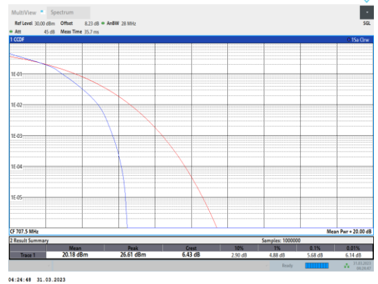
Band12-1.4MHz-16QAM-23095-6RB#0
