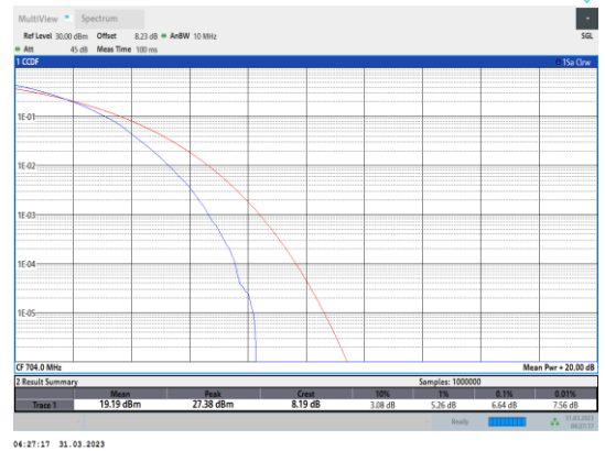
Band12-10MHz-64QAM-23060-50RB#0
