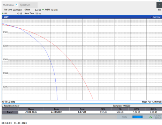
Band17-10MHz-16QAM-23800-50RB#0
