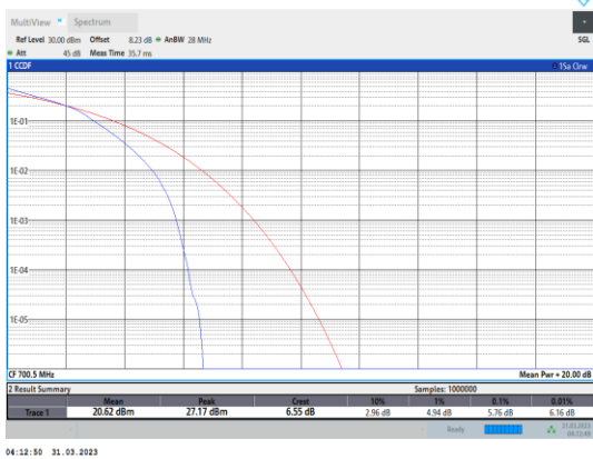
Band12-3MHz-16QAM-23025-15RB#0
