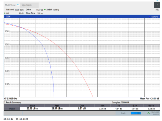
Band7-5MHz-16QAM-20775-25RB#0
