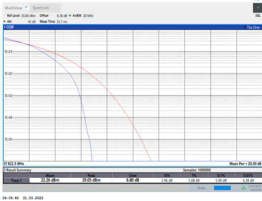
Band26-3MHz-16QAM-26775-15RB#0
