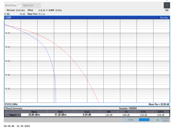
Band26-3MHz-QPSK-26705-15RB#0
