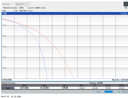
Band12-10MHz-16QAM-23060-50RB#0
