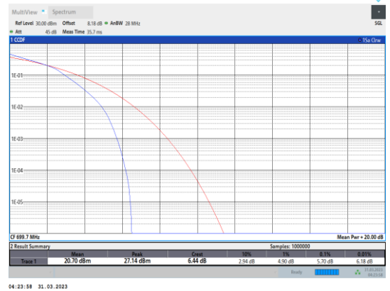
Band12-1.4MHz-16QAM-23017-6RB#0
