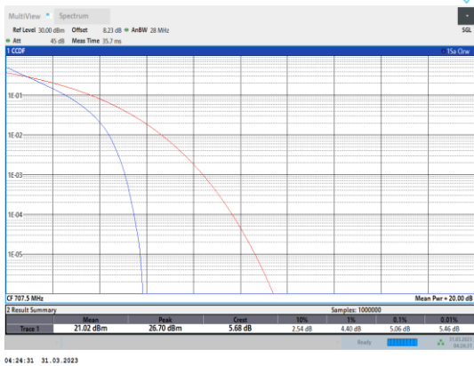
Band12-1.4MHz-QPSK-23095-6RB#0
