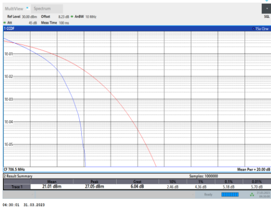
Band17-5MHz-QPSK-23755-25RB#0
