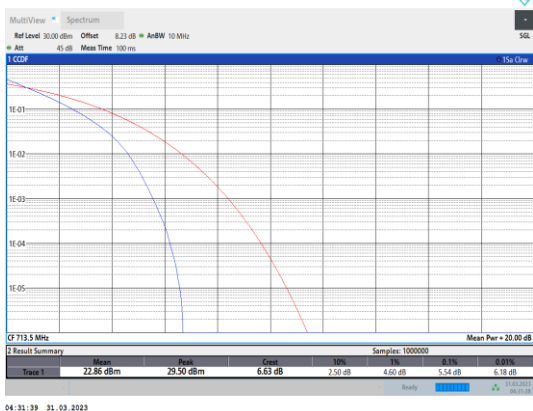
Band17-5MHz-QPSK-23825-25RB#0
