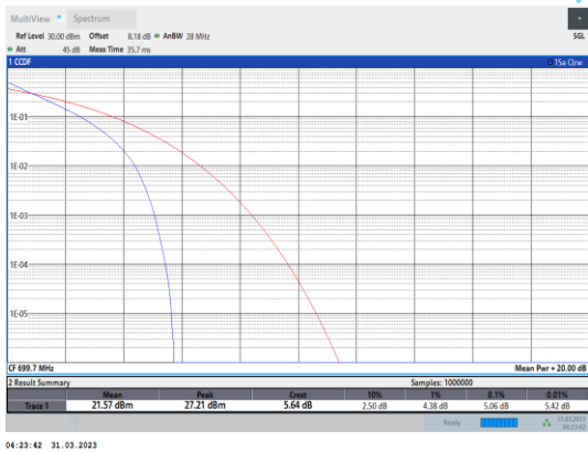
Band12-1.4MHz-QPSK-23017-6RB#0
