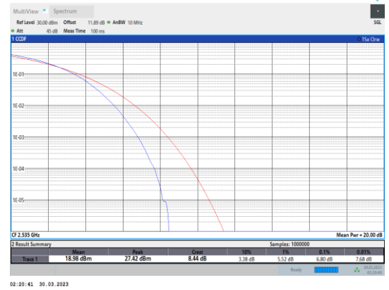
Band7-20MHz-64QAM-21100-100RB#0
