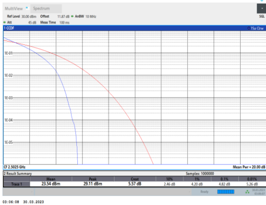
Band7-5MHz-QPSK-20775-25RB#0
