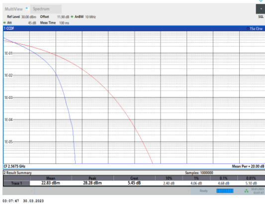
Band7-5MHz-QPSK-21425-25RB#0
