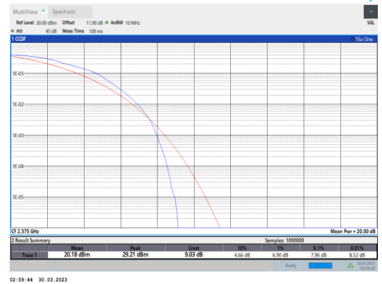
Band38-10MHz-16QAM-37800-50RB#0
