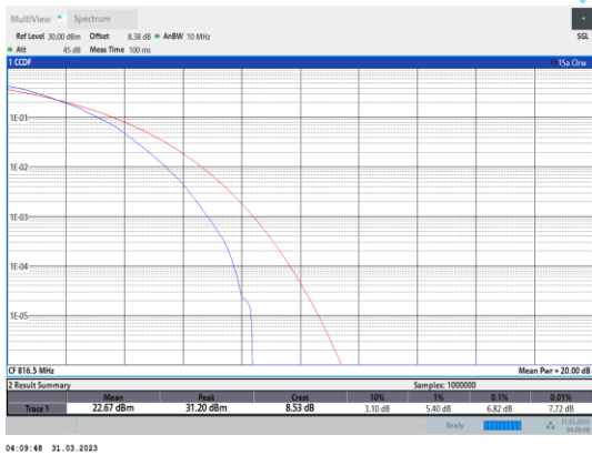
Band26-5MHz-64QAM-26715-25RB#0
