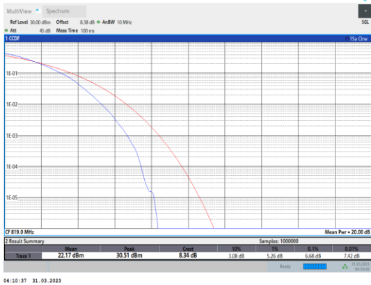
Band26-5MHz-64QAM-26740-25RB#0
