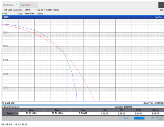
Band38-5MHz-16QAM-38000-25RB#0
