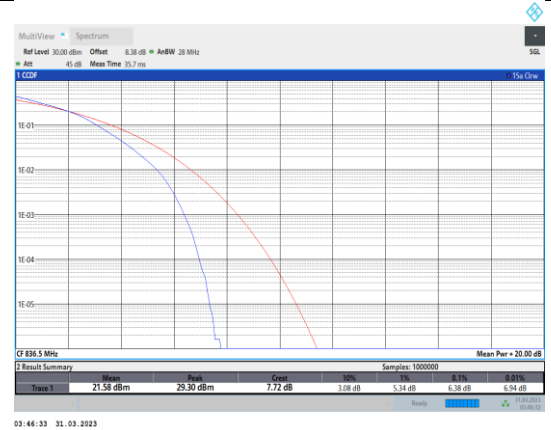
Band26-15MHz-16QAM-26915-75RB#0
