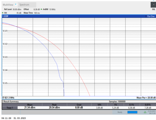
Band26-5MHz-64QAM-26765-25RB#0
