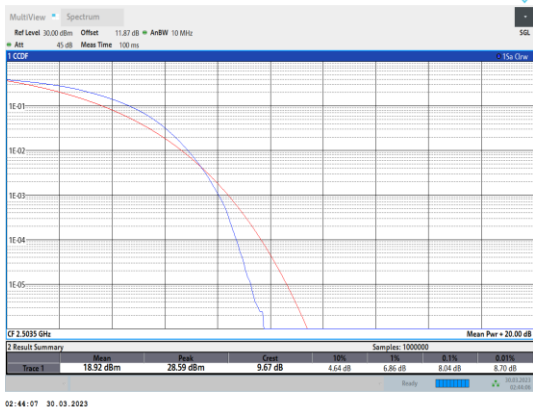
Band41-15MHz-16QAM-39725-75RB#0
