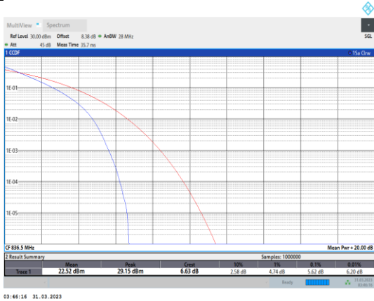
Band26-15MHz-QPSK-26915-75RB#0
