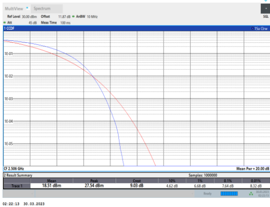
Band41-20MHz-QPSK-39750-100RB#0
