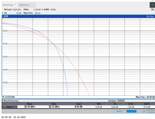
Band38-5MHz-16QAM-37775-25RB#0
