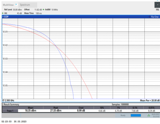
Band41-20MHz-QPSK-40620-100RB#0
