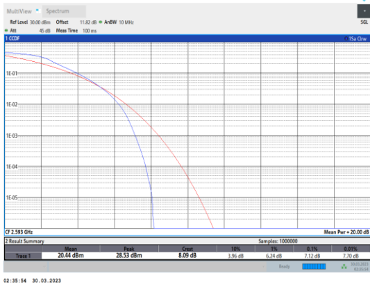
Band41-10MHz-QPSK-40620-50RB#0
