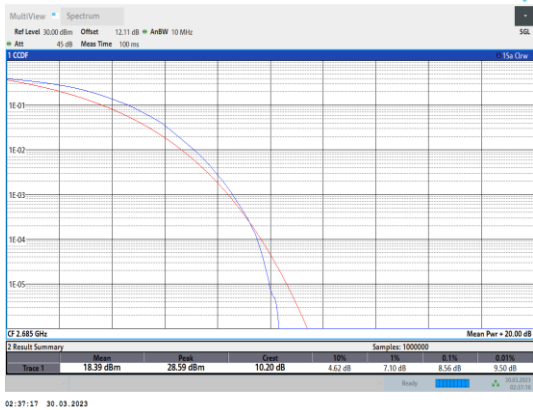
Band41-10MHz-64QAM-41540-50RB#0
