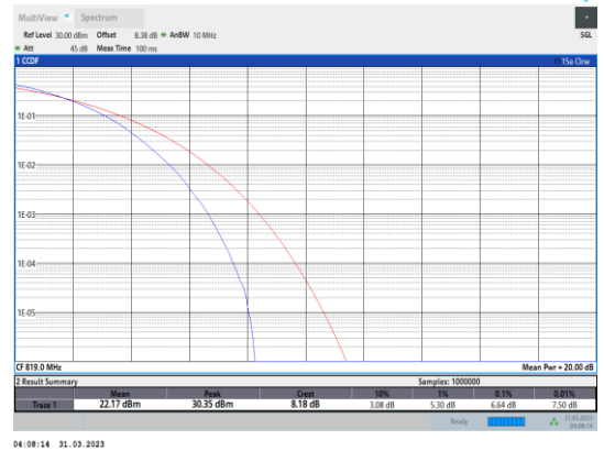
Band26-10MHz-64QAM-26740-50RB#0
