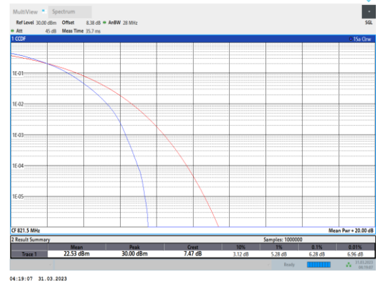
Band26-15MHz-16QAM-26765-75RB#0
