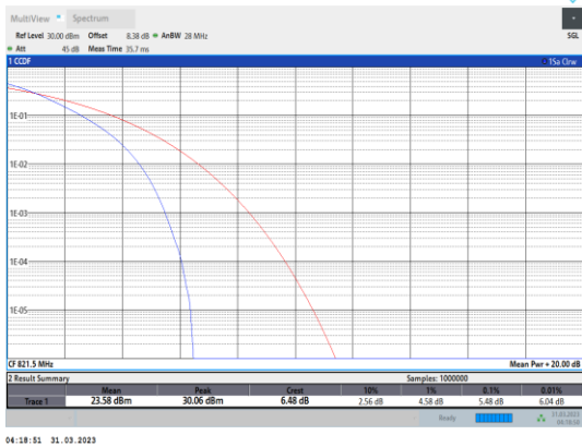
Band26-15MHz-QPSK-26765-75RB#0
