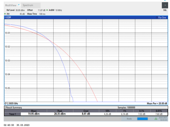
Band41-15MHz-QPSK-39725-75RB#0
