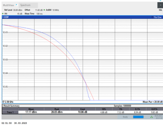
Band38-20MHz-64QAM-37850-100RB#0
