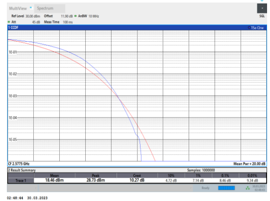
Band38-15MHz-64QAM-37825-75RB#0
