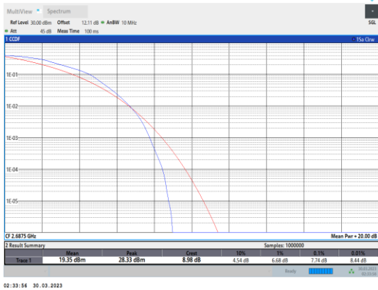
Band41-5MHz-16QAM-41565-25RB#0
