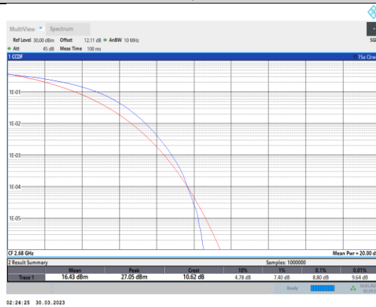
Band41-20MHz-64QAM-41490-100RB#0
