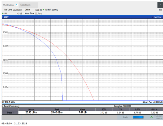
Band26-15MHz-64QAM-26915-1RB#0
