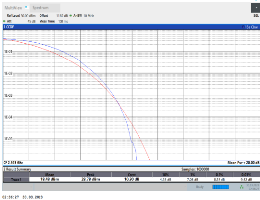
Band41-10MHz-64QAM-40620-50RB#0
