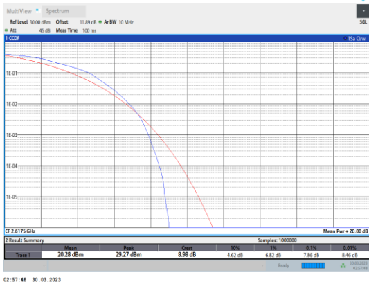
Band38-5MHz-16QAM-38225-25RB#0
