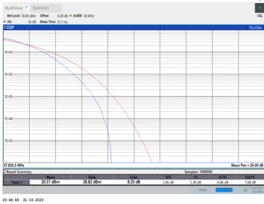
Band26-15MHz-64QAM-26915-75RB#0
