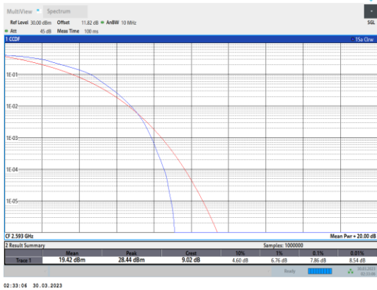
Band41-5MHz-16QAM-40620-25RB#0
