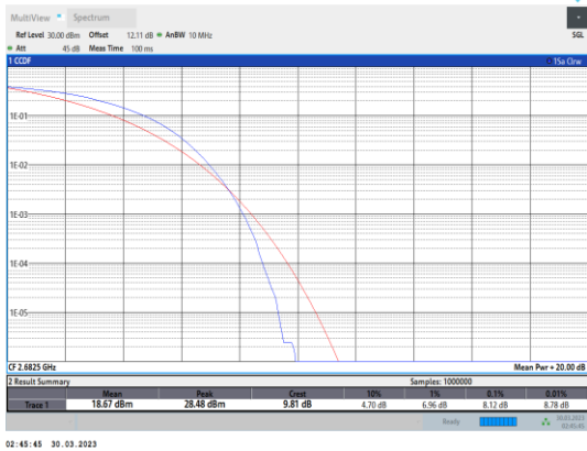
Band41-15MHz-16QAM-41515-75RB#0
