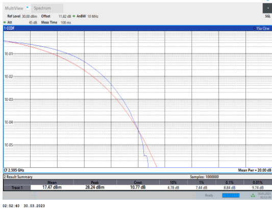
Band38-20MHz-64QAM-38000-100RB#0
