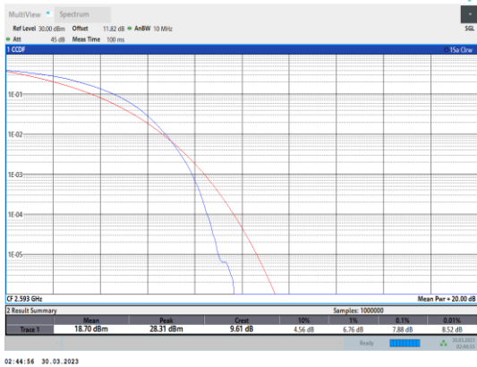
Band41-15MHz-16QAM-40620-75RB#0
