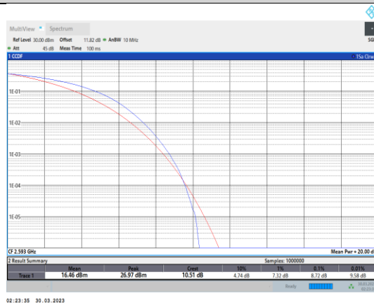
Band41-20MHz-64QAM-40620-100RB#0
