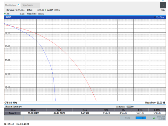
Band26-10MHz-QPSK-26740-50RB#0
