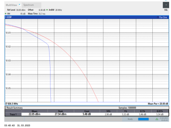
Band26-15MHz-16QAM-26915-1RB#0
