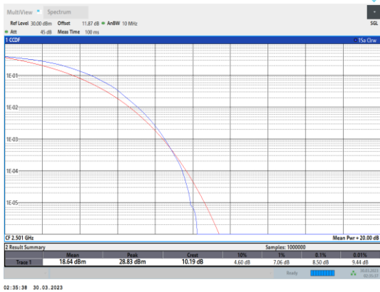
Band41-10MHz-64QAM-39700-50RB#0
