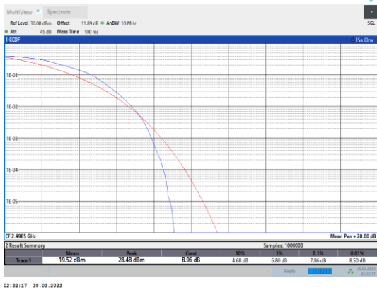
Band41-5MHz-16QAM-39675-25RB#0
