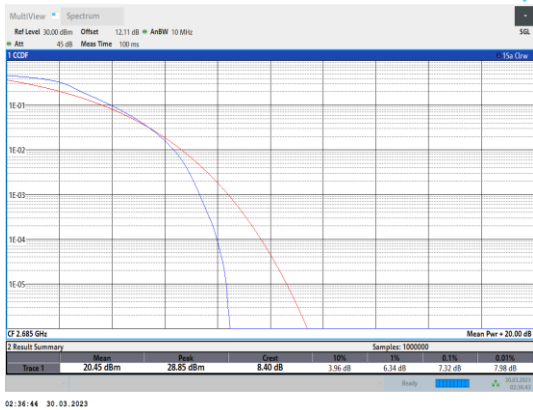
Band41-10MHz-QPSK-41540-50RB#0
