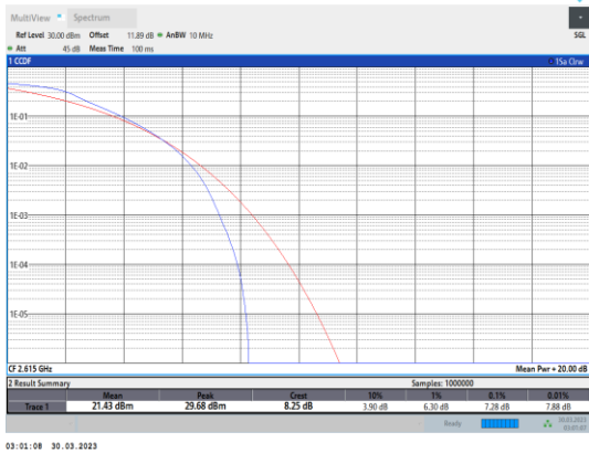
Band38-10MHz-QPSK-38200-50RB#0
