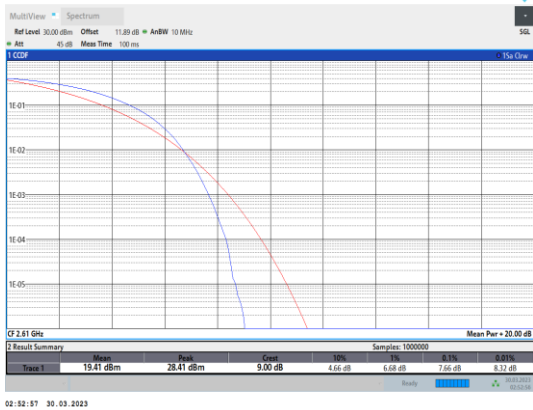
Band38-20MHz-QPSK-38150-100RB#0
