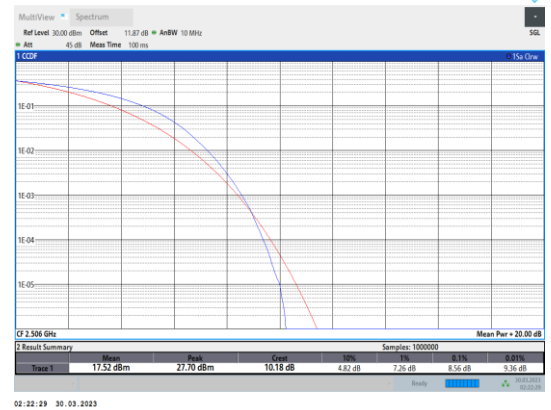
Band41-20MHz-16QAM-39750-100RB#0
