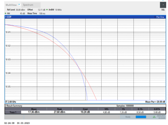
Band41-20MHz-16QAM-41490-100RB#0
