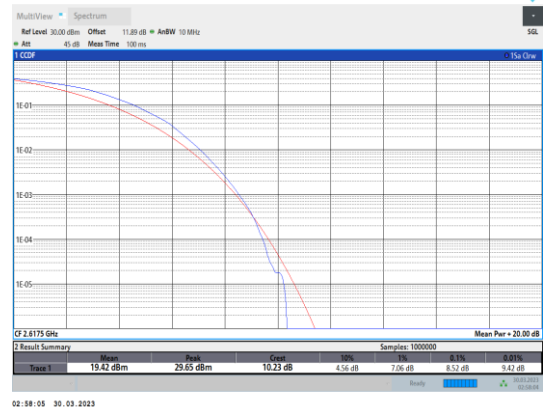
Band38-5MHz-64QAM-38225-25RB#0
