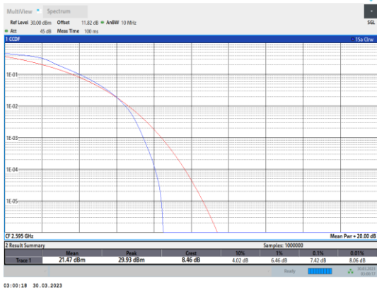
Band38-10MHz-QPSK-38000-50RB#0
