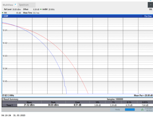
Band26-15MHz-64QAM-26765-75RB#0
