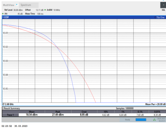
Band41-20MHz-QPSK-41490-100RB#0
