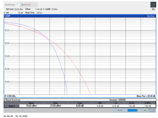
Band41-15MHz-QPSK-40620-75RB#0
