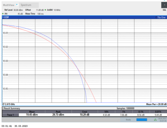
Band38-10MHz-64QAM-38200-50RB#0
