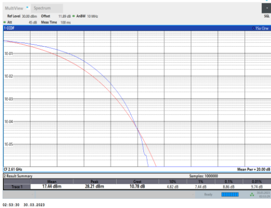
Band38-20MHz-64QAM-38150-100RB#0
