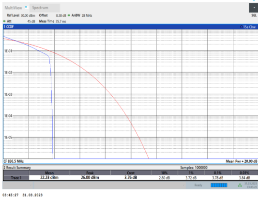
Band26-15MHz-QPSK-26915-1RB#0
