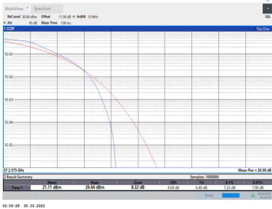
Band38-10MHz-QPSK-37800-50RB#0
