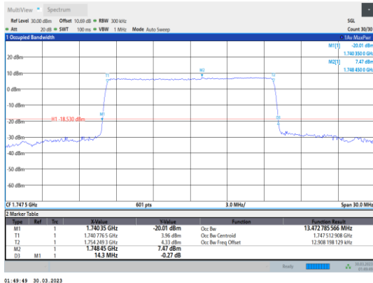
Band4-15MHz-QPSK-20325-75RB#0
