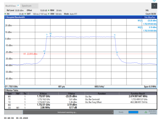
Band4-3MHz-QPSK-20385-15RB#0
