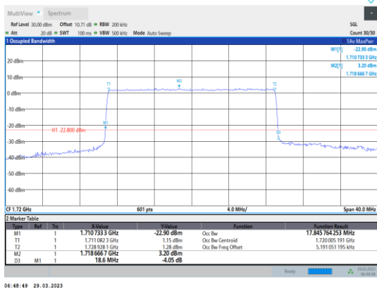
Band4-20MHz-16QAM-20050-100RB#0
