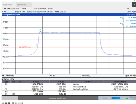
Band4-3MHz-16QAM-20385-15RB#0
