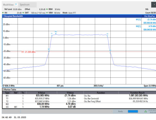
Band5-1.4MHz-64QAM-20525-6RB#0
