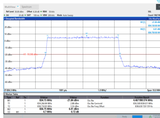
Band5-5MHz-16QAM-20525-25RB#0
