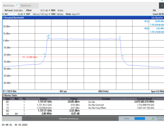
Band4-3MHz-16QAM-20175-15RB#0
