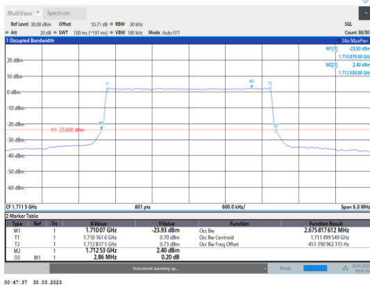
Band4-3MHz-16QAM-19965-15RB#0
