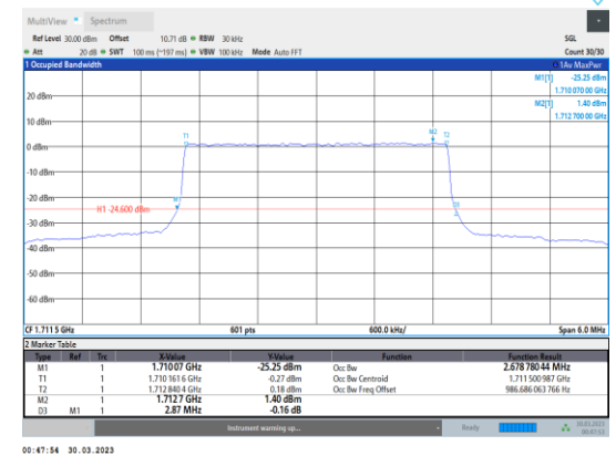
Band4-3MHz-64QAM-19965-15RB#0
