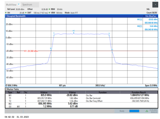
Band5-1.4MHz-16QAM-20525-6RB#0
