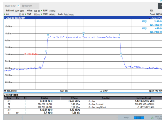
Band5-5MHz-16QAM-20425-25RB#0
