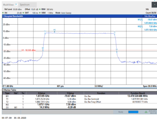
Band2-15MHz-QPSK-18900-75RB#0
