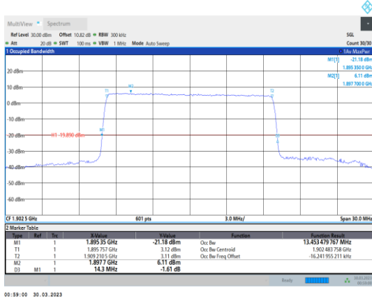
Band2-15MHz-64QAM-19125-75RB#0
