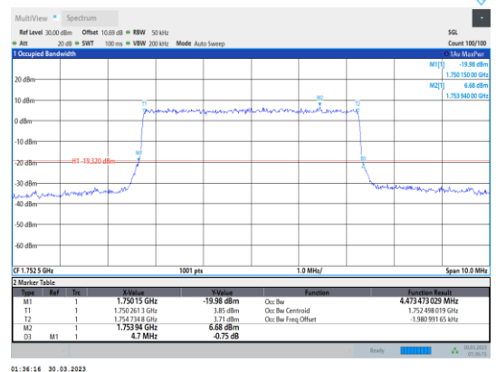
Band4-5MHz-16QAM-20375-25RB#0
