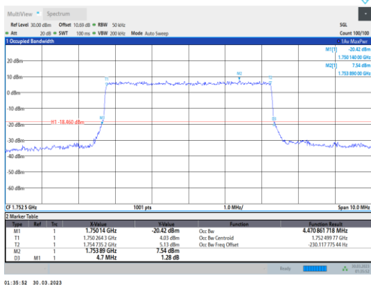
Band4-5MHz-QPSK-20375-25RB#0
