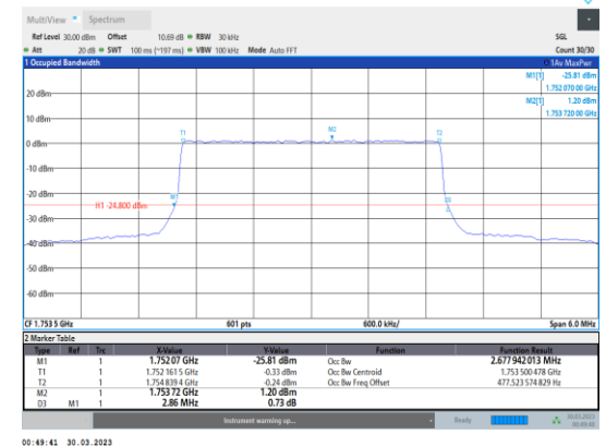
Band4-3MHz-64QAM-20385-15RB#0
