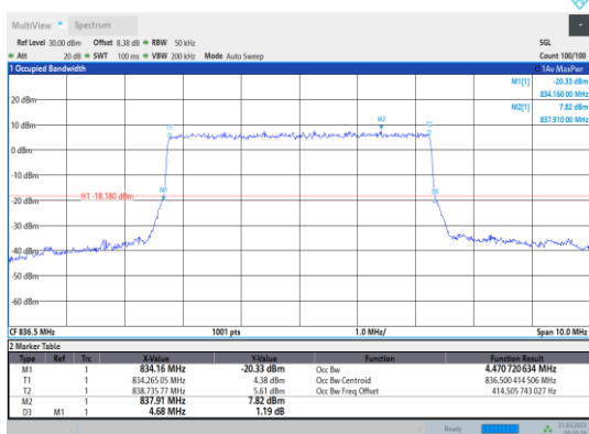
Band5-5MHz-QPSK-20525-25RB#0
