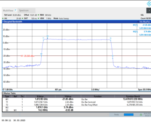
Band2-15MHz-64QAM-18900-75RB#0
