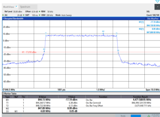
Band5-5MHz-QPSK-20625-25RB#0
