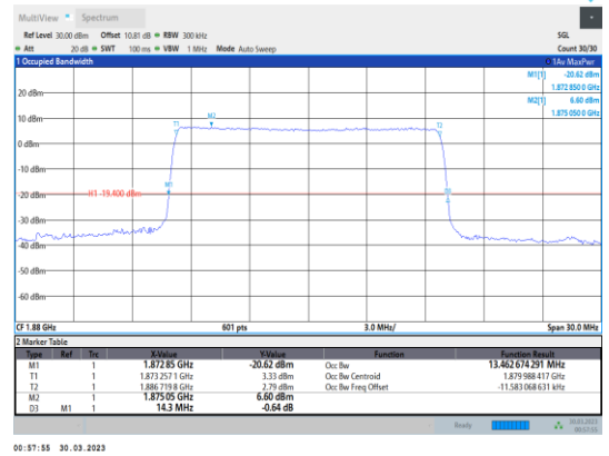
Band2-15MHz-16QAM-18900-75RB#0
