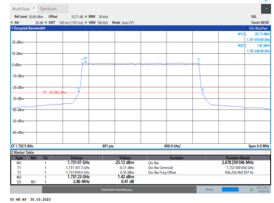
Band4-3MHz-64QAM-20175-15RB#0
