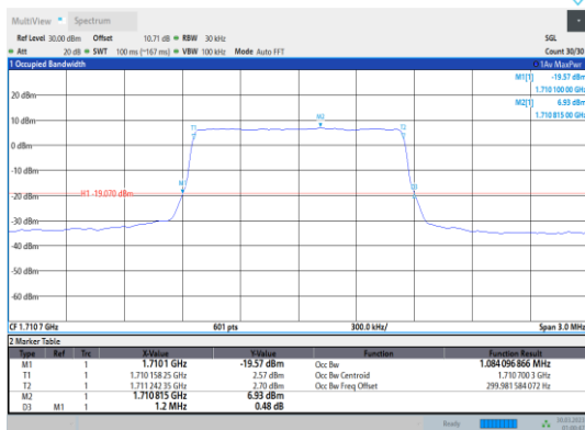
Band4-1.4MHz-QPSK-19957-6RB#0
