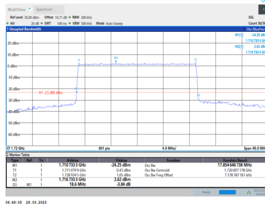
Band4-20MHz-64QAM-20050-100RB#0
