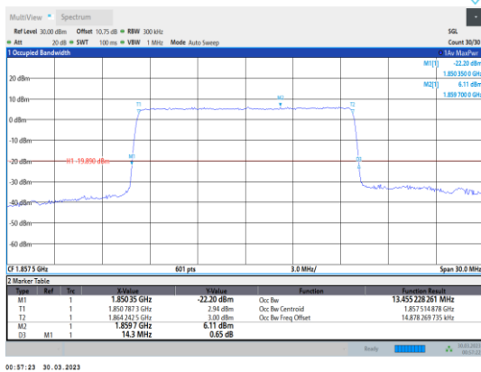
Band2-15MHz-64QAM-18675-75RB#0
