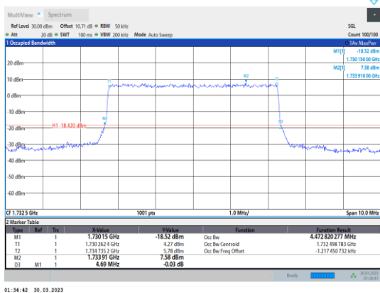
Band4-5MHz-QPSK-20175-25RB#0
