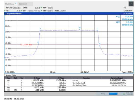
Band5-3MHz-QPSK-20525-15RB#0
