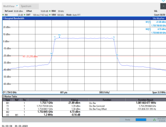
Band4-1.4MHz-64QAM-20393-6RB#0
