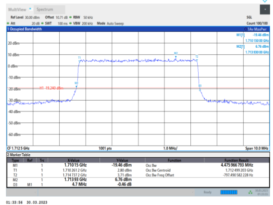
Band4-5MHz-16QAM-19975-25RB#0
