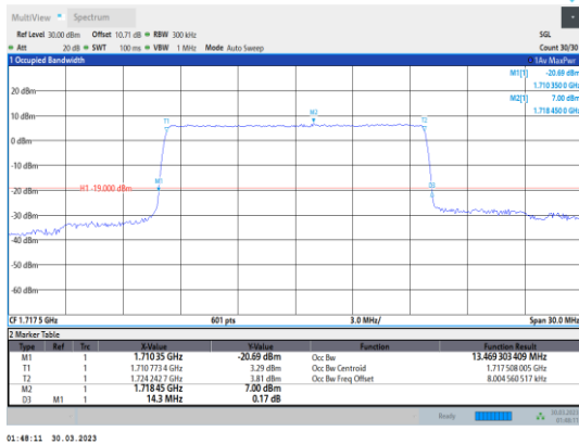
Band4-15MHz-QPSK-20025-75RB#0
