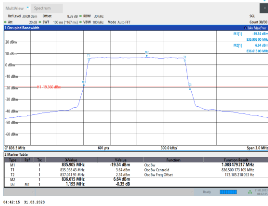
Band5-1.4MHz-QPSK-20525-6RB#0
