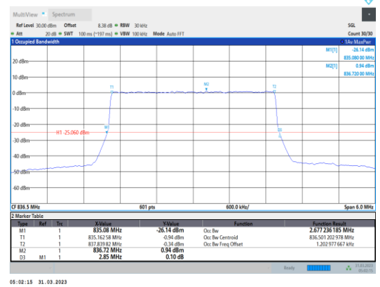
Band5-3MHz-64QAM-20525-15RB#0
