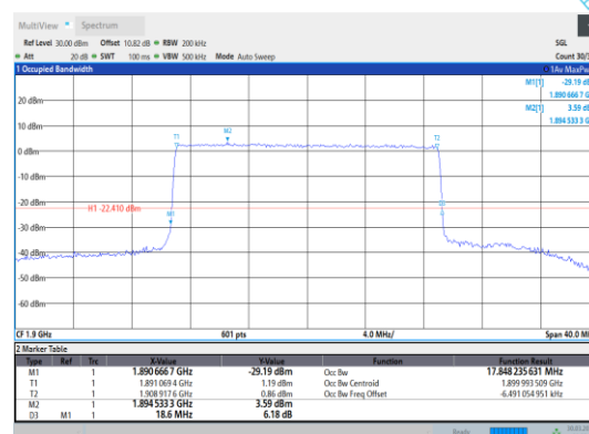
Band2-20MHz-64QAM-19100-100RB#0
