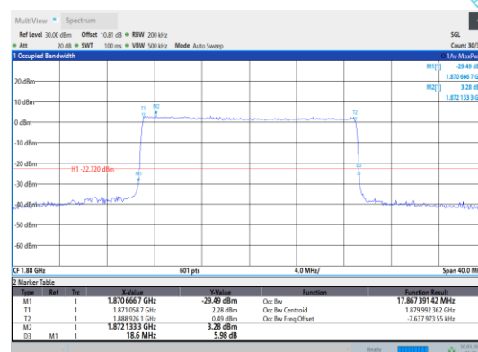
Band2-20MHz-64QAM-18900-100RB#0
