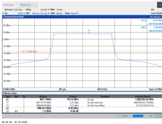
Band5-1.4MHz-QPSK-20643-6RB#0
