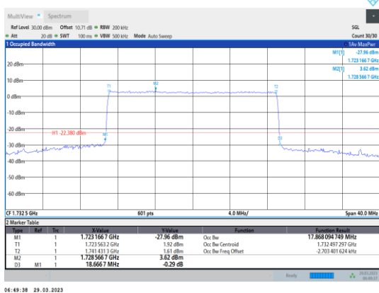
Band4-20MHz-16QAM-20175-100RB#0
