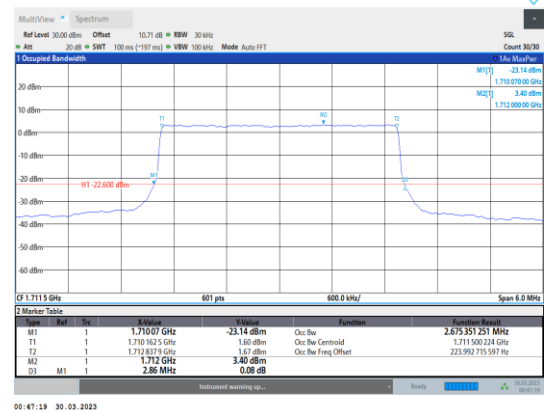
Band4-3MHz-QPSK-19965-15RB#0
