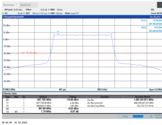
Band5-1.4MHz-64QAM-20643-6RB#0
