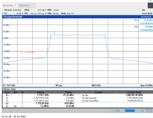
Band4-1.4MHz-64QAM-19957-6RB#0
