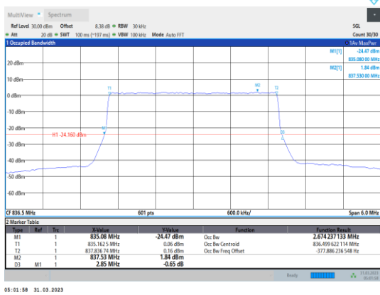
Band5-3MHz-16QAM-20525-15RB#0
