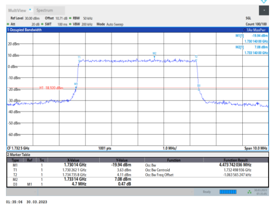
Band4-5MHz-16QAM-20175-25RB#0
