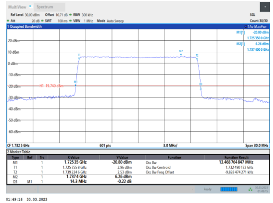
Band4-15MHz-16QAM-20175-75RB#0
