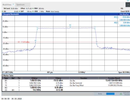
Band2-15MHz-QPSK-18675-75RB#0
