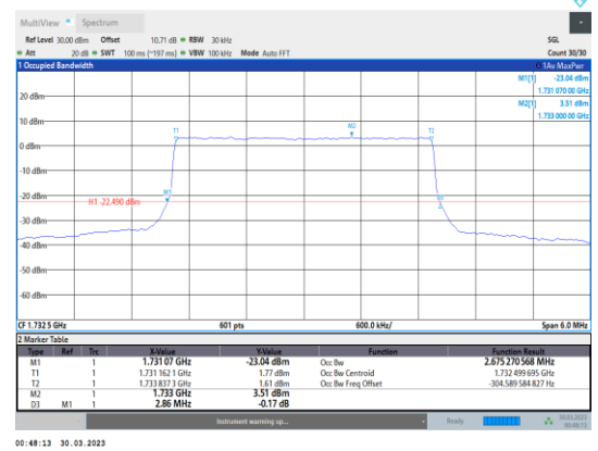
Band4-3MHz-QPSK-20175-15RB#0
