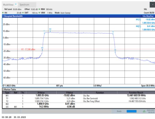
Band2-15MHz-QPSK-19125-75RB#0
