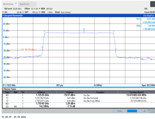
Band4-15MHz-QPSK-20175-75RB#0
