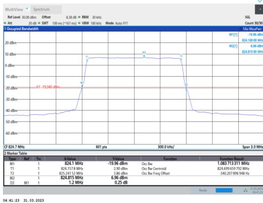
Band5-1.4MHz-QPSK-20407-6RB#0
