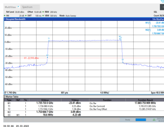
Band4-20MHz-64QAM-20300-100RB#0
