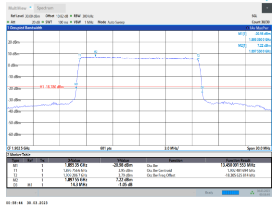
Band2-15MHz-16QAM-19125-75RB#0
