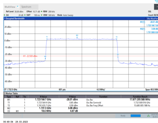
Band4-20MHz-64QAM-20175-100RB#0
