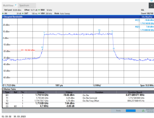
Band4-5MHz-QPSK-19975-25RB#0
