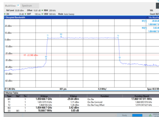
Band2-20MHz-64QAM-18700-100RB#0
