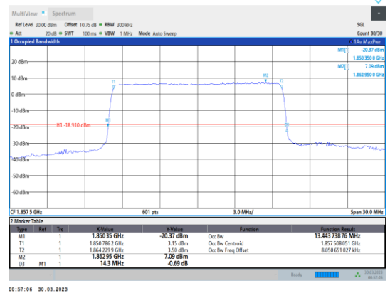
Band2-15MHz-16QAM-18675-75RB#0
