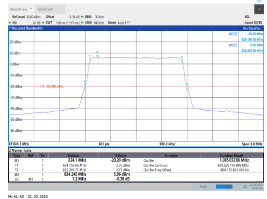
Band5-1.4MHz-16QAM-20407-6RB#0
