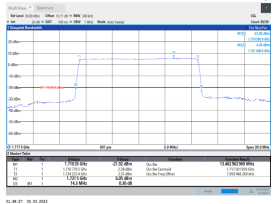
Band4-15MHz-16QAM-20025-75RB#0
