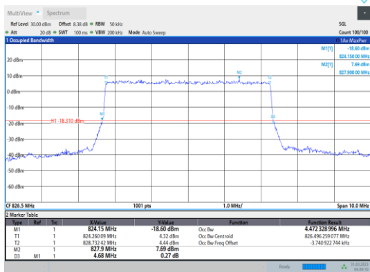
Band5-5MHz-QPSK-20425-25RB#0
