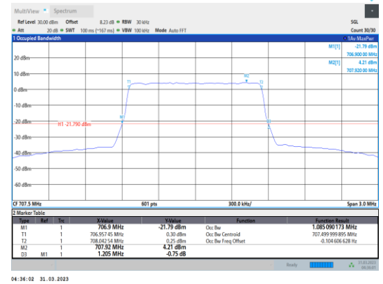
Band12-1.4MHz-16QAM-23095-6RB#0
