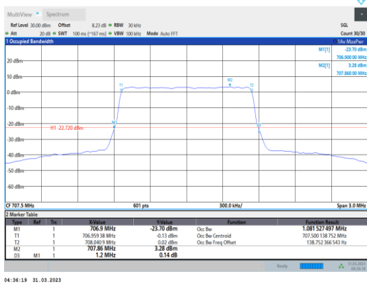
Band12-1.4MHz-64QAM-23095-6RB#0
