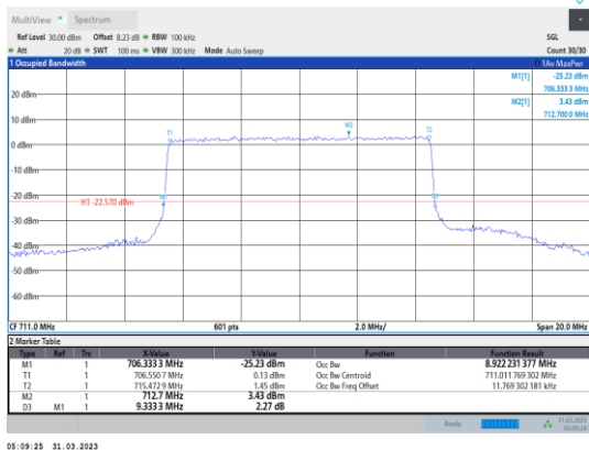
Band12-10MHz-16QAM-23130-50RB#0
