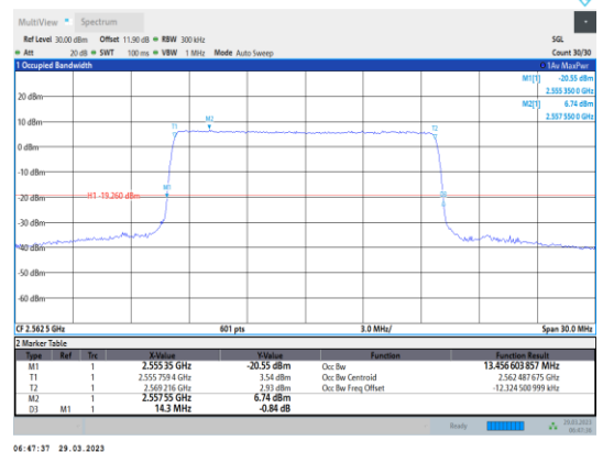
Band7-15MHz-16QAM-21375-75RB#0
