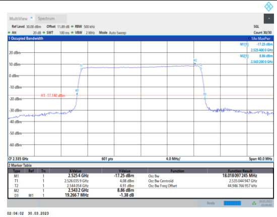
Band7-20MHz-QPSK-21100-100RB#0
