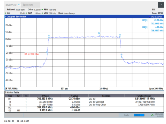
Band12-10MHz-QPSK-23095-50RB#0
