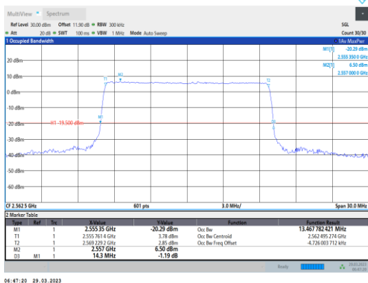
Band7-15MHz-QPSK-21375-75RB#0
