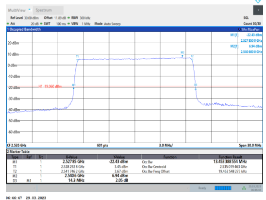
Band7-15MHz-16QAM-21100-75RB#0
