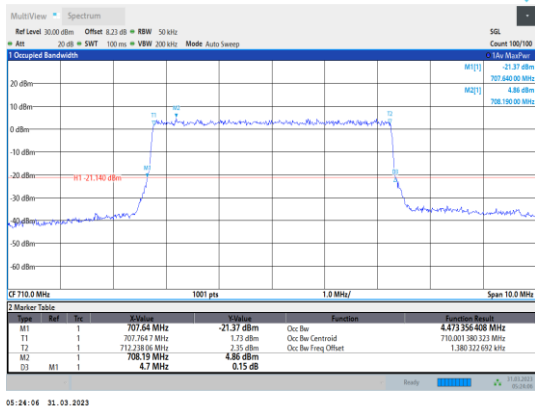
Band17-5MHz-64QAM-23790-25RB#0
