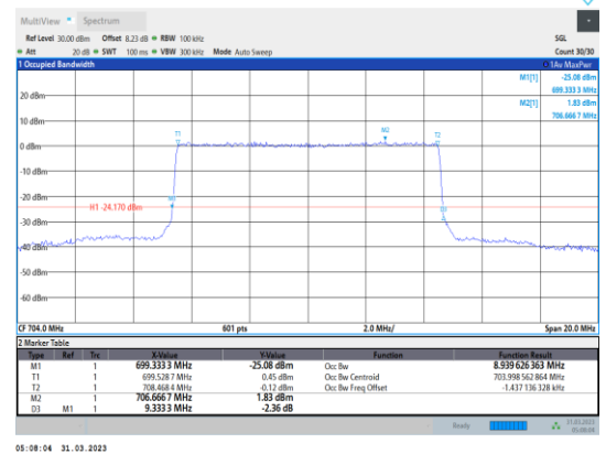
Band12-10MHz-64QAM-23060-50RB#0
