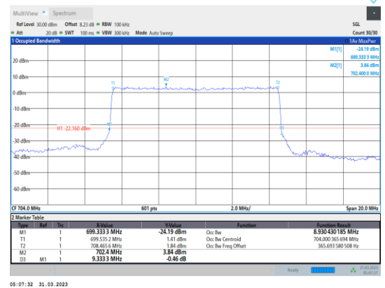
Band12-10MHz-QPSK-23060-50RB#0
