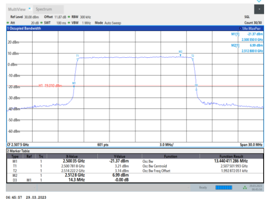
Band7-15MHz-16QAM-20825-75RB#0
