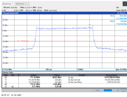
Band12-5MHz-64QAM-23155-25RB#0
