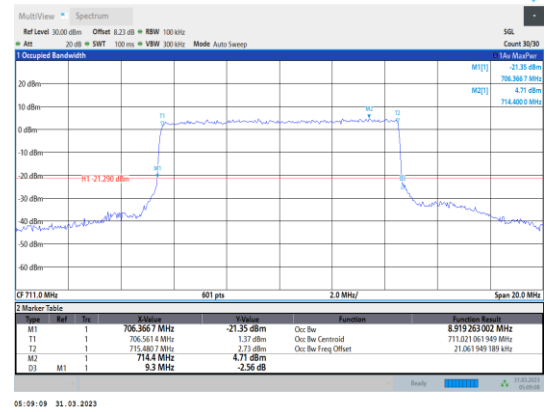
Band12-10MHz-QPSK-23130-50RB#0
