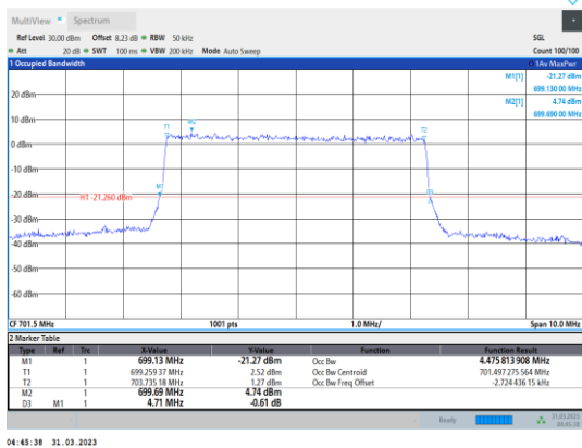
Band12-5MHz-64QAM-23035-25RB#0
