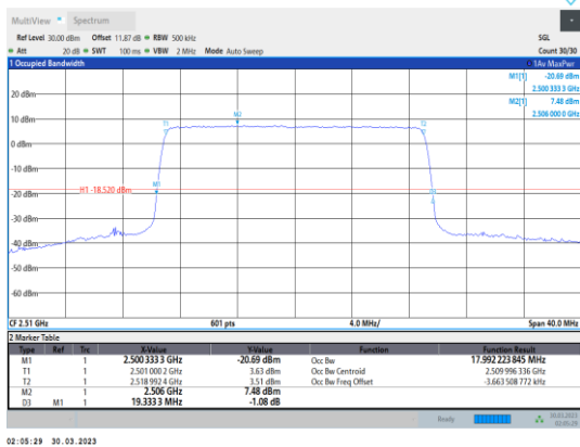
Band7-20MHz-16QAM-20850-100RB#0
