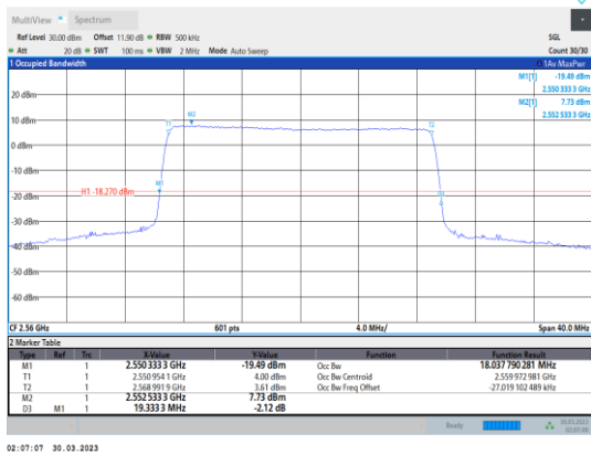
Band7-20MHz-16QAM-21350-100RB#0
