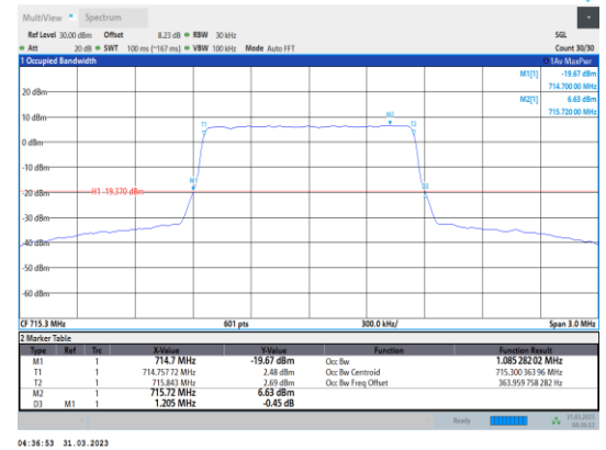
Band12-1.4MHz-16QAM-23173-6RB#0
