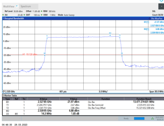
Band7-15MHz-QPSK-21100-75RB#0
