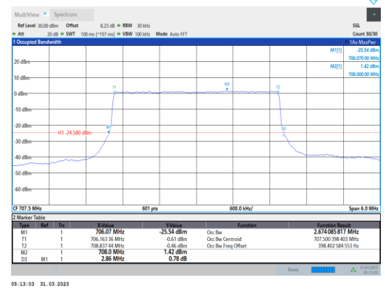
Band12-3MHz-QPSK-23095-15RB#0
