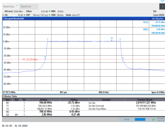
Band12-3MHz-16QAM-23095-15RB#0
