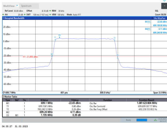
Band12-1.4MHz-64QAM-23017-6RB#0
