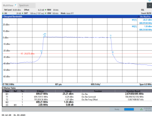
Band12-3MHz-16QAM-23025-15RB#0
