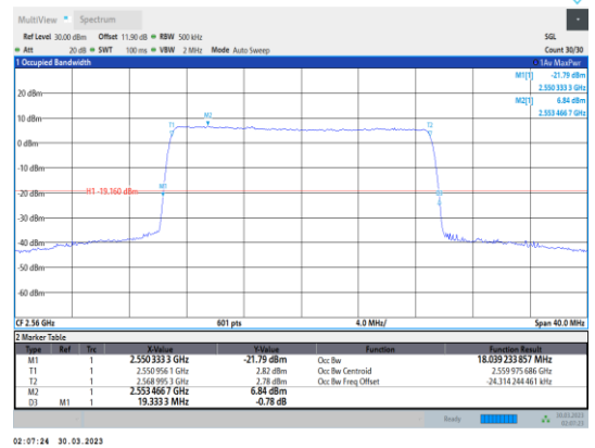
Band7-20MHz-64QAM-21350-100RB#0
