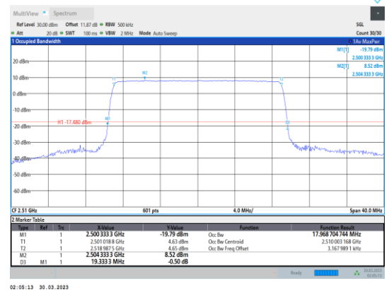
Band7-20MHz-QPSK-20850-100RB#0
