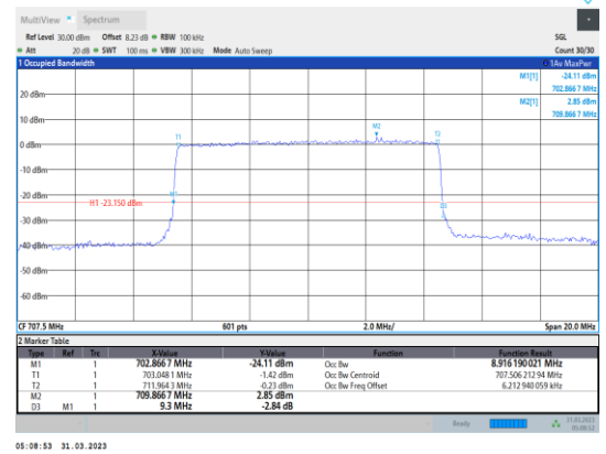
Band12-10MHz-64QAM-23095-50RB#0
