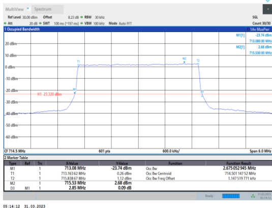
Band12-3MHz-16QAM-23165-15RB#0
