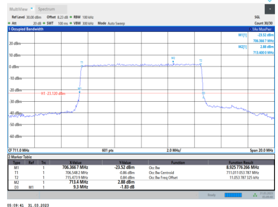
Band12-10MHz-64QAM-23130-50RB#0
