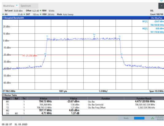
Band17-5MHz-64QAM-23755-25RB#0
