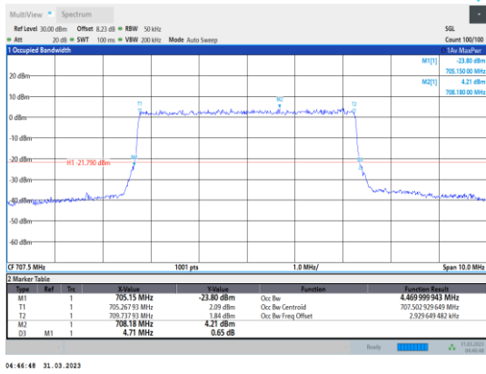
Band12-5MHz-64QAM-23095-25RB#0
