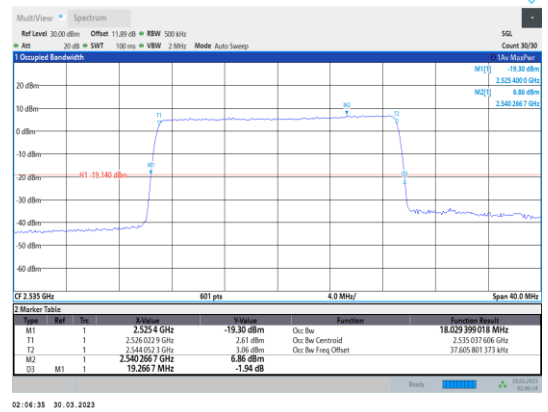
Band7-20MHz-64QAM-21100-100RB#0
