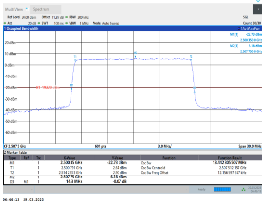
Band7-15MHz-64QAM-20825-75RB#0
