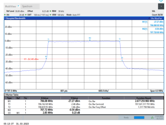
Band12-3MHz-64QAM-23095-15RB#0
