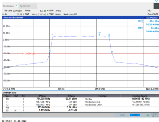
Band12-1.4MHz-64QAM-23173-6RB#0
