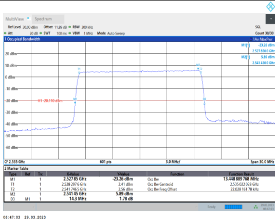
Band7-15MHz-64QAM-21100-75RB#0
