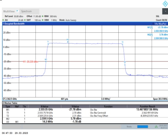
Band7-15MHz-64QAM-21375-75RB#0
