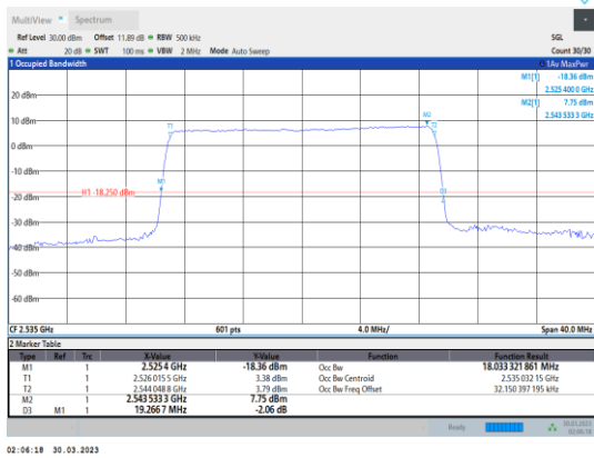
Band7-20MHz-16QAM-21100-100RB#0
