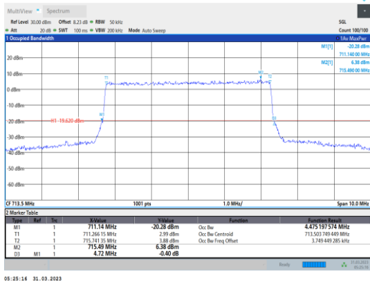
Band17-5MHz-64QAM-23825-25RB#0
