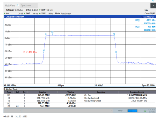
Band26-15MHz-64QAM-26865-75RB#0
