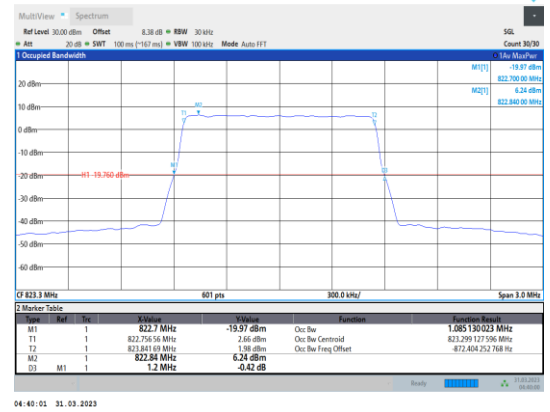
Band26-1.4MHz-16QAM-26783-6RB#0
