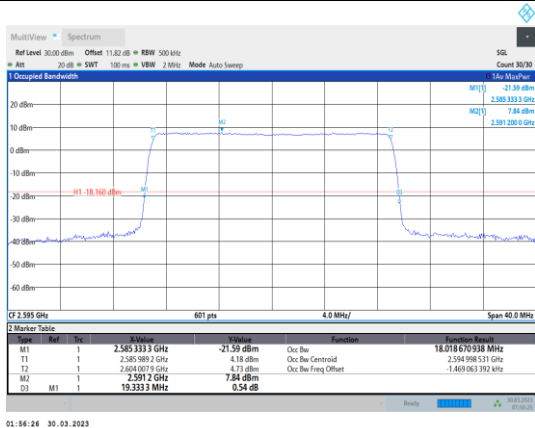
Band38-20MHz-16QAM-38000-100RB#0
