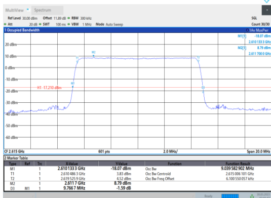
Band38-10MHz-16QAM-38200-50RB#0
