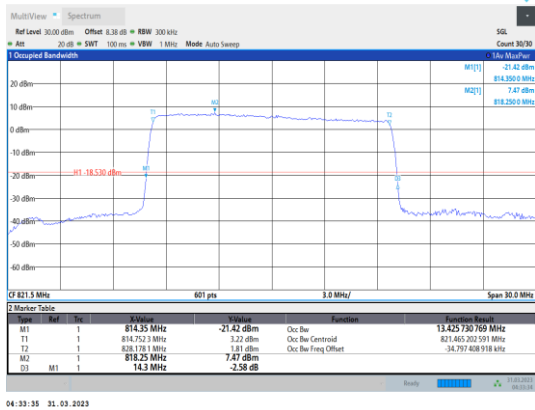
Band26-15MHz-64QAM-26765-75RB#0
