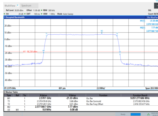
Band38-10MHz-64QAM-37800-50RB#0
