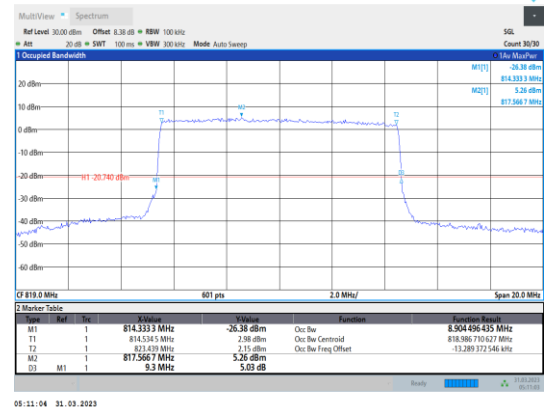
Band26-10MHz-64QAM-26740-50RB#0
