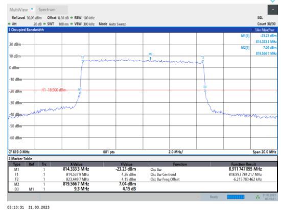
Band26-10MHz-QPSK-26740-50RB#0
