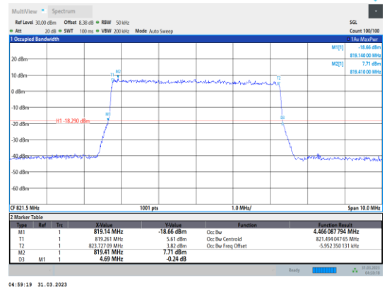
Band26-5MHz-16QAM-26765-25RB#0
