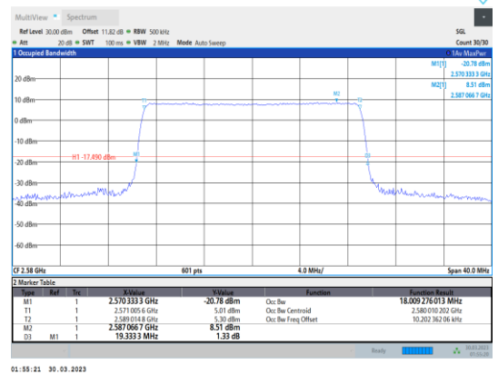
Band38-20MHz-QPSK-37850-100RB#0
