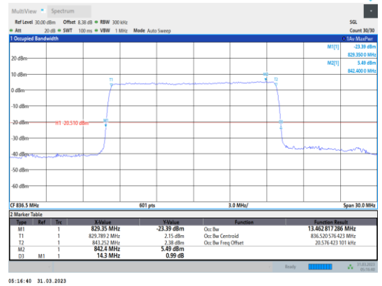
Band26-15MHz-64QAM-26915-75RB#0
