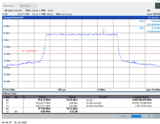
Band26-5MHz-QPSK-26715-25RB#0
