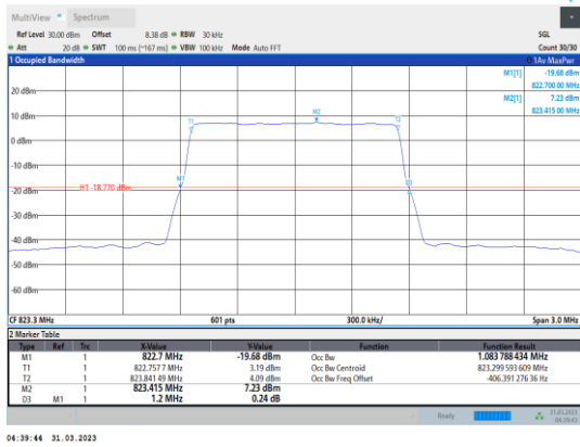
Band26-1.4MHz-QPSK-26783-6RB#0
