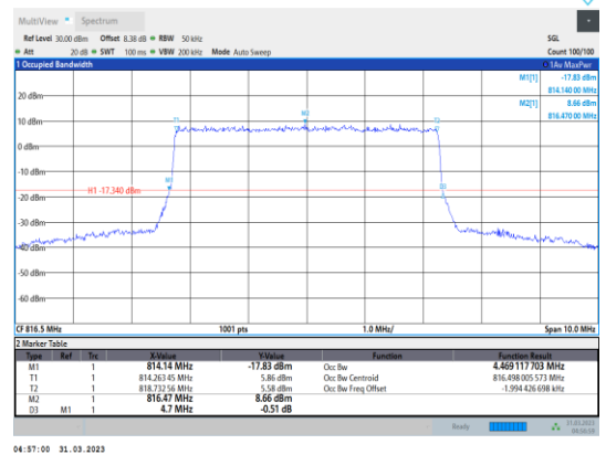
Band26-5MHz-16QAM-26715-25RB#0
