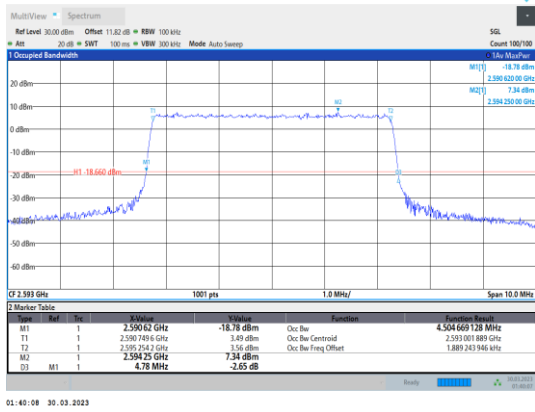
Band41-5MHz-64QAM-40620-25RB#0
