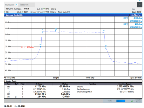
Band26-3MHz-QPSK-26740-15RB#0
