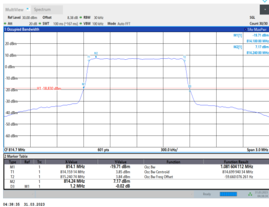
Band26-1.4MHz-64QAM-26697-6RB#0
