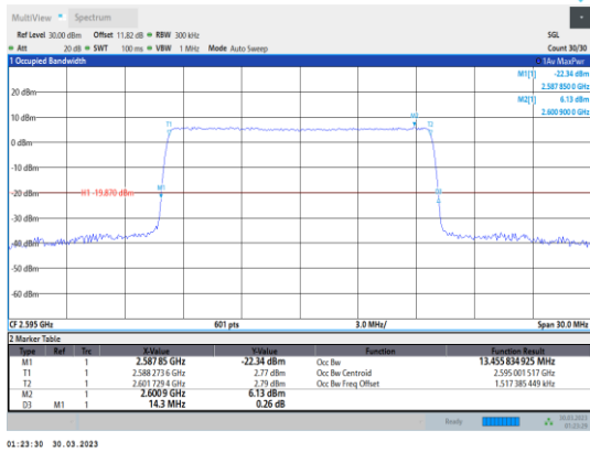
Band38-15MHz-64QAM-38000-75RB#0
