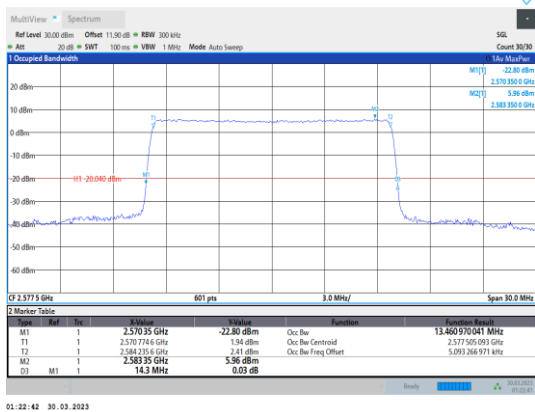
Band38-15MHz-64QAM-37825-75RB#0
