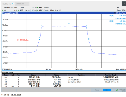
Band26-1.4MHz-QPSK-26740-6RB#0
