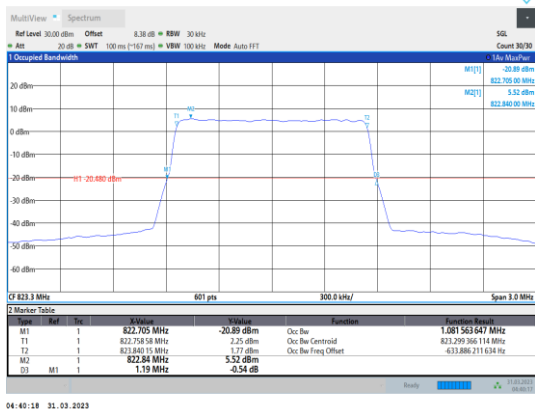
Band26-1.4MHz-64QAM-26783-6RB#0
