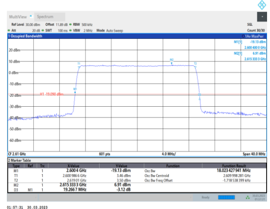
Band38-20MHz-64QAM-38150-100RB#0
