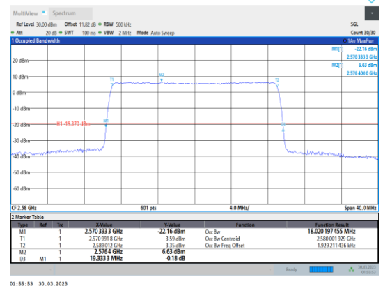
Band38-20MHz-64QAM-37850-100RB#0
