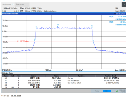
Band26-5MHz-64QAM-26715-25RB#0
