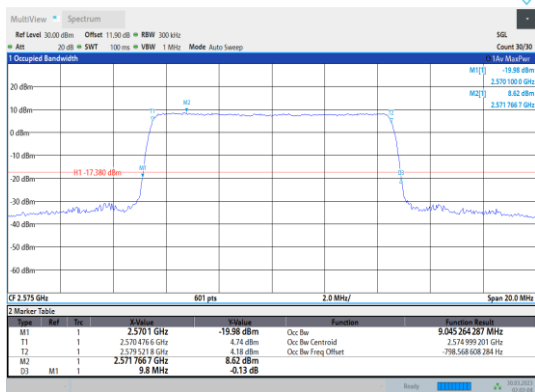
Band38-10MHz-16QAM-37800-50RB#0
