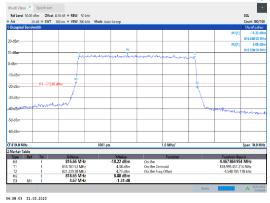
Band26-5MHz-16QAM-26740-25RB#0
