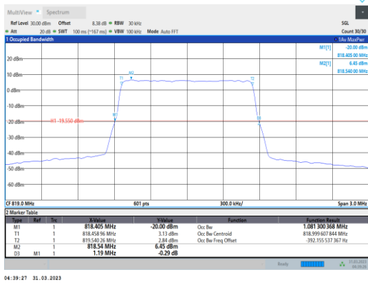
Band26-1.4MHz-64QAM-26740-6RB#0
