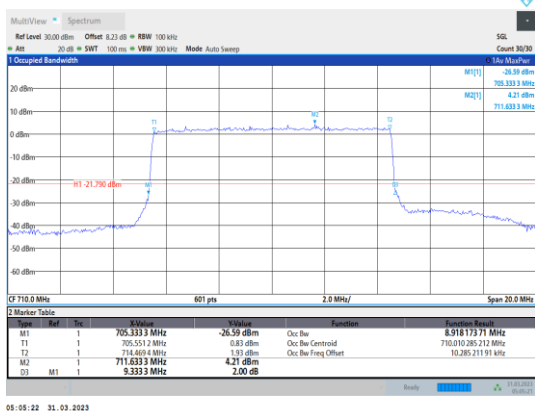
Band17-10MHz-16QAM-23790-50RB#0
