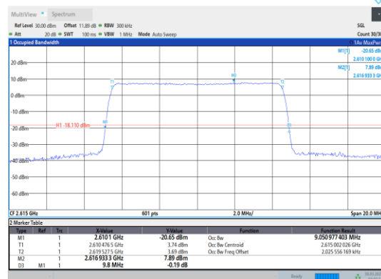
Band38-10MHz-64QAM-38200-50RB#0
