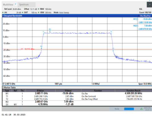
Band41-5MHz-64QAM-41565-25RB#0
