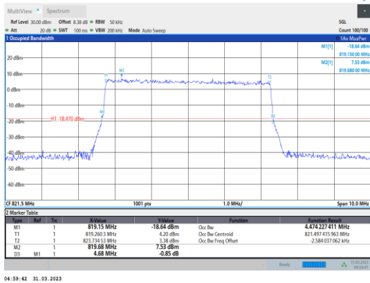
Band26-5MHz-64QAM-26765-25RB#0
