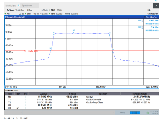
Band26-1.4MHz-16QAM-26697-6RB#0
