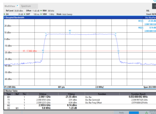
Band38-10MHz-64QAM-38000-50RB#0
