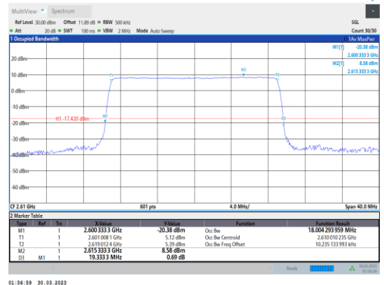
Band38-20MHz-QPSK-38150-100RB#0
