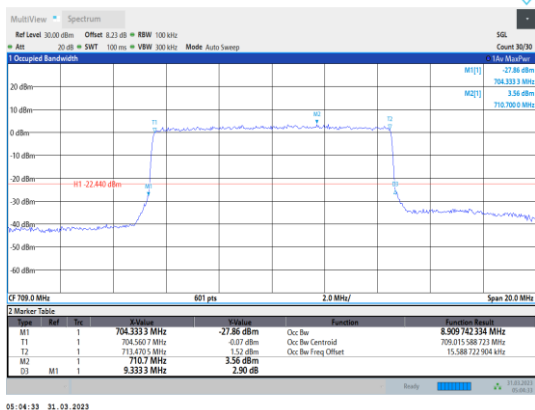
Band17-10MHz-16QAM-23780-50RB#0
