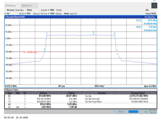
Band26-3MHz-QPSK-26705-15RB#0
