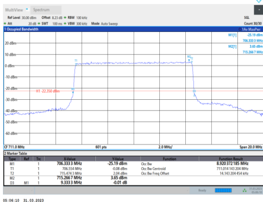
Band17-10MHz-16QAM-23800-50RB#0
