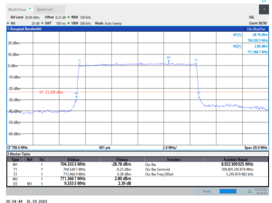
Band17-10MHz-64QAM-23780-50RB#0
