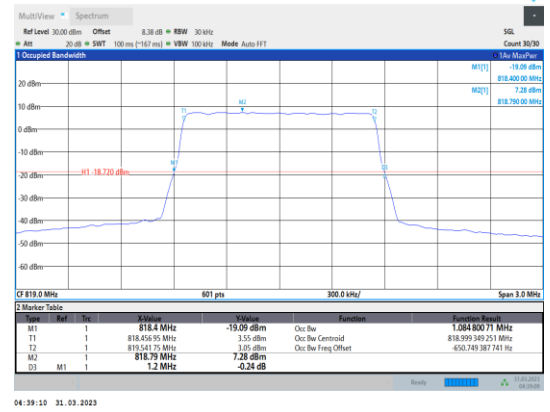
Band26-1.4MHz-16QAM-26740-6RB#0
