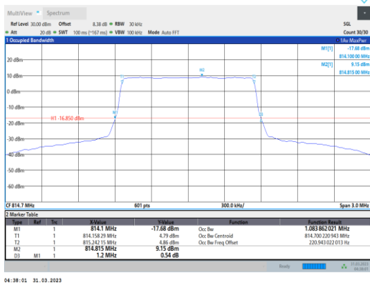
Band26-1.4MHz-QPSK-26697-6RB#0
