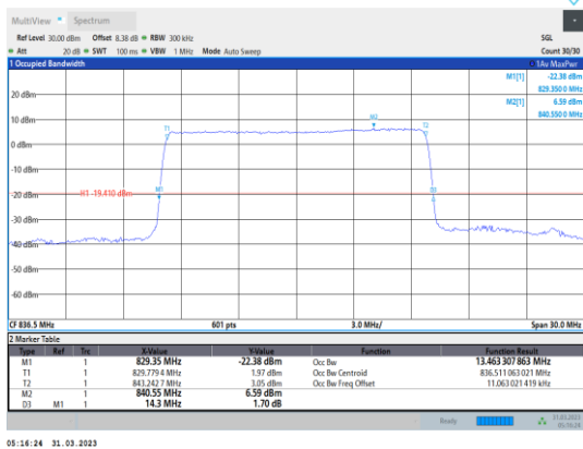
Band26-15MHz-16QAM-26915-75RB#0
