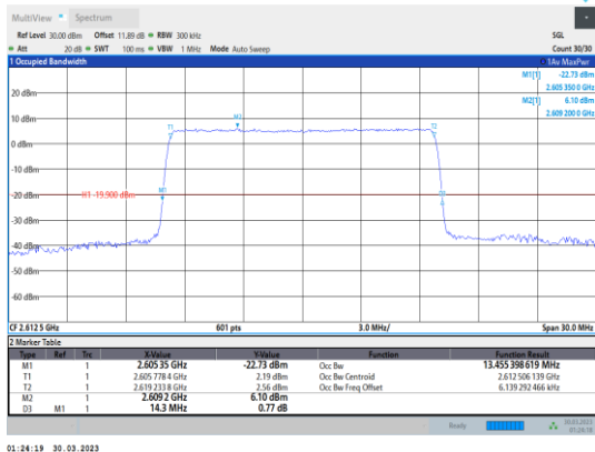
Band38-15MHz-64QAM-38175-75RB#0
