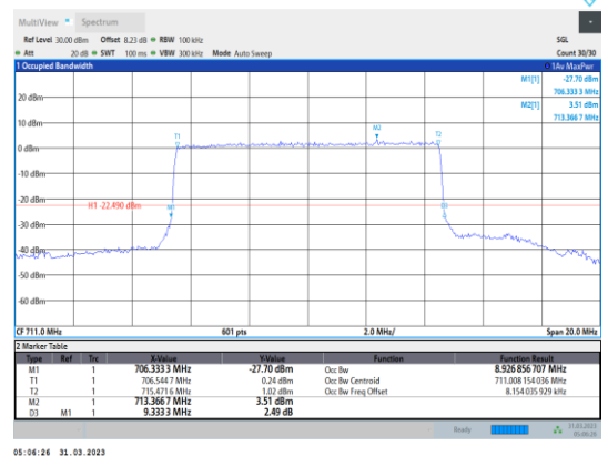
Band17-10MHz-64QAM-23800-50RB#0
