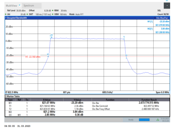
Band26-3MHz-QPSK-26775-15RB#0
