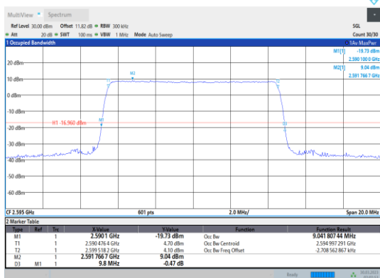
Band38-10MHz-16QAM-38000-50RB#0
