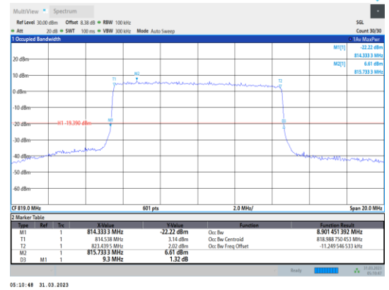
Band26-10MHz-16QAM-26740-50RB#0
