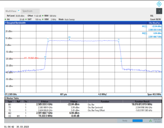
Band38-20MHz-64QAM-38000-100RB#0
