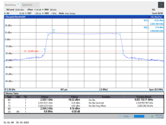
Band41-10MHz-QPSK-40290-50RB#0
