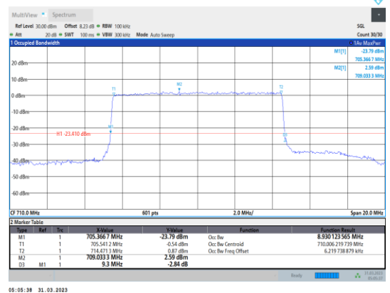
Band17-10MHz-64QAM-23790-50RB#0
