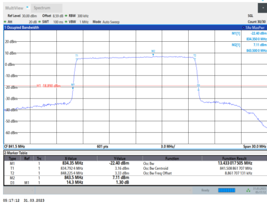
Band26-15MHz-16QAM-26965-75RB#0
