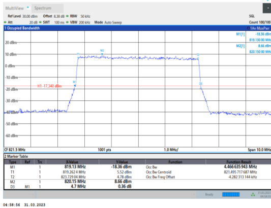
Band26-5MHz-QPSK-26765-25RB#0
