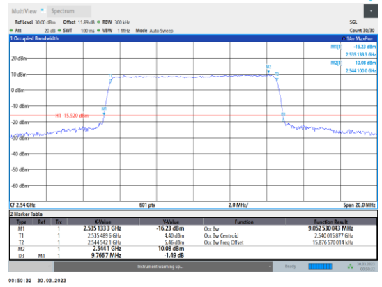
Band41-10MHz-QPSK-40090-50RB#0
