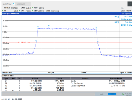
Band26-5MHz-64QAM-26740-25RB#0
