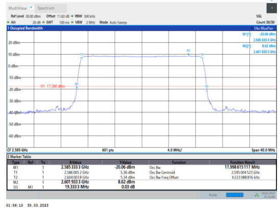
Band38-20MHz-QPSK-38000-100RB#0
