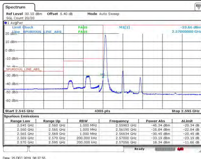
Band38_10MHz_QPSK_37800_50RB#0
