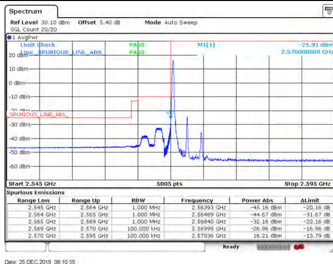
Band38_5MHz_64QAM_3775_25RB#0
