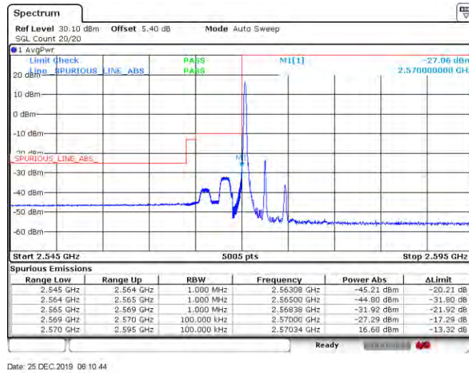
Band38_5MHz_16QAM_3775_25RB#0
