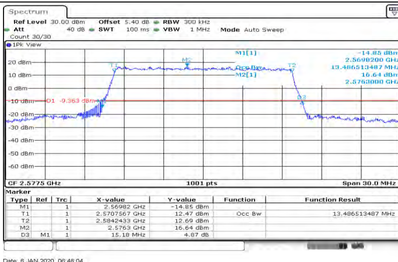
Band38-15MHz-QPSK-38000-75RB#0-13.487
