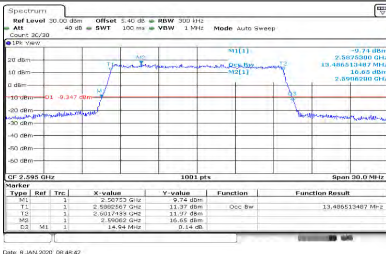
Band38-15MHz-QPSK-38175-75RB#0-13.487
