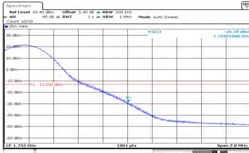
Band4-15MHz-16QAM-20325-75RB#0
