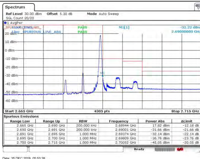
Band41_10MHz_16QAM_41540_50RB#0
