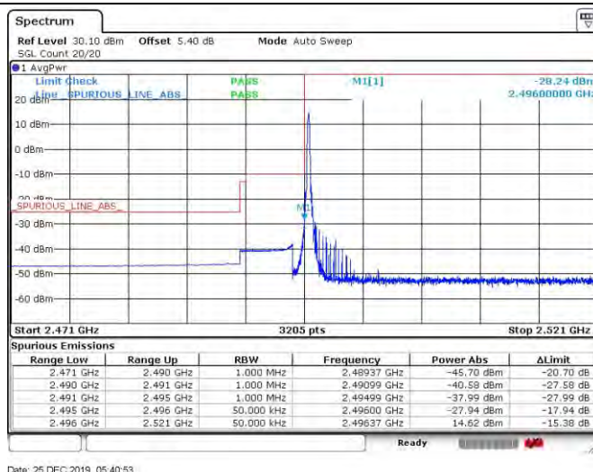
Band41_5MHz_64QAM_39675_25RB#0
