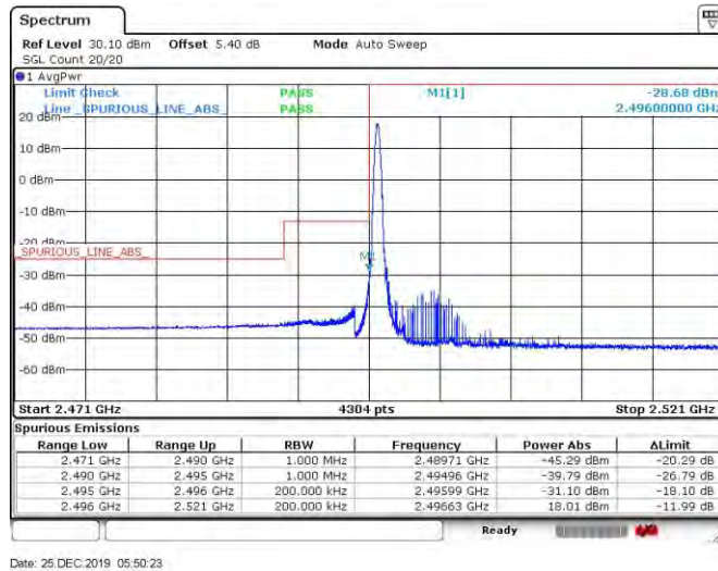
Band41_10MHz_64QAM_39700_50RB#0
